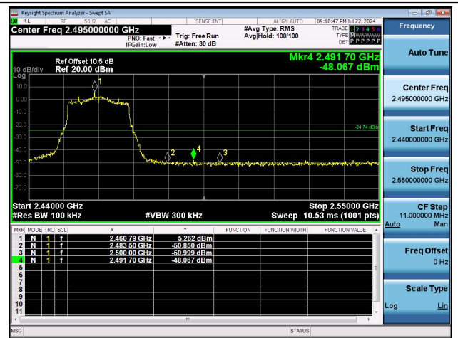
11AX20MIMO-Ant1-2462-PASS
