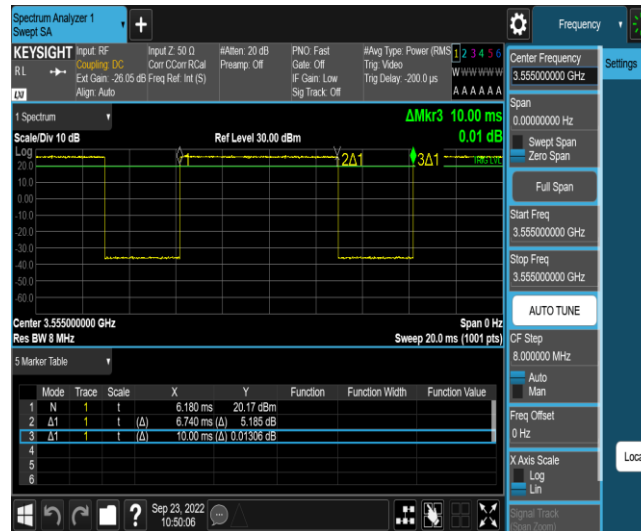
Band48-10MHz-64QAM-55290-E-TM3.1
