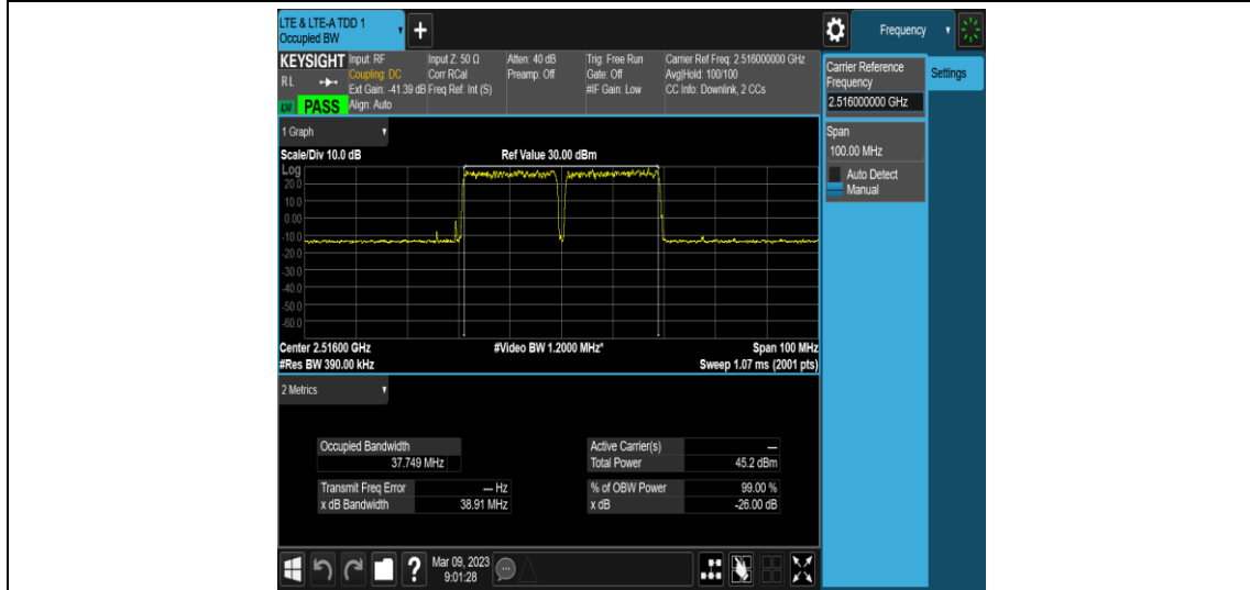
Band41-40MHz-256QAM-Middle-E-TM3.1A
