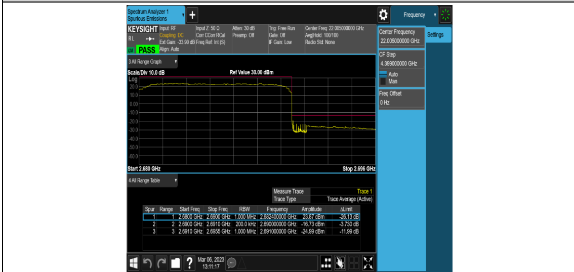
Band41-20MHz-256QAM-Highest-E-TM3.1A-2690.00~2691.00
