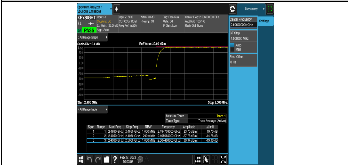
Band41-20MHz-QPSK-Lowest-E-TM1.1-2486.00~2495.00
