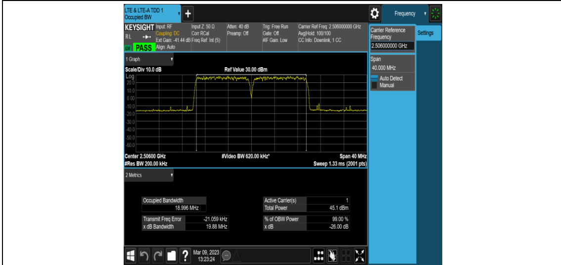
Band41-20MHz-256QAM-Middle-E-TM3.1A
