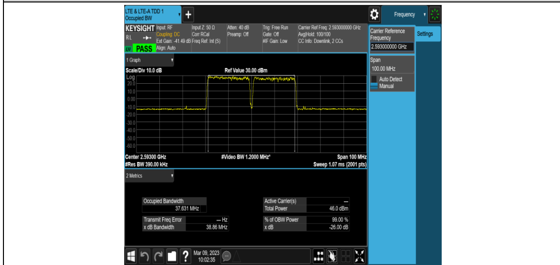
Band41-40MHz-256QAM-Middle-E-TM3.1A
