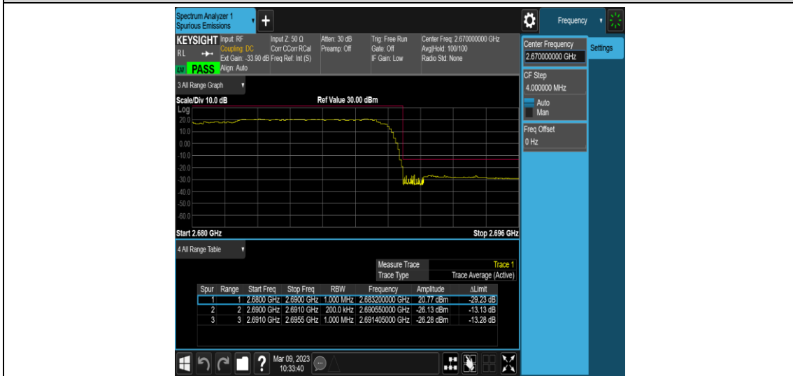
Band41-40MHz-256QAM-Highest-E-TM3.1A-2690.00~2691.00
