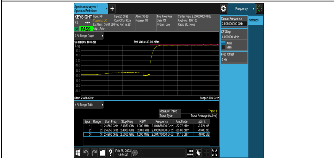
Band41-20MHz-QPSK-Lowest-E-TM1.1-2486.00~2495.00
