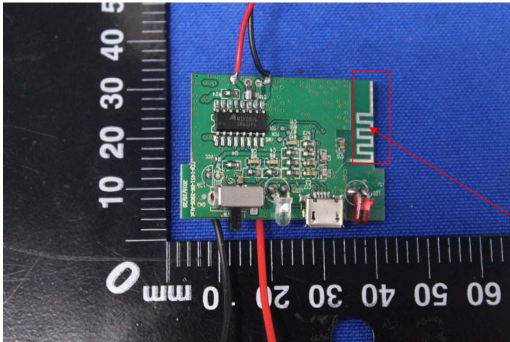
BT Antenna
