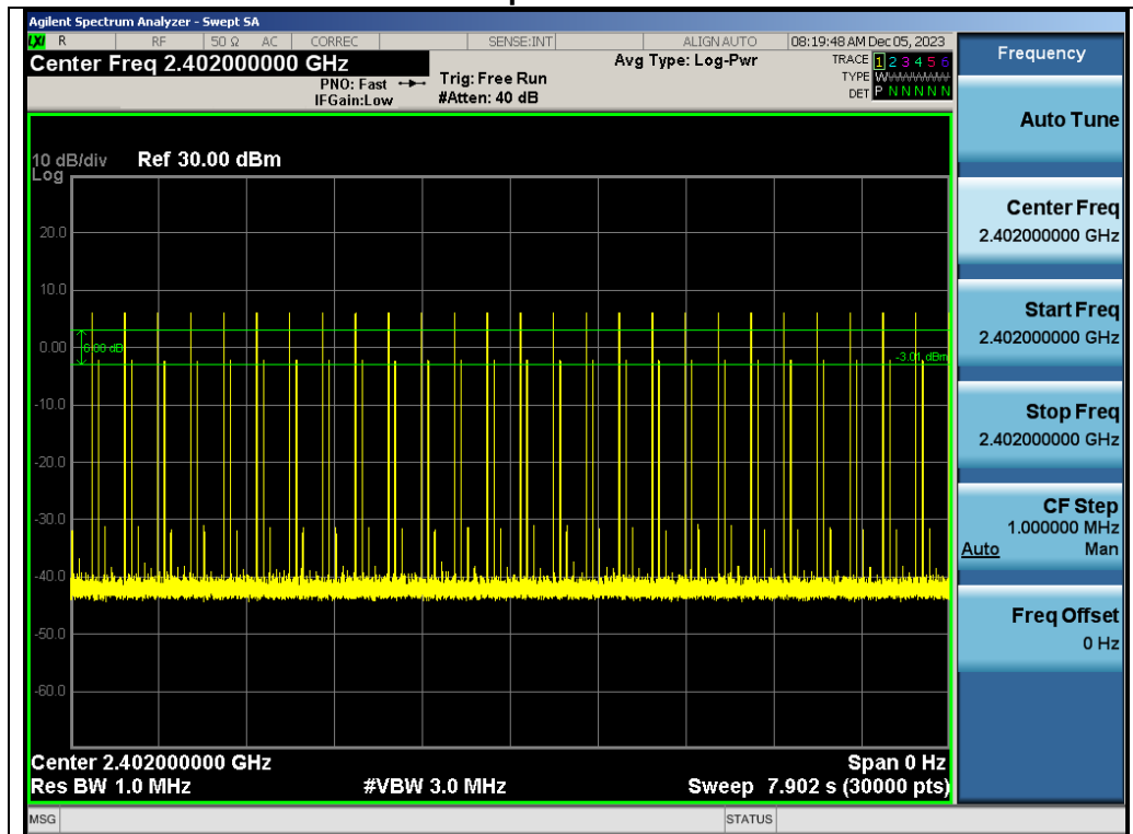
Test_Graph_GFSK_HOP_ANT1_NA_1Mbps_2402_Number of Burst
