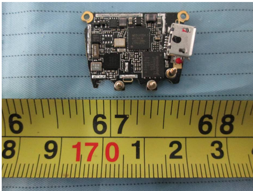
EUT – BT & WIFI Main Board Top View
