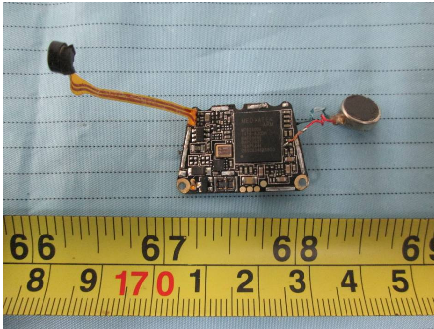
EUT –GSM Main Board Bottom View
