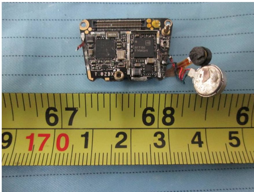
EUT – GSM Main Board Top View
