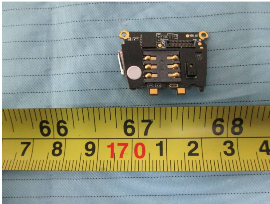
EUT –BT & WIFI Main Board Bottom View
