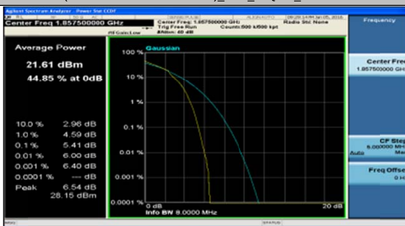
(Channel Bandwidth 15 MHz)_LCH_16QAM_37RB#38
