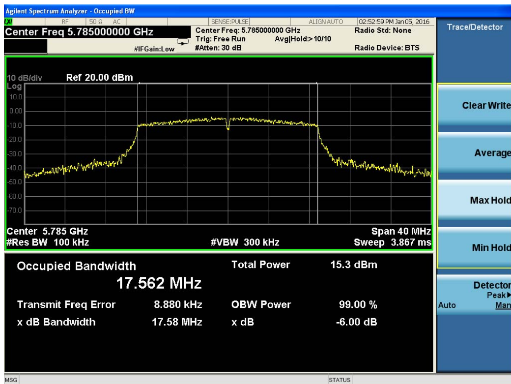
Test Plot For 802.11ac(VHT20)-6dB BW-5785M
