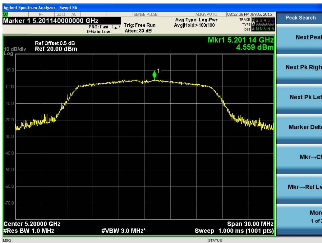
Test Plot For 802.11a-5200M
