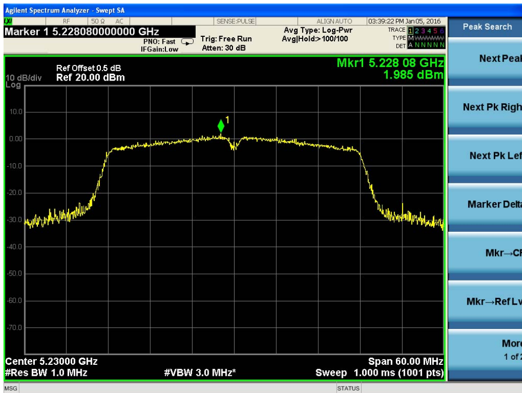
Test Plot For 802.11ac(VHT40)-5230M
