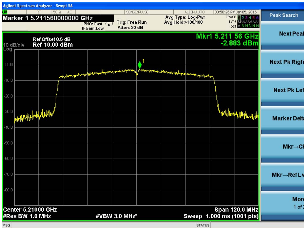
Test Plot For 802.11ac(VHT80)-5210M
