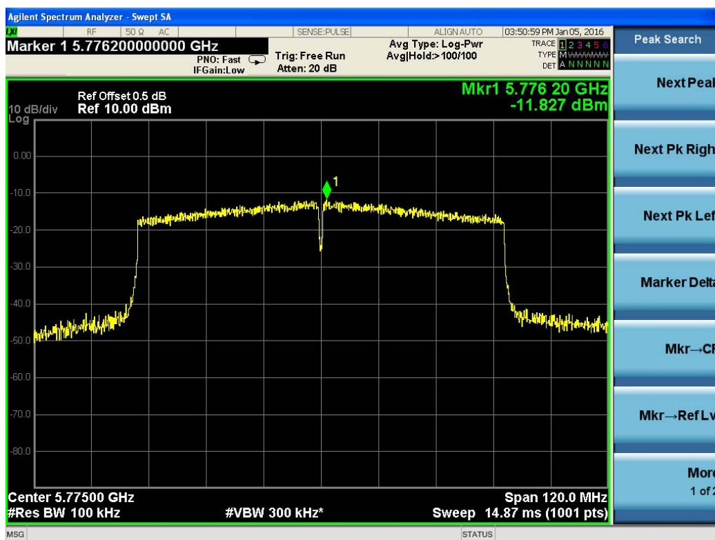
Test Plot For 802.11ac(VHT80)-5775M
