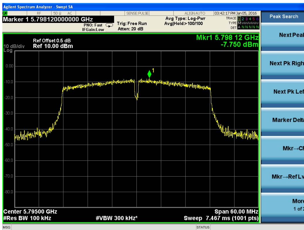
Test Plot For 802.11ac(VHT40)-5795M
