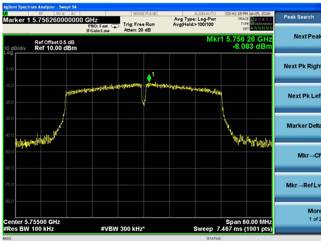
Test Plot For 802.11ac(VHT40)-5755M
