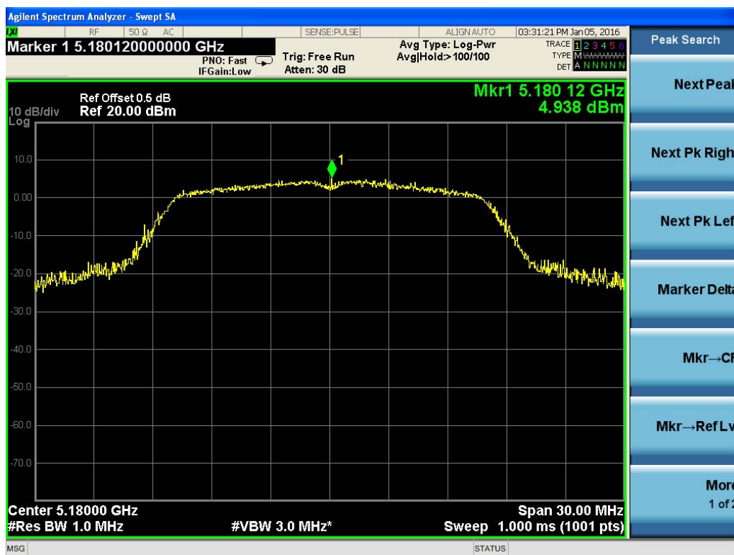
Test Plot For 802.11a-5180M
