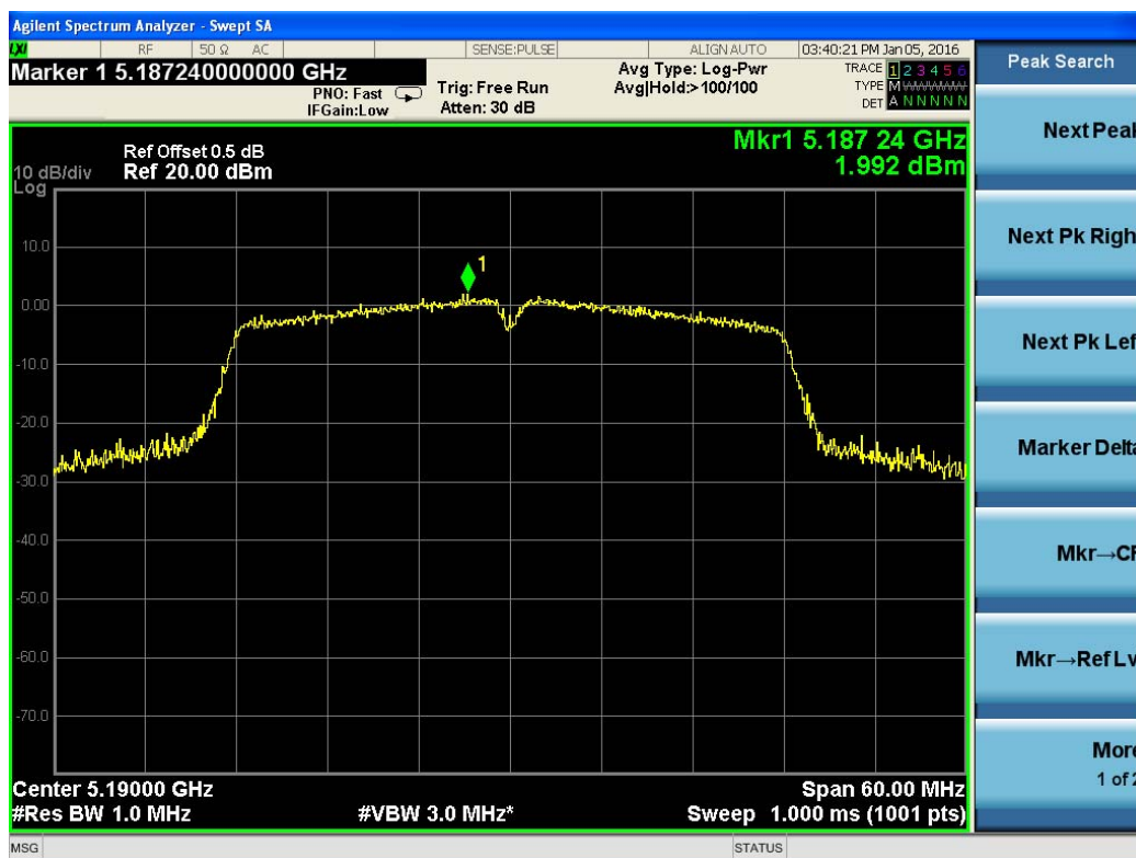
Test Plot For 802.11n(HT40)-5190M
