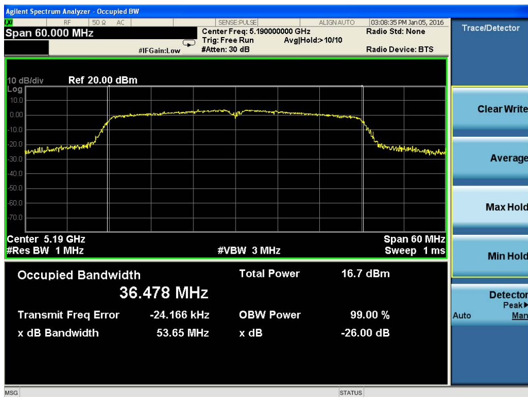
Test Plot For 802.11ac(VHT40)-26dB BW-5190M
