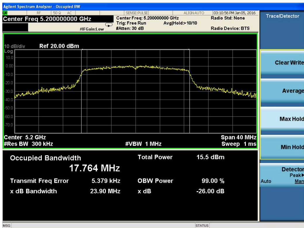
Test Plot For 802.11ac(VHT20)-26dB BW-5200M
