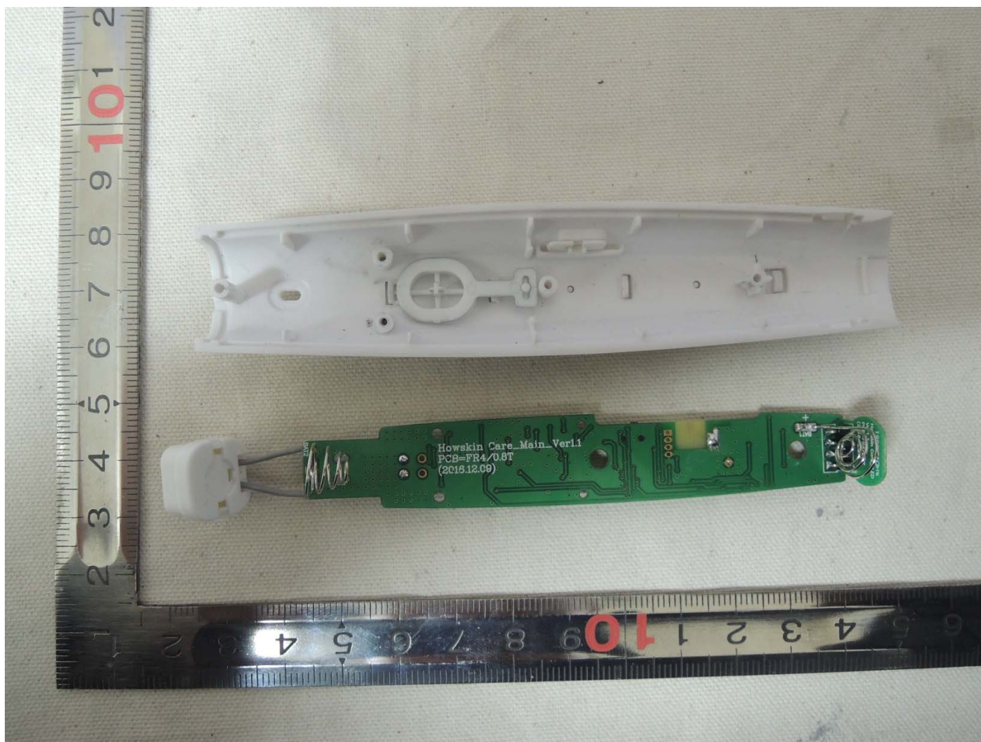
Removed Main Board
