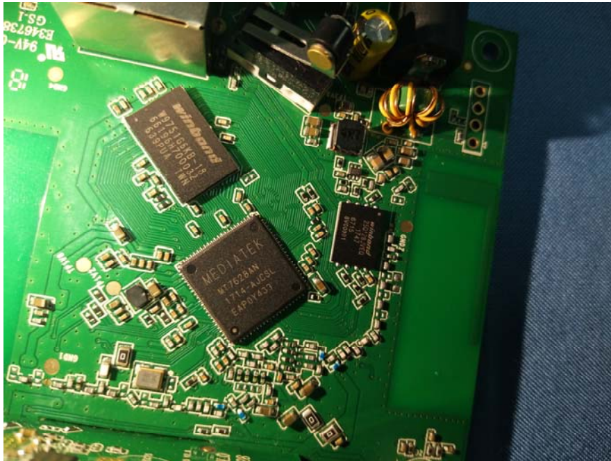
EUT – Wi-Fi Main Chip View
