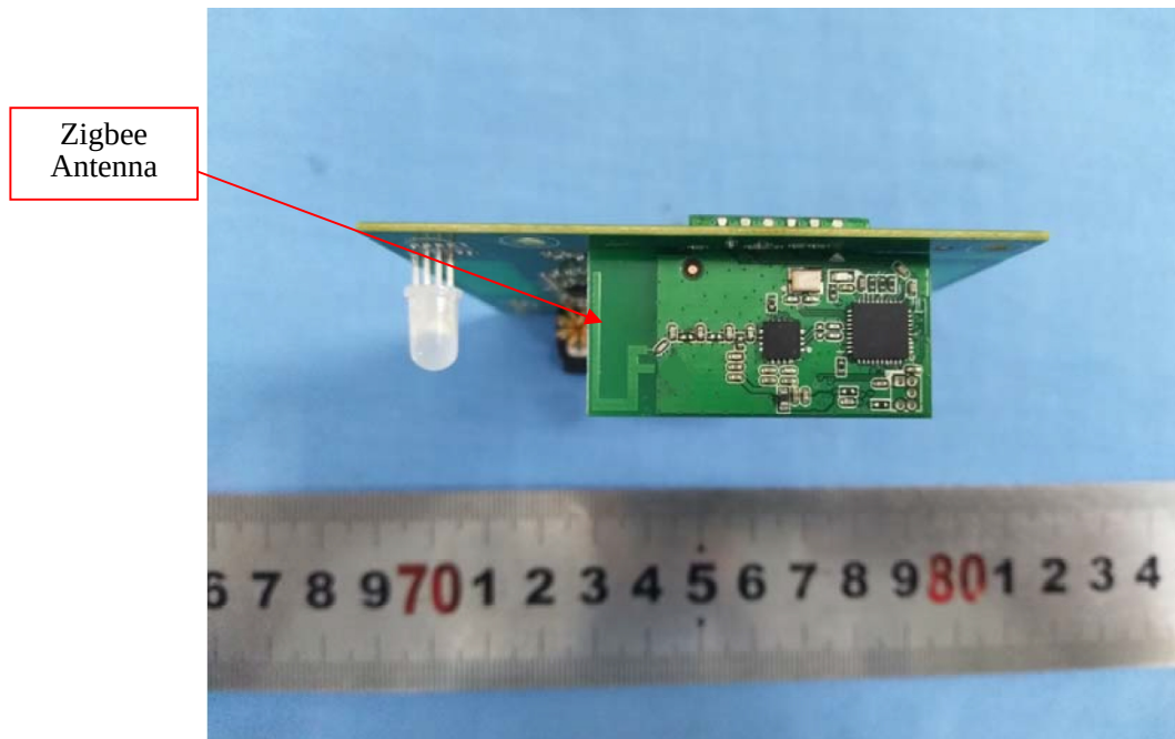
EUT – Zigbee Module Top View
