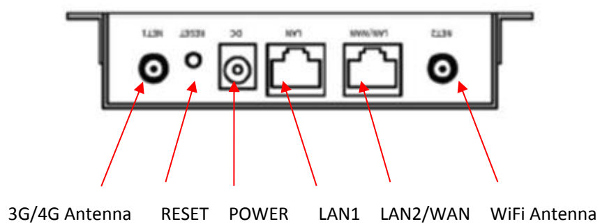
Figure 2-5 Back pannel
