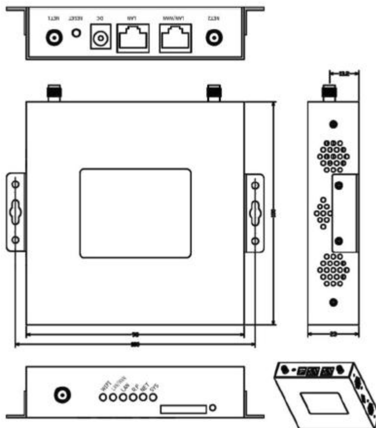
Figure 2-3 H8951 3G 4G router Figure
