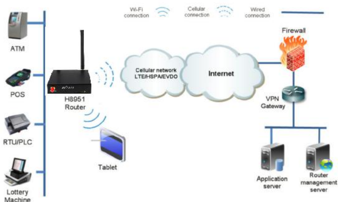
Figure 1-1 Network structure
