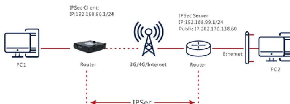
Figure 6-5 Build IPsec
