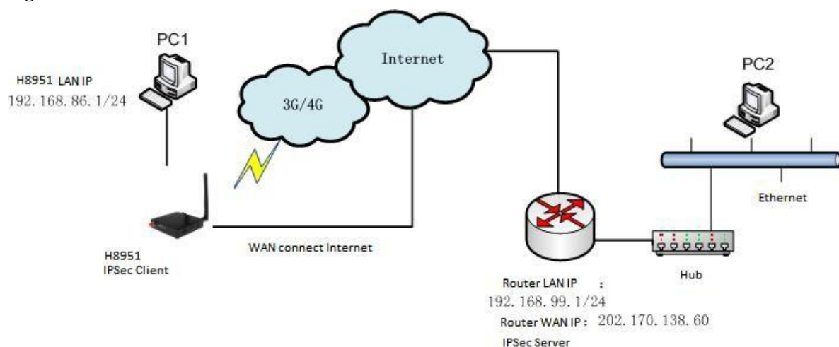
Figure 6-88 Build IPSec
