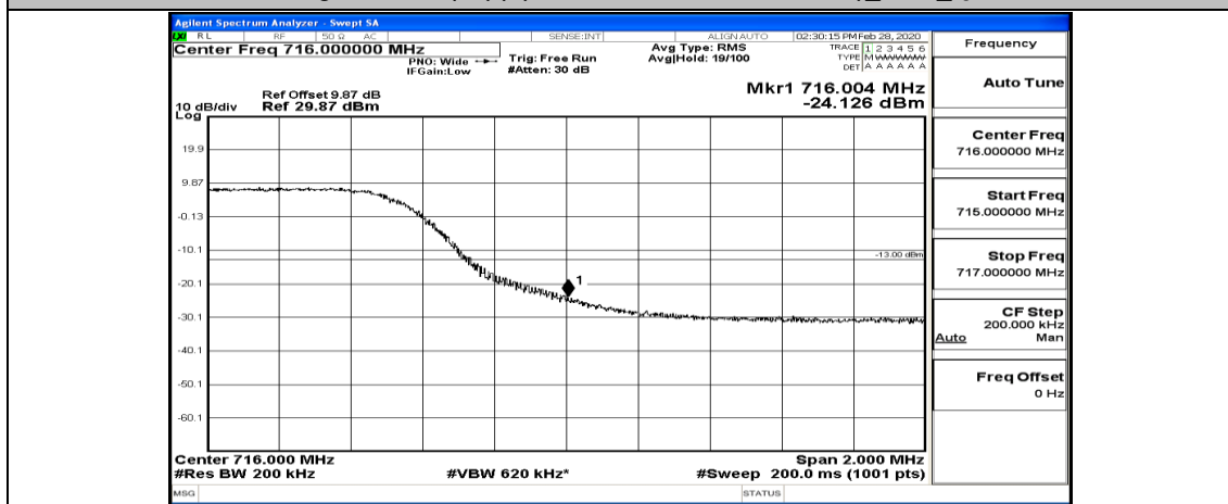
Band Edge Test Graph(s) (Channel Bandwidth: 10 MHz)_HCH_QPSK
