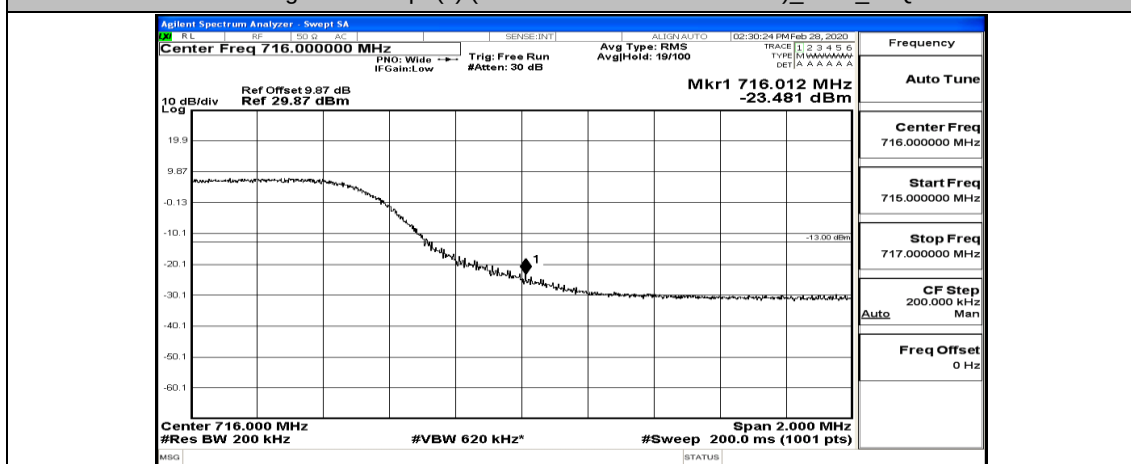
Band Edge Test Graph(s) (Channel Bandwidth: 10 MHz)_HCH_16QAM
