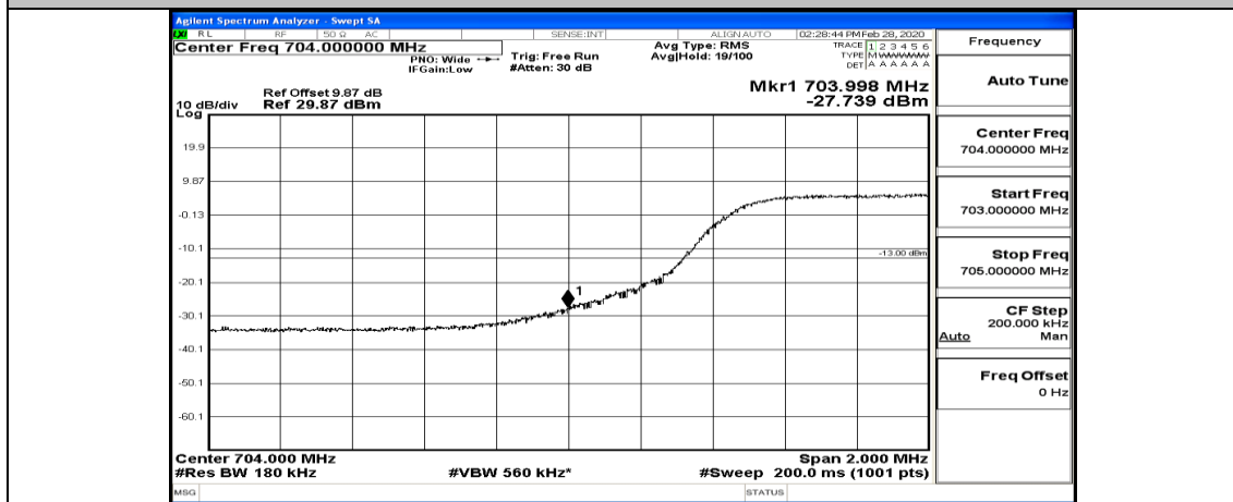
Band Edge Test Graph(s) (Channel Bandwidth: 10 MHz)_LCH_16QAM
