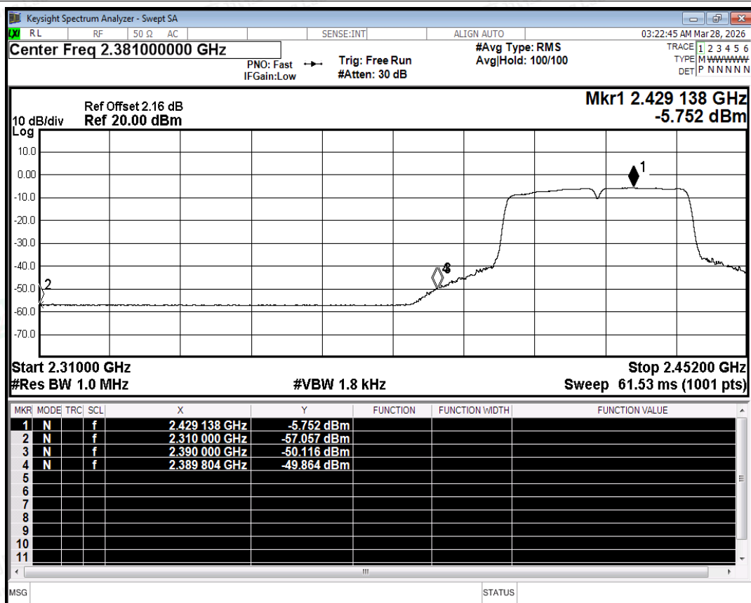
Restrict Band NVNT n40 2422MHz Ant1 Average
