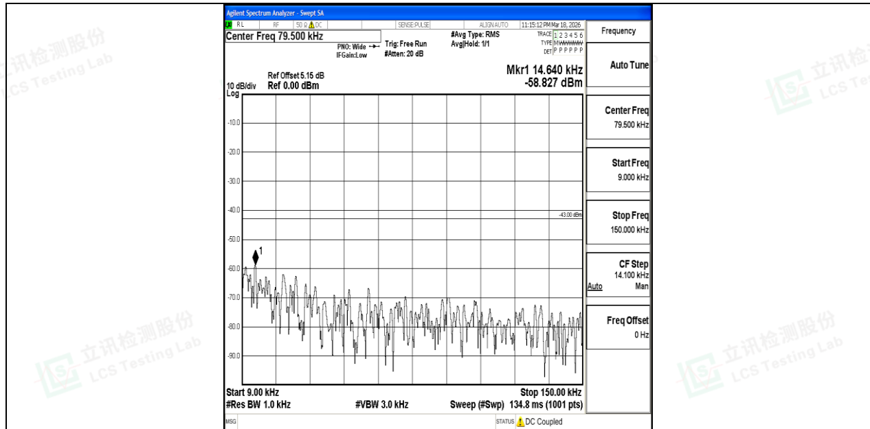
Band4_20MHz_QPSK_20175_1RB#0_0.009~0.15_0.009~0.15
