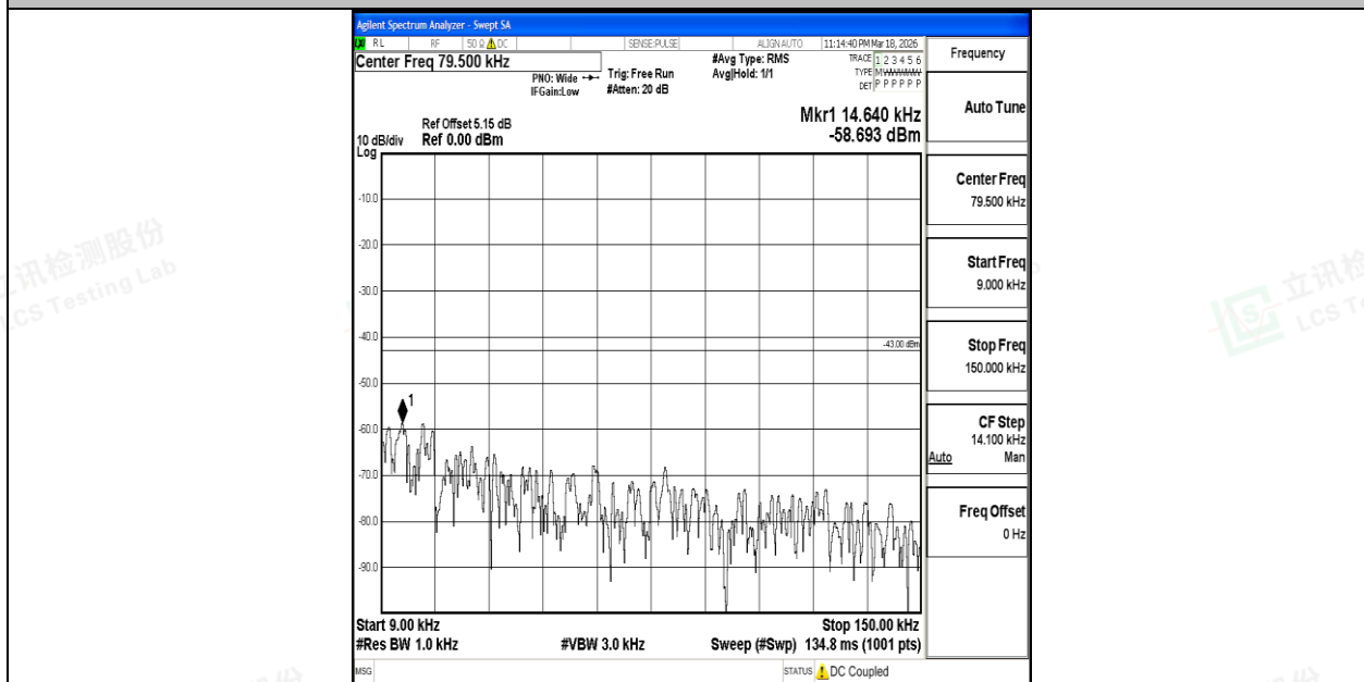
Band4_20MHz_16QAM_20050_1RB#0_0.009~0.15_0.009~0.15
