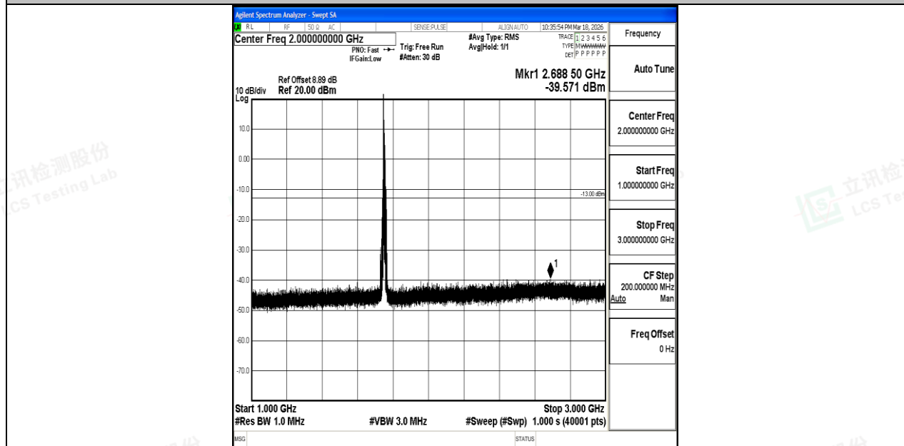
Band4_10MHz_QPSK_20350_1RB#0_1000~3000_1000~3000
