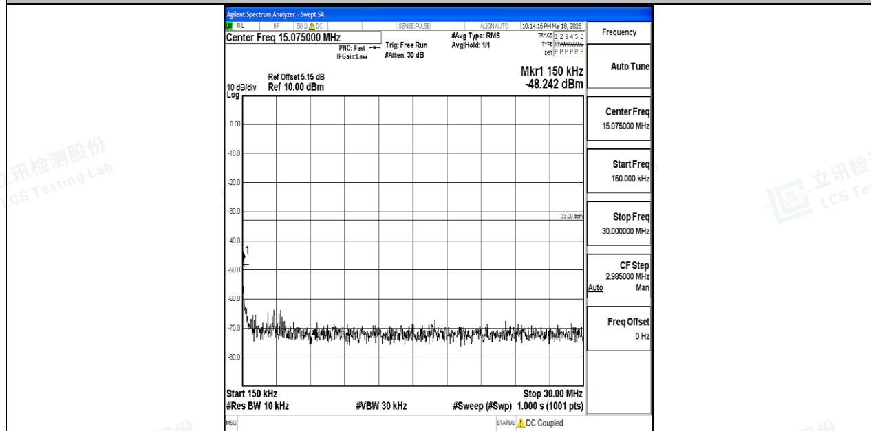
Band4_5MHz_QPSK_20375_1RB#0_0.15~30_0.15~30
