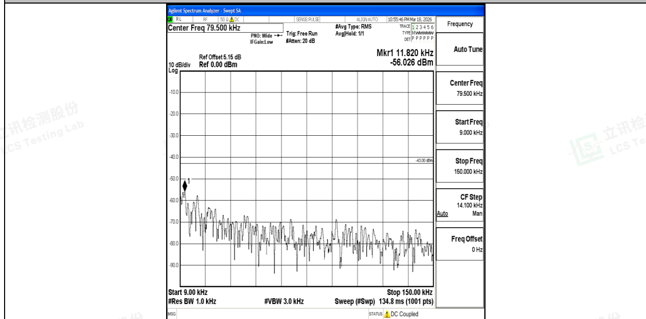
Band4_15MHz_16QAM_20175_1RB#0_0.009~0.15_0.009~0.15
