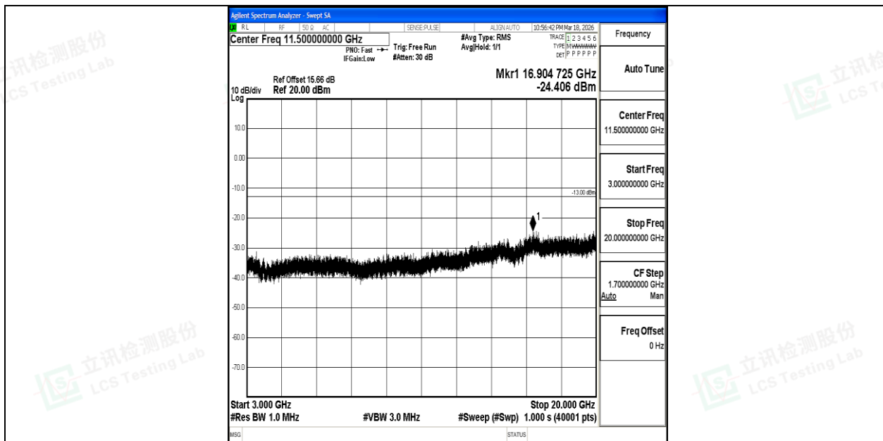
Band4_15MHz_QPSK_20325_1RB#0_3000~20000_3000~20000
