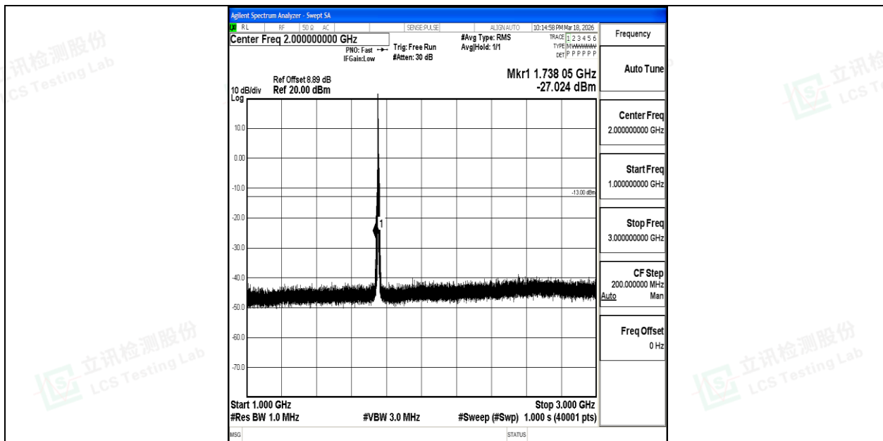
Band4_5MHz_16QAM_20375_1RB#0_1000~3000_1000~3000
