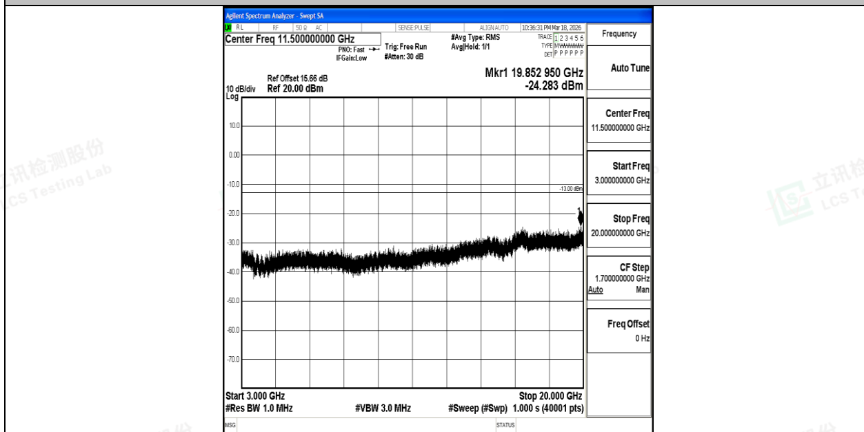
Band4_10MHz_16QAM_20350_1RB#0_3000~20000_3000~20000
