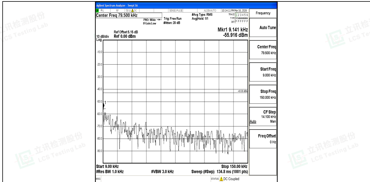
Band4_5MHz_QPSK_20375_1RB#0_0.009~0.15_0.009~0.15
