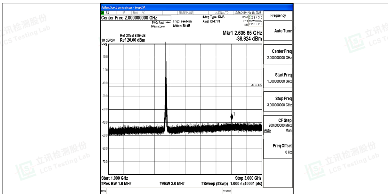
Band4_10MHz_16QAM_20350_1RB#0_1000~3000_1000~3000
