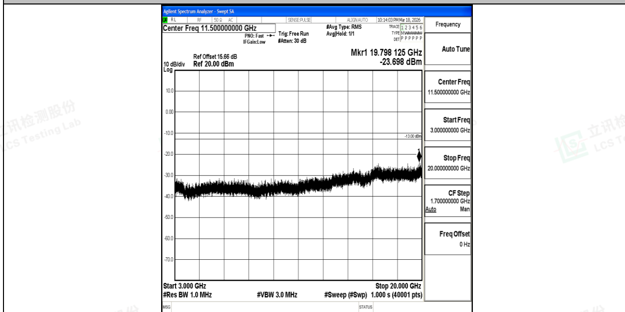
Band4_5MHz_16QAM_20175_1RB#0_3000~20000_3000~20000
