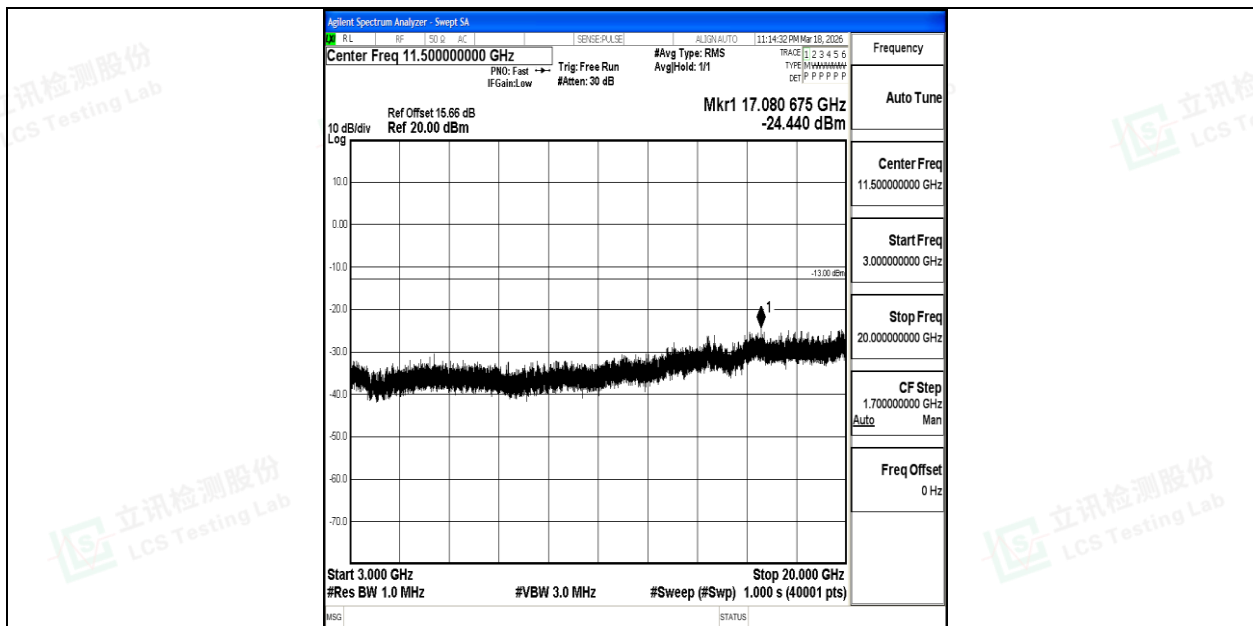
Band4_20MHz_QPSK_20050_1RB#0_3000~20000_3000~20000
