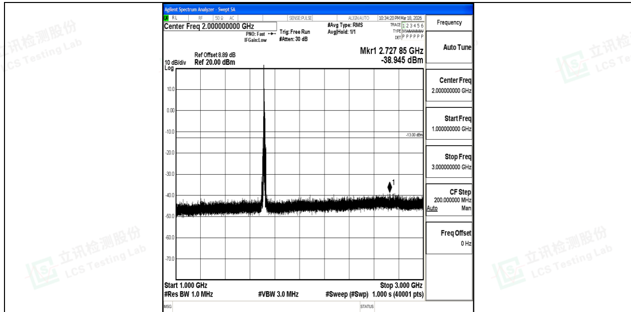
Band4_10MHz_16QAM_20000_1RB#0_1000~3000_1000~3000
