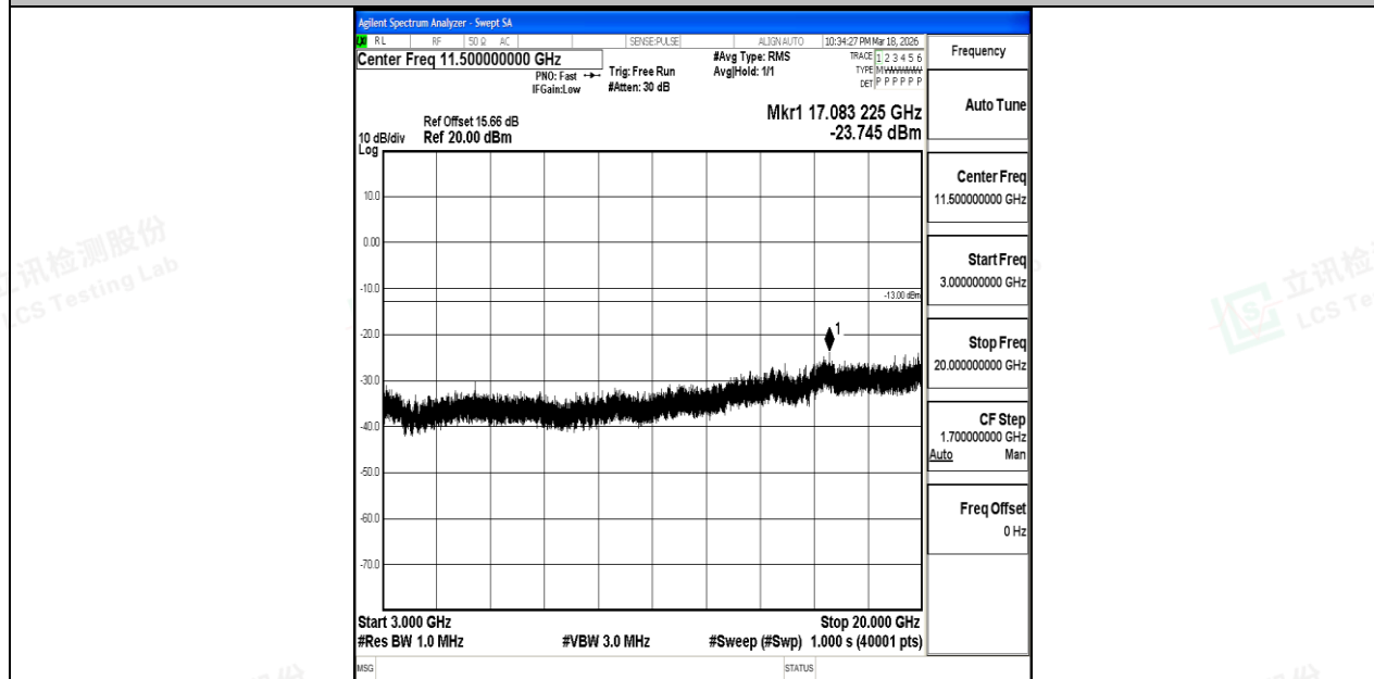
Band4_10MHz_16QAM_20000_1RB#0_3000~20000_3000~20000
