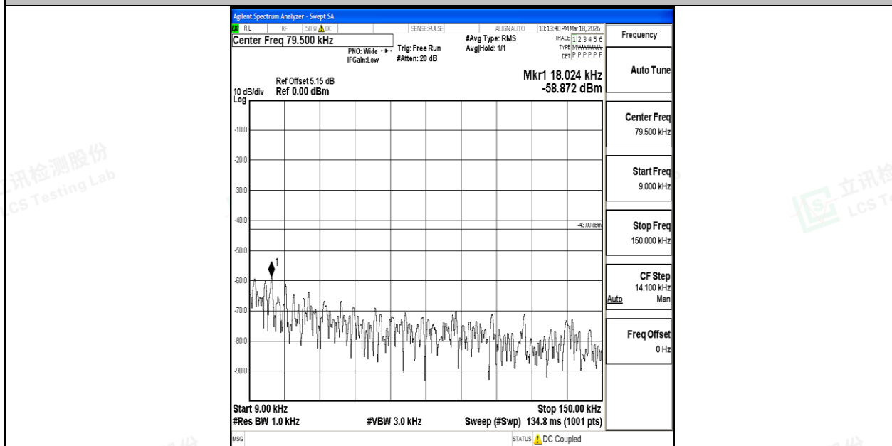
Band4_5MHz_16QAM_20175_1RB#0_0.009~0.15_0.009~0.15
