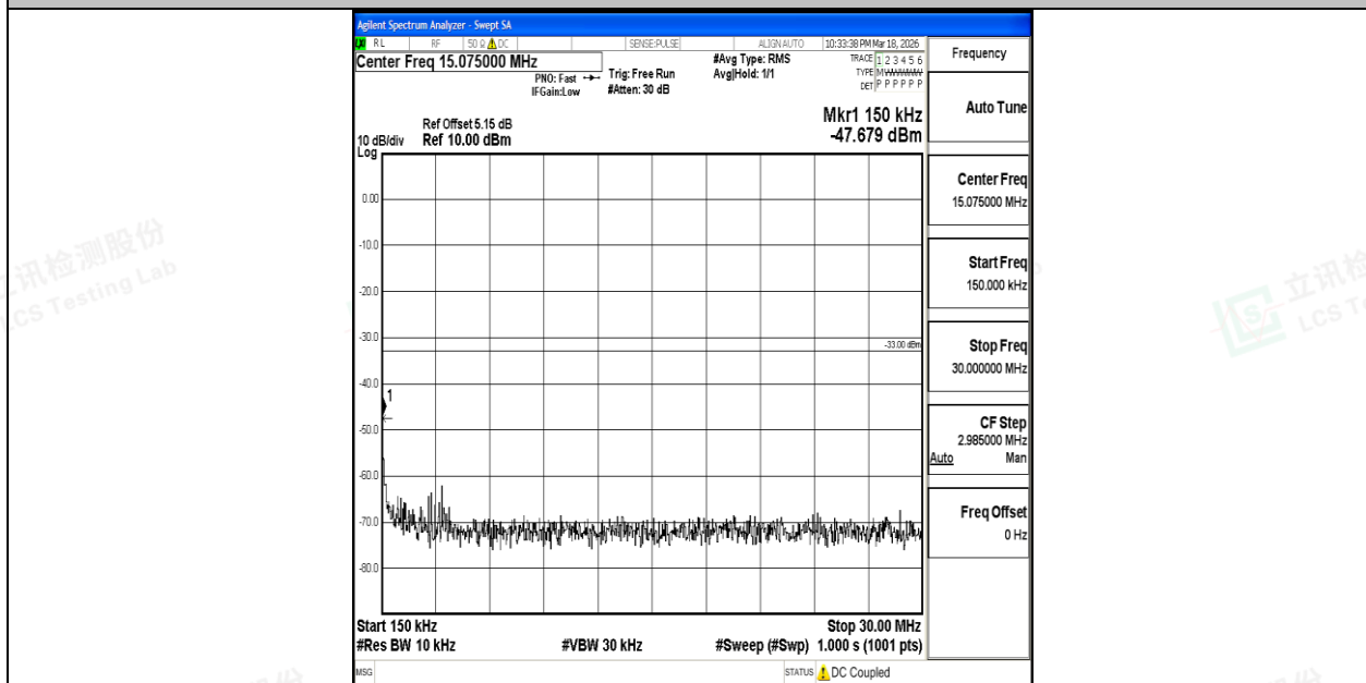
Band4_10MHz_QPSK_20000_1RB#0_0.15~30_0.15~30
