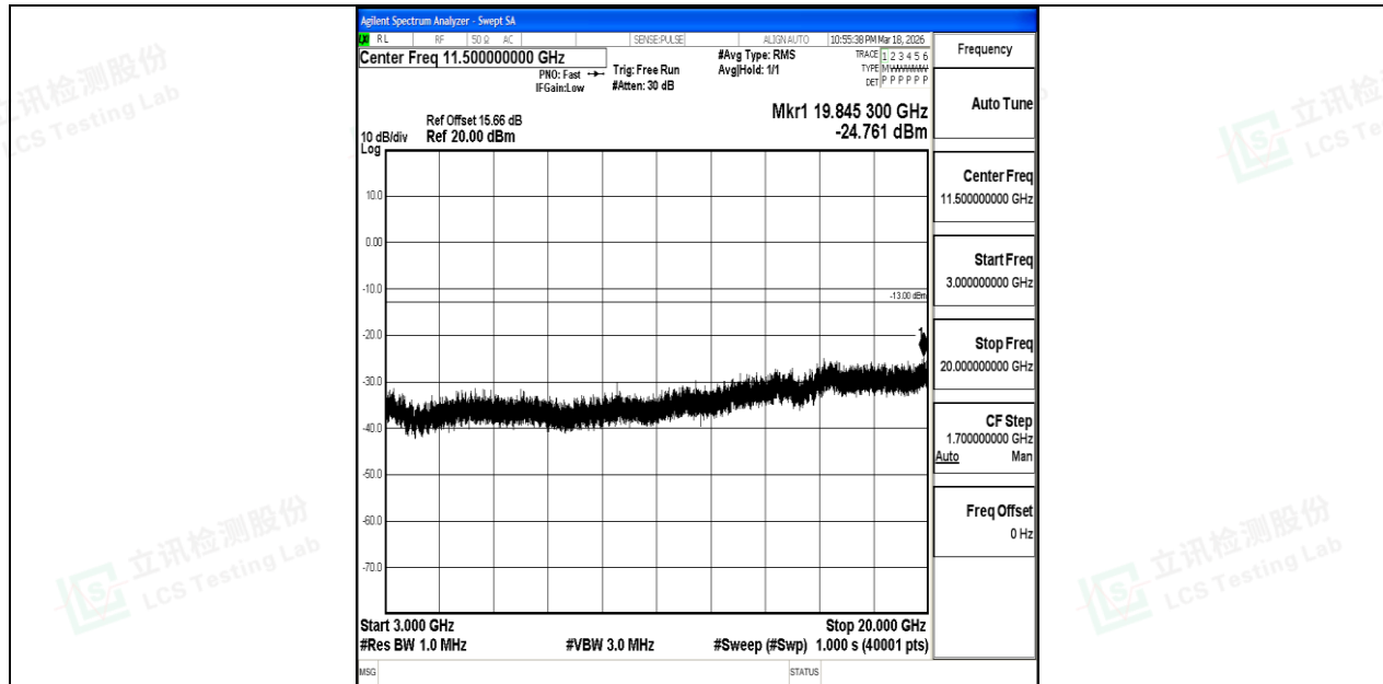
Band4_15MHz_QPSK_20175_1RB#0_3000~20000_3000~20000
