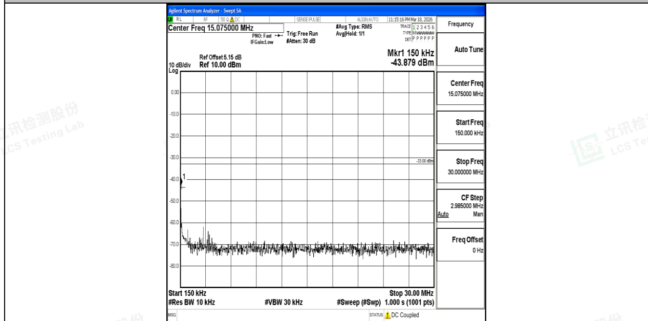
Band4_20MHz_QPSK_20175_1RB#0_0.15~30_0.15~30
