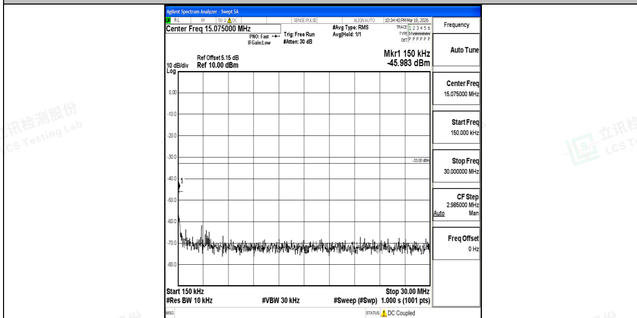
Band4_10MHz_QPSK_20175_1RB#0_0.15~30_0.15~30
