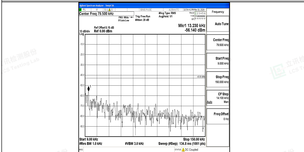
Band4_15MHz_16QAM_20025_1RB#0_0.009~0.15_0.009~0.15
