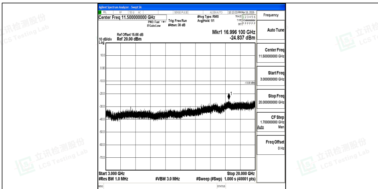
Band4_5MHz_QPSK_20175_1RB#0_3000~20000_3000~20000
