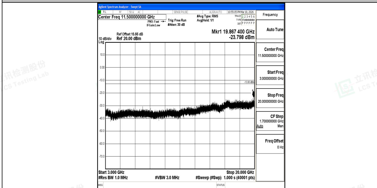
Band4_15MHz_16QAM_20025_1RB#0_3000~20000_3000~20000
