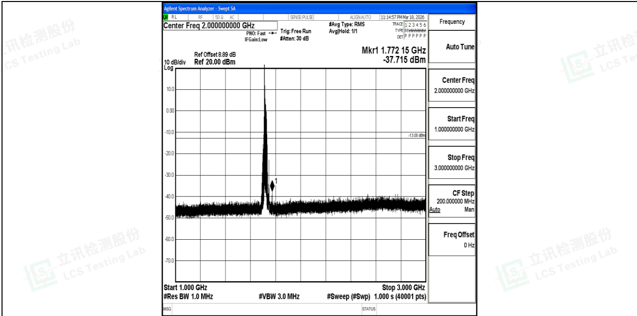
Band4_20MHz_16QAM_20050_1RB#0_1000~3000_1000~3000
