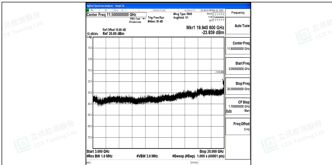
Band4_10MHz_QPSK_20350_1RB#0_3000~20000_3000~20000
