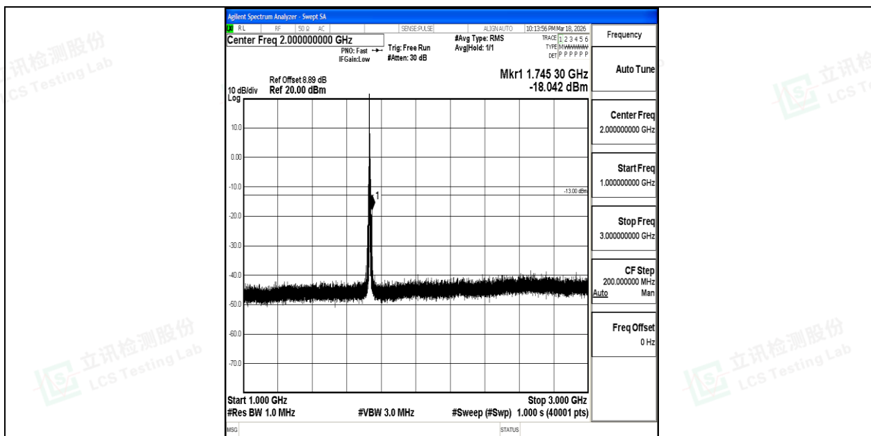
Band4_5MHz_16QAM_20175_1RB#0_1000~3000_1000~3000
