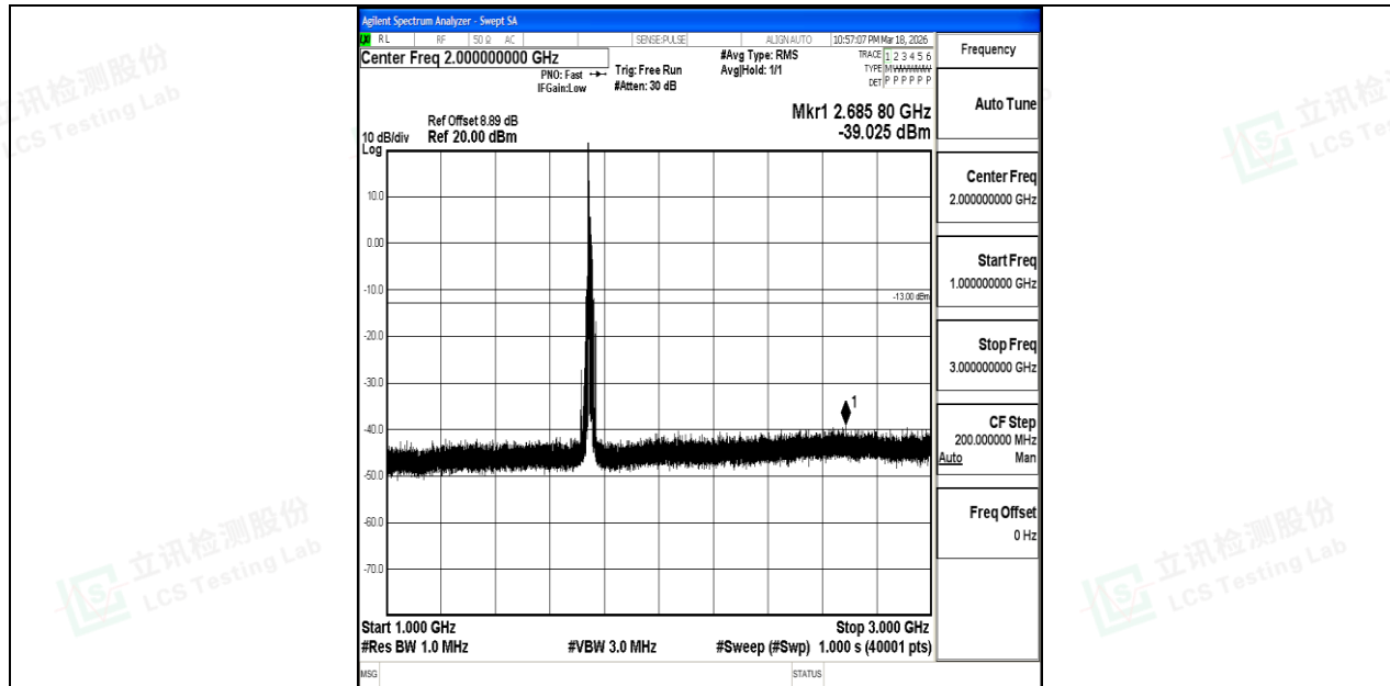
Band4_15MHz_16QAM_20325_1RB#0_1000~3000_1000~3000
