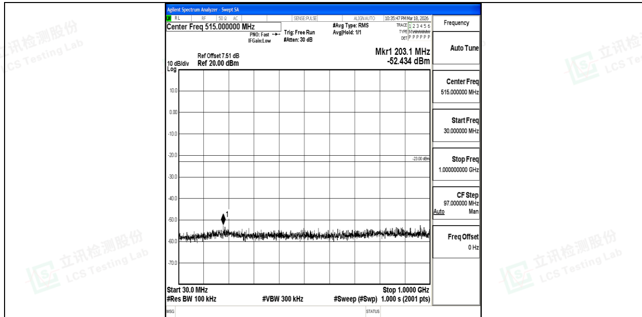
Band4_10MHz_QPSK_20350_1RB#0_30~1000_30~1000
