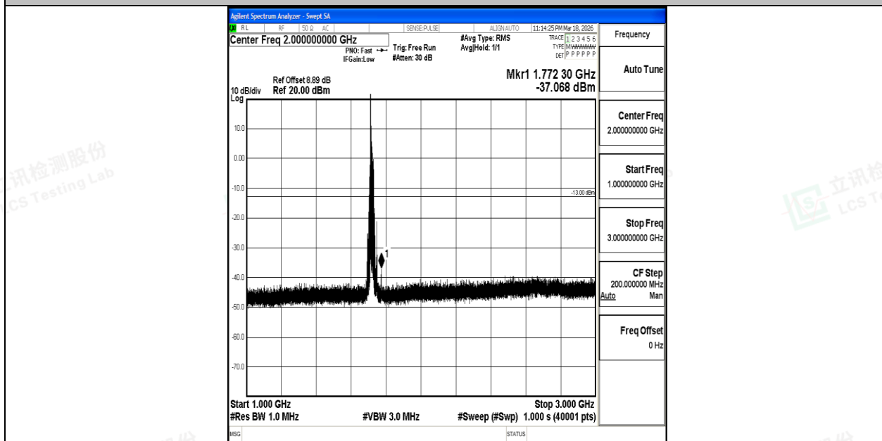
Band4_20MHz_QPSK_20050_1RB#0_1000~3000_1000~3000
