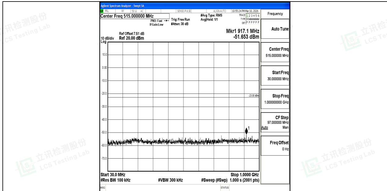
Band4_15MHz_QPSK_20175_1RB#0_30~1000_30~1000
