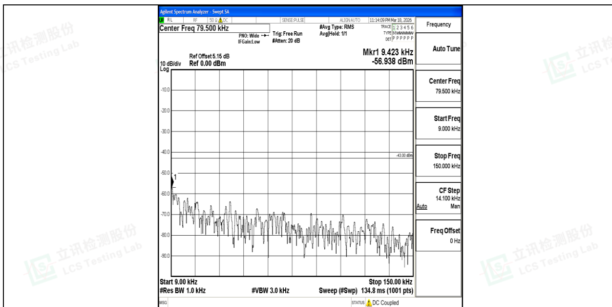
Band4_20MHz_QPSK_20050_1RB#0_0.009~0.15_0.009~0.15
