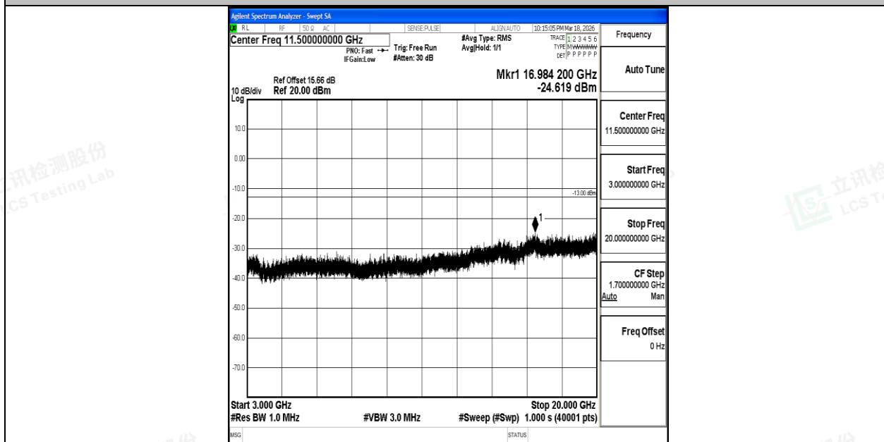
Band4_5MHz_16QAM_20375_1RB#0_3000~20000_3000~20000
