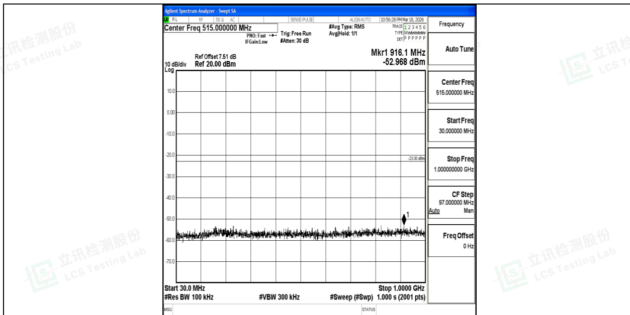
Band4_15MHz_QPSK_20325_1RB#0_30~1000_30~1000
