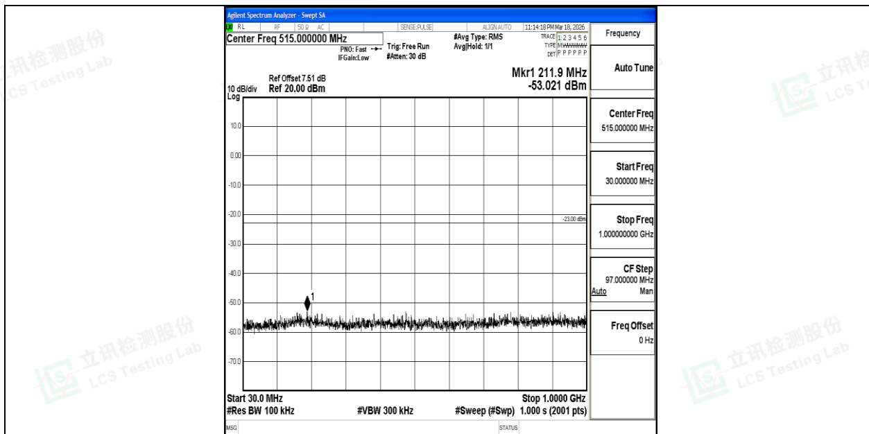
Band4_20MHz_QPSK_20050_1RB#0_30~1000_30~1000
