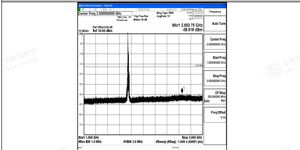
Band4_15MHz_QPSK_20325_1RB#0_1000~3000_1000~3000
