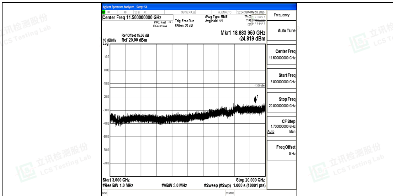
Band4_15MHz_QPSK_20025_1RB#0_3000~20000_3000~20000
