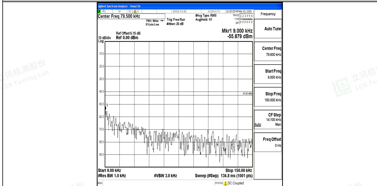
Band4_10MHz_16QAM_20175_1RB#0_0.009~0.15_0.009~0.15
