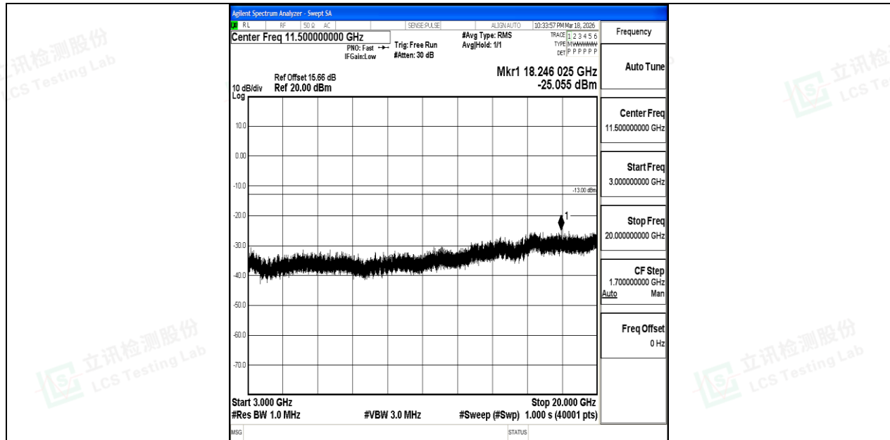
Band4_10MHz_QPSK_20000_1RB#0_3000~20000_3000~20000
