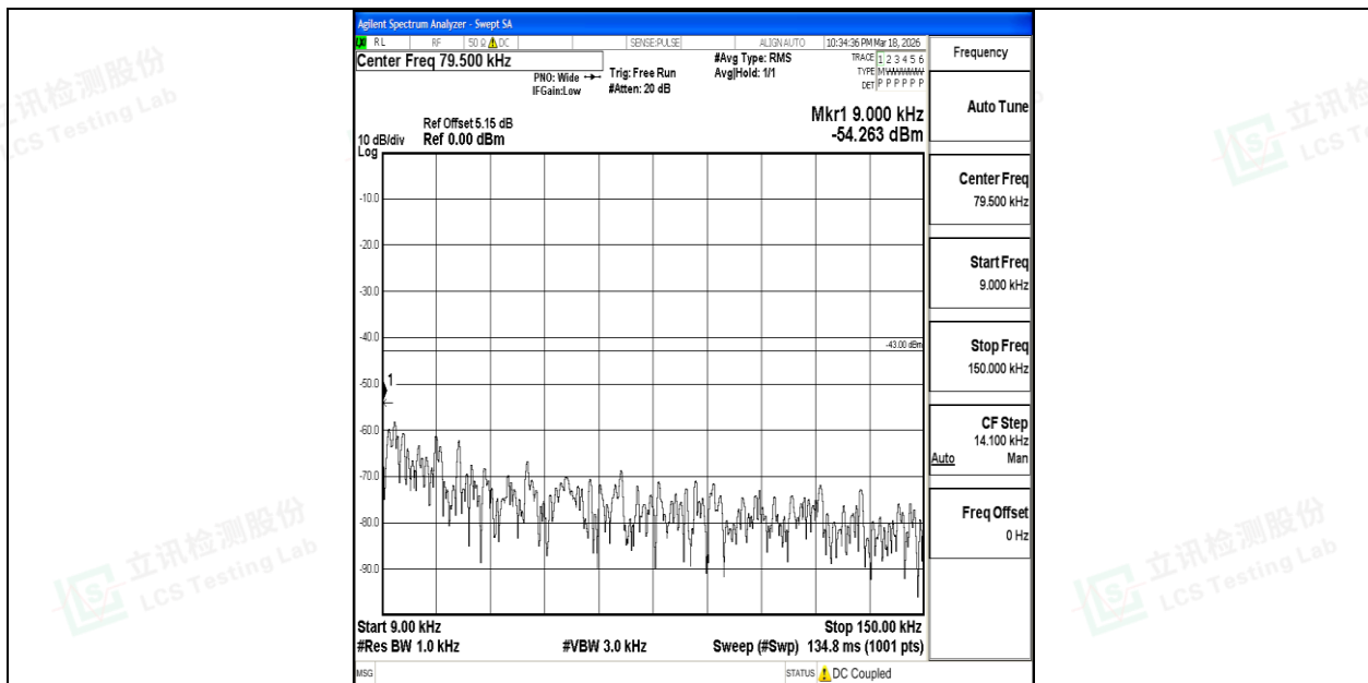
Band4_10MHz_QPSK_20175_1RB#0_0.009~0.15_0.009~0.15
