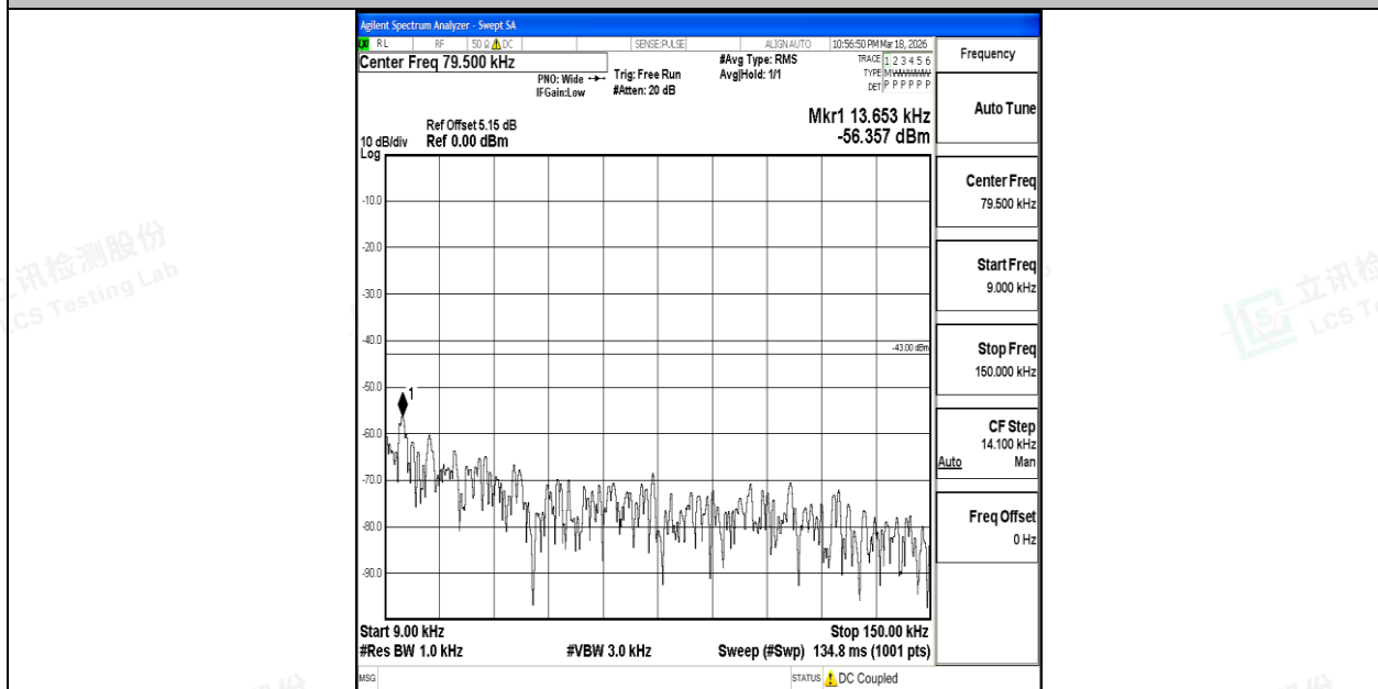
Band4_15MHz_16QAM_20325_1RB#0_0.009~0.15_0.009~0.15
