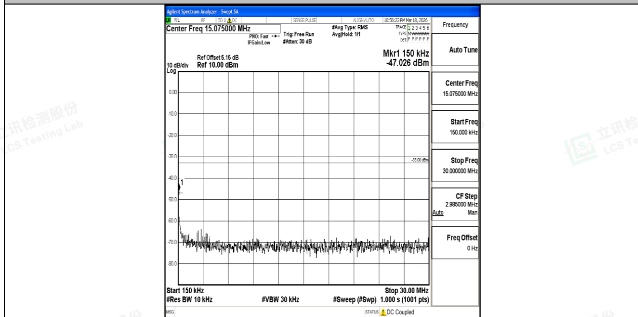
Band4_15MHz_QPSK_20325_1RB#0_0.15~30_0.15~30
