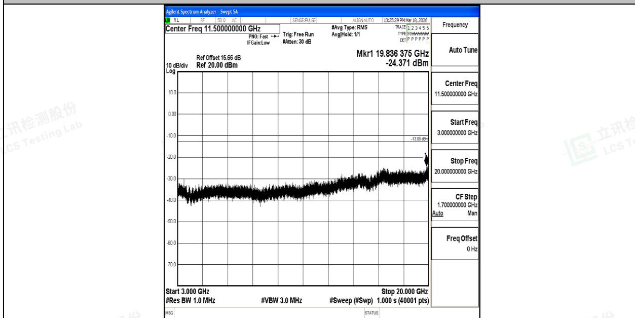
Band4_10MHz_16QAM_20175_1RB#0_3000~20000_3000~20000
