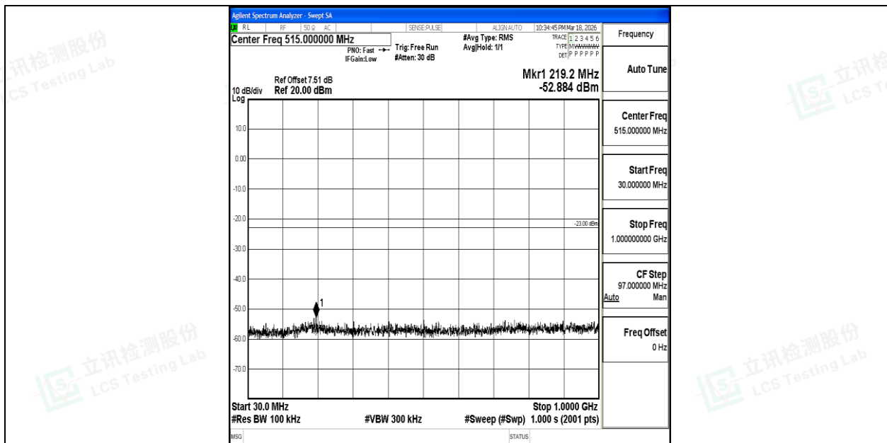
Band4_10MHz_QPSK_20175_1RB#0_30~1000_30~1000
