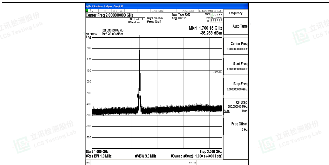
Band4_10MHz_16QAM_20175_1RB#0_1000~3000_1000~3000
