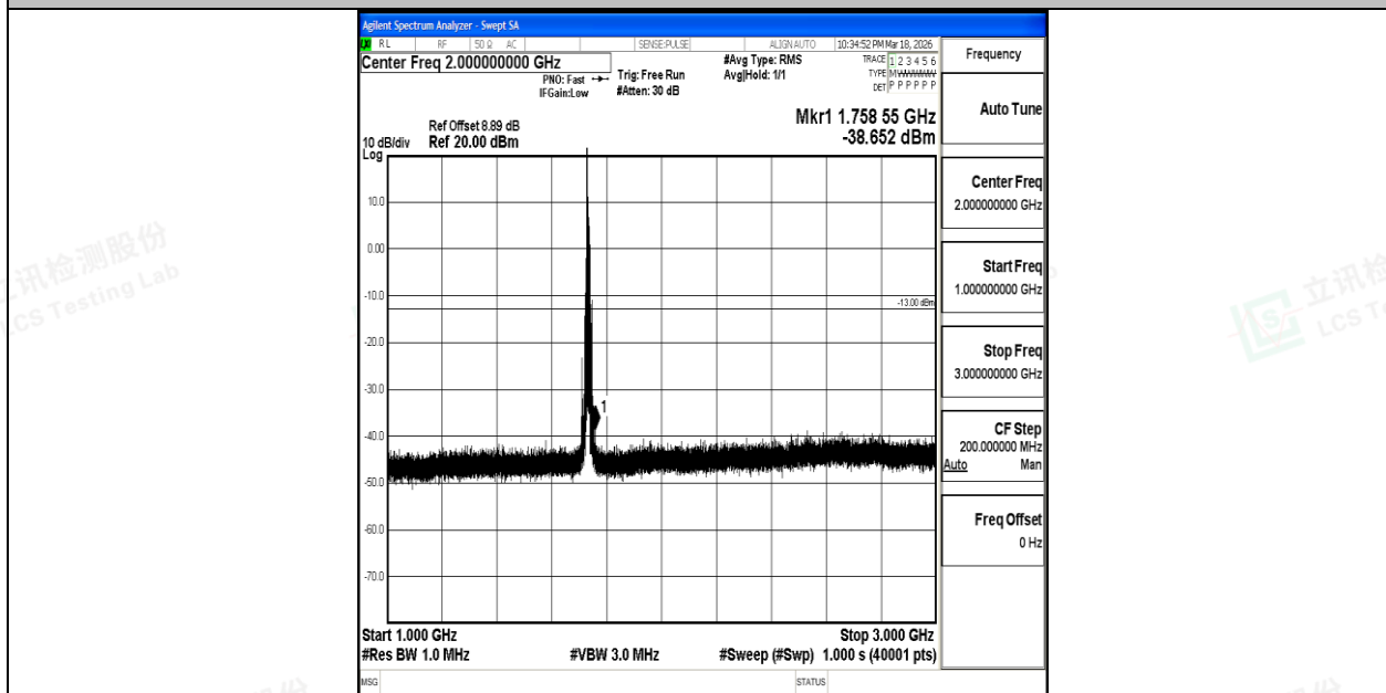
Band4_10MHz_QPSK_20175_1RB#0_1000~3000_1000~3000
