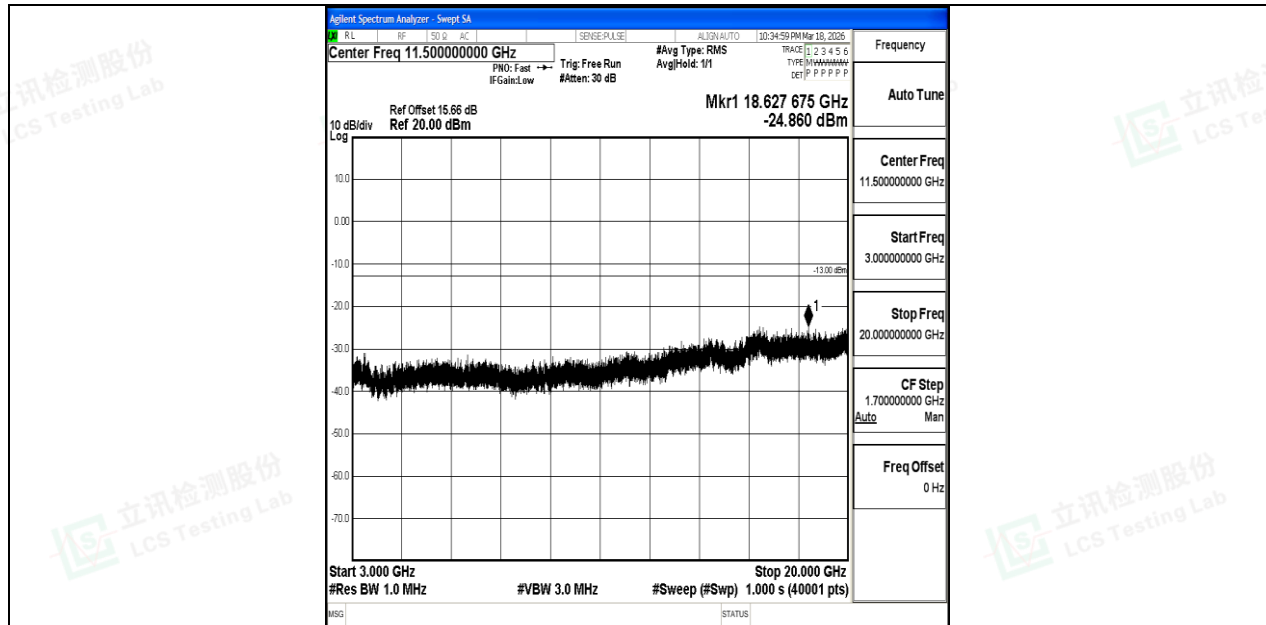
Band4_10MHz_QPSK_20175_1RB#0_3000~20000_3000~20000
