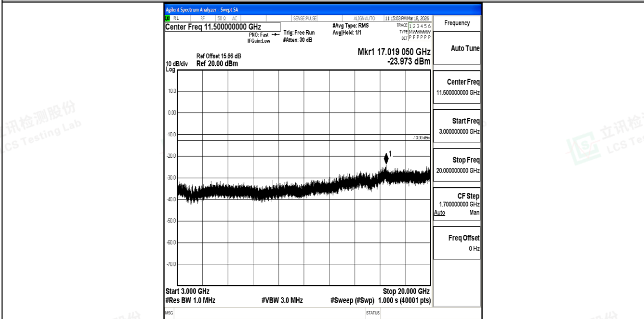
Band4_20MHz_16QAM_20050_1RB#0_3000~20000_3000~20000
