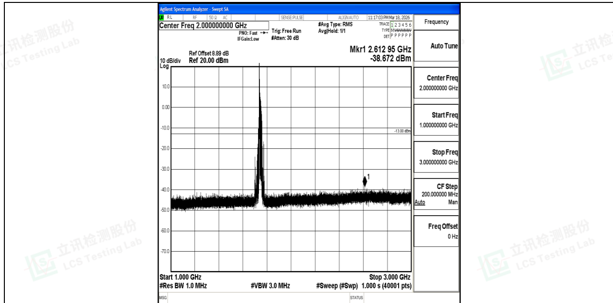
Band4_20MHz_16QAM_20300_1RB#0_1000~3000_1000~3000
