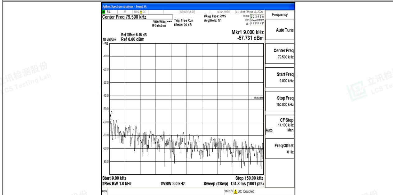
Band4_20MHz_16QAM_20300_1RB#0_0.009~0.15_0.009~0.15
