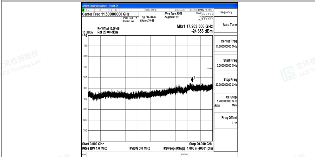
Band4_1.4MHz_16QAM_20393_1RB#0_3000~20000_3000~20000
