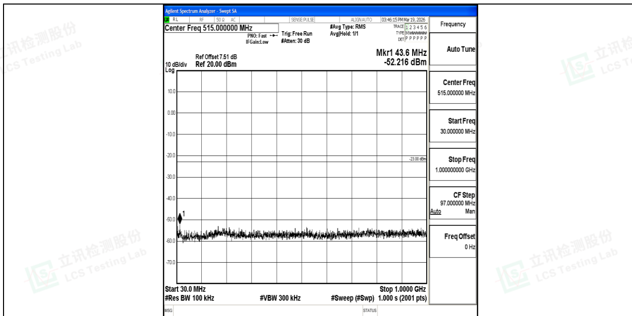
Band4_3MHz_QPSK_19965_1RB#0_30~1000_30~1000
