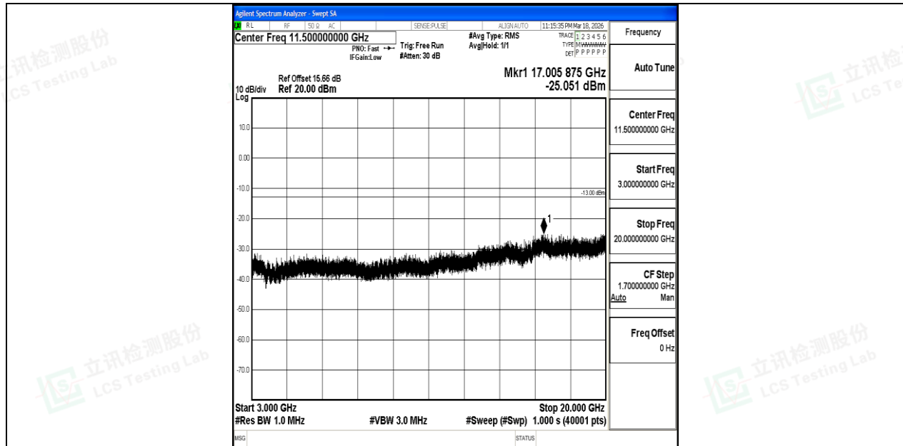
Band4_20MHz_QPSK_20175_1RB#0_3000~20000_3000~20000
