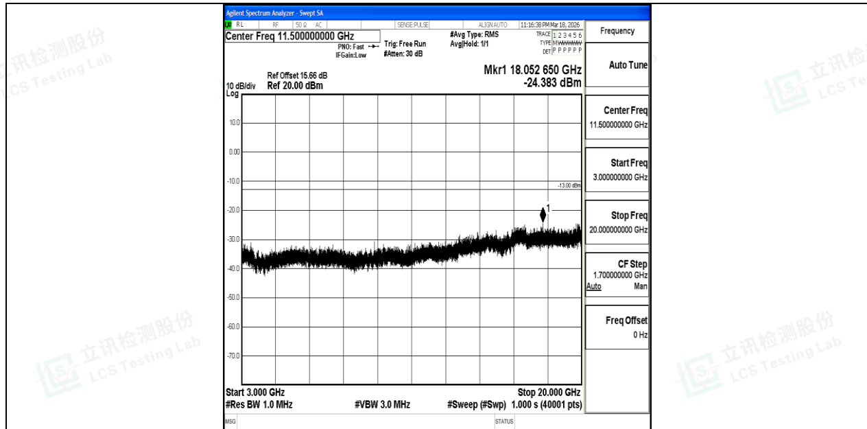
Band4_20MHz_QPSK_20300_1RB#0_3000~20000_3000~20000
