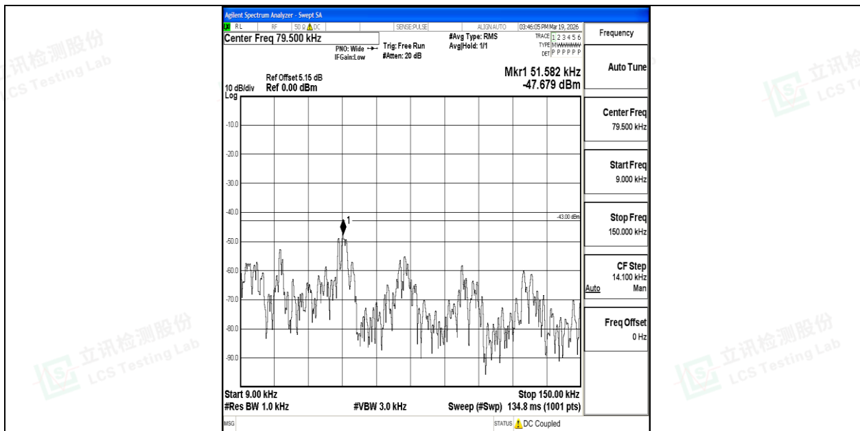
Band4_3MHz_QPSK_19965_1RB#0_0.009~0.15_0.009~0.15
