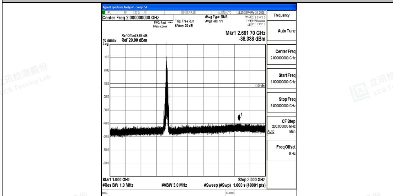
Band4_20MHz_QPSK_20175_1RB#0_1000~3000_1000~3000
