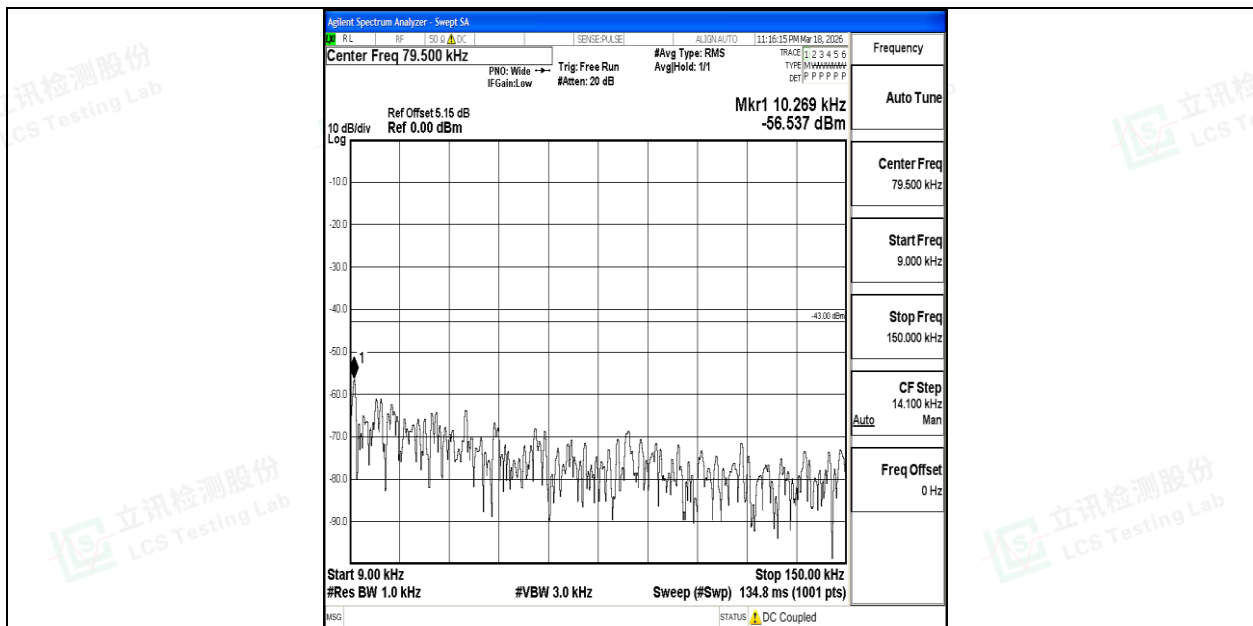
Band4_20MHz_QPSK_20300_1RB#0_0.009~0.15_0.009~0.15
