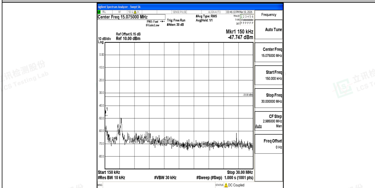
Band4_3MHz_QPSK_19965_1RB#0_0.15~30_0.15~30
