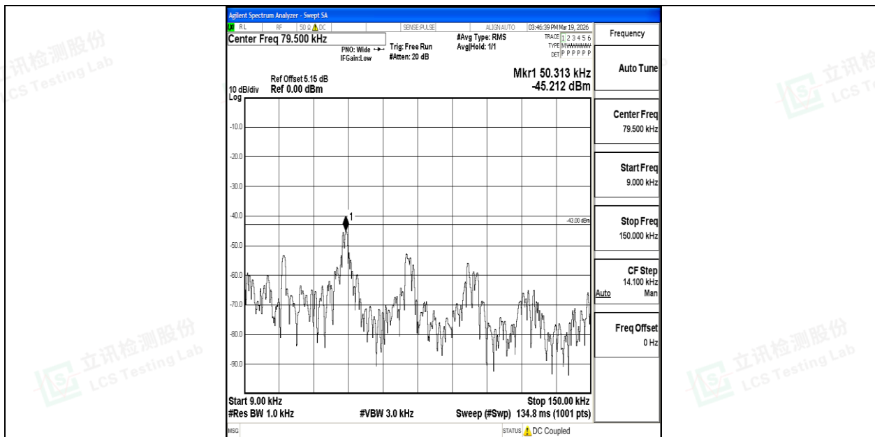
Band4_3MHz_16QAM_19965_1RB#0_0.009~0.15_0.009~0.15
