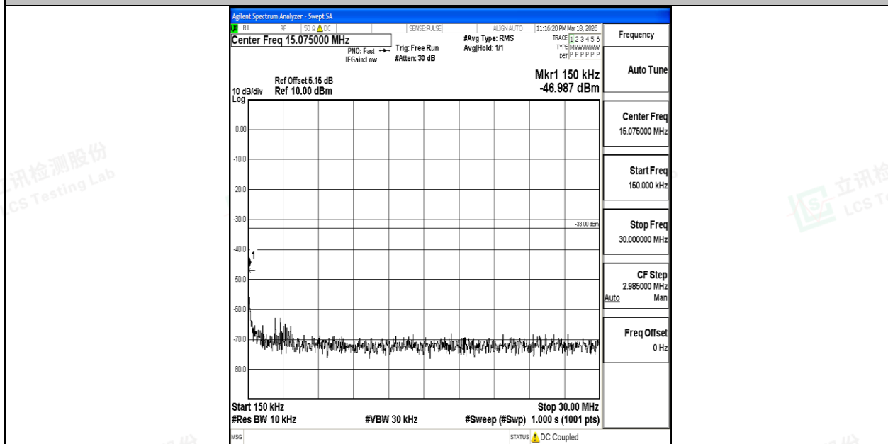
Band4_20MHz_QPSK_20300_1RB#0_0.15~30_0.15~30
