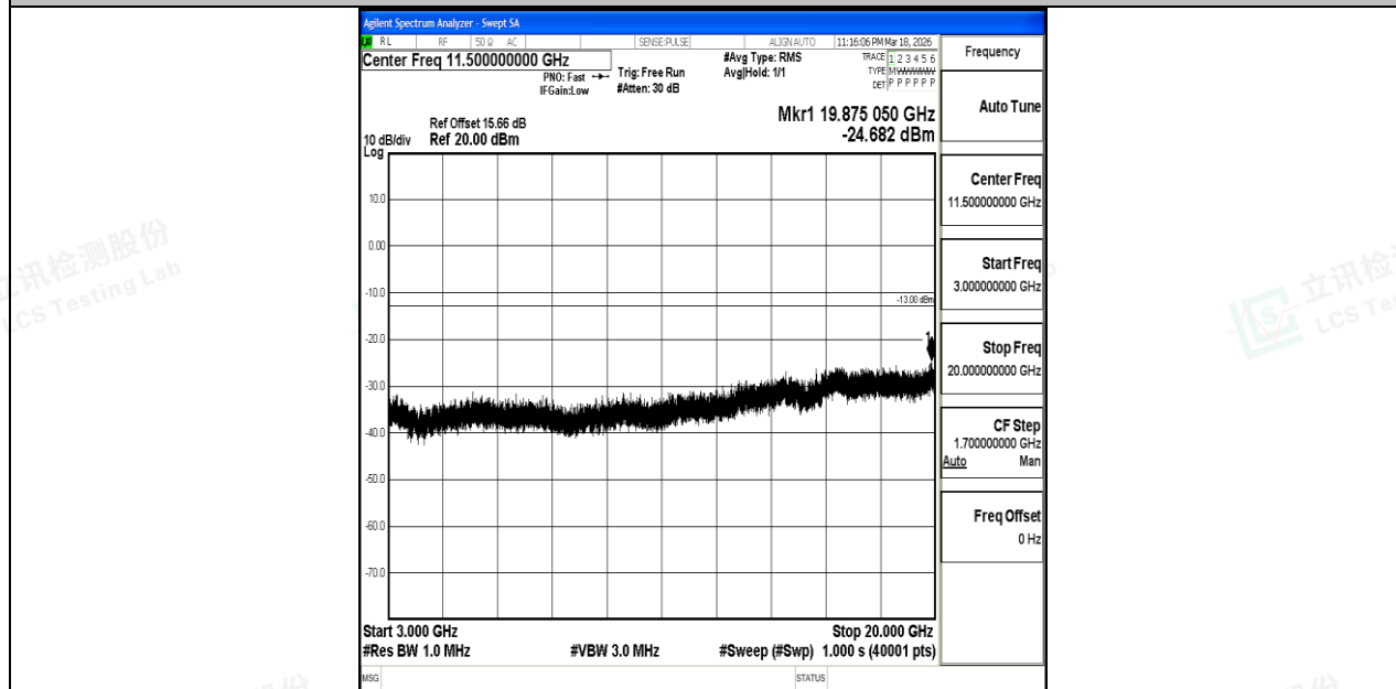
Band4_20MHz_16QAM_20175_1RB#0_3000~20000_3000~20000
