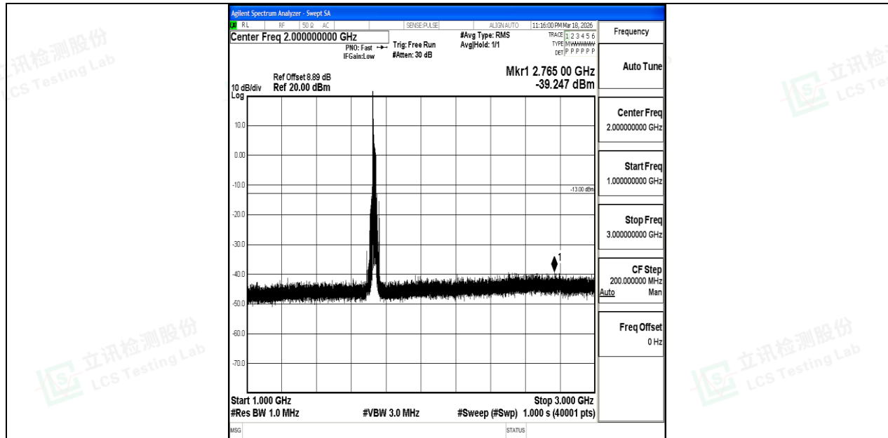
Band4_20MHz_16QAM_20175_1RB#0_1000~3000_1000~3000
