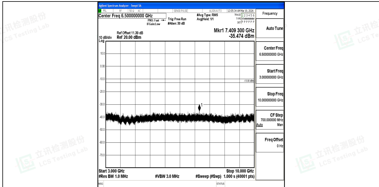
Band5_3MHz_QPSK_20525_1RB#0_3000~10000_3000~10000
