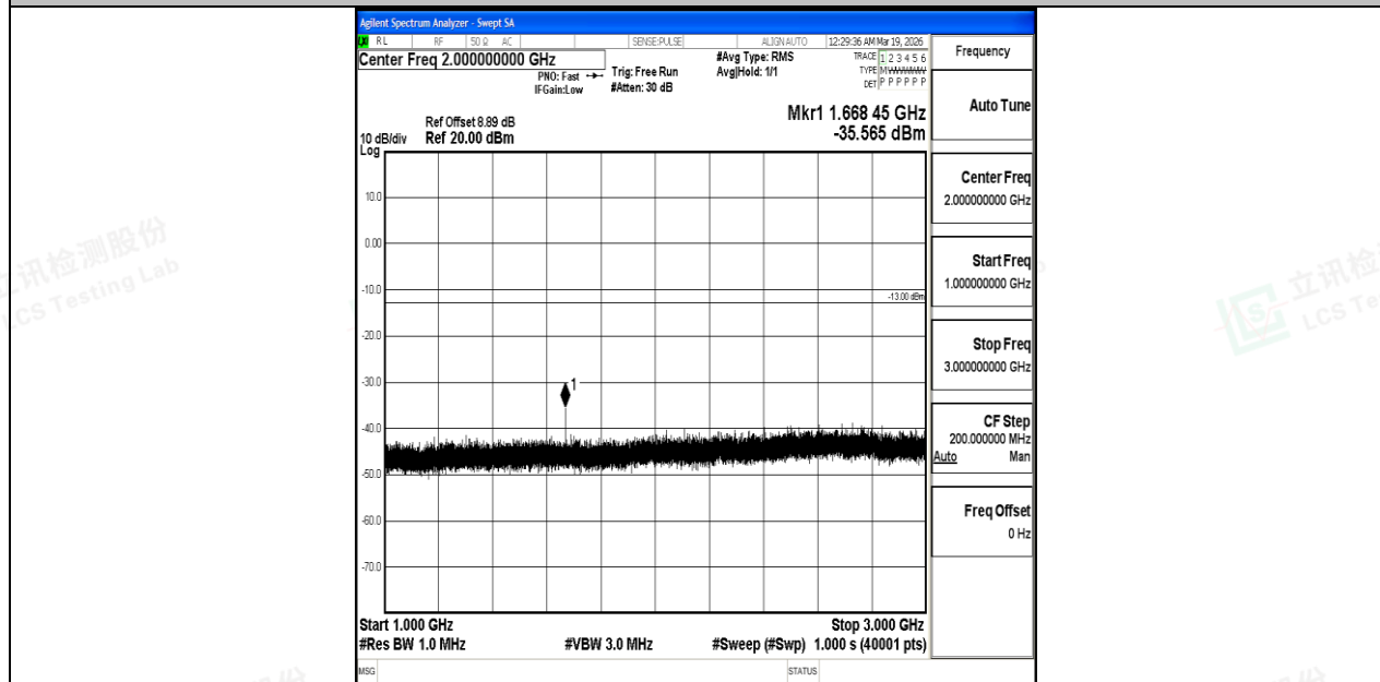
Band5_5MHz_QPSK_20525_1RB#0_1000~3000_1000~3000
