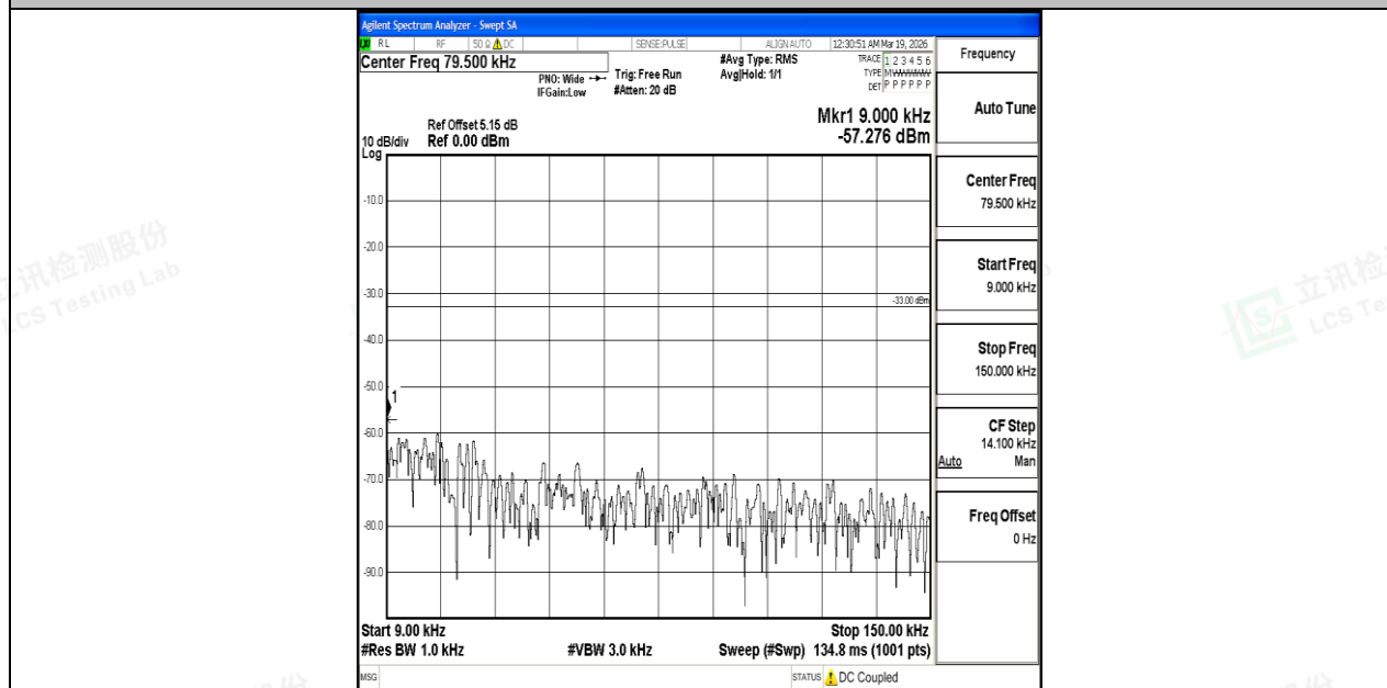
Band5_5MHz_16QAM_20625_1RB#0_0.009~0.15_0.009~0.15
