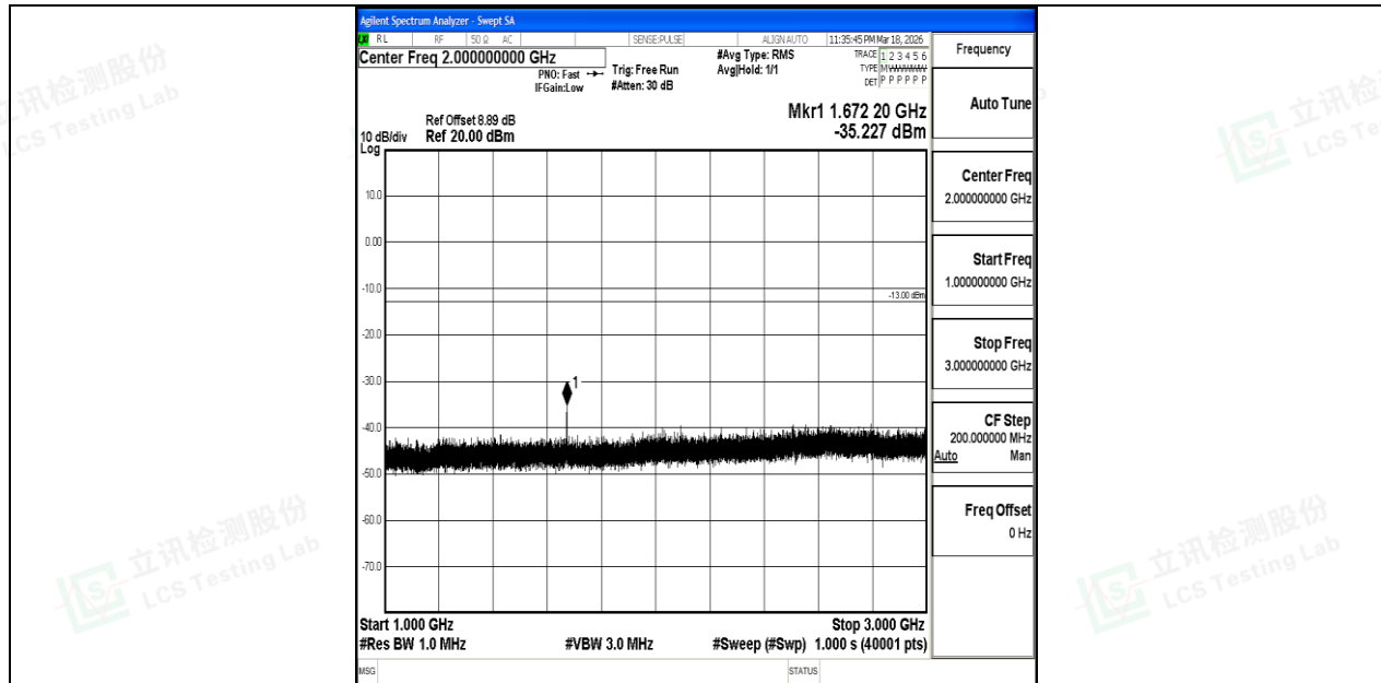
Band5_1.4MHz_16QAM_20525_1RB#0_1000~3000_1000~3000
