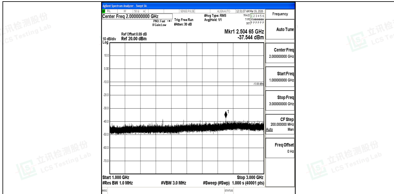
Band5_5MHz_16QAM_20625_1RB#0_1000~3000_1000~3000
