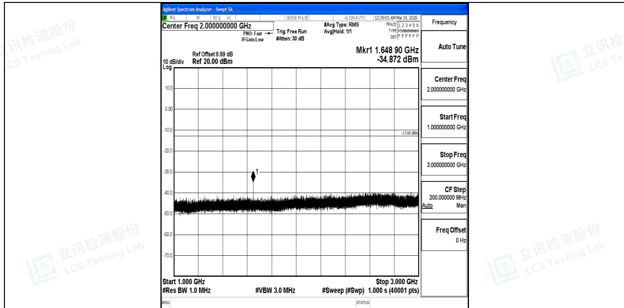
Band5_5MHz_16QAM_20425_1RB#0_1000~3000_1000~3000
