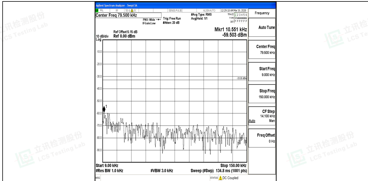
Band5_5MHz_QPSK_20525_1RB#0_0.009~0.15_0.009~0.15
