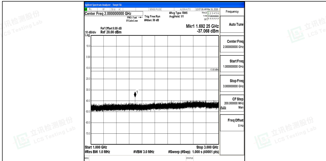
Band5_3MHz_16QAM_20635_1RB#0_1000~3000_1000~3000
