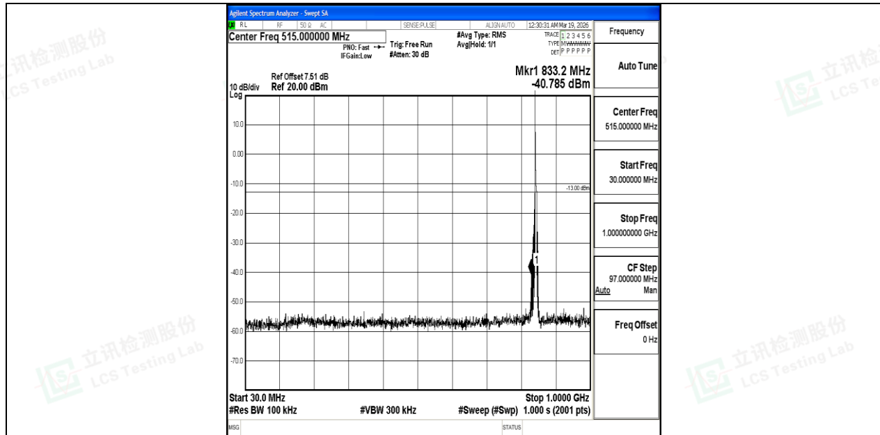
Band5_5MHz_QPSK_20625_1RB#0_30~1000_30~1000
