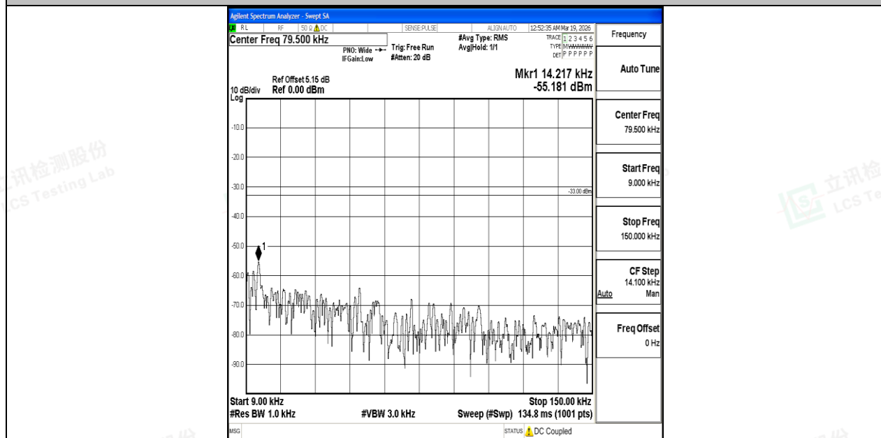
Band5_10MHz_16QAM_20525_1RB#0_0.009~0.15_0.009~0.15
