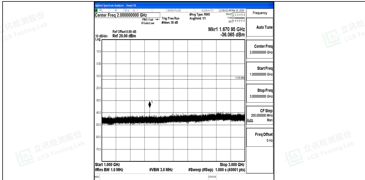
Band5_3MHz_16QAM_20525_1RB#0_1000~3000_1000~3000
