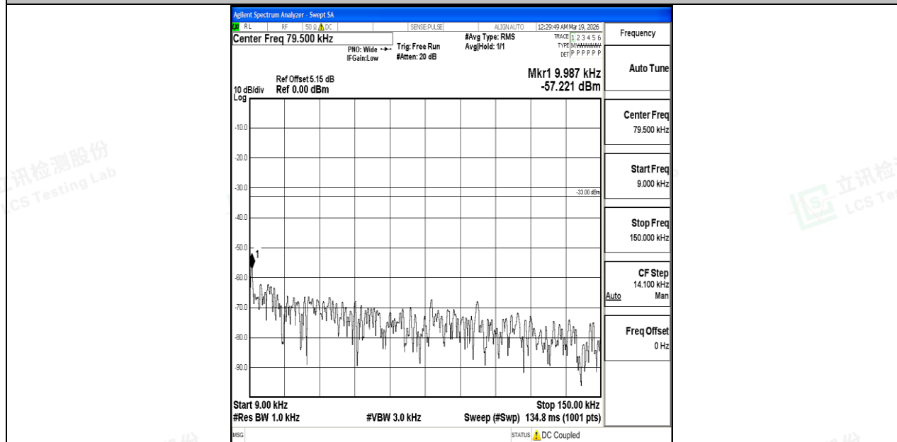
Band5_5MHz_16QAM_20525_1RB#0_0.009~0.15_0.009~0.15
