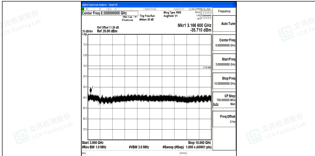
Band5_1.4MHz_QPSK_20643_1RB#0_3000~10000_3000~10000
