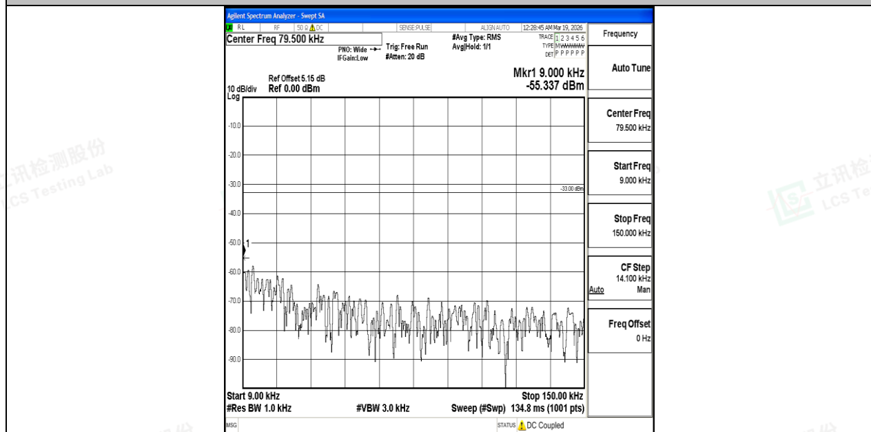
Band5_5MHz_16QAM_20425_1RB#0_0.009~0.15_0.009~0.15
