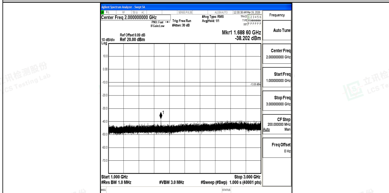
Band5_5MHz_QPSK_20625_1RB#0_1000~3000_1000~3000
