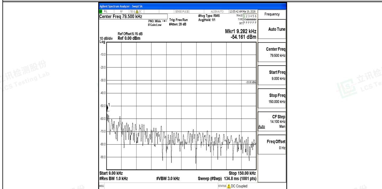
Band5_3MHz_16QAM_20525_1RB#0_0.009~0.15_0.009~0.15
