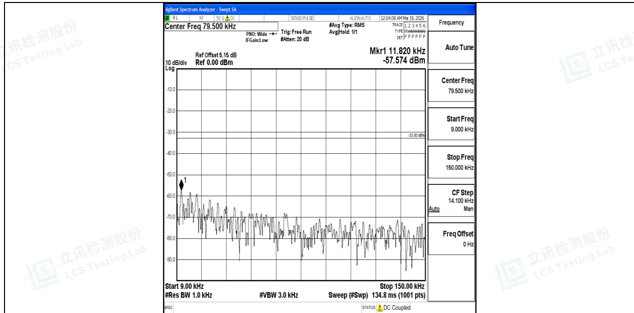
Band5_3MHz_QPSK_20415_1RB#0_0.009~0.15_0.009~0.15
