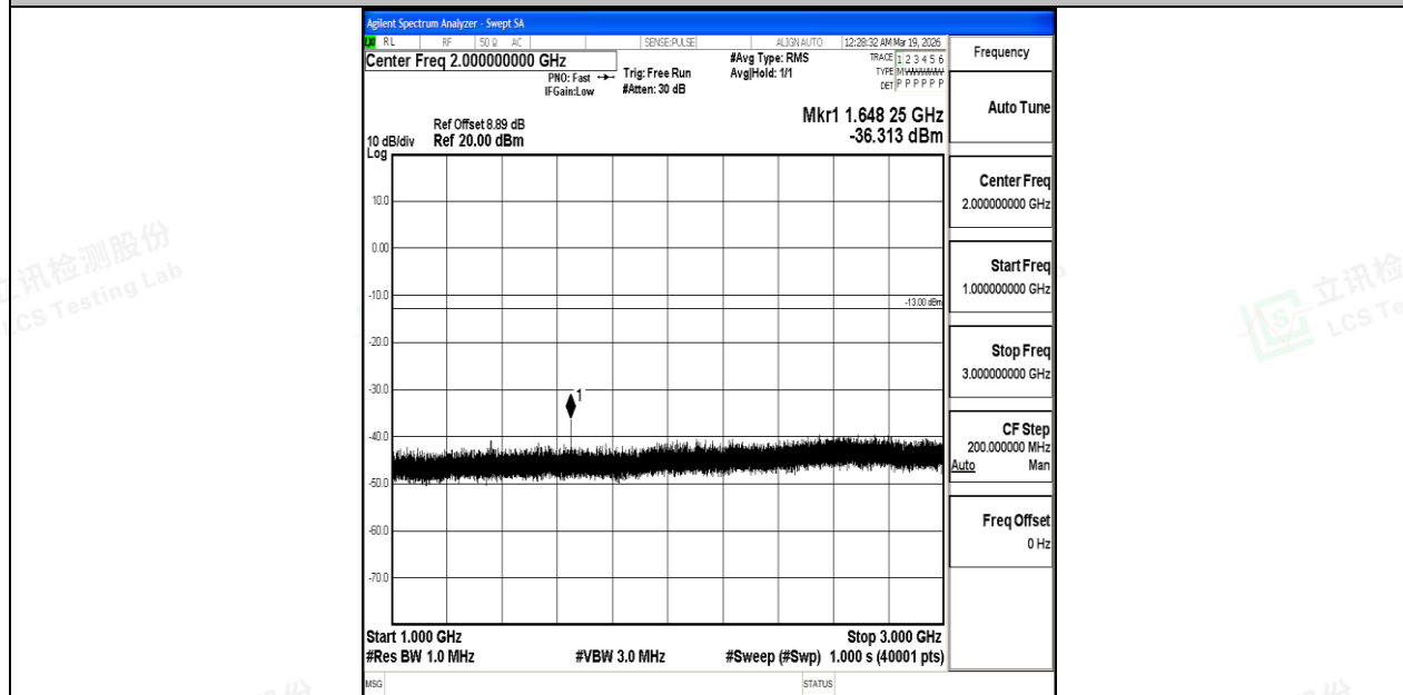
Band5_5MHz_QPSK_20425_1RB#0_1000~3000_1000~3000
