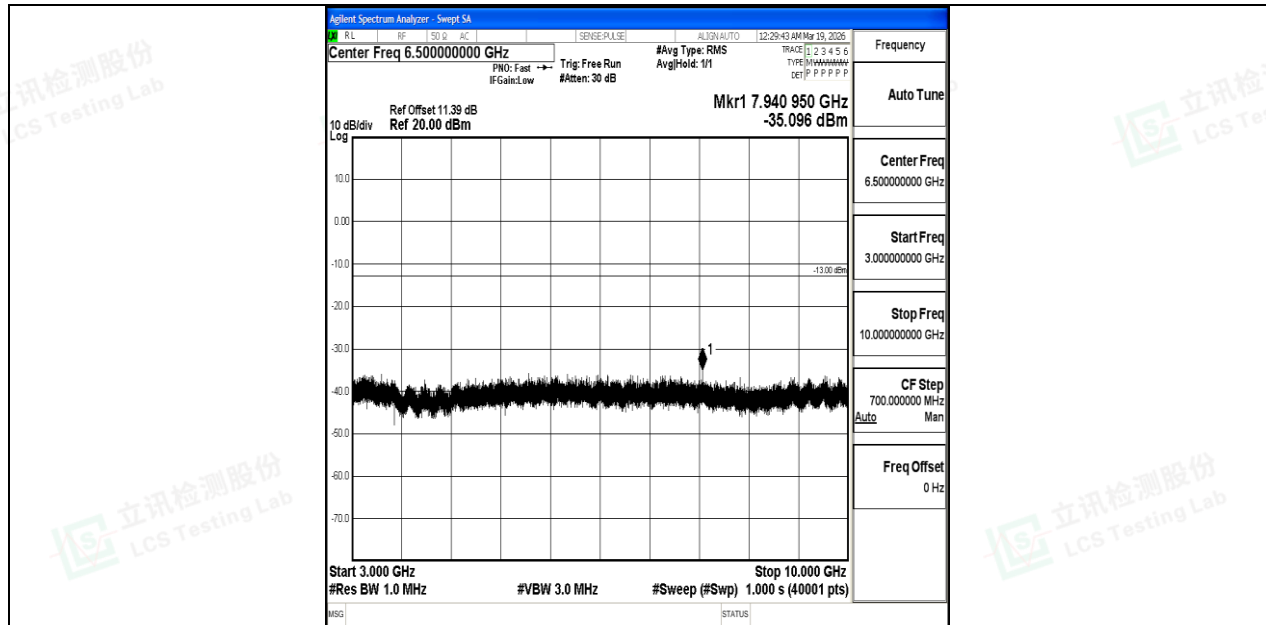
Band5_5MHz_QPSK_20525_1RB#0_3000~10000_3000~10000
