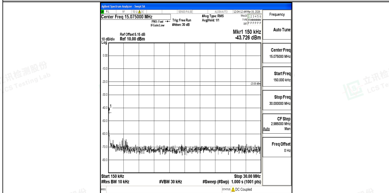
Band5_3MHz_QPSK_20415_1RB#0_0.15~30_0.15~30
