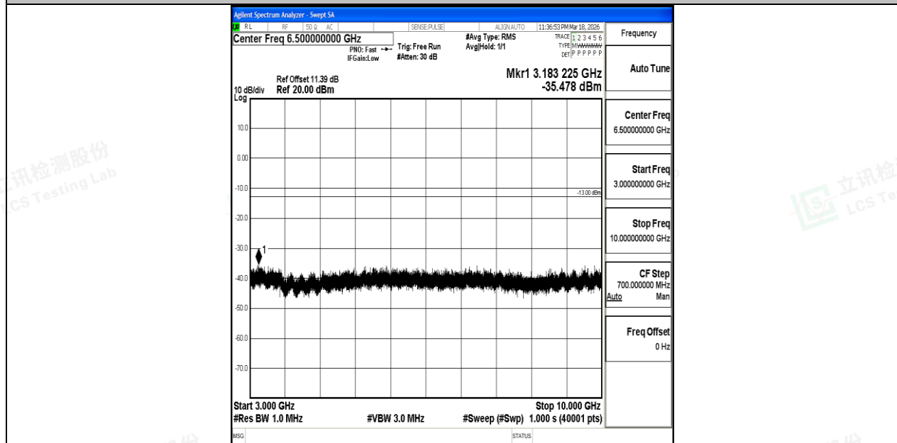
Band5_1.4MHz_16QAM_20643_1RB#0_3000~10000_3000~10000
