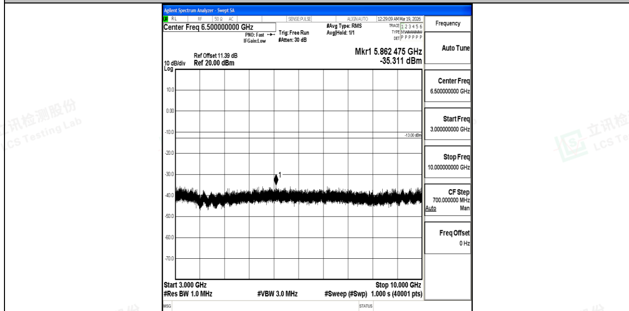
Band5_5MHz_16QAM_20425_1RB#0_3000~10000_3000~10000
