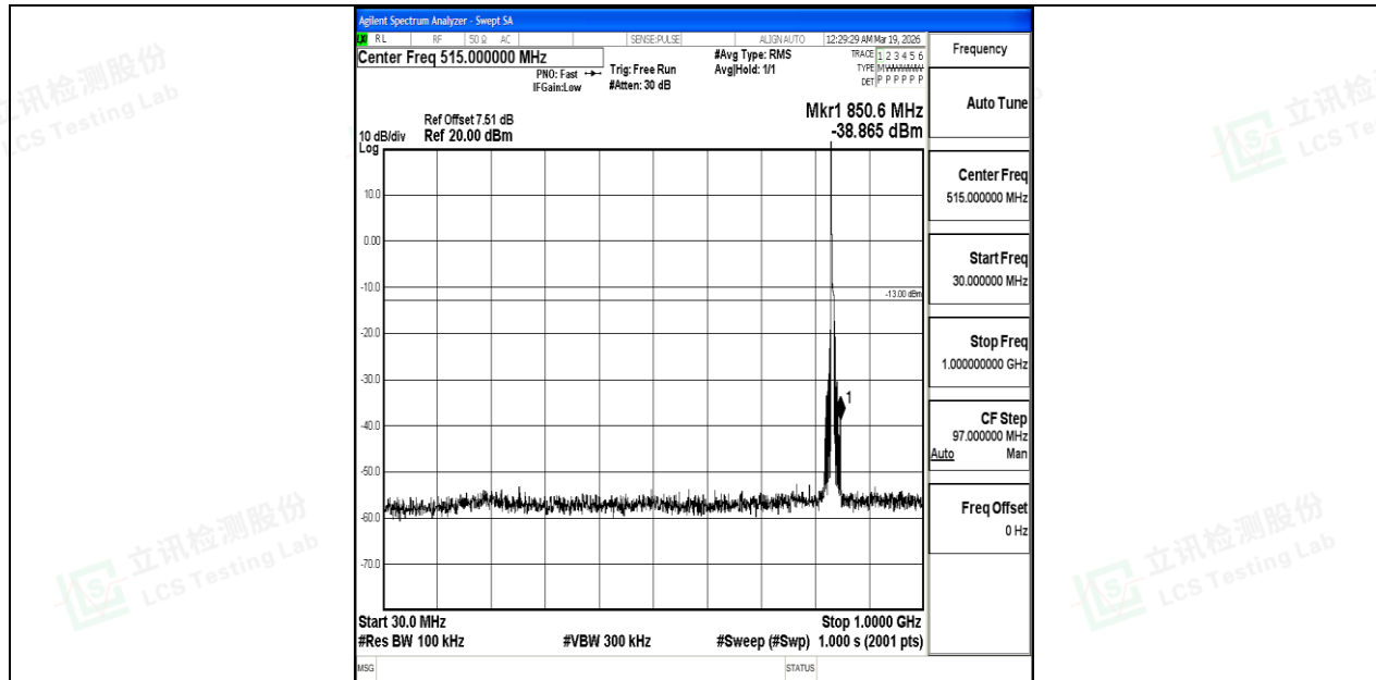
Band5_5MHz_QPSK_20525_1RB#0_30~1000_30~1000
