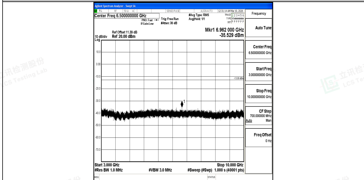
Band5_5MHz_16QAM_20625_1RB#0_3000~10000_3000~10000
