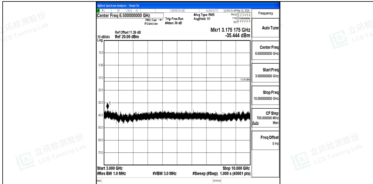
Band5_3MHz_QPSK_20415_1RB#0_3000~10000_3000~10000
