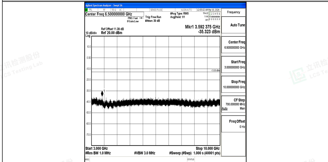
Band5_3MHz_16QAM_20415_1RB#0_3000~10000_3000~10000
