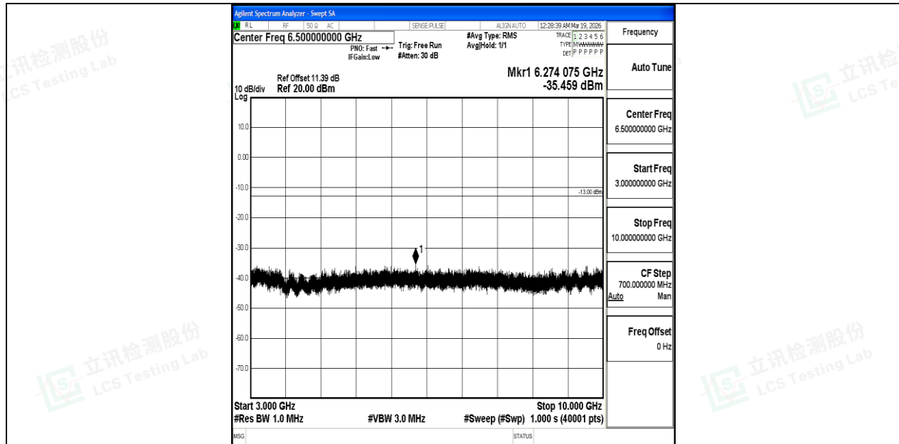
Band5_5MHz_QPSK_20425_1RB#0_3000~10000_3000~10000
