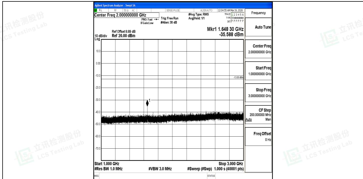
Band5_3MHz_16QAM_20415_1RB#0_1000~3000_1000~3000
