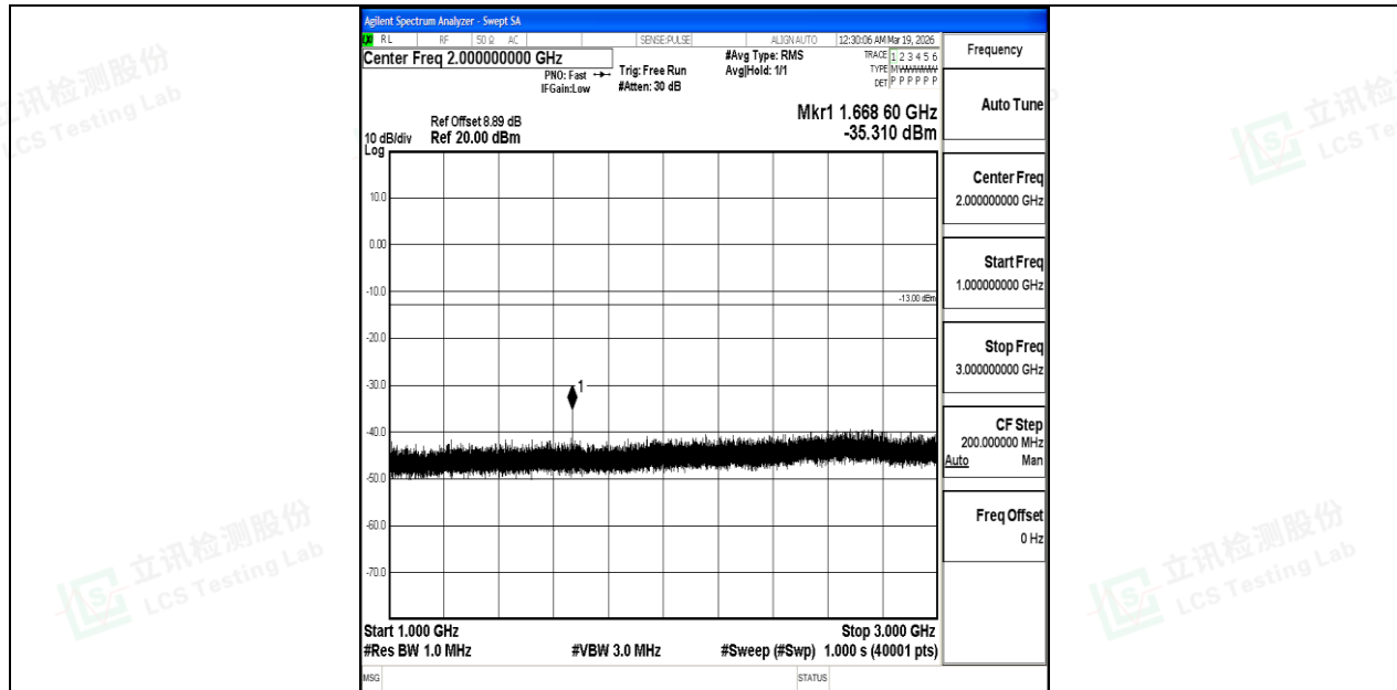
Band5_5MHz_16QAM_20525_1RB#0_1000~3000_1000~3000
