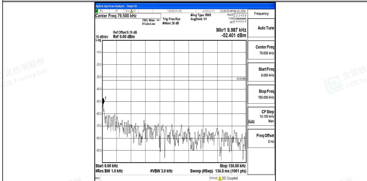
Band5_3MHz_16QAM_20635_1RB#0_0.009~0.15_0.009~0.15
