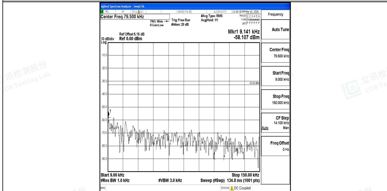
Band5_1.4MHz_16QAM_20643_1RB#0_0.009~0.15_0.009~0.15
