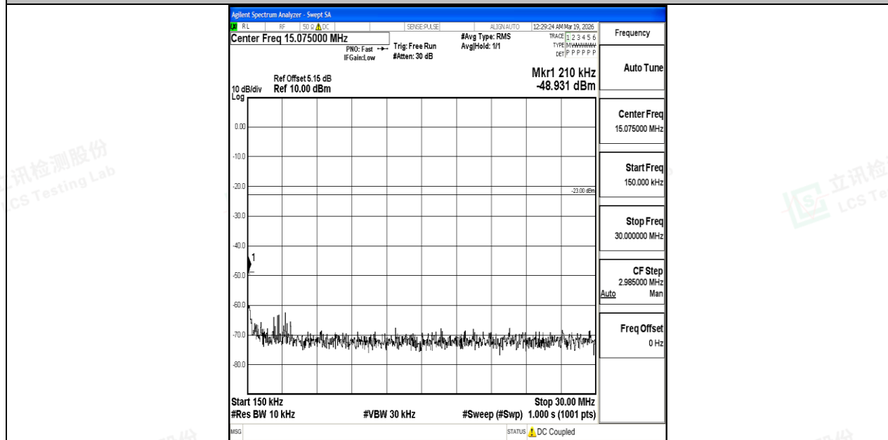
Band5_5MHz_QPSK_20525_1RB#0_0.15~30_0.15~30
