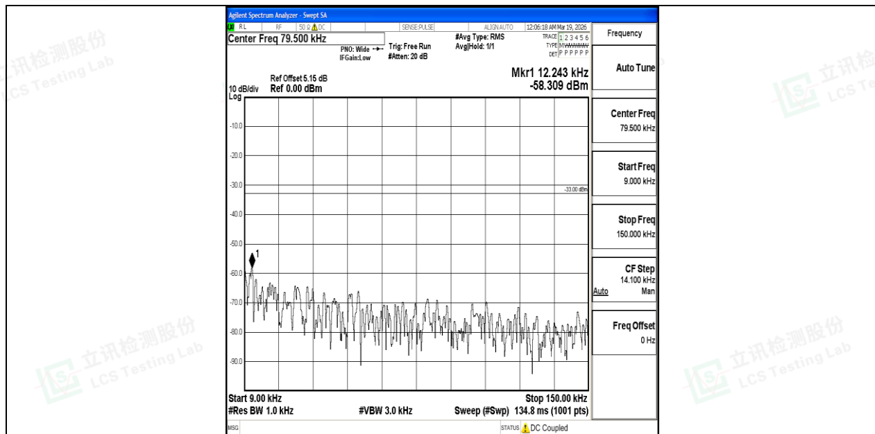
Band5_3MHz_QPSK_20635_1RB#0_0.009~0.15_0.009~0.15
