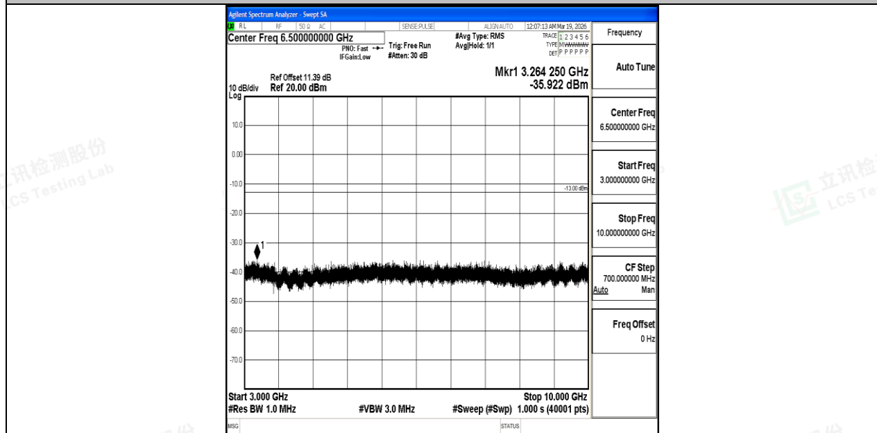
Band5_3MHz_16QAM_20635_1RB#0_3000~10000_3000~10000
