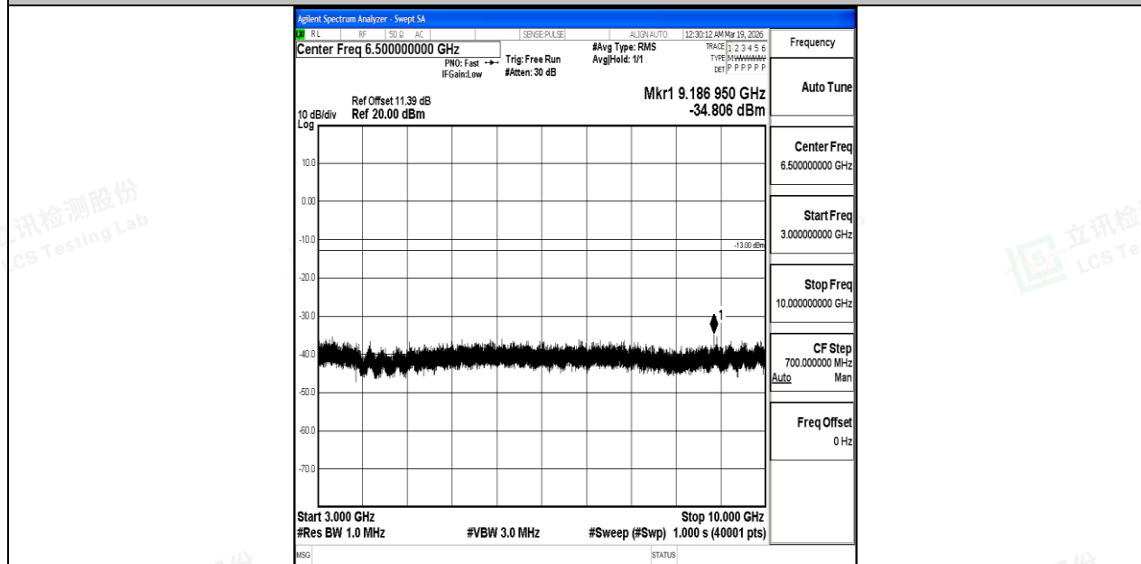
Band5_5MHz_16QAM_20525_1RB#0_3000~10000_3000~10000
