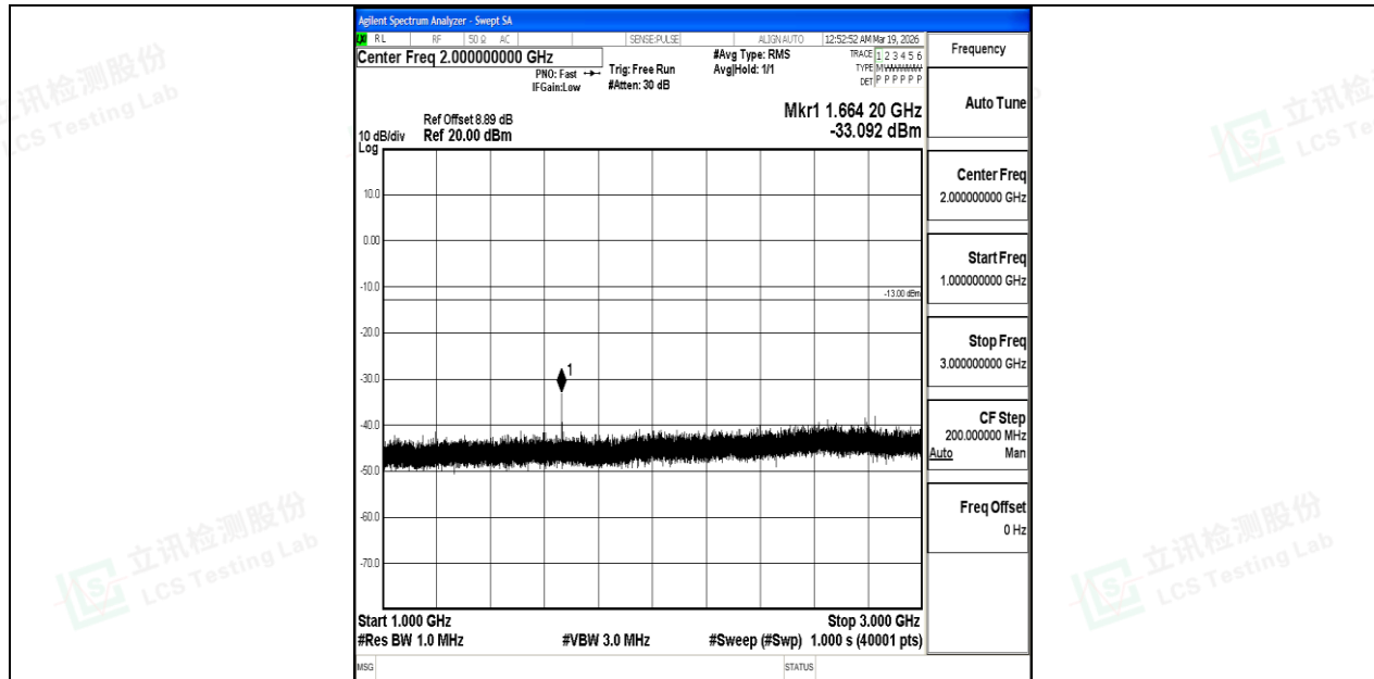
Band5_10MHz_16QAM_20525_1RB#0_1000~3000_1000~3000
