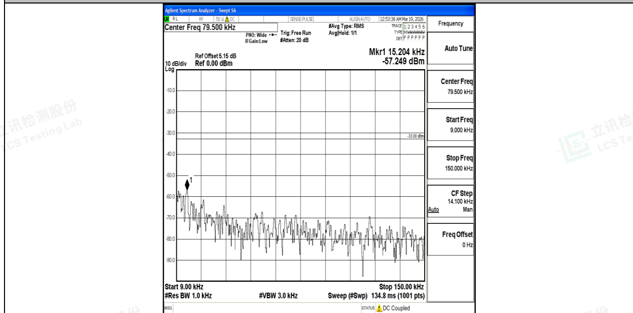
Band5_10MHz_16QAM_20600_1RB#0_0.009~0.15_0.009~0.15
