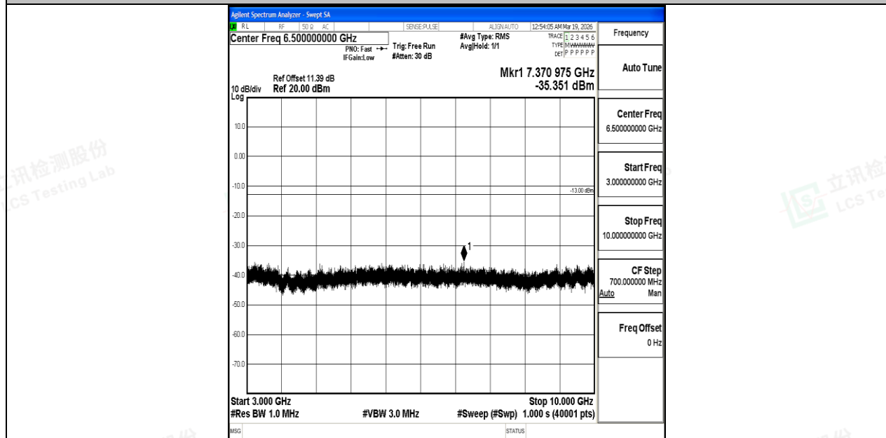
Band5_10MHz_16QAM_20600_1RB#0_3000~10000_3000~10000
