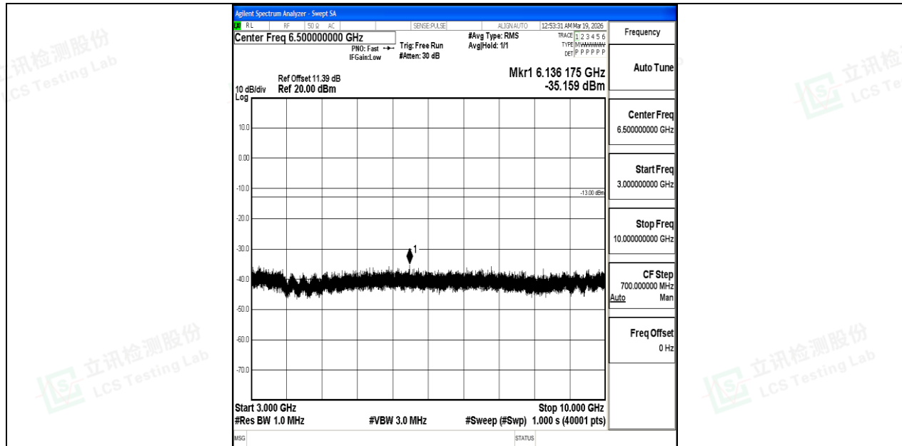
Band5_10MHz_QPSK_20600_1RB#0_3000~10000_3000~10000
