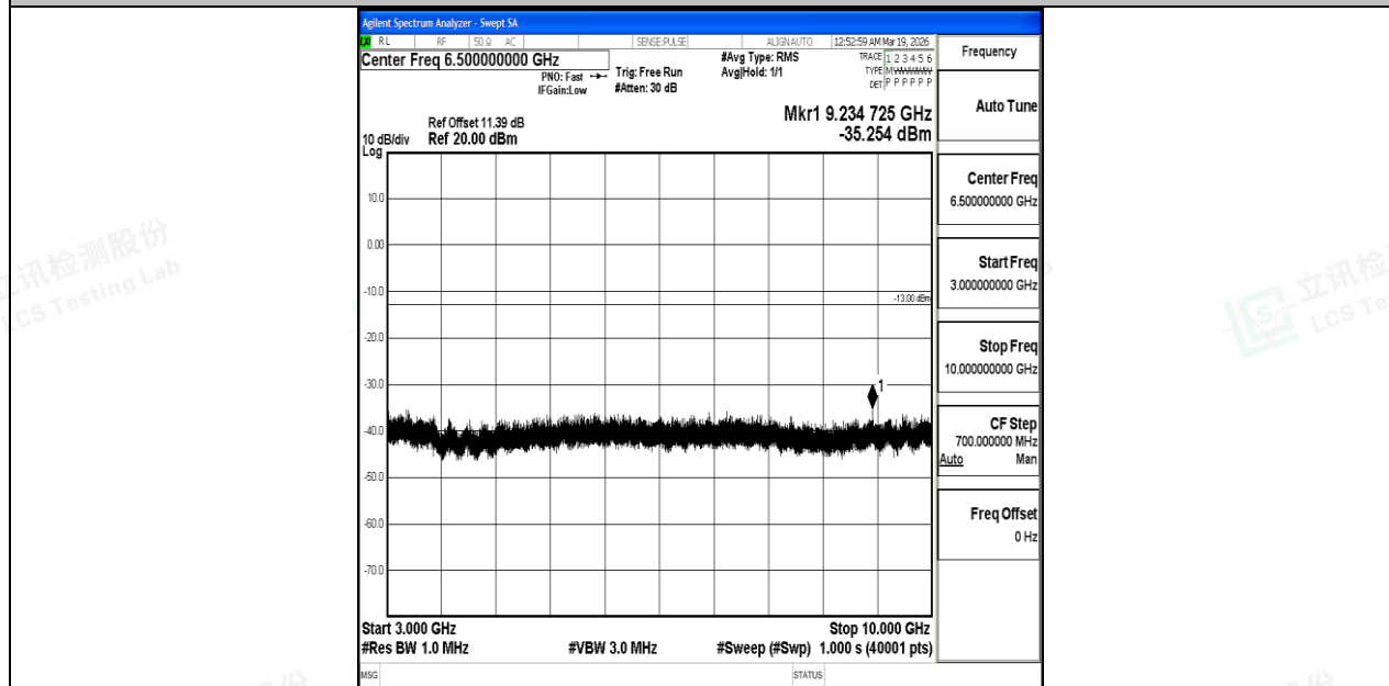
Band5_10MHz_16QAM_20525_1RB#0_3000~10000_3000~10000
