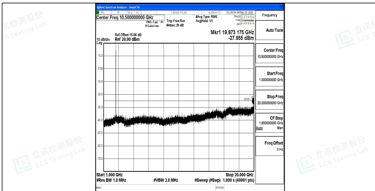
Band7_10MHz_16QAM_21400_1RB#0_1000~20000_1000~20000
