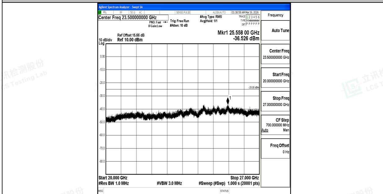
Band7_10MHz_16QAM_21100_1RB#0_20000~27000_20000~27000
