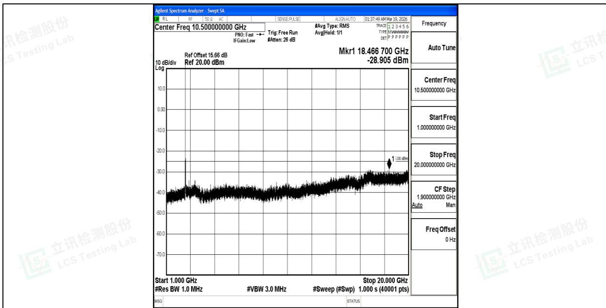
Band7_10MHz_16QAM_20800_1RB#0_1000~20000_1000~20000
