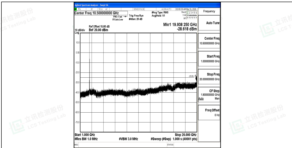
Band7_15MHz_16QAM_21100_1RB#0_1000~20000_1000~20000
