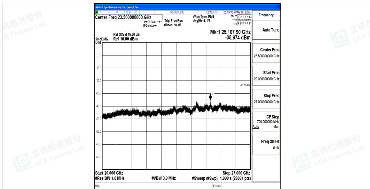
Band7_10MHz_QPSK_21400_1RB#0_20000~27000_20000~27000
