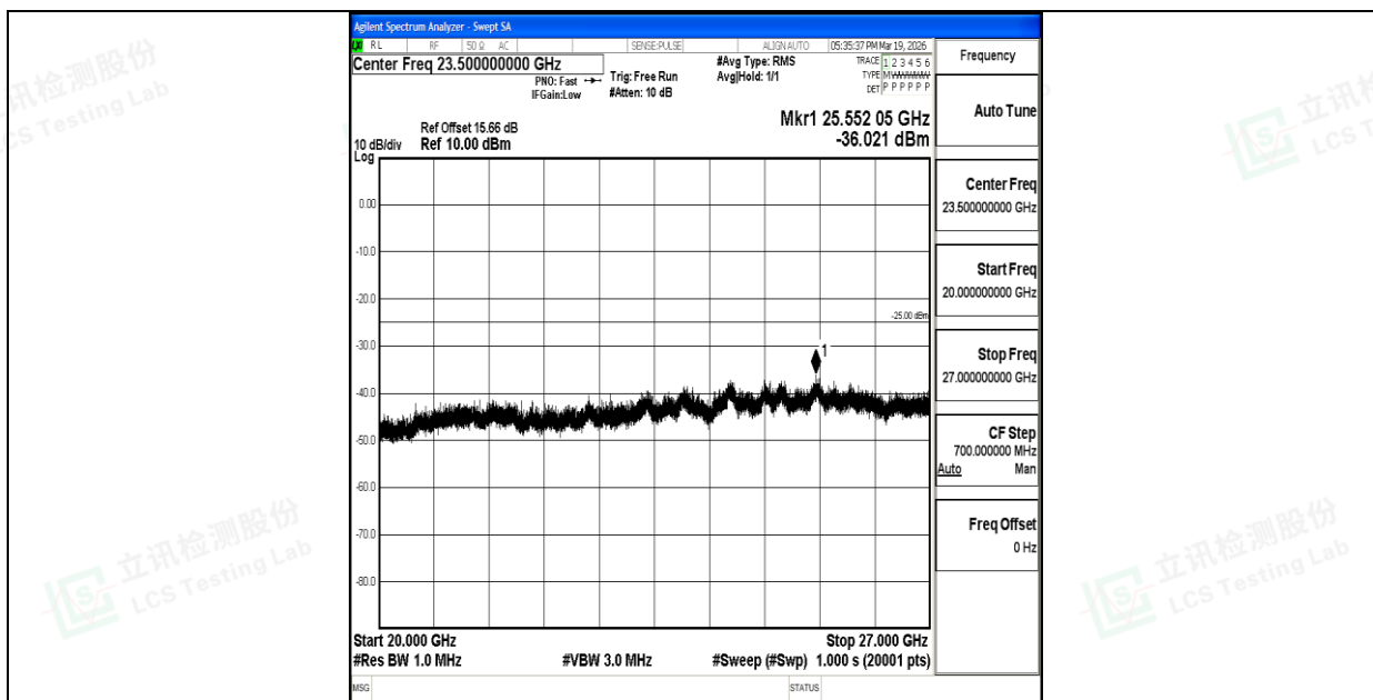
Band7_5MHz_QPSK_21425_1RB#0_20000~27000_20000~27000
