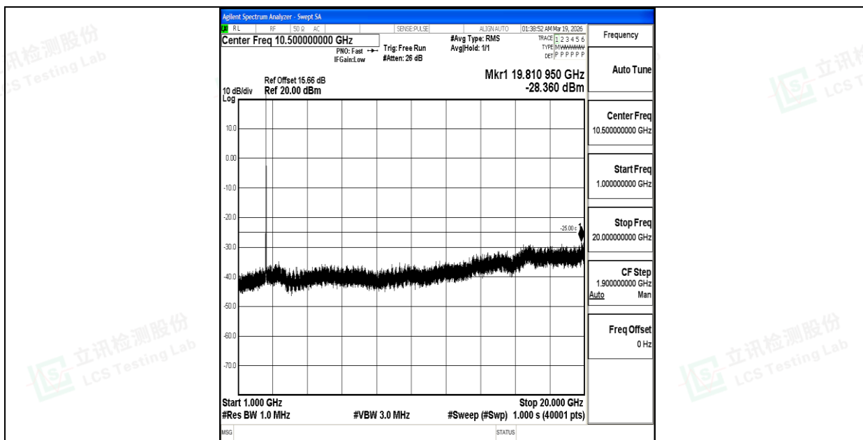
Band7_10MHz_16QAM_21100_1RB#0_1000~20000_1000~20000
