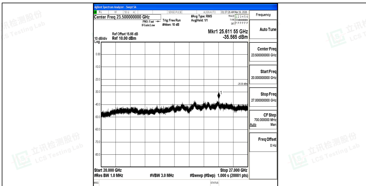
Band7_10MHz_QPSK_20800_1RB#0_20000~27000_20000~27000
