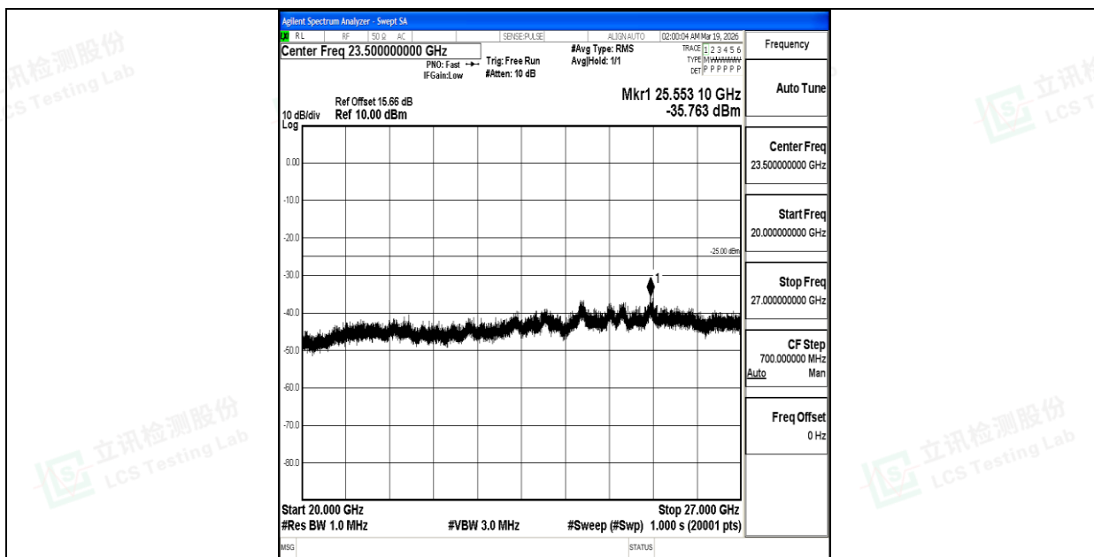
Band7_15MHz_QPSK_21100_1RB#0_20000~27000_20000~27000
