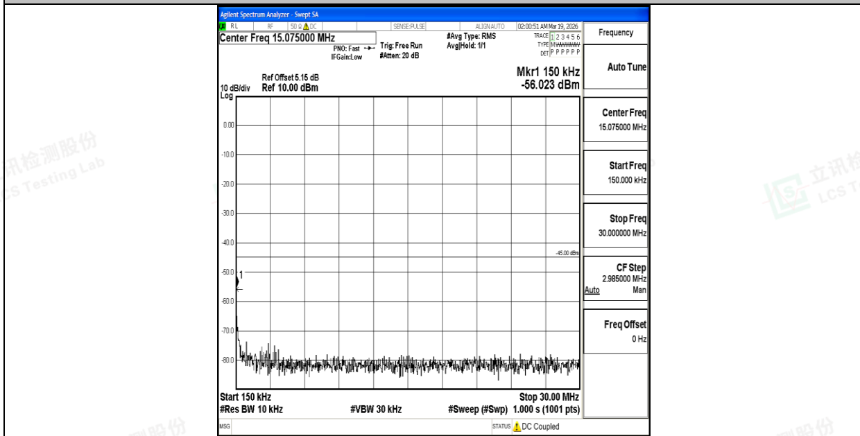
Band7_15MHz_QPSK_21375_1RB#0_0.15~30_0.15~30
