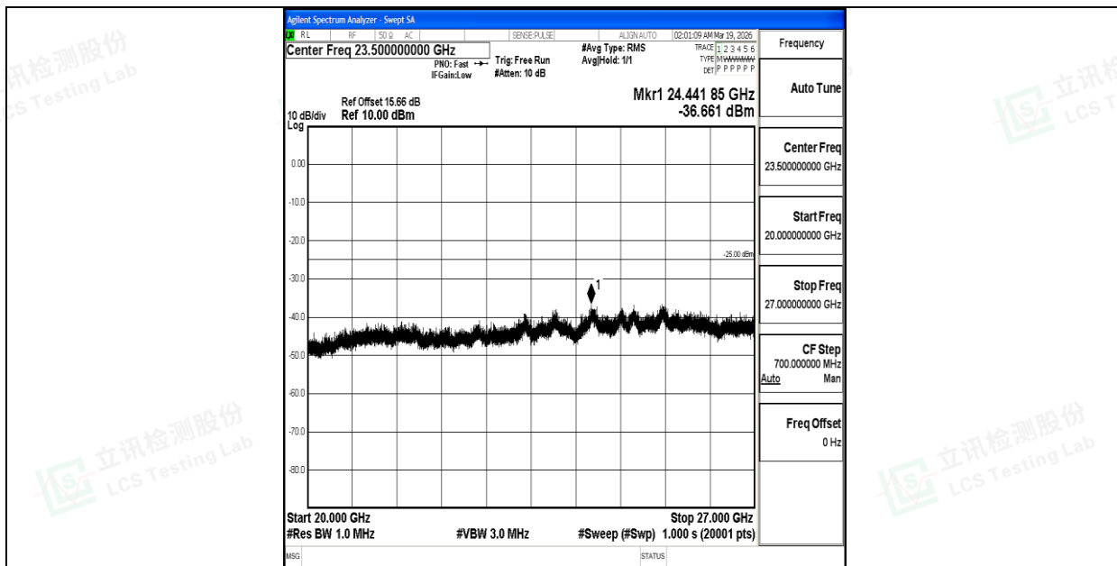
Band7_15MHz_QPSK_21375_1RB#0_20000~27000_20000~27000
