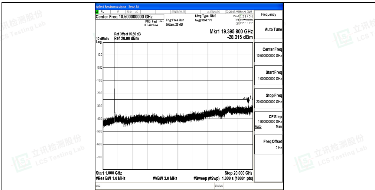
Band7_20MHz_16QAM_20850_1RB#0_1000~20000_1000~20000
