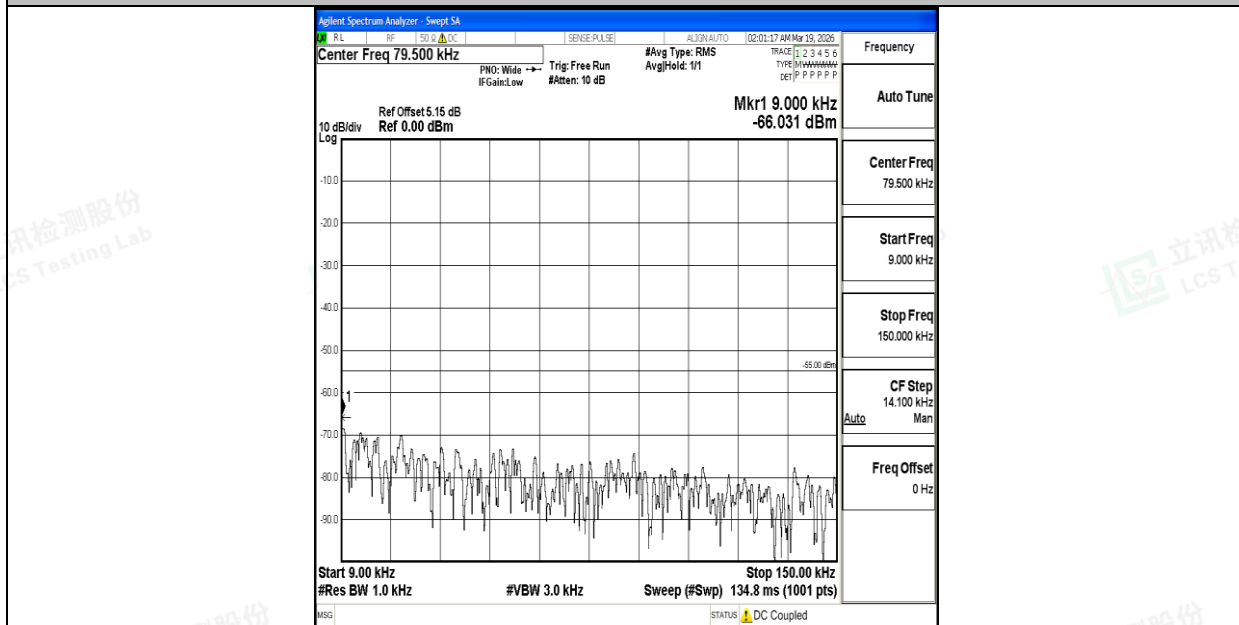
Band7_15MHz_16QAM_21375_1RB#0_0.009~0.15_0.009~0.15
