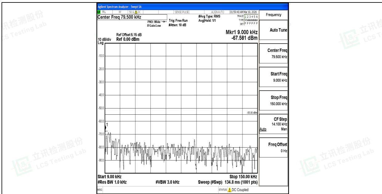
Band7_15MHz_QPSK_21100_1RB#0_0.009~0.15_0.009~0.15
