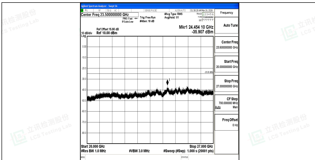
Band7_10MHz_QPSK_21100_1RB#0_20000~27000_20000~27000
