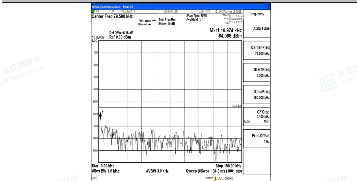
Band7_10MHz_16QAM_21400_1RB#0_0.009~0.15_0.009~0.15
