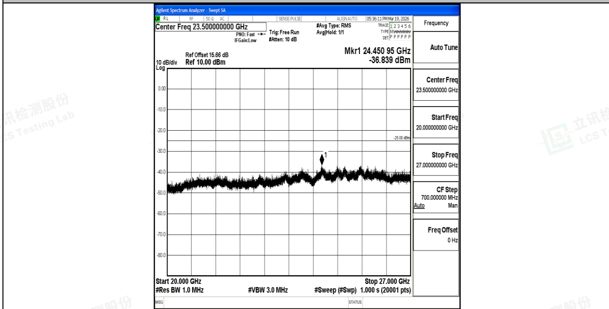
Band7_5MHz_16QAM_21425_1RB#0_20000~27000_20000~27000
