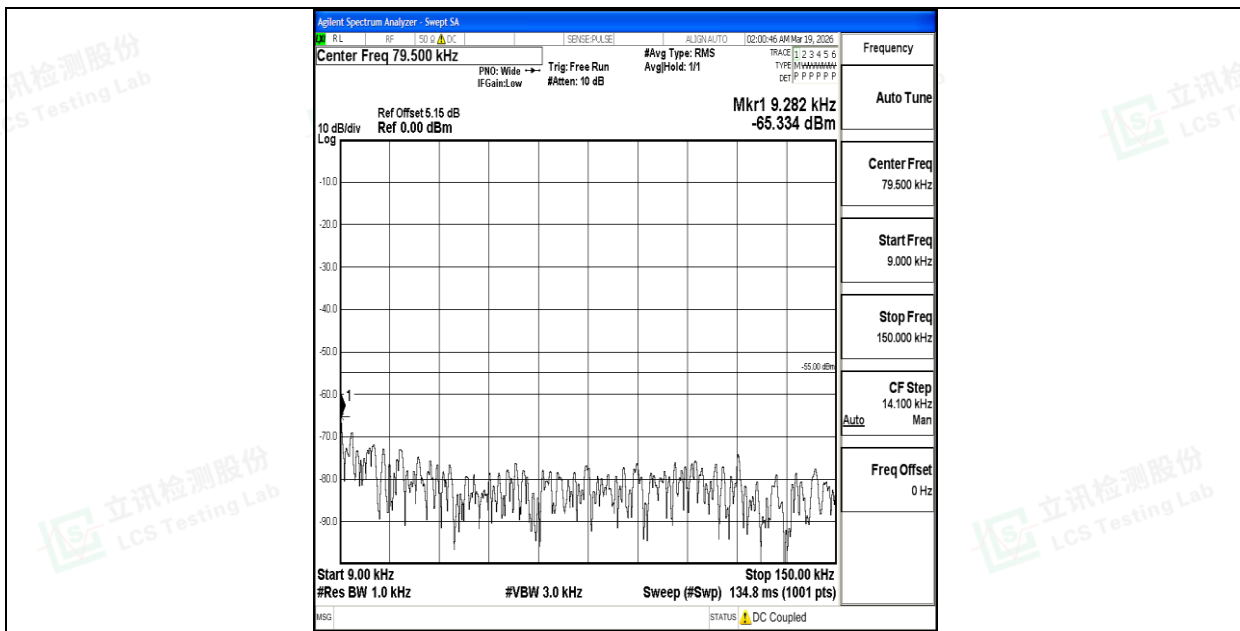
Band7_15MHz_QPSK_21375_1RB#0_0.009~0.15_0.009~0.15
