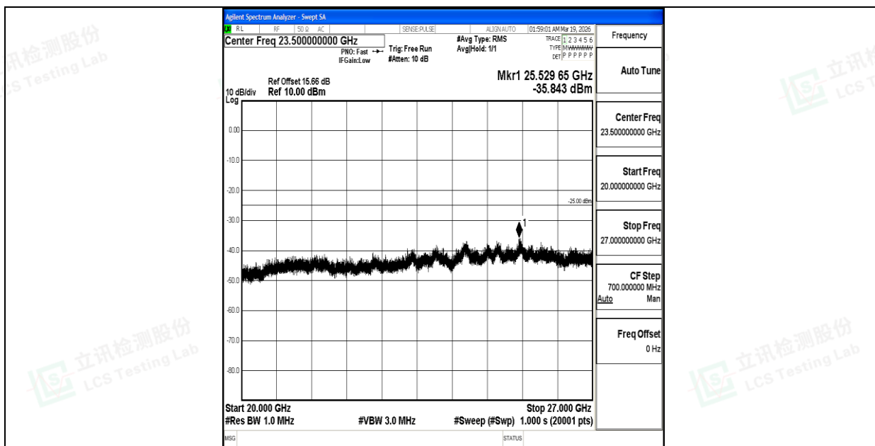
Band7_15MHz_QPSK_20825_1RB#0_20000~27000_20000~27000
