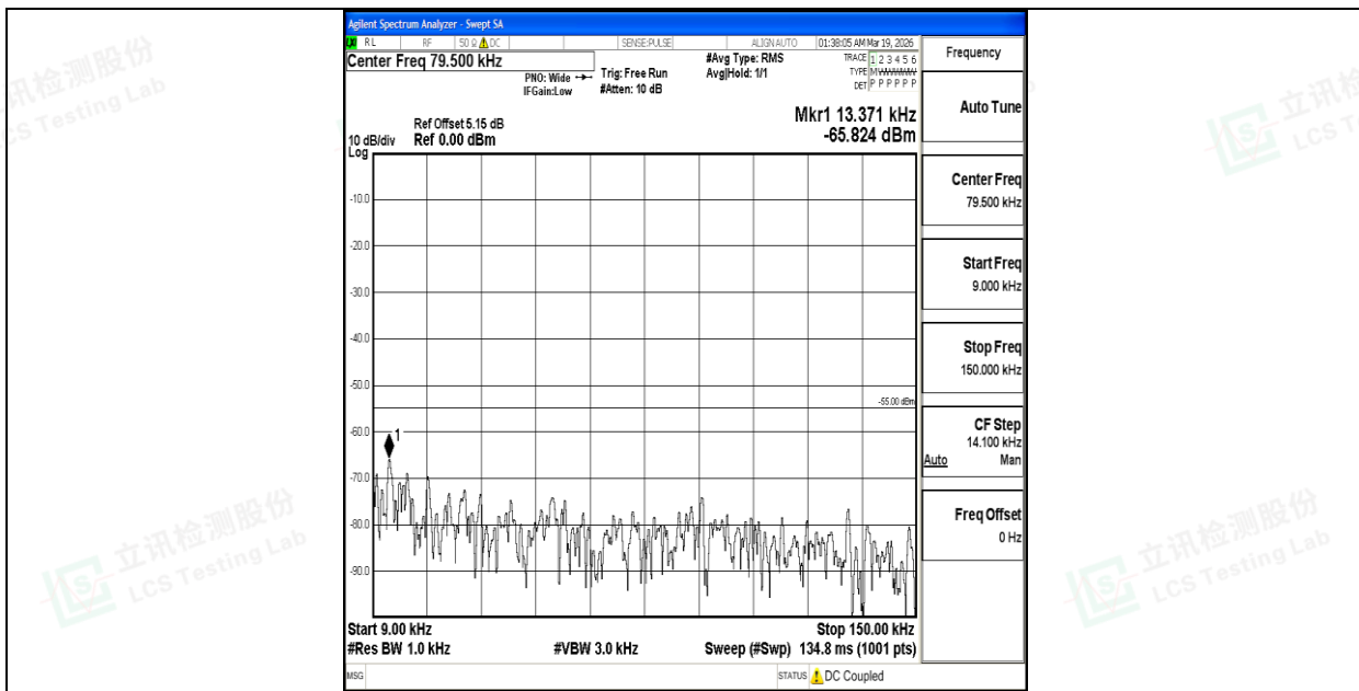
Band7_10MHz_QPSK_21100_1RB#0_0.009~0.15_0.009~0.15
