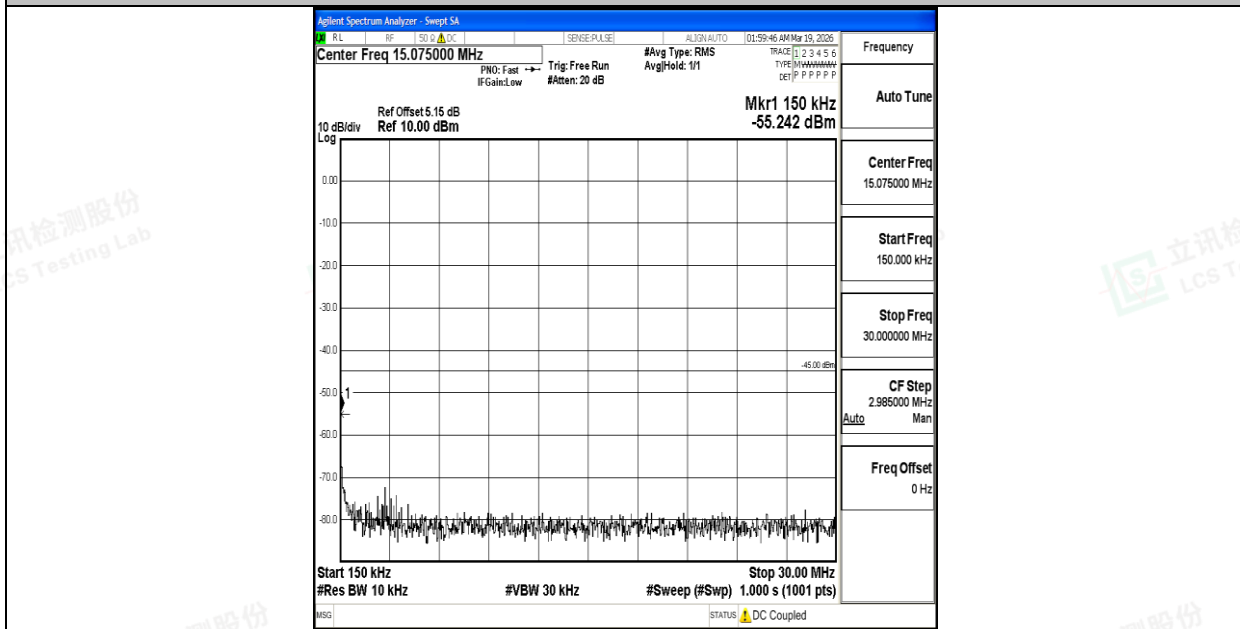
Band7_15MHz_QPSK_21100_1RB#0_0.15~30_0.15~30
