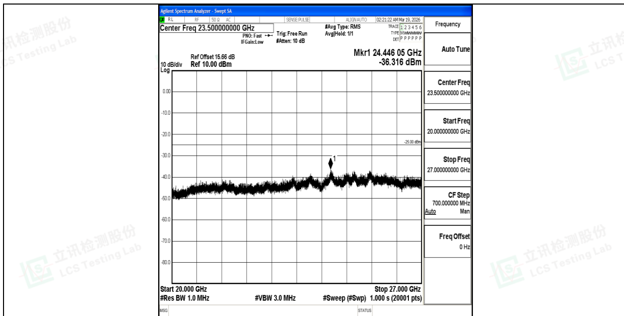
Band7_20MHz_QPSK_21100_1RB#0_20000~27000_20000~27000
