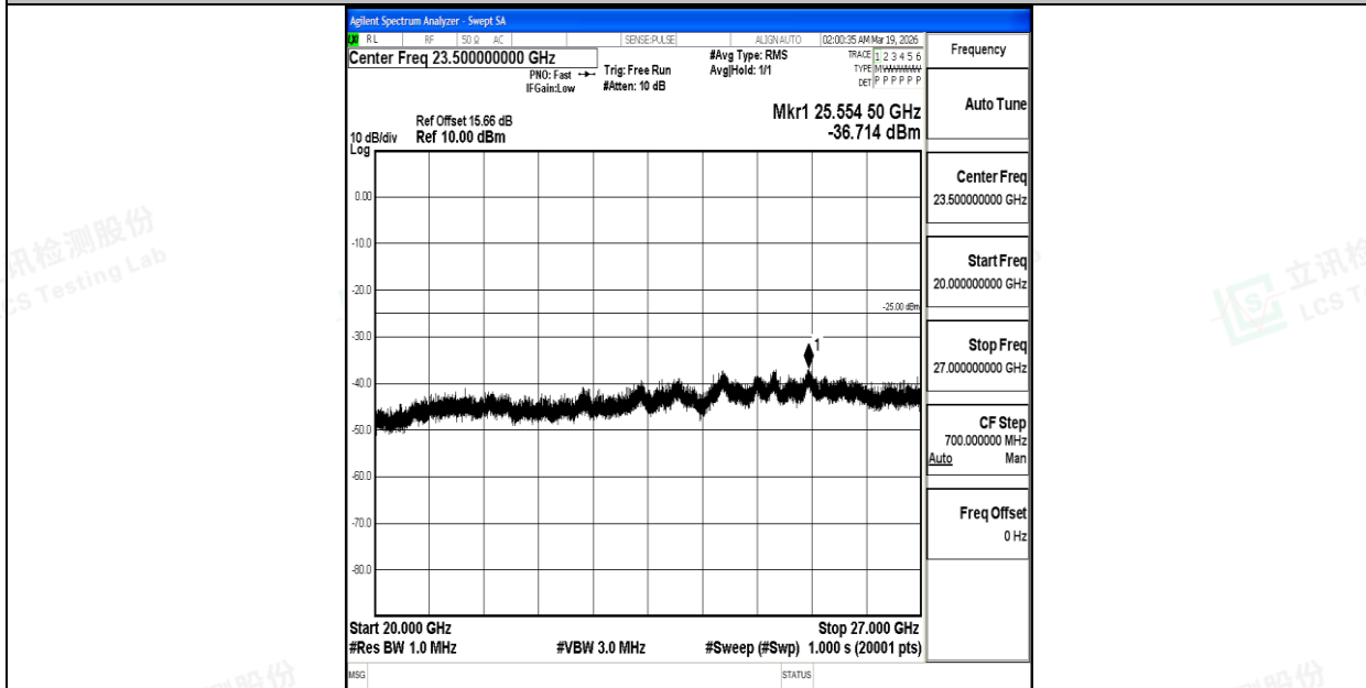
Band7_15MHz_16QAM_21100_1RB#0_20000~27000_20000~27000
