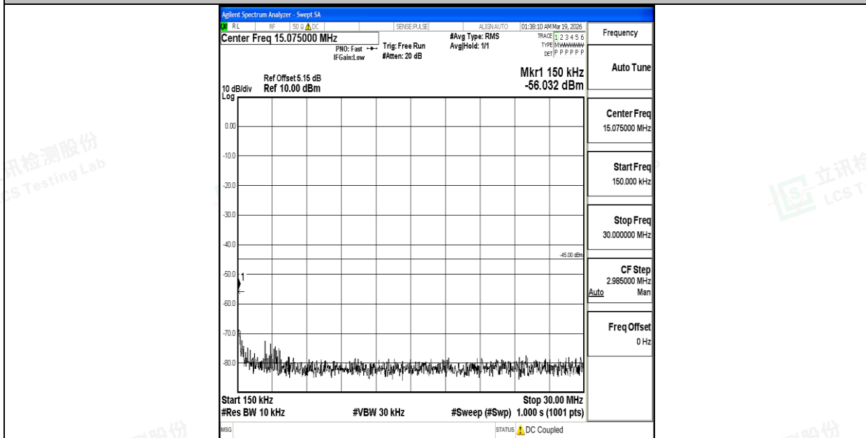
Band7_10MHz_QPSK_21100_1RB#0_0.15~30_0.15~30
