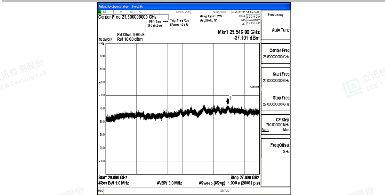
Band7_20MHz_16QAM_20850_1RB#0_20000~27000_20000~27000
