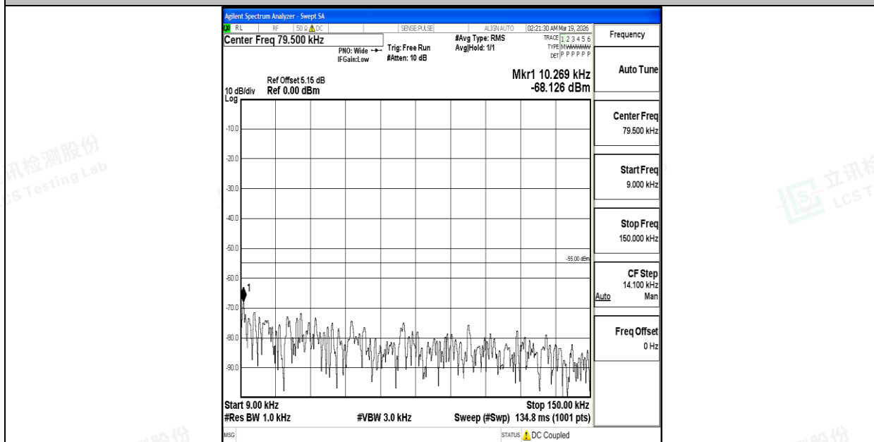
Band7_20MHz_16QAM_21100_1RB#0_0.009~0.15_0.009~0.15
