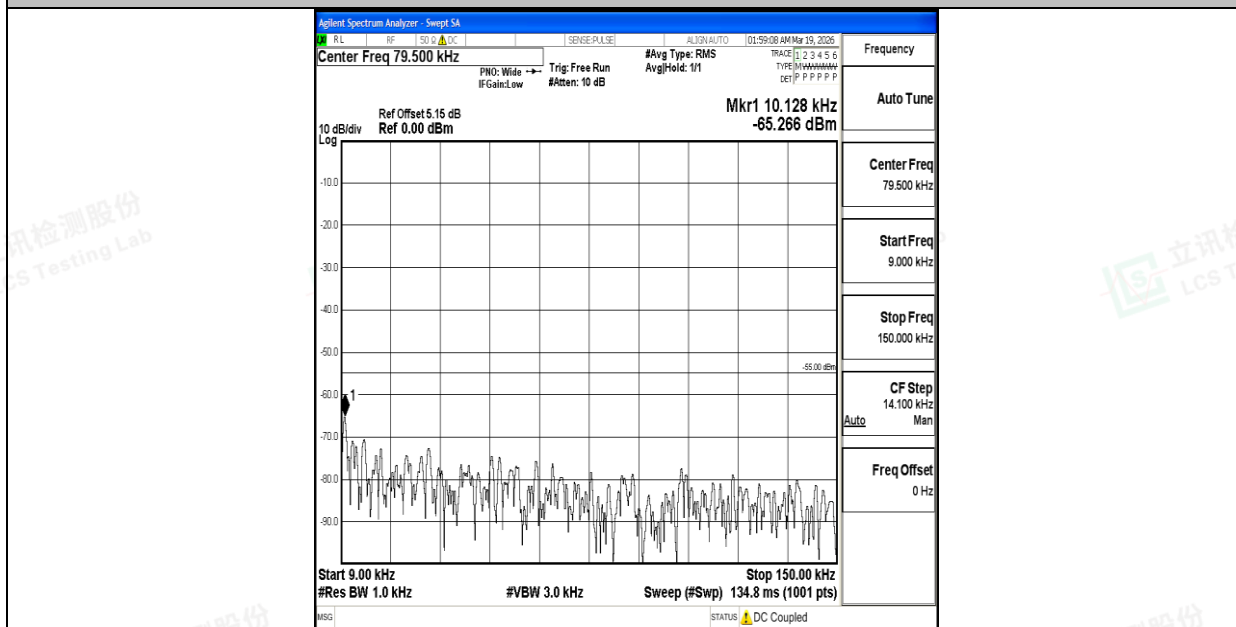
Band7_15MHz_16QAM_20825_1RB#0_0.009~0.15_0.009~0.15
