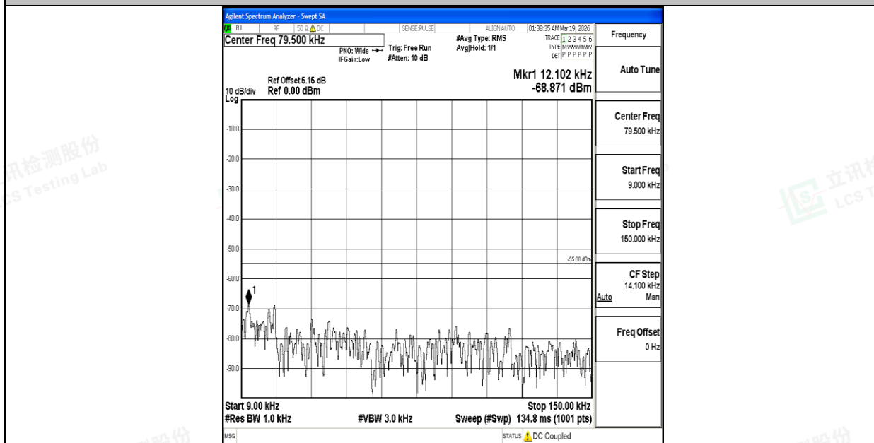
Band7_10MHz_16QAM_21100_1RB#0_0.009~0.15_0.009~0.15
