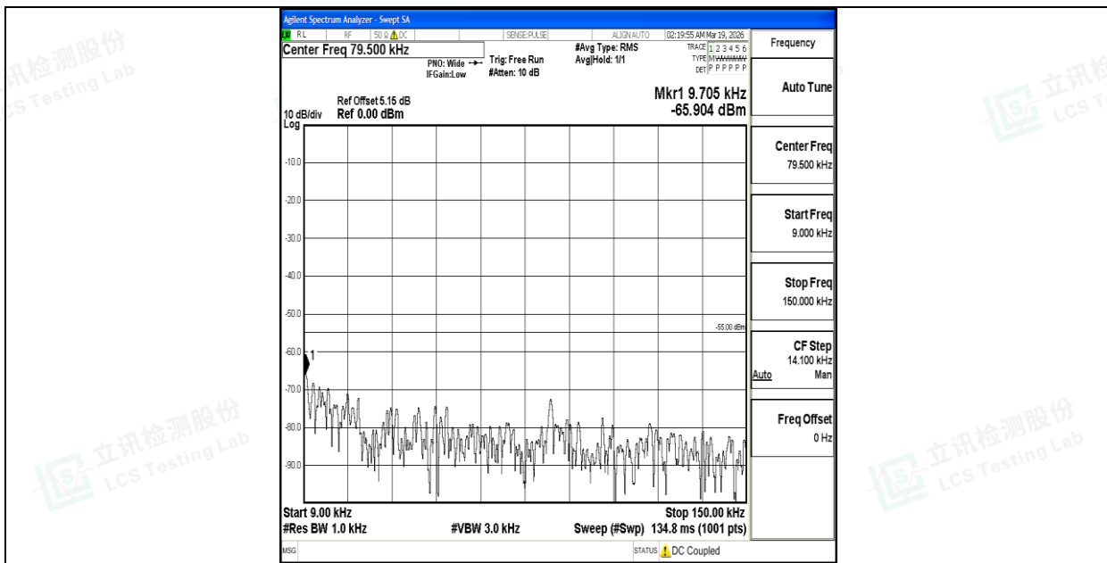
Band7_20MHz_QPSK_20850_1RB#0_0.009~0.15_0.009~0.15
