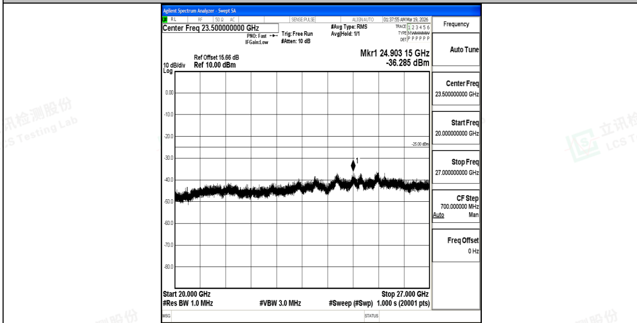
Band7_10MHz_16QAM_20800_1RB#0_20000~27000_20000~27000
