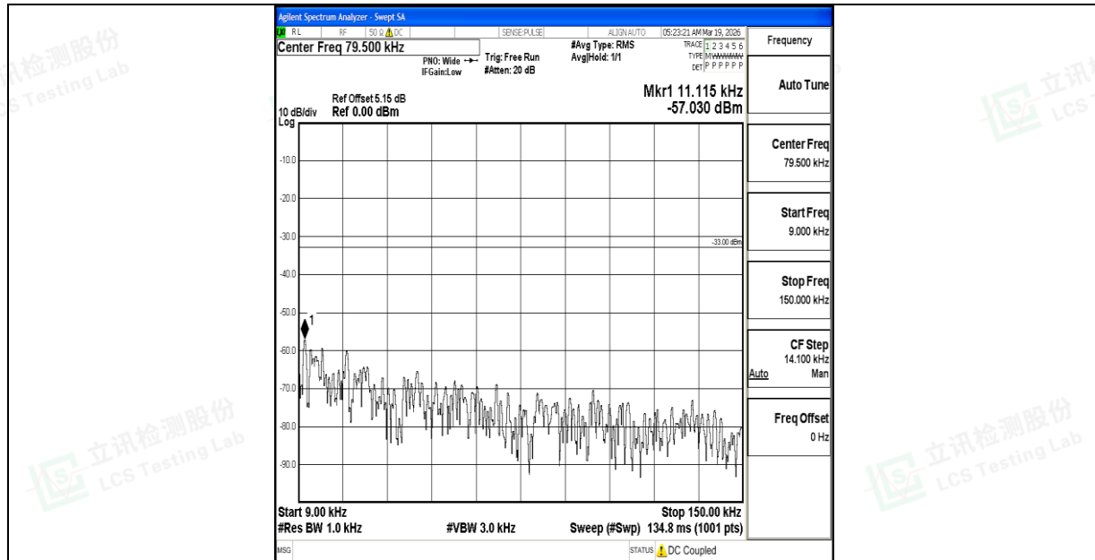
Band17_10MHz_16QAM_23800_1RB#0_0.009~0.15_0.009~0.15
