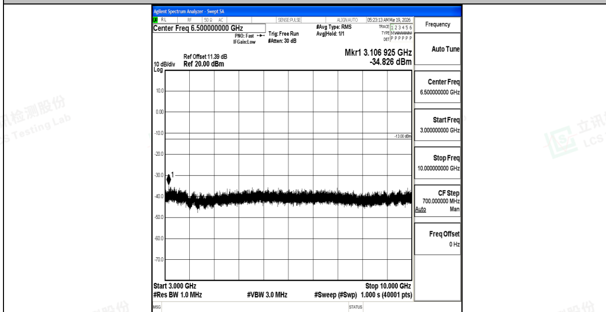
Band17_10MHz_QPSK_23800_1RB#0_3000~10000_3000~10000
