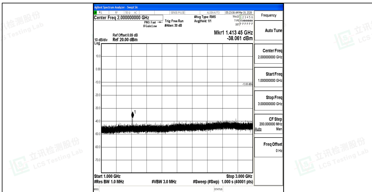
Band17_10MHz_QPSK_23800_1RB#0_1000~3000_1000~3000
