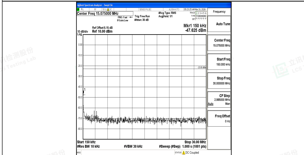
Band17_10MHz_16QAM_23800_1RB#0_0.15~30_0.15~30
