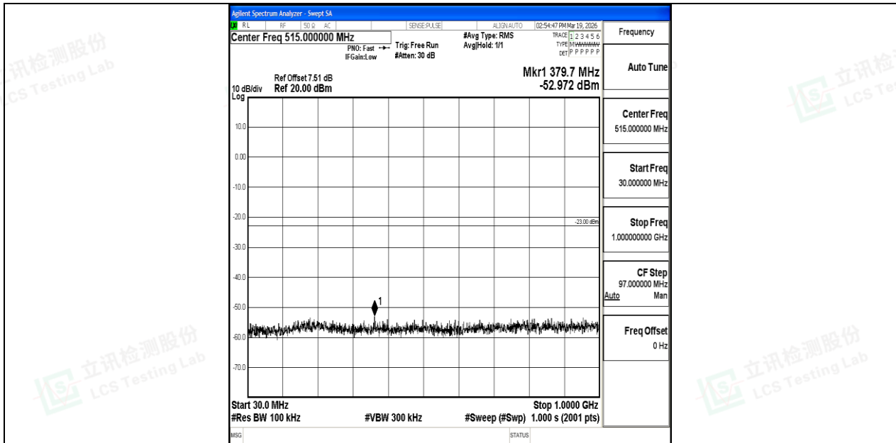
Band25_3MHz_16QAM_26675_1RB#0_30~1000_30~1000
