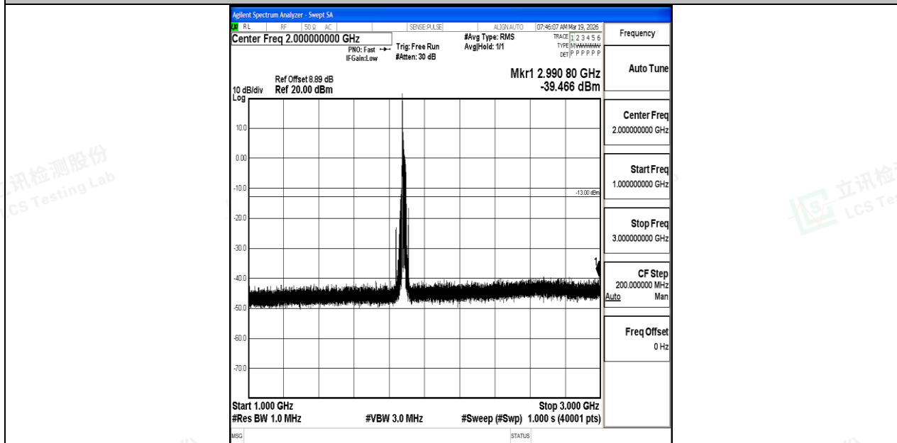
Band25_20MHz_QPSK_26365_1RB#0_1000~3000_1000~3000
