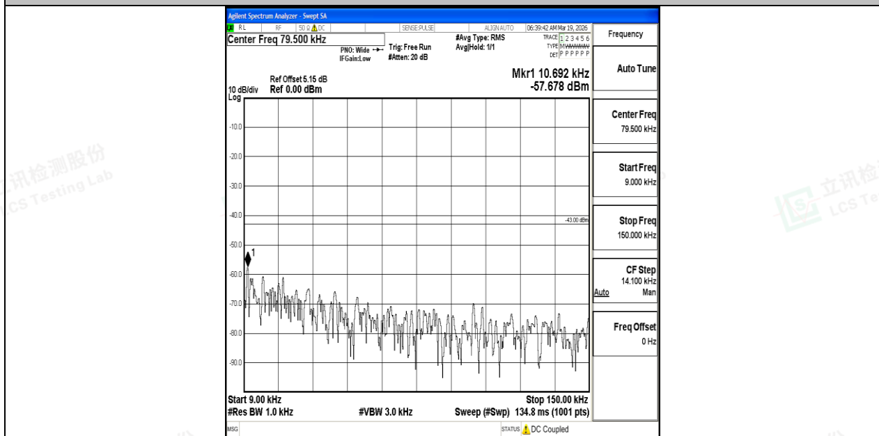
Band25_5MHz_16QAM_26665_1RB#0_0.009~0.15_0.009~0.15
