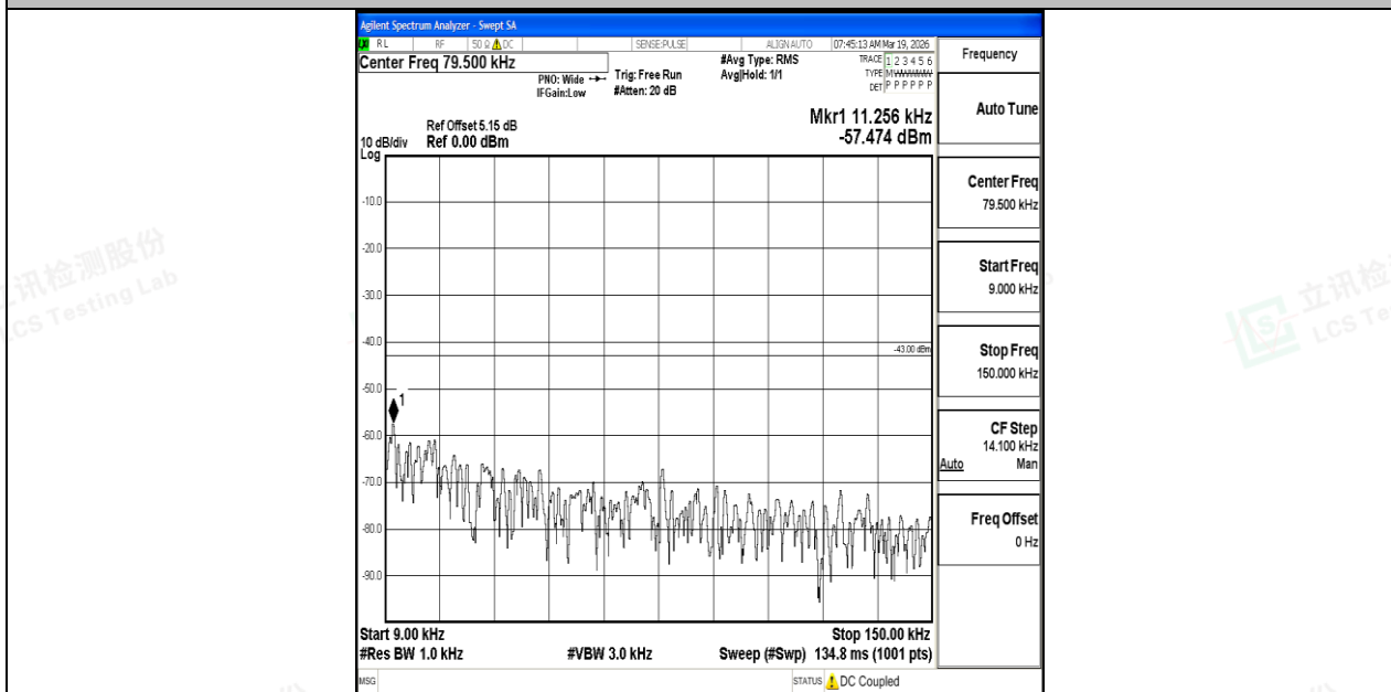
Band25_20MHz_16QAM_26140_1RB#0_0.009~0.15_0.009~0.15
