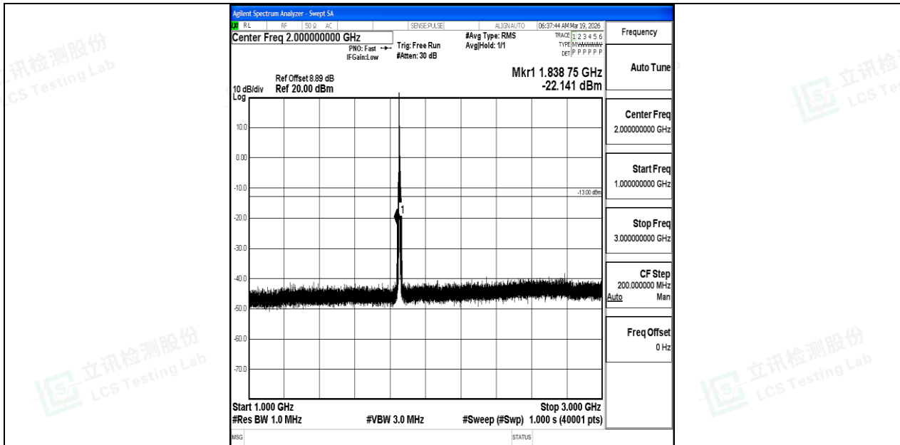
Band25_5MHz_16QAM_26065_1RB#0_1000~3000_1000~3000
