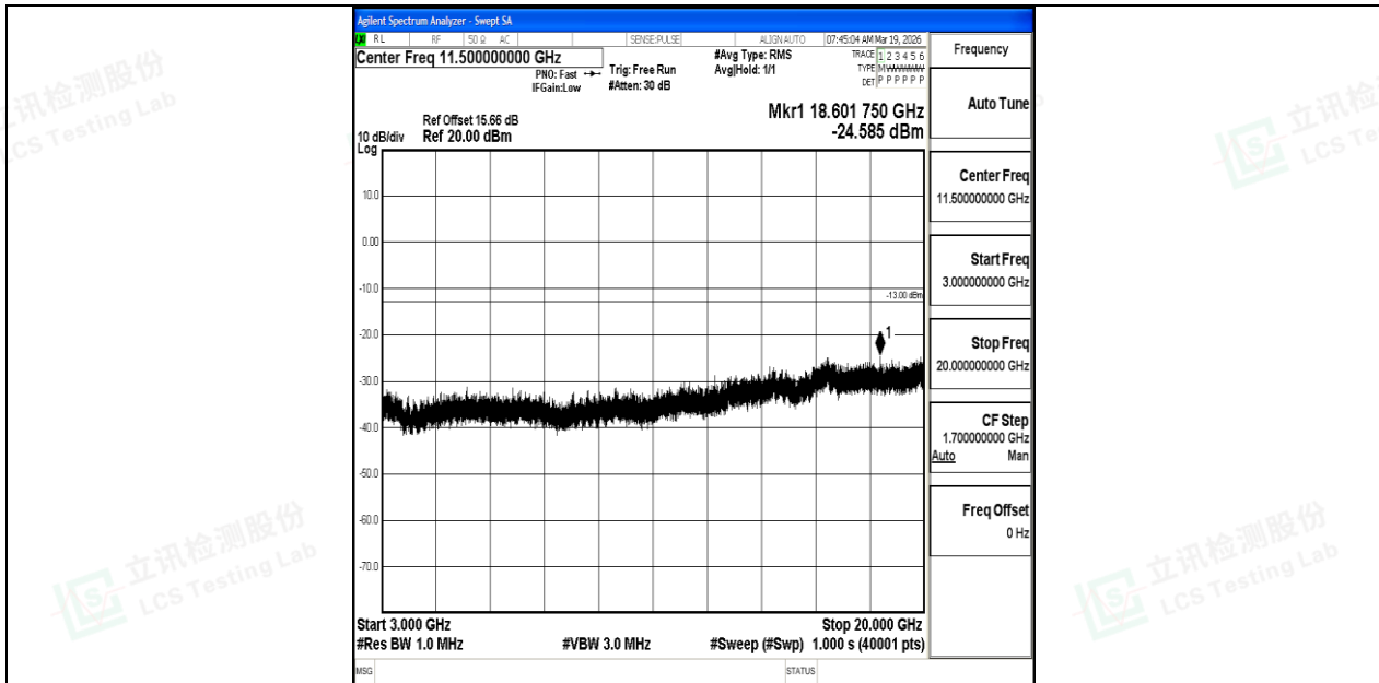
Band25_20MHz_QPSK_26140_1RB#0_3000~20000_3000~20000
