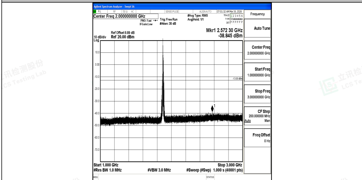
Band25_10MHz_QPSK_26365_1RB#0_1000~3000_1000~3000
