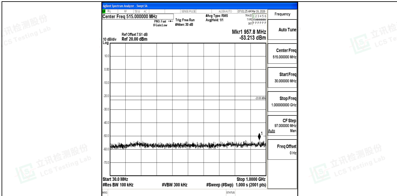
Band25_10MHz_QPSK_26365_1RB#0_30~1000_30~1000
