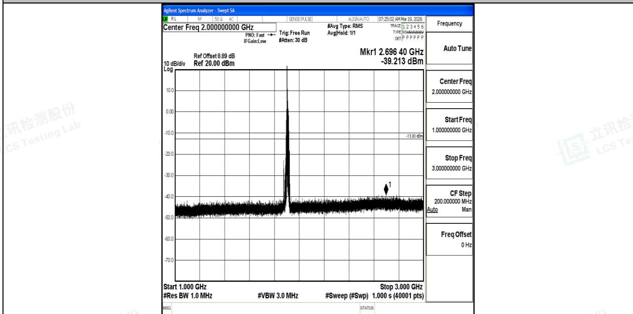
Band25_15MHz_QPSK_26615_1RB#0_1000~3000_1000~3000
