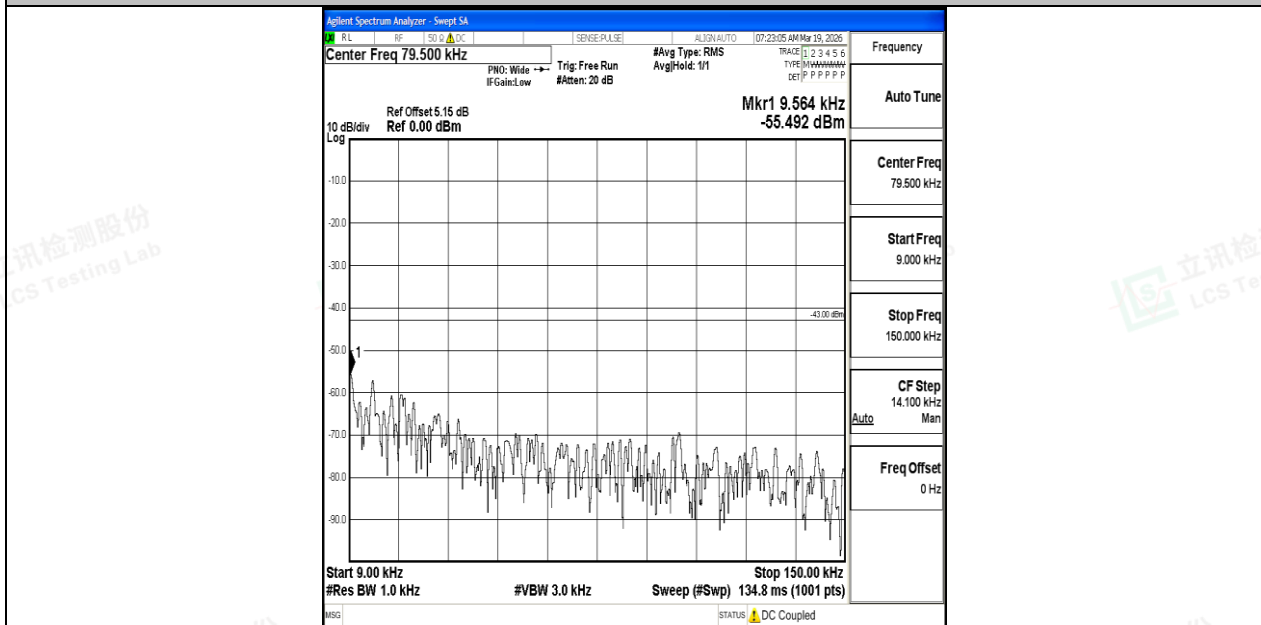
Band25_15MHz_16QAM_26115_1RB#0_0.009~0.15_0.009~0.15
