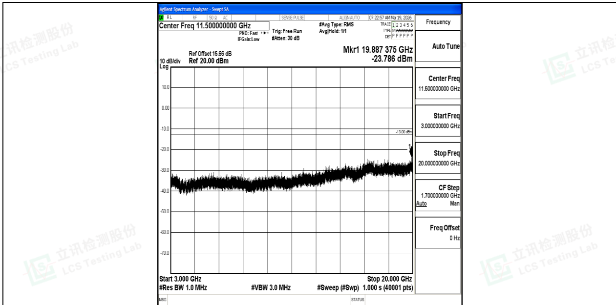
Band25_15MHz_QPSK_26115_1RB#0_3000~20000_3000~20000
