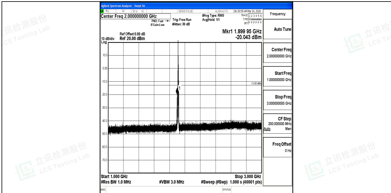
Band25_5MHz_16QAM_26665_1RB#0_1000~3000_1000~3000
