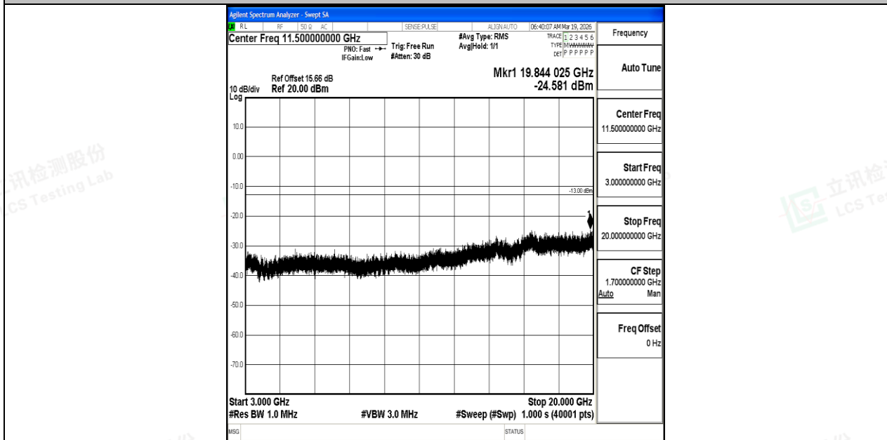
Band25_5MHz_16QAM_26665_1RB#0_3000~20000_3000~20000
