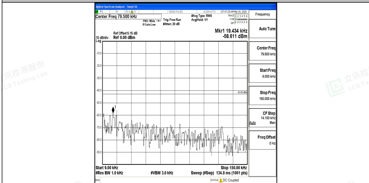
Band25_20MHz_16QAM_26590_1RB#0_0.009~0.15_0.009~0.15
