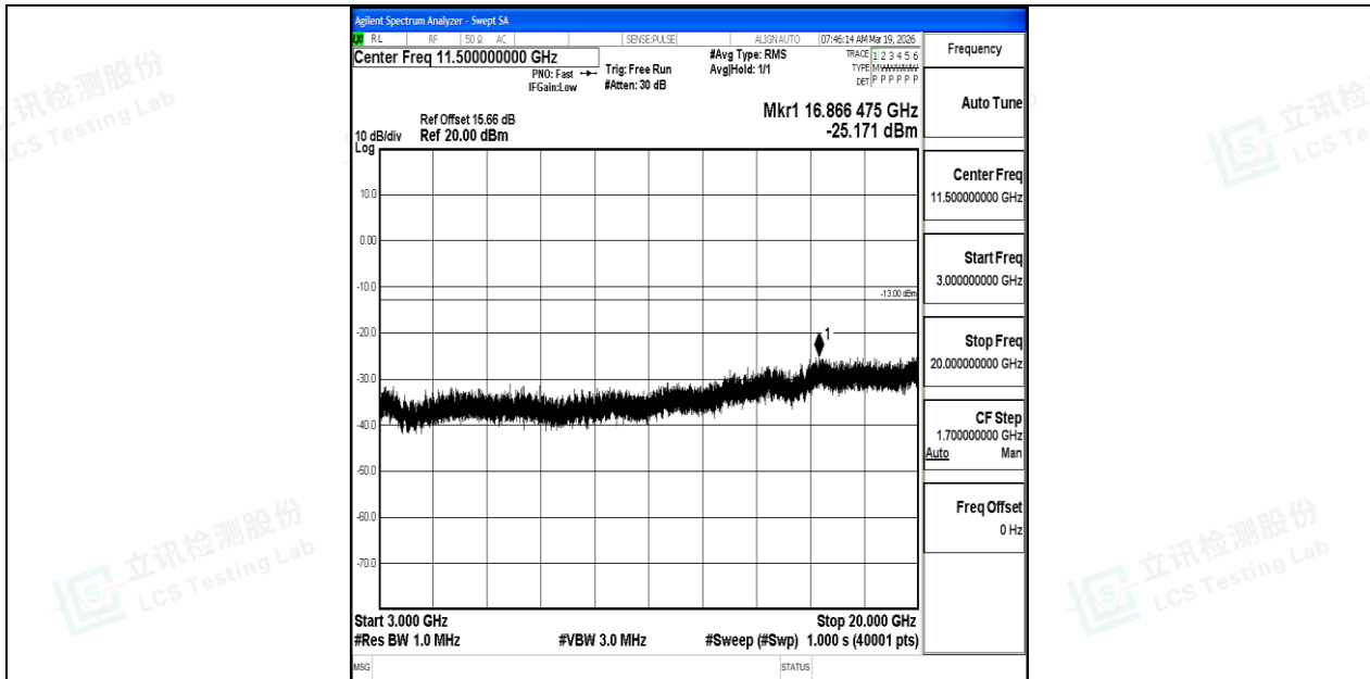
Band25_20MHz_QPSK_26365_1RB#0_3000~20000_3000~20000
