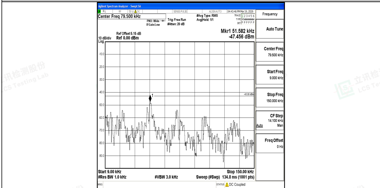
Band25_1.4MHz_16QAM_26365_1RB#0_0.009~0.15_0.009~0.15
