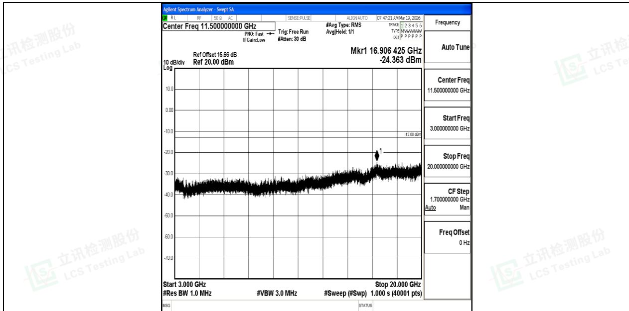
Band25_20MHz_QPSK_26590_1RB#0_3000~20000_3000~20000
