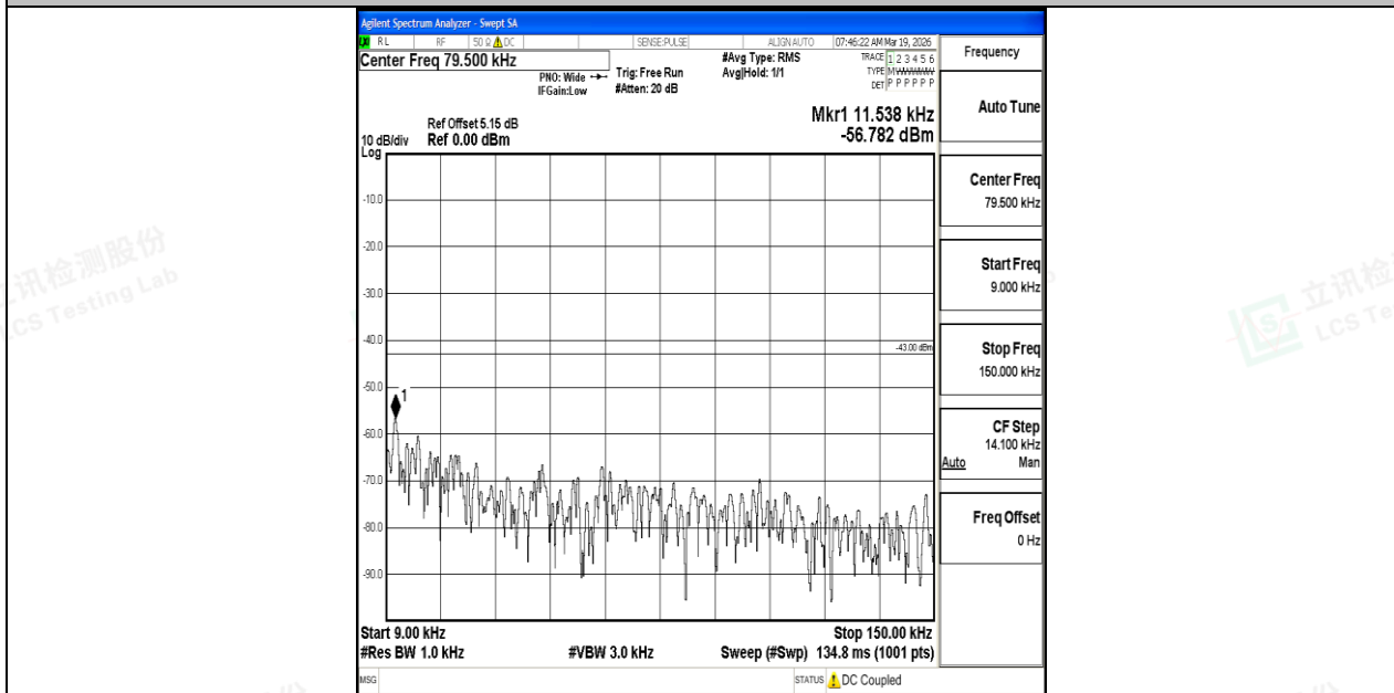
Band25_20MHz_16QAM_26365_1RB#0_0.009~0.15_0.009~0.15
