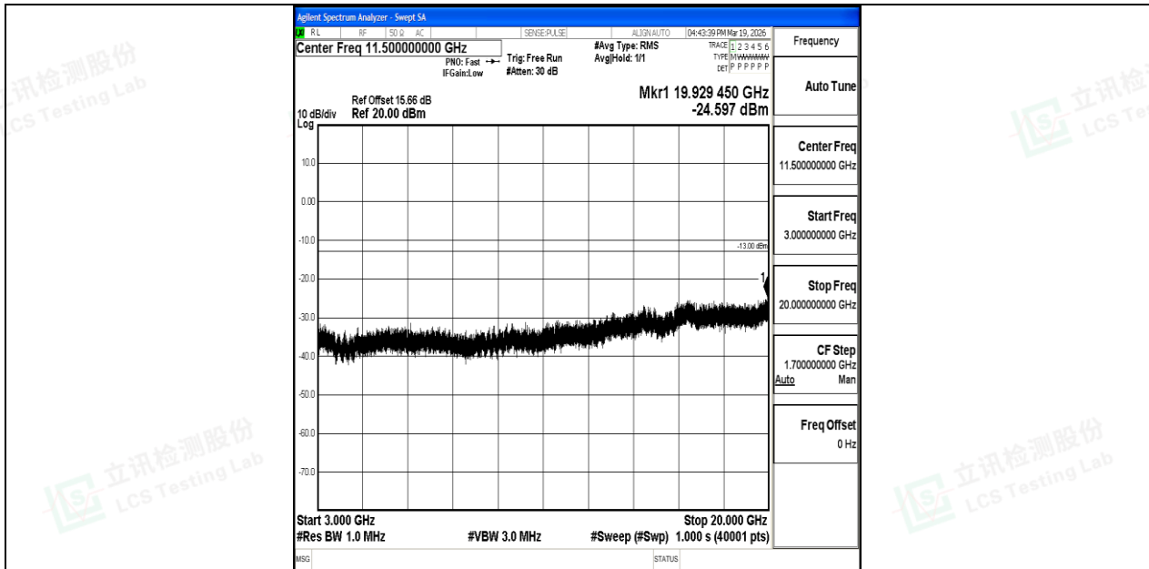
Band25_1.4MHz_QPSK_26365_1RB#0_3000~20000_3000~20000
