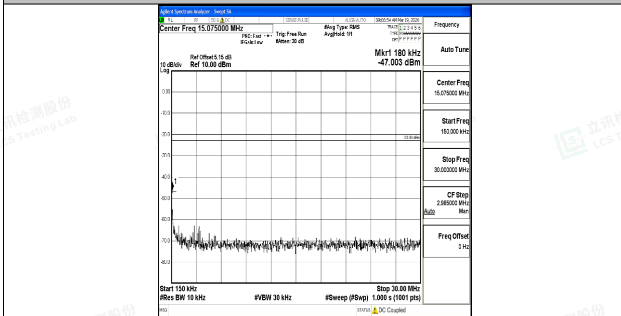
Band26_5MHz_16QAM_26765_1RB#0_0.15~30_0.15~30
