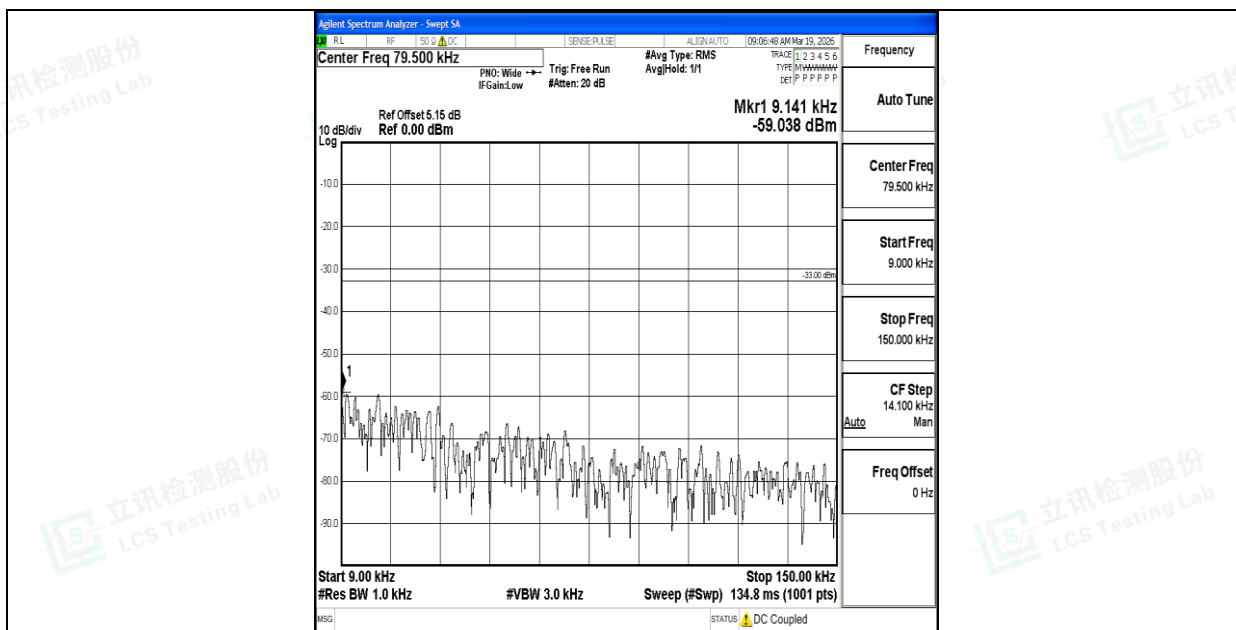
Band26_5MHz_16QAM_26765_1RB#0_0.009~0.15_0.009~0.15
