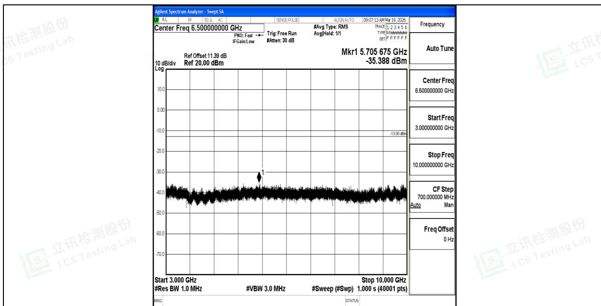
Band26_5MHz_16QAM_26765_1RB#0_3000~10000_3000~10000
