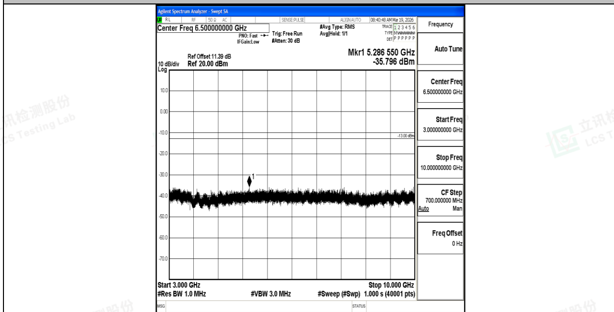
Band26_3MHz_QPSK_26775_1RB#0_3000~10000_3000~10000
