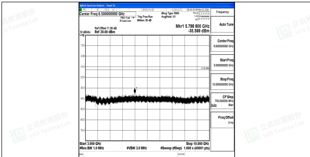
Band26_3MHz_16QAM_26740_1RB#0_3000~10000_3000~10000
