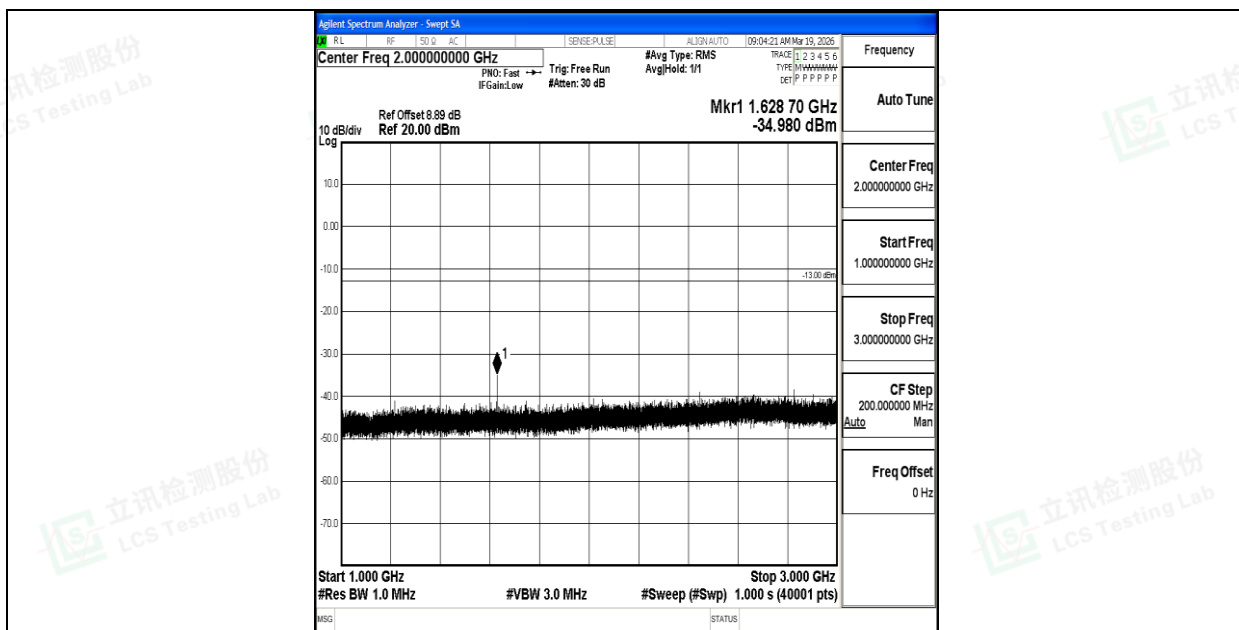
Band26_5MHz_QPSK_26715_1RB#0_1000~3000_1000~3000
