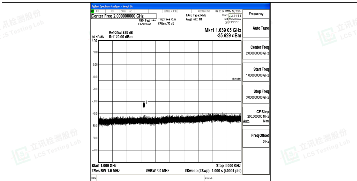
Band26_5MHz_QPSK_26765_1RB#0_1000~3000_1000~3000
