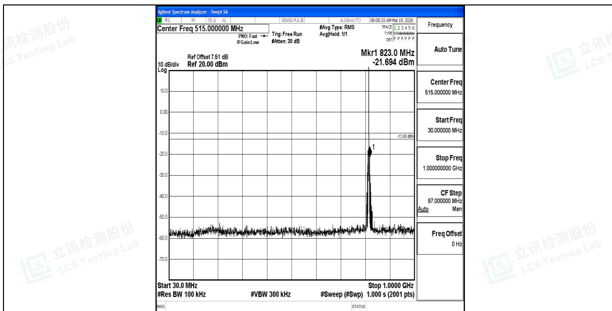
Band26_1.4MHz_16QAM_26740_1RB#0_30~1000_30~1000
