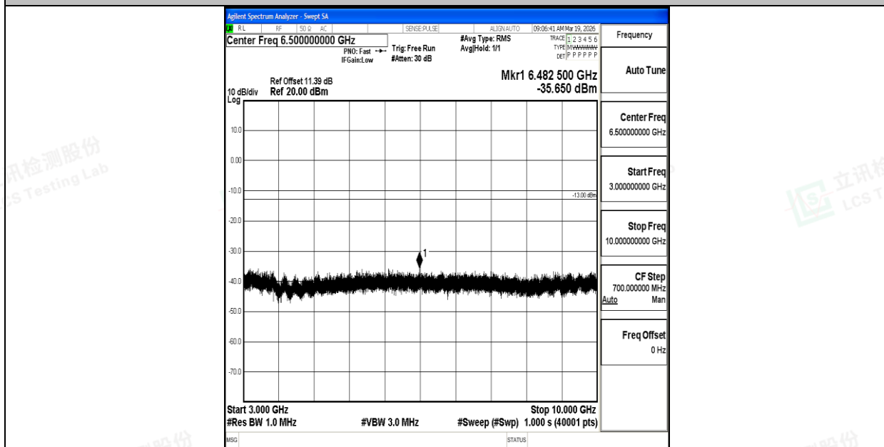
Band26_5MHz_QPSK_26765_1RB#0_3000~10000_3000~10000
