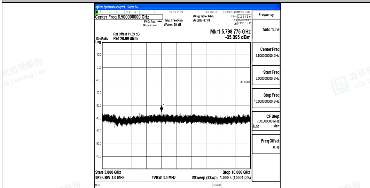
Band26_1.4MHz_QPSK_26783_1RB#0_3000~10000_3000~10000
