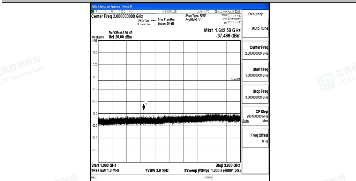
Band26_3MHz_16QAM_26775_1RB#0_1000~3000_1000~3000
