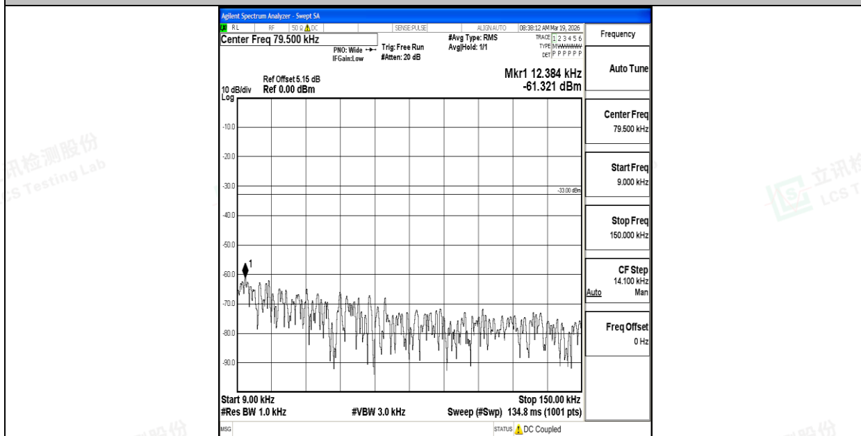
Band26_3MHz_QPSK_26705_1RB#0_0.009~0.15_0.009~0.15
