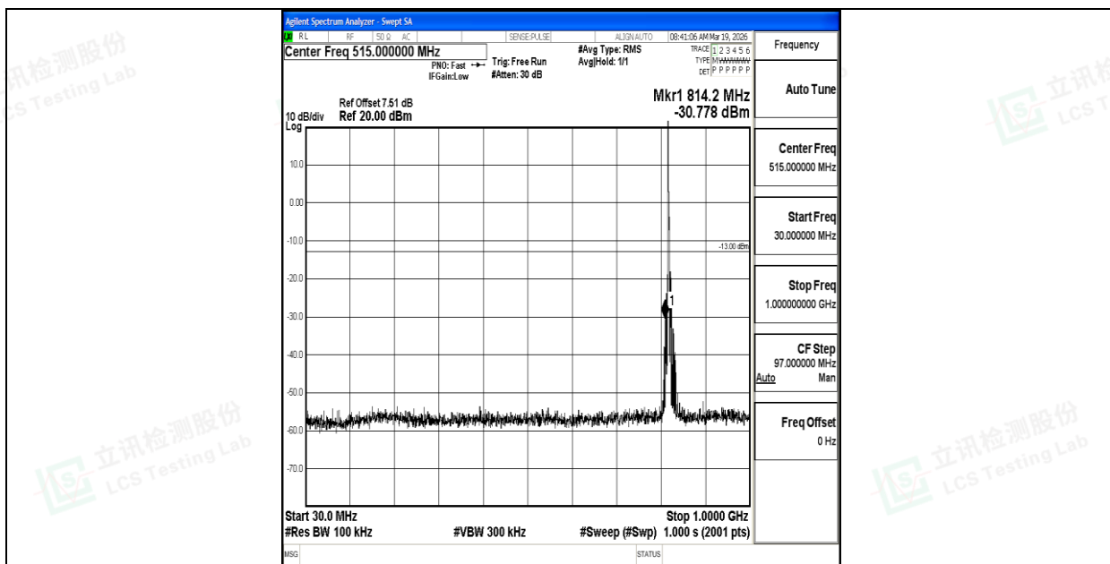
Band26_3MHz_16QAM_26775_1RB#0_30~1000_30~1000
