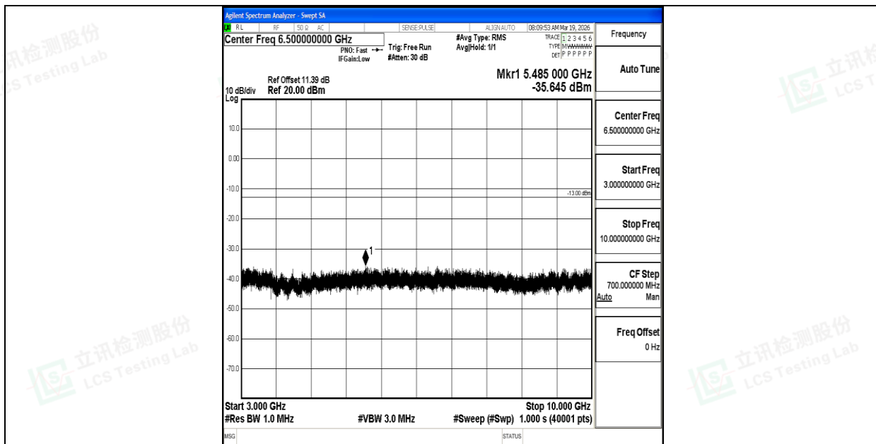
Band26_1.4MHz_16QAM_26783_1RB#0_3000~10000_3000~10000
