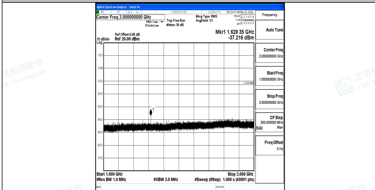
Band26_10MHz_16QAM_26740_1RB#0_1000~3000_1000~3000
