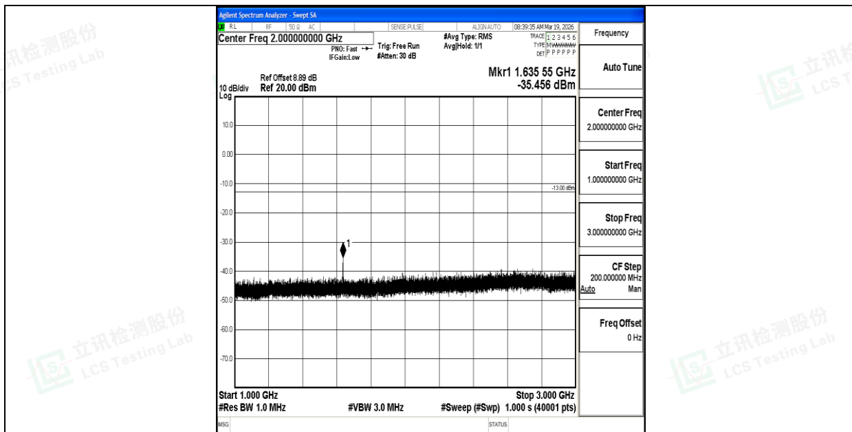
Band26_3MHz_QPSK_26740_1RB#0_1000~3000_1000~3000
