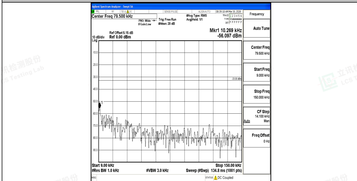
Band26_3MHz_QPSK_26740_1RB#0_0.009~0.15_0.009~0.15
