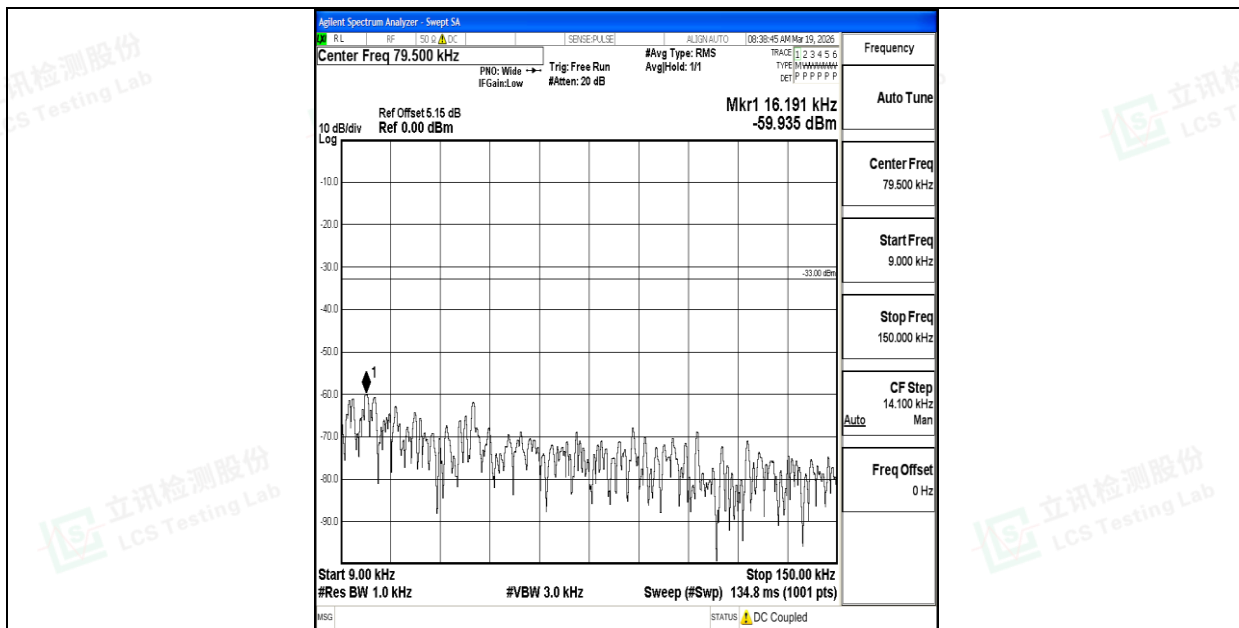
Band26_3MHz_16QAM_26705_1RB#0_0.009~0.15_0.009~0.15
