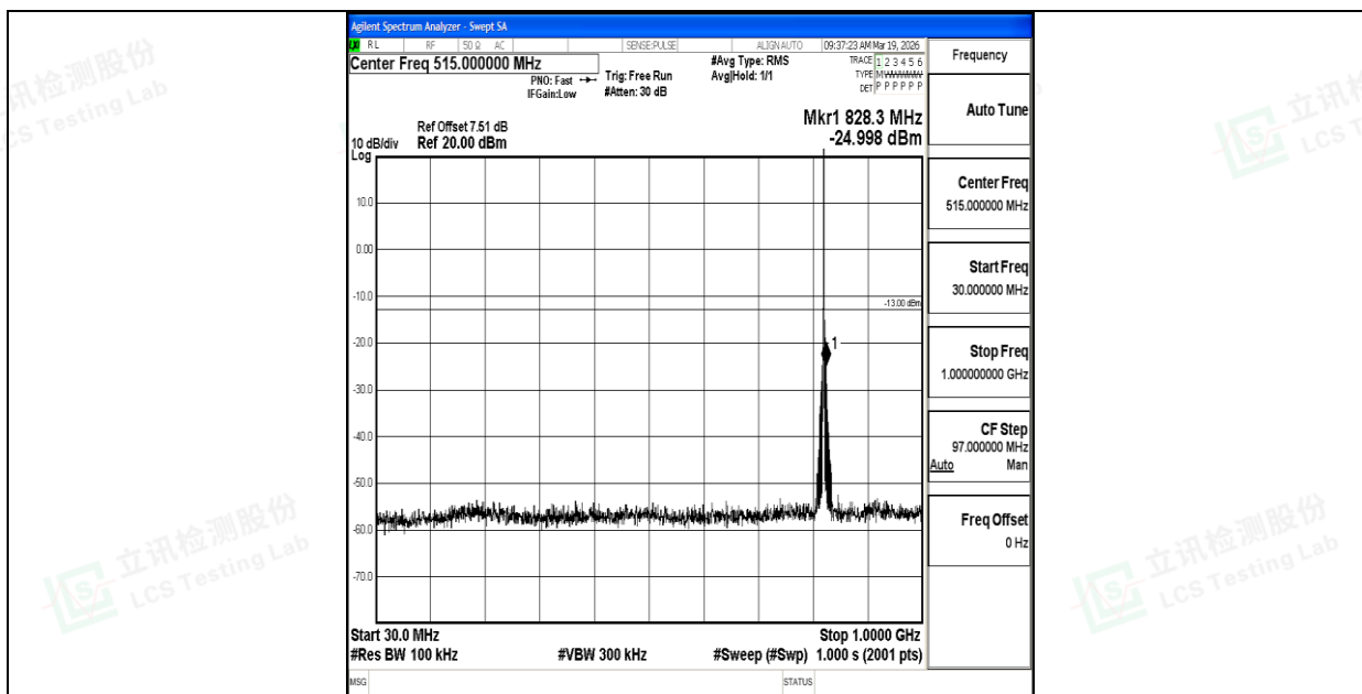
Band26_1.4MHz_QPSK_26797_1RB#0_30~1000_30~1000
