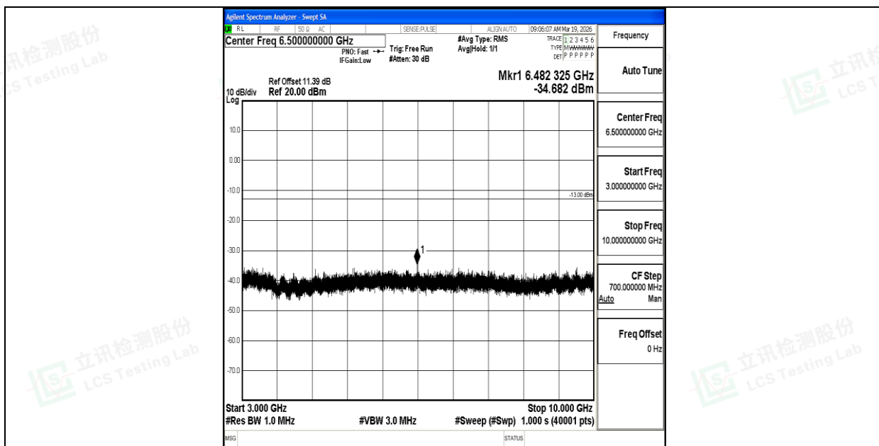
Band26_5MHz_16QAM_26740_1RB#0_3000~10000_3000~10000
