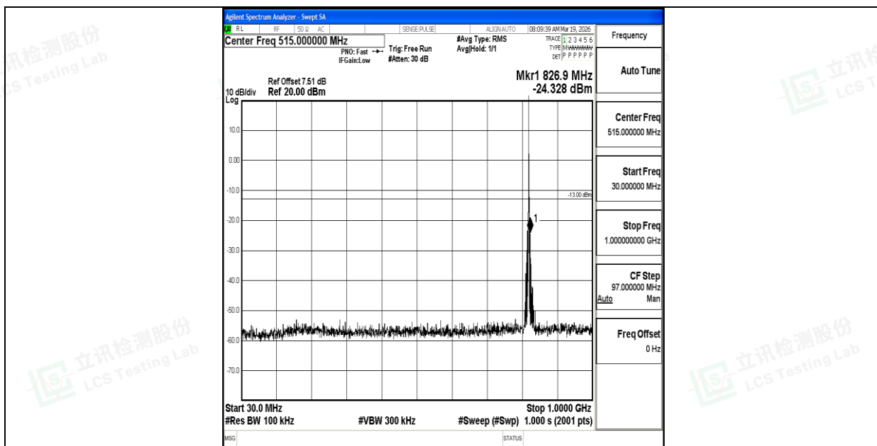
Band26_1.4MHz_16QAM_26783_1RB#0_30~1000_30~1000
