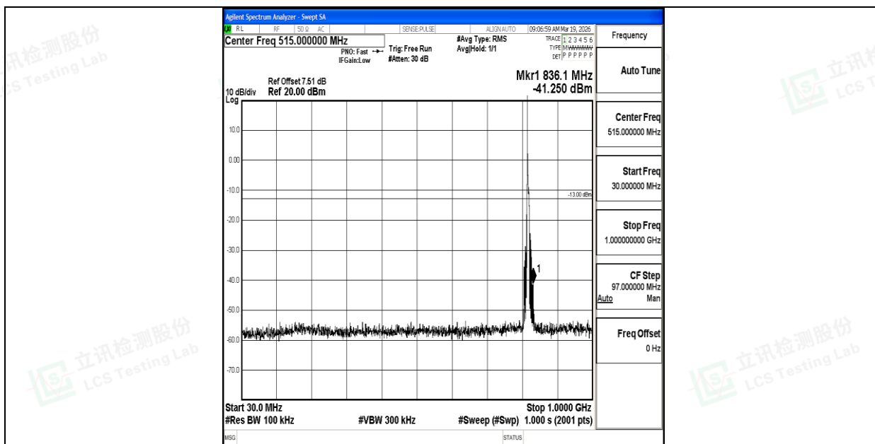
Band26_5MHz_16QAM_26765_1RB#0_30~1000_30~1000
