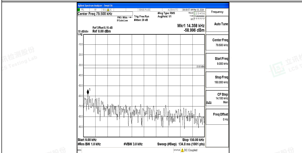
Band26_1.4MHz_QPSK_26783_1RB#0_0.009~0.15_0.009~0.15
