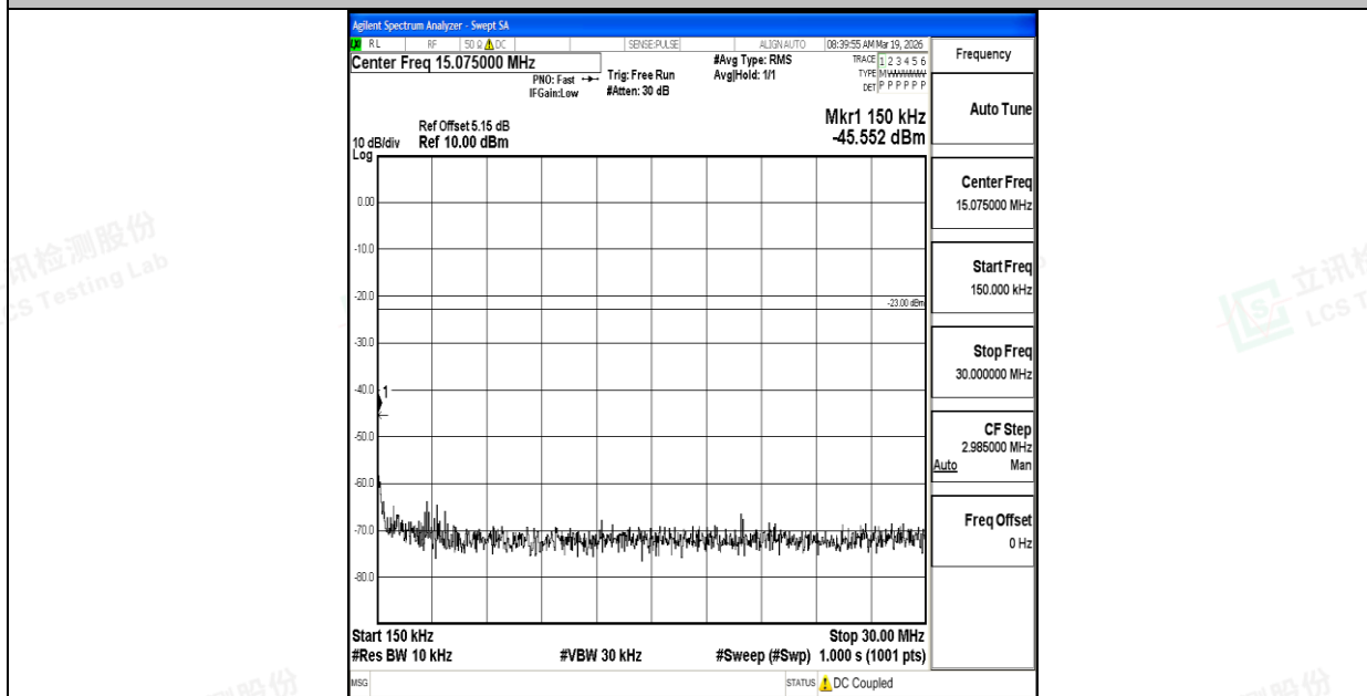
Band26_3MHz_16QAM_26740_1RB#0_0.15~30_0.15~30
