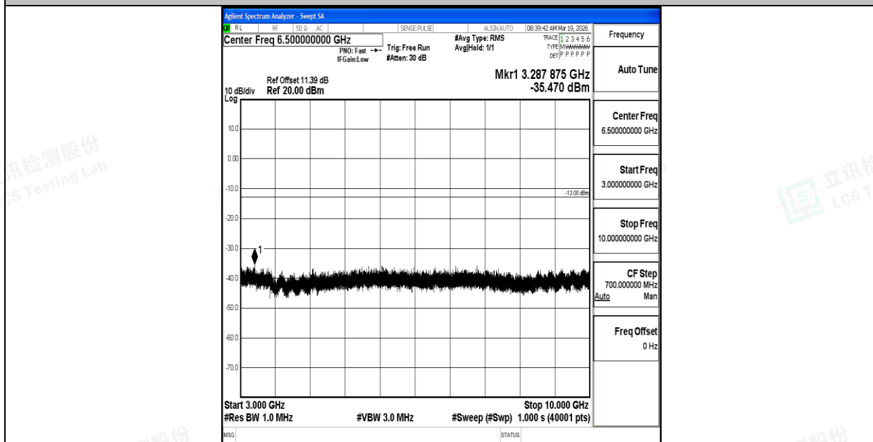
Band26_3MHz_QPSK_26740_1RB#0_3000~10000_3000~10000
