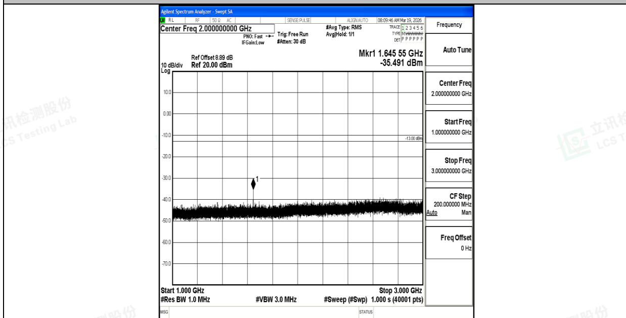
Band26_1.4MHz_16QAM_26783_1RB#0_1000~3000_1000~3000
