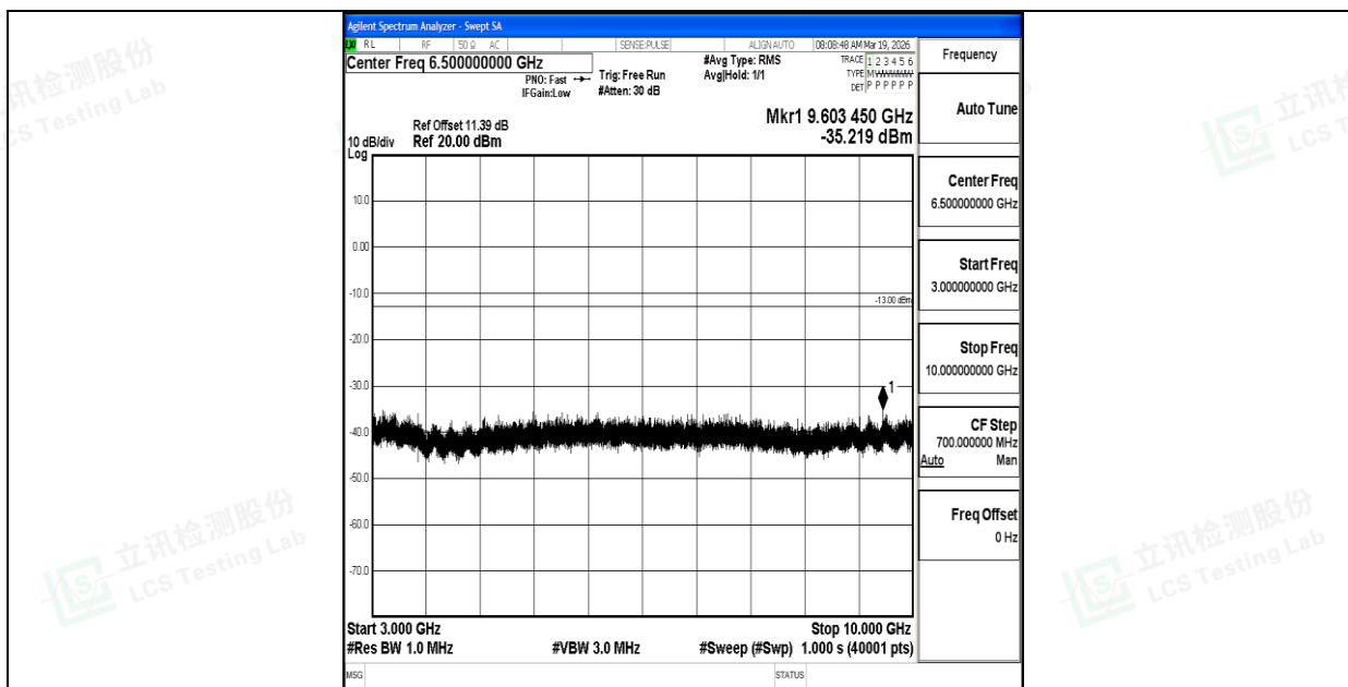
Band26_1.4MHz_16QAM_26740_1RB#0_3000~10000_3000~10000
