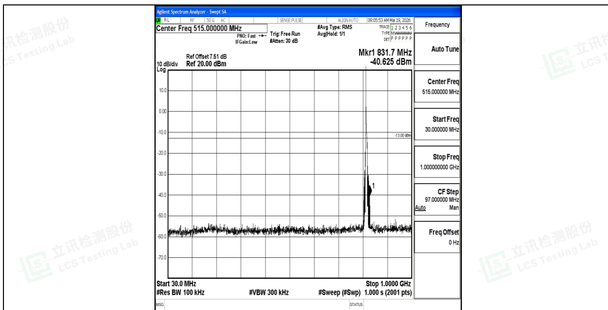
Band26_5MHz_16QAM_26740_1RB#0_30~1000_30~1000
