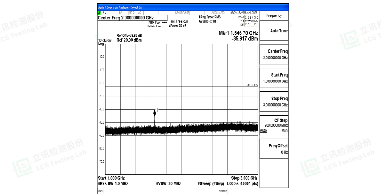
Band26_1.4MHz_QPSK_26783_1RB#0_1000~3000_1000~3000
