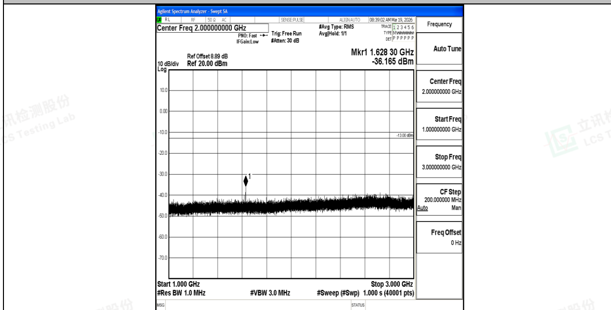
Band26_3MHz_16QAM_26705_1RB#0_1000~3000_1000~3000
