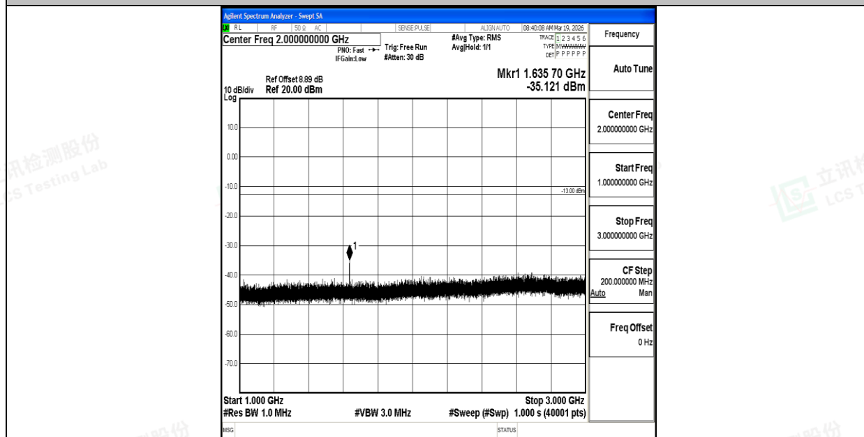
Band26_3MHz_16QAM_26740_1RB#0_1000~3000_1000~3000
