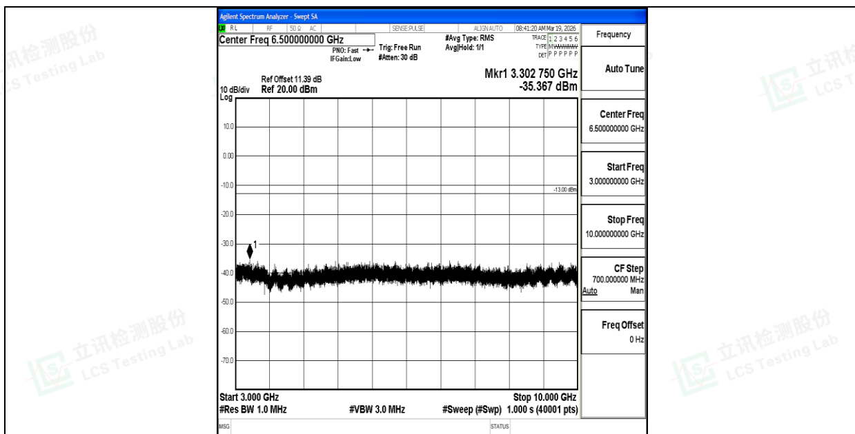
Band26_3MHz_16QAM_26775_1RB#0_3000~10000_3000~10000
