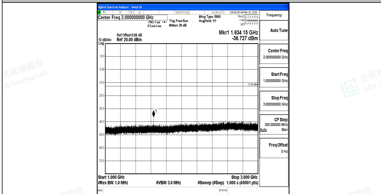
Band26_5MHz_16QAM_26740_1RB#0_1000~3000_1000~3000
