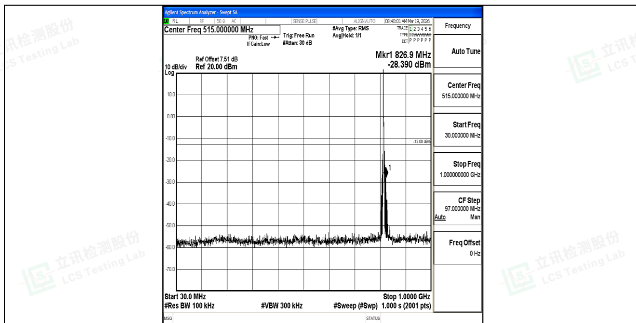
Band26_3MHz_16QAM_26740_1RB#0_30~1000_30~1000
