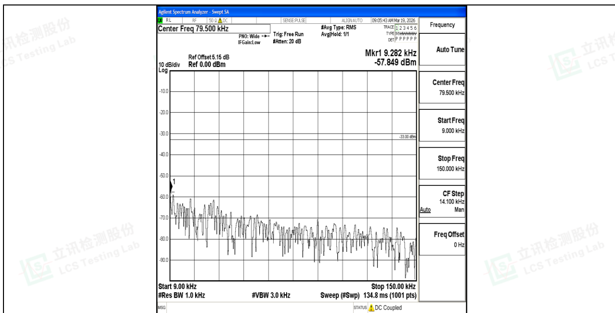
Band26_5MHz_16QAM_26740_1RB#0_0.009~0.15_0.009~0.15
