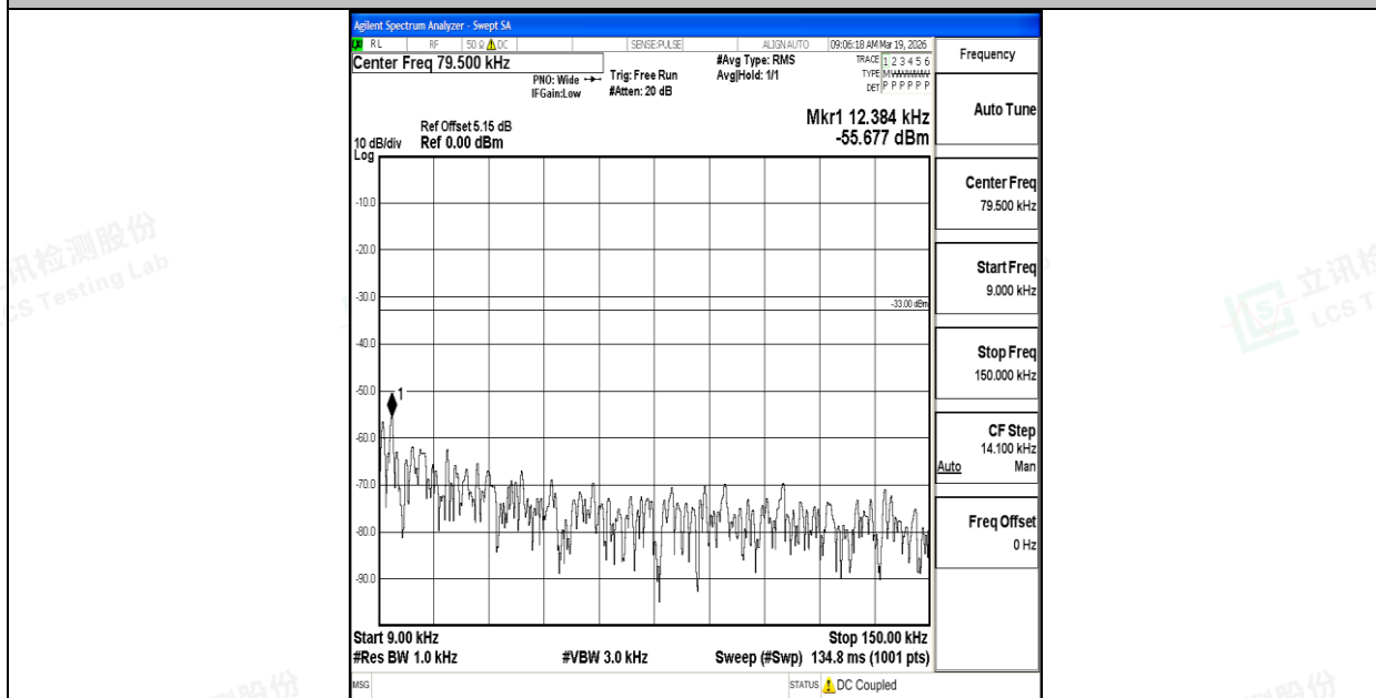
Band26_5MHz_QPSK_26765_1RB#0_0.009~0.15_0.009~0.15
