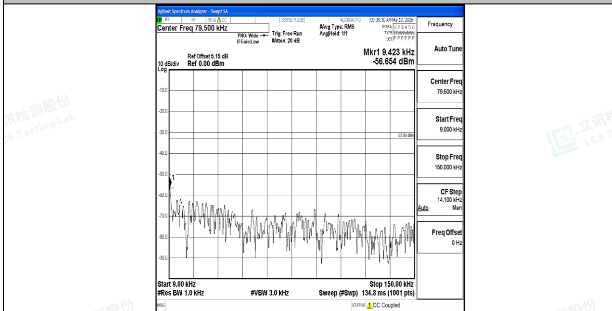
Band26_5MHz_QPSK_26740_1RB#0_0.009~0.15_0.009~0.15
