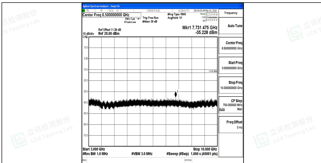
Band26_3MHz_16QAM_26705_1RB#0_3000~10000_3000~10000
