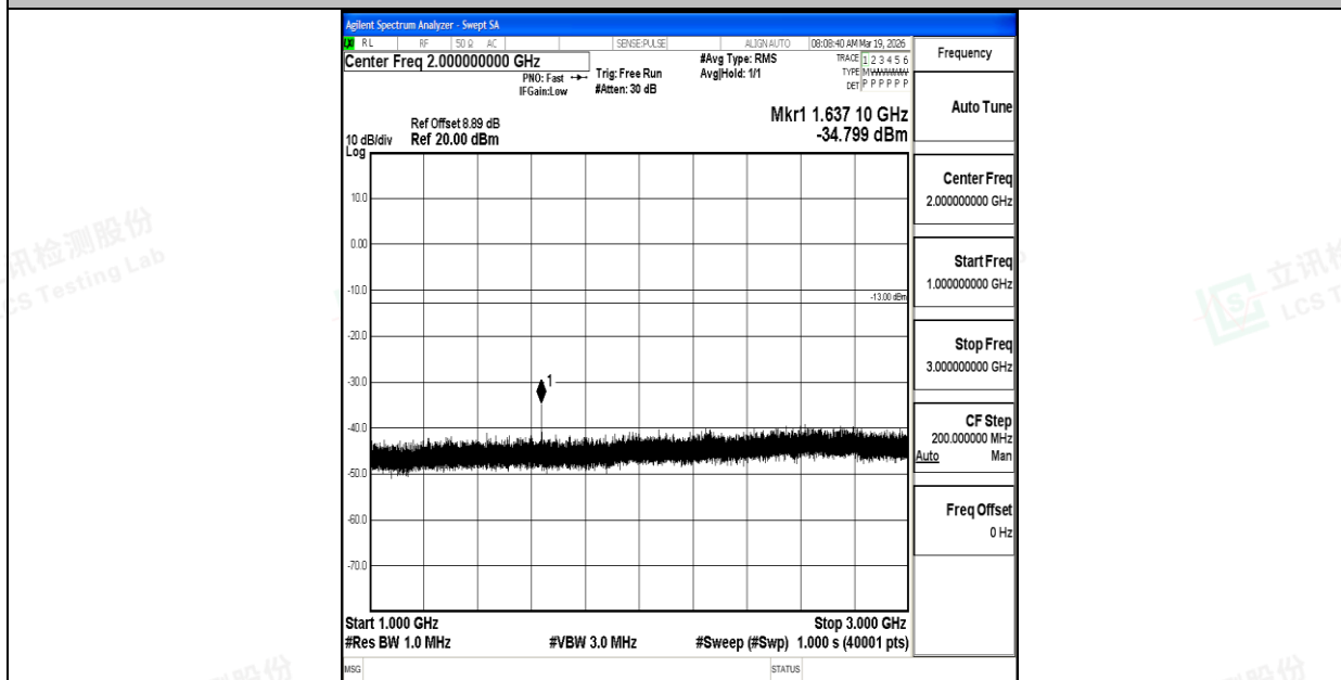
Band26_1.4MHz_16QAM_26740_1RB#0_1000~3000_1000~3000
