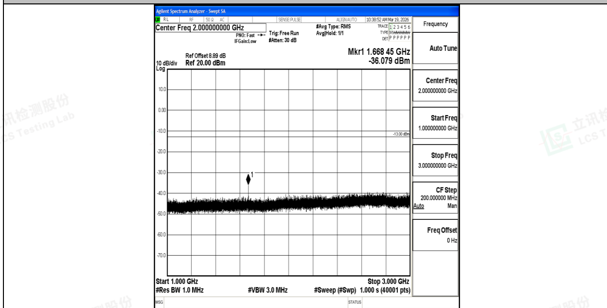
Band26_5MHz_QPSK_26915_1RB#0_1000~3000_1000~3000
