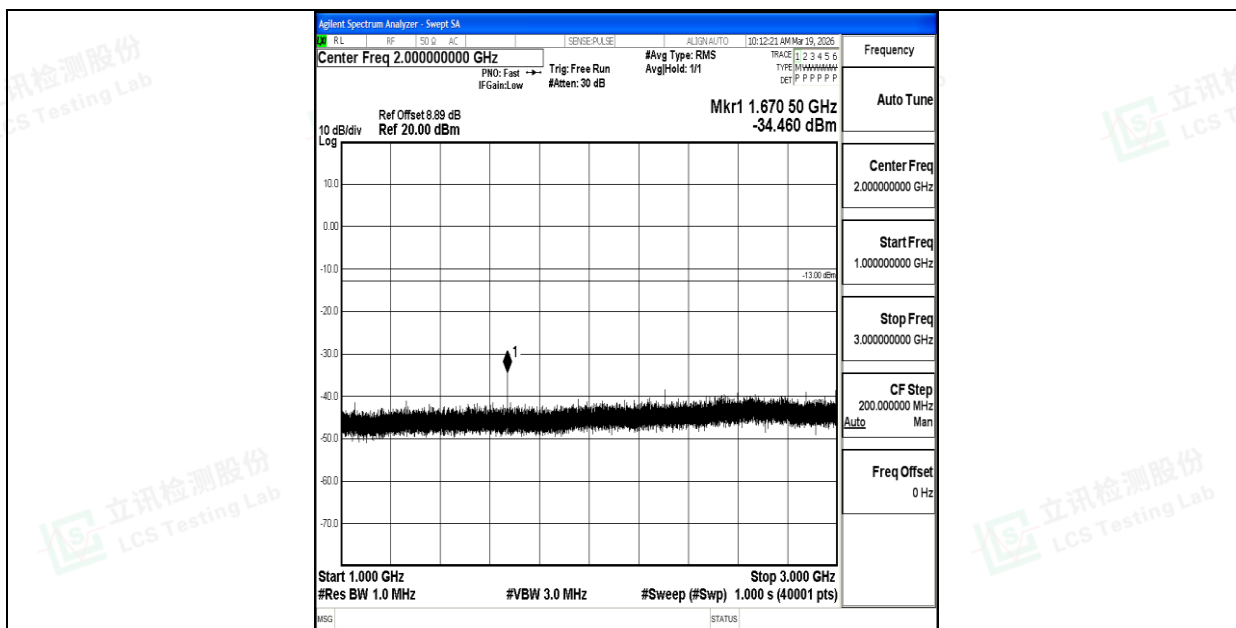
Band26_3MHz_16QAM_26915_1RB#0_1000~3000_1000~3000
