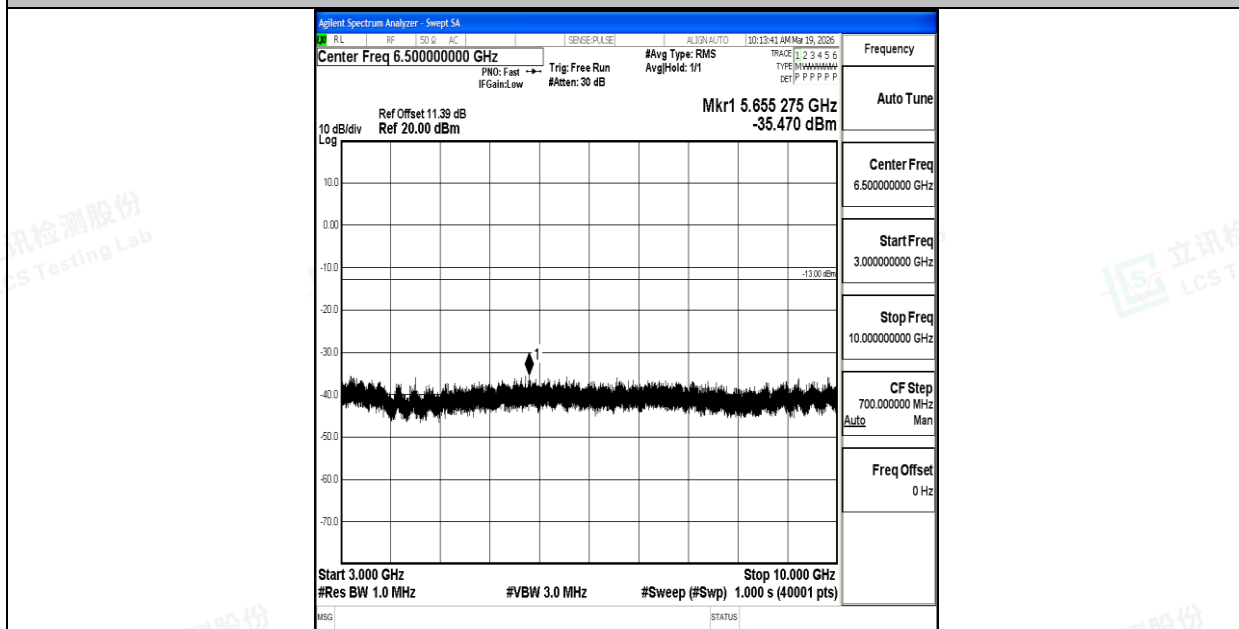
Band26_3MHz_16QAM_27025_1RB#0_3000~10000_3000~10000
