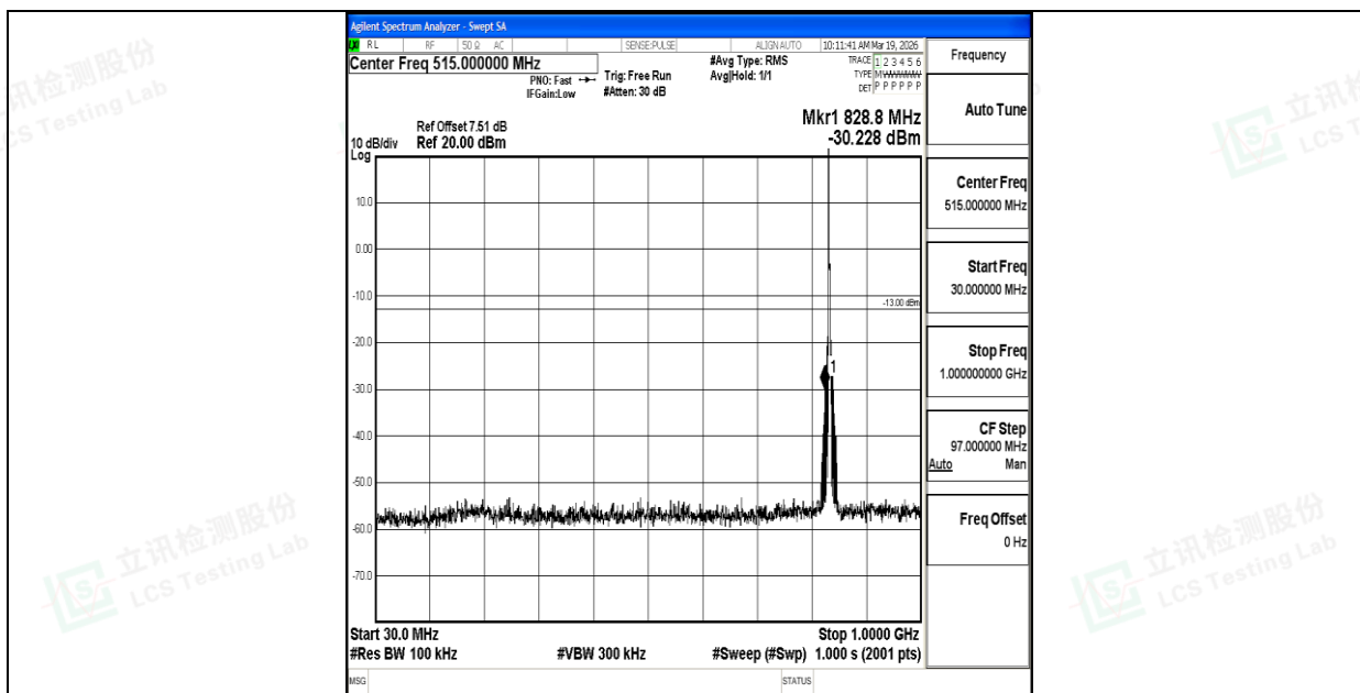
Band26_3MHz_QPSK_26915_1RB#0_30~1000_30~1000
