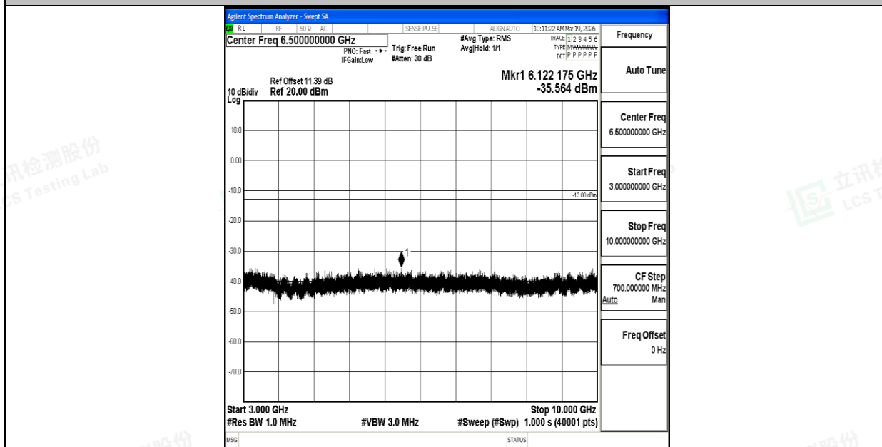
Band26_3MHz_16QAM_26805_1RB#0_3000~10000_3000~10000
