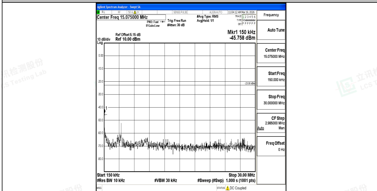
Band26_10MHz_QPSK_26915_1RB#0_0.15~30_0.15~30
