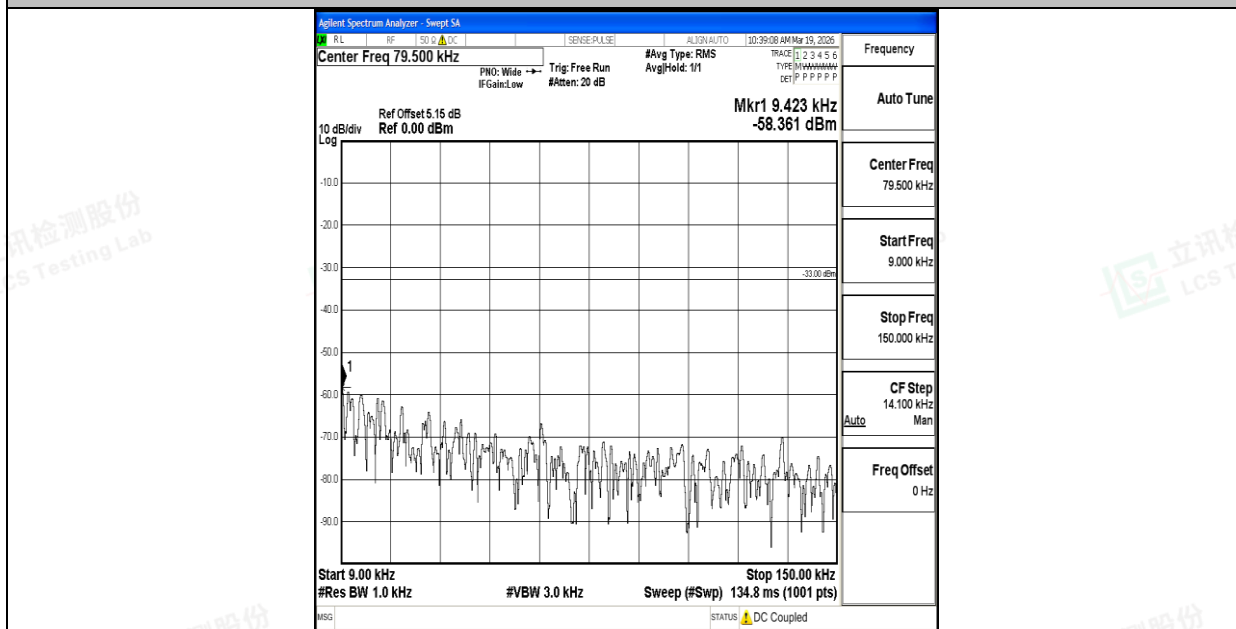
Band26_5MHz_16QAM_26915_1RB#0_0.009~0.15_0.009~0.15
