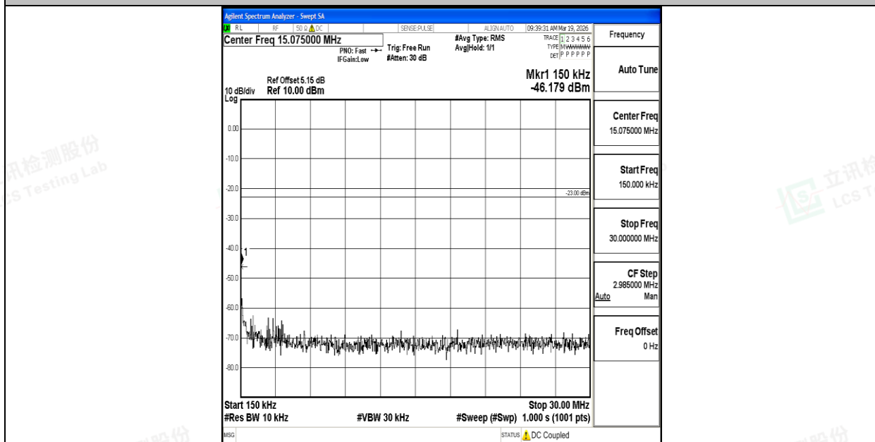
Band26_1.4MHz_QPSK_27033_1RB#0_0.15~30_0.15~30
