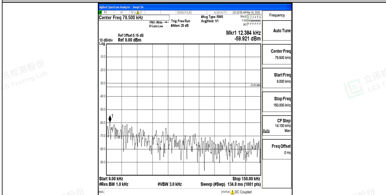
Band26_3MHz_16QAM_26805_1RB#0_0.009~0.15_0.009~0.15
