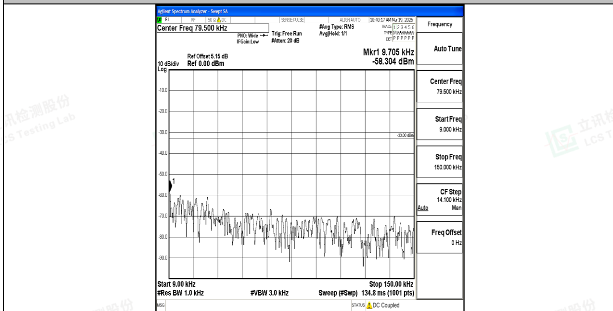
Band26_5MHz_16QAM_27015_1RB#0_0.009~0.15_0.009~0.15
