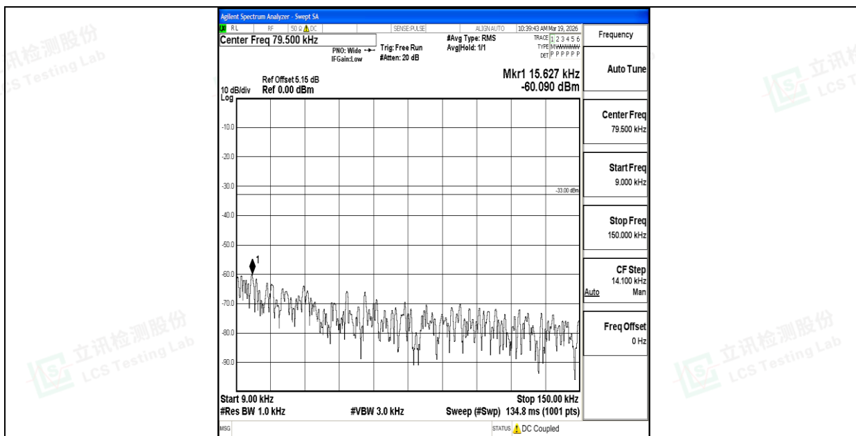
Band26_5MHz_QPSK_27015_1RB#0_0.009~0.15_0.009~0.15
