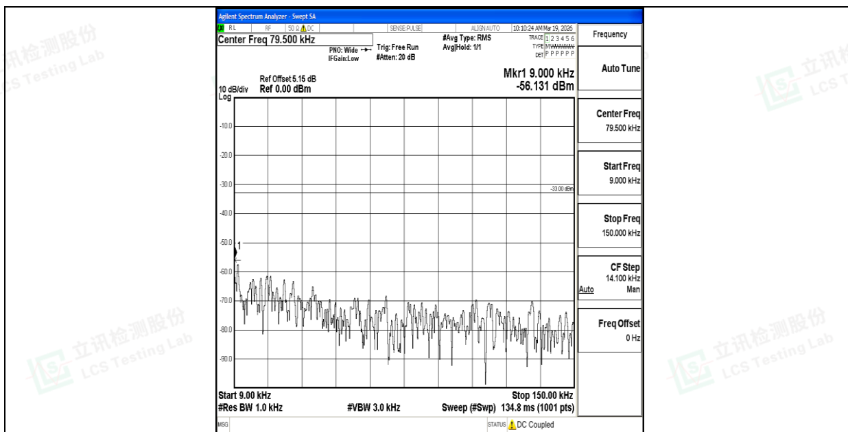
Band26_3MHz_QPSK_26805_1RB#0_0.009~0.15_0.009~0.15
