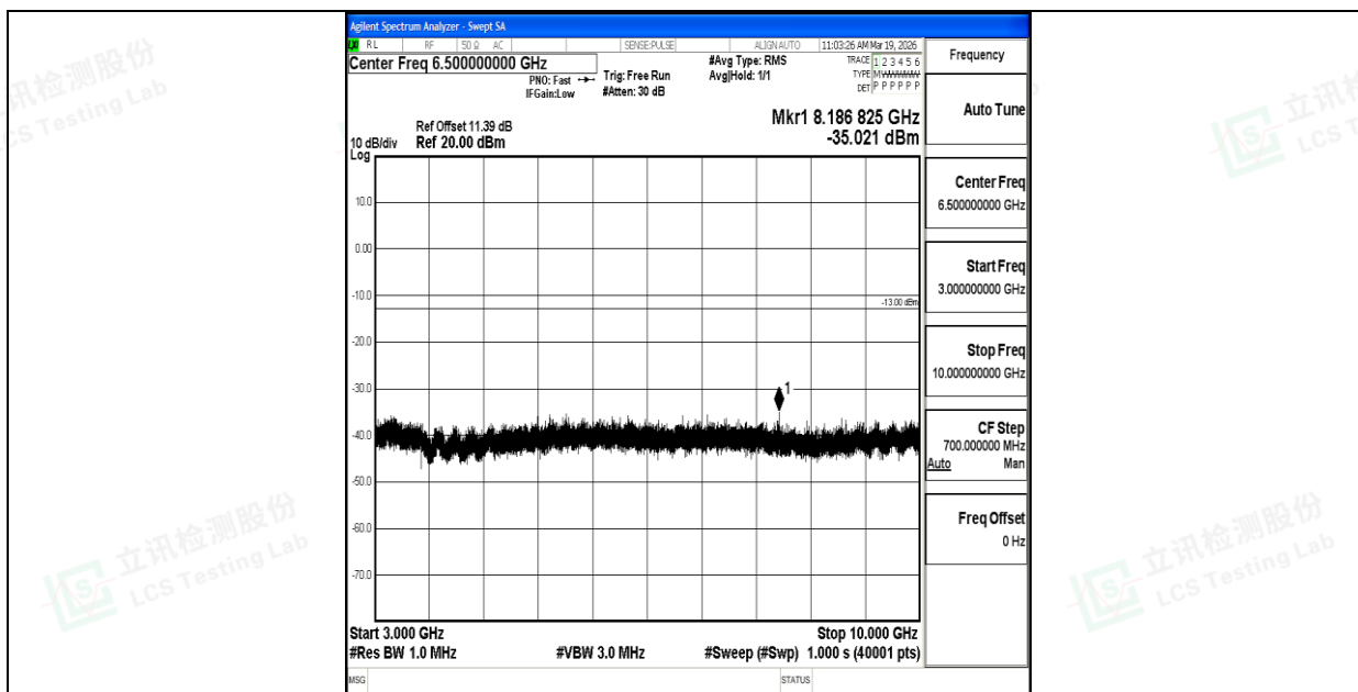
Band26_10MHz_QPSK_26840_1RB#0_3000~10000_3000~10000
