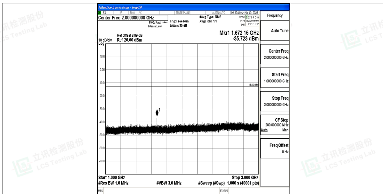
Band26_1.4MHz_16QAM_26915_1RB#0_1000~3000_1000~3000
