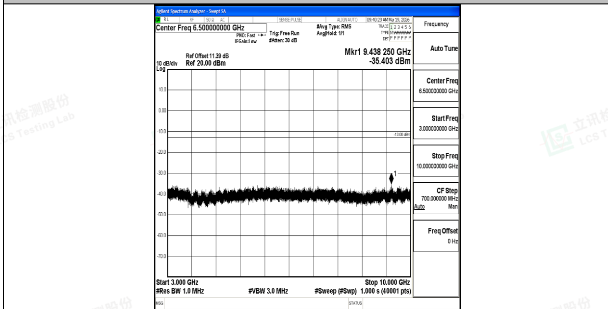
Band26_1.4MHz_16QAM_27033_1RB#0_3000~10000_3000~10000
