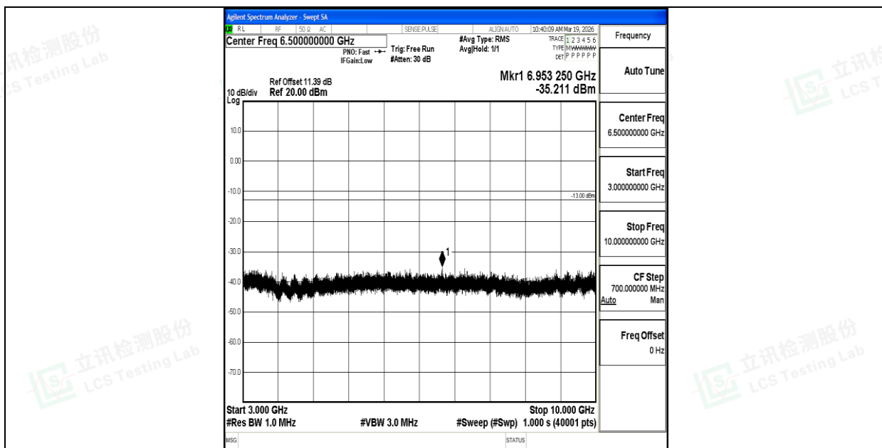
Band26_5MHz_QPSK_27015_1RB#0_3000~10000_3000~10000
