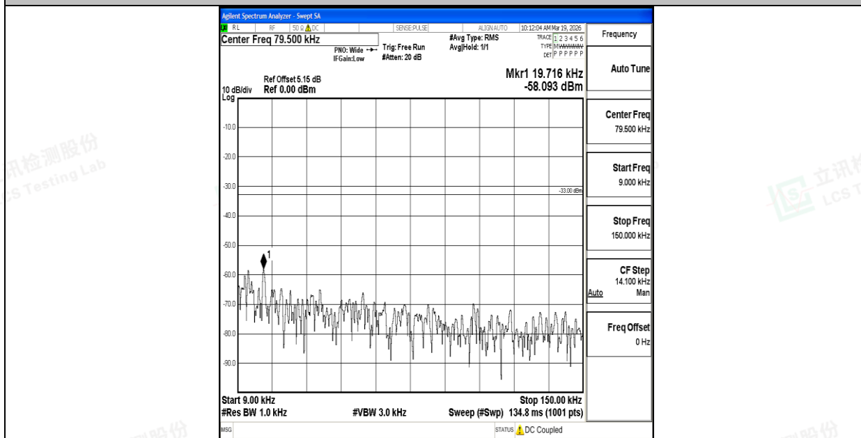
Band26_3MHz_16QAM_26915_1RB#0_0.009~0.15_0.009~0.15
