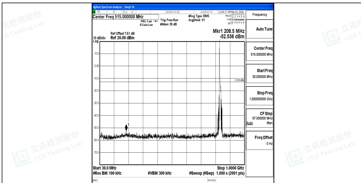
Band26_10MHz_QPSK_26915_1RB#0_30~1000_30~1000
