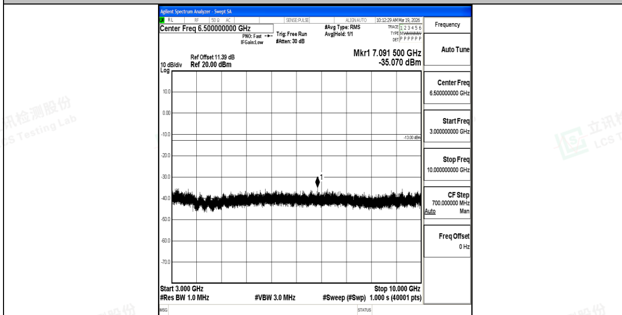
Band26_3MHz_16QAM_26915_1RB#0_3000~10000_3000~10000
