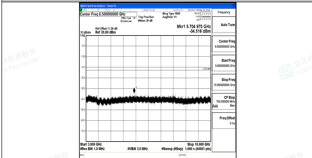
Band26_1.4MHz_16QAM_26915_1RB#0_3000~10000_3000~10000
