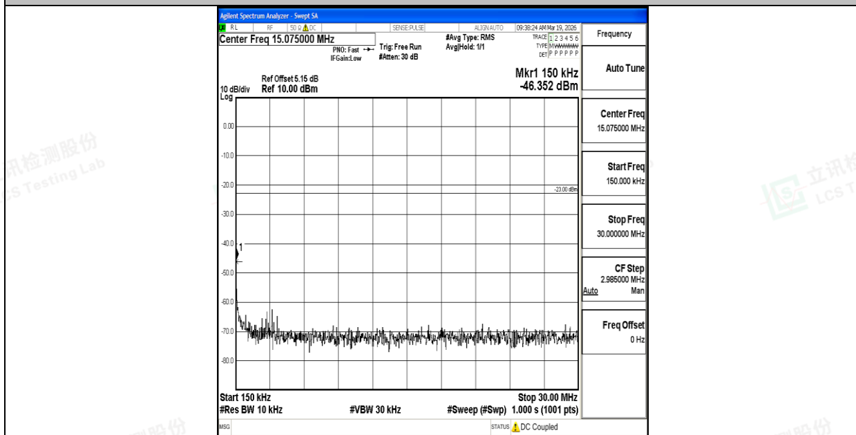
Band26_1.4MHz_QPSK_26915_1RB#0_0.15~30_0.15~30
