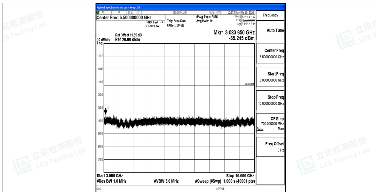
Band26_5MHz_QPSK_26815_1RB#0_3000~10000_3000~10000
