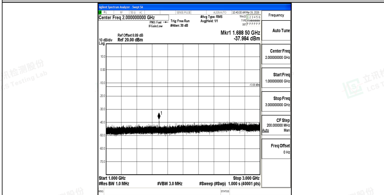
Band26_5MHz_QPSK_27015_1RB#0_1000~3000_1000~3000
