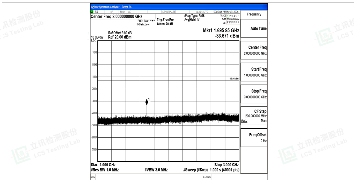
Band26_1.4MHz_16QAM_27033_1RB#0_1000~3000_1000~3000
