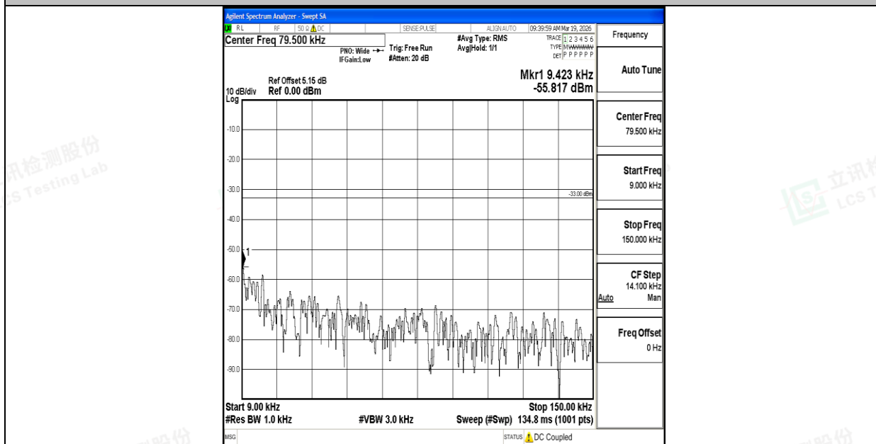
Band26_1.4MHz_16QAM_27033_1RB#0_0.009~0.15_0.009~0.15
