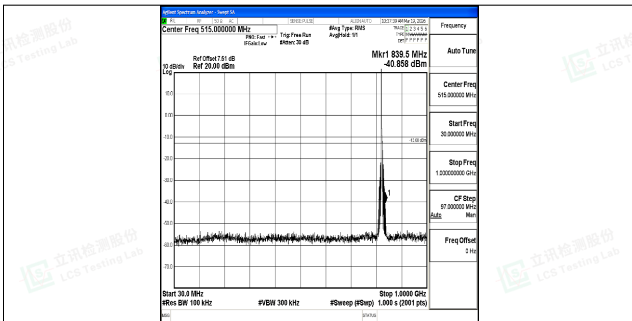
Band26_5MHz_QPSK_26815_1RB#0_30~1000_30~1000
