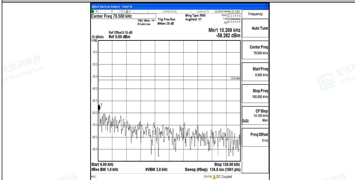
Band26_5MHz_16QAM_26815_1RB#0_0.009~0.15_0.009~0.15
