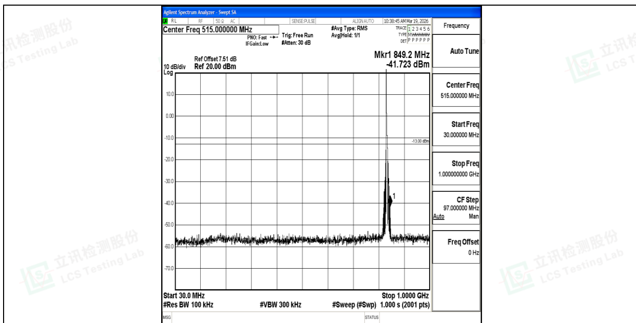
Band26_5MHz_QPSK_26915_1RB#0_30~1000_30~1000
