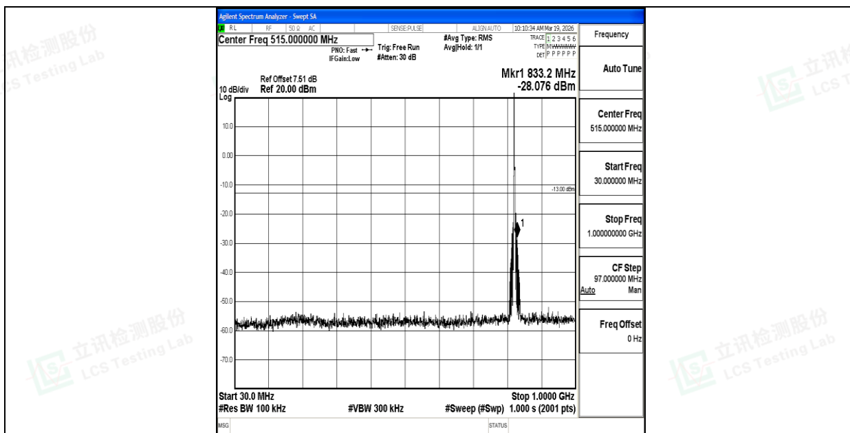
Band26_3MHz_QPSK_26805_1RB#0_30~1000_30~1000
