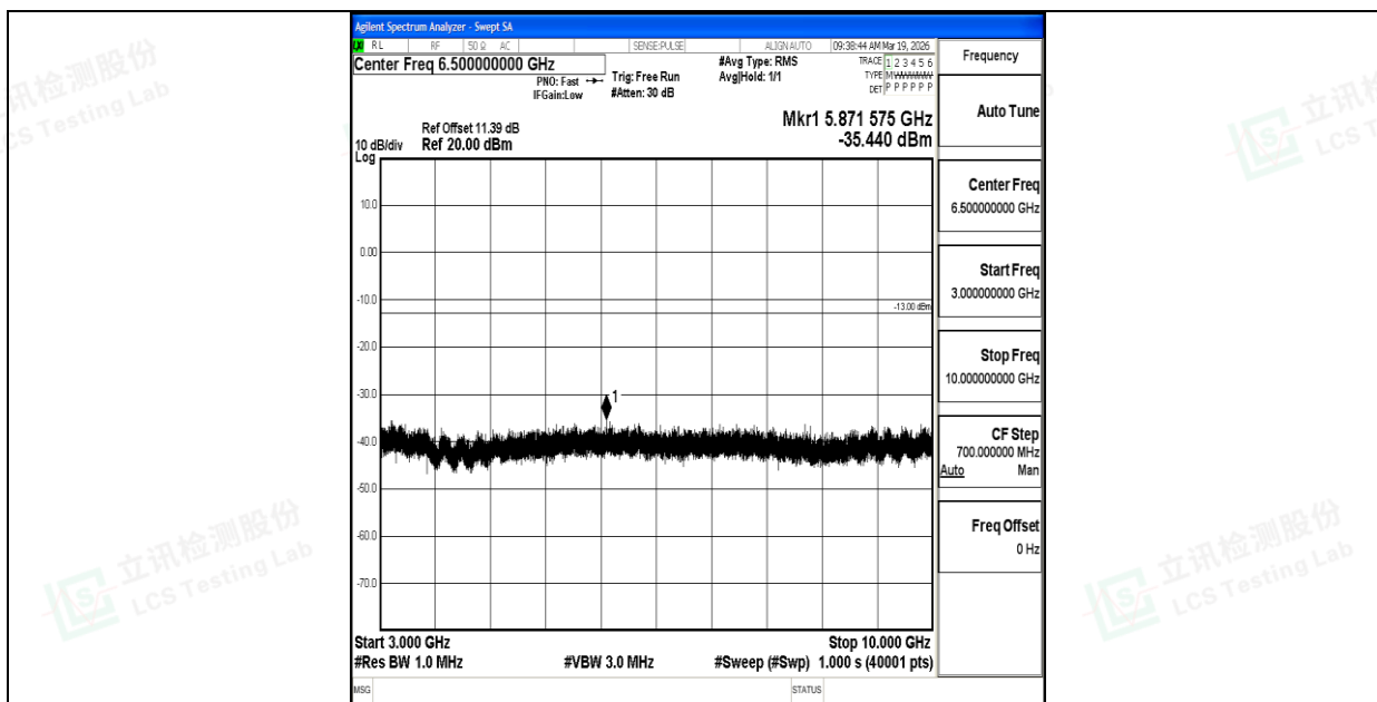
Band26_1.4MHz_QPSK_26915_1RB#0_3000~10000_3000~10000
