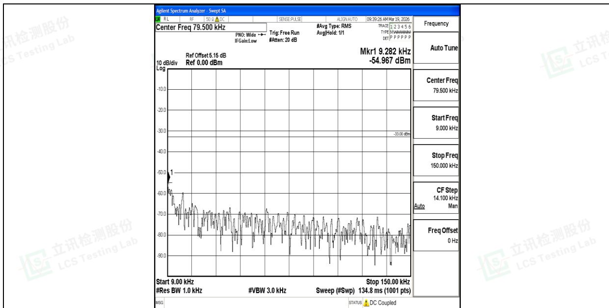
Band26_1.4MHz_QPSK_27033_1RB#0_0.009~0.15_0.009~0.15
