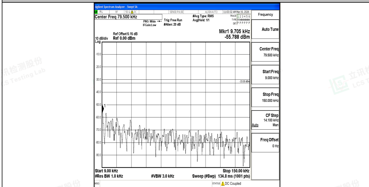
Band26_10MHz_16QAM_26840_1RB#0_0.009~0.15_0.009~0.15
