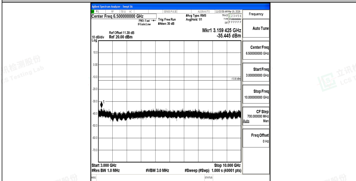
Band26_10MHz_16QAM_26840_1RB#0_3000~10000_3000~10000
