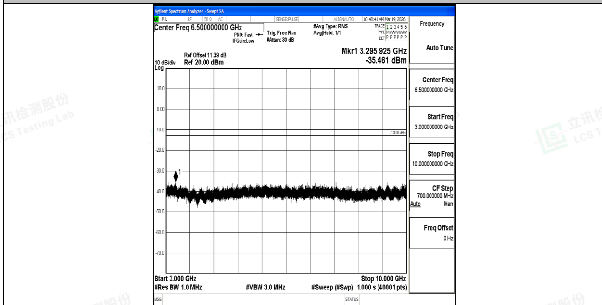
Band26_5MHz_16QAM_27015_1RB#0_3000~10000_3000~10000
