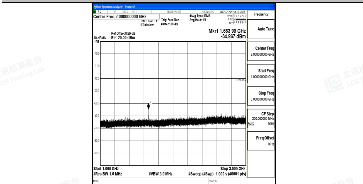
Band26_10MHz_QPSK_26915_1RB#0_1000~3000_1000~3000
