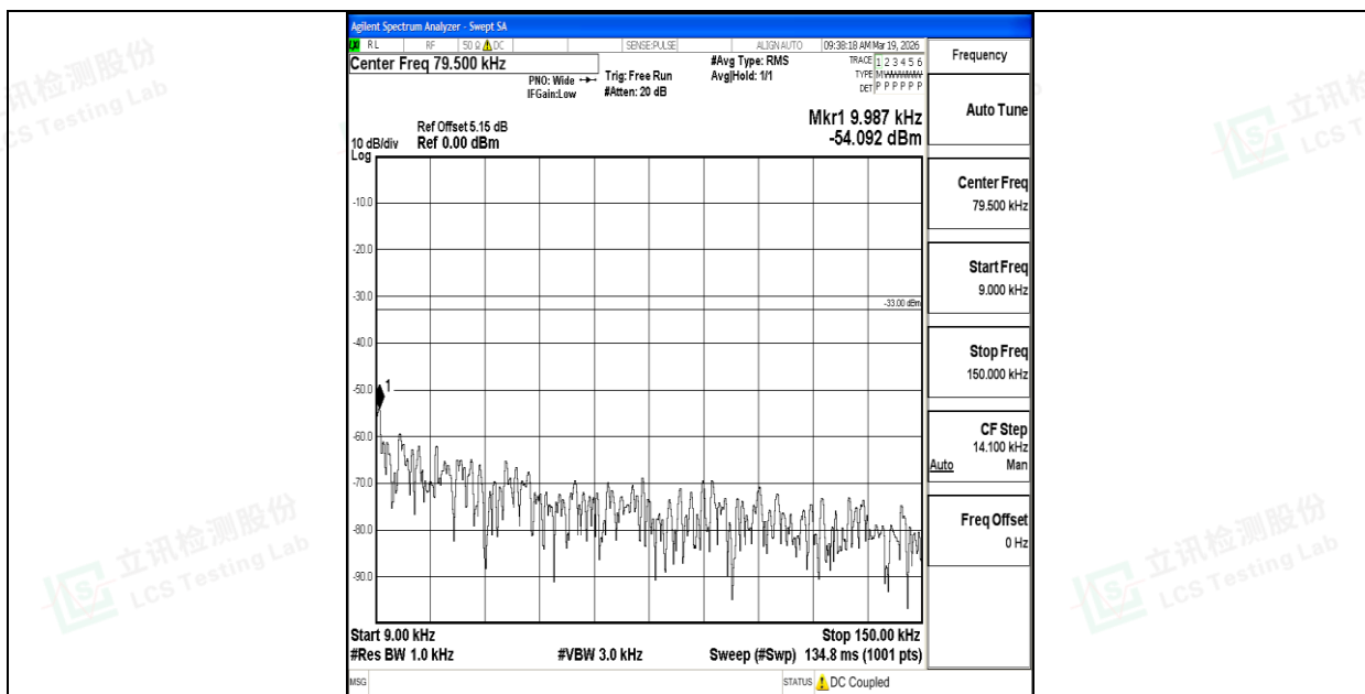
Band26_1.4MHz_QPSK_26915_1RB#0_0.009~0.15_0.009~0.15
