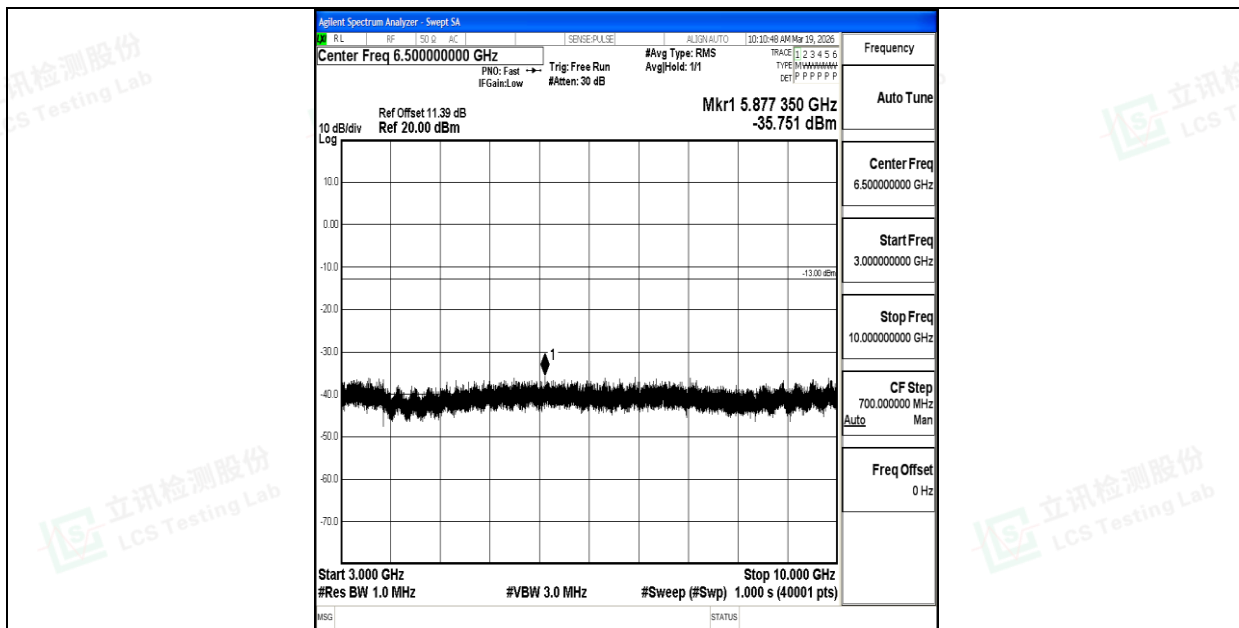
Band26_3MHz_QPSK_26805_1RB#0_3000~10000_3000~10000
