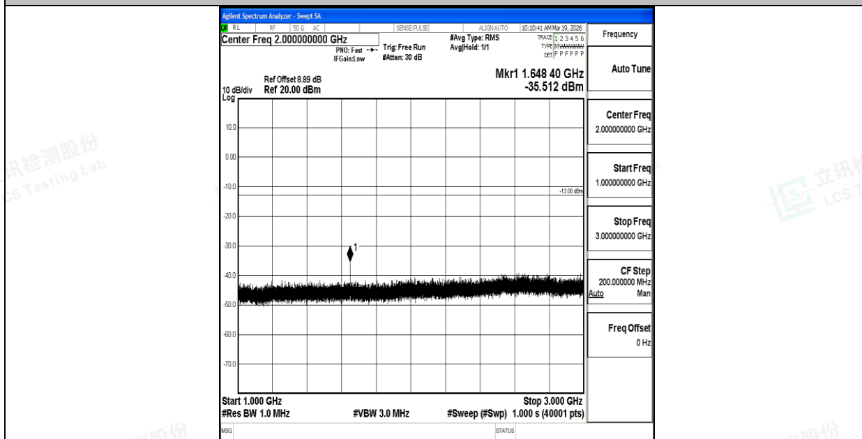
Band26_3MHz_QPSK_26805_1RB#0_1000~3000_1000~3000
