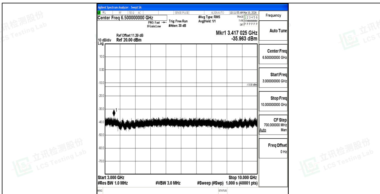
Band26_3MHz_QPSK_26915_1RB#0_3000~10000_3000~10000
