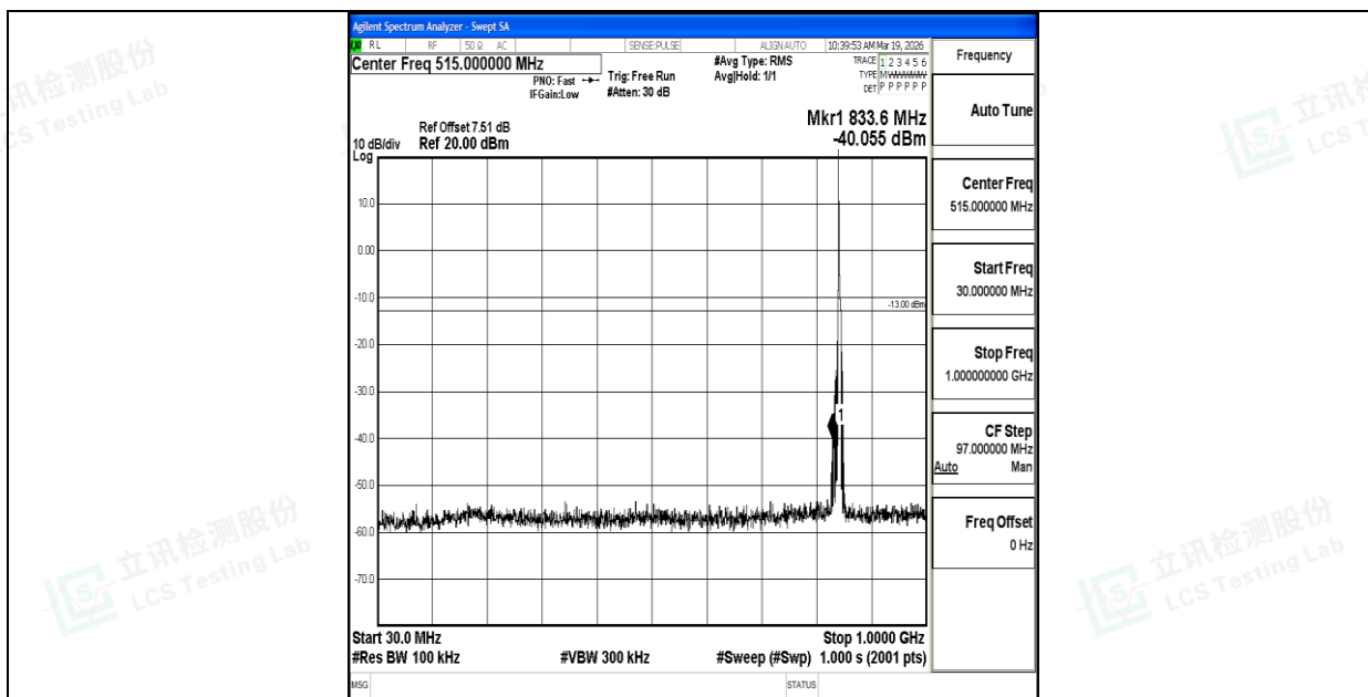
Band26_5MHz_QPSK_27015_1RB#0_30~1000_30~1000
