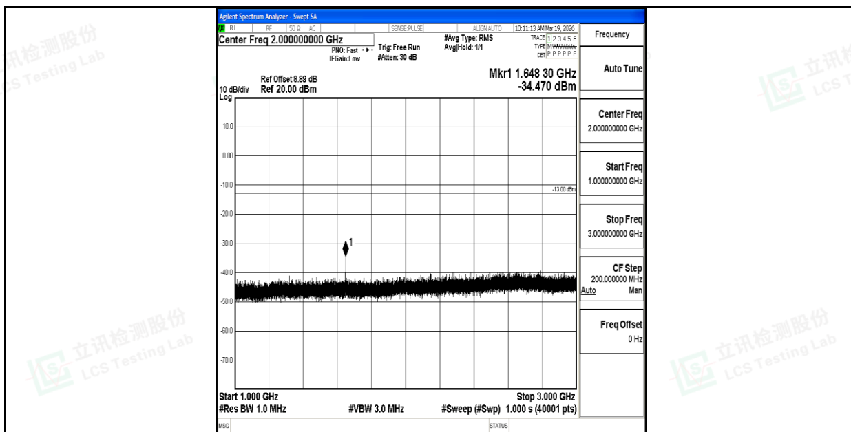
Band26_3MHz_16QAM_26805_1RB#0_1000~3000_1000~3000
