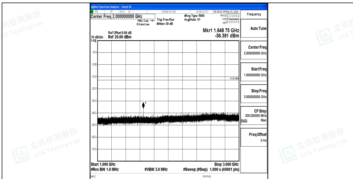
Band26_1.4MHz_16QAM_26797_1RB#0_1000~3000_1000~3000
