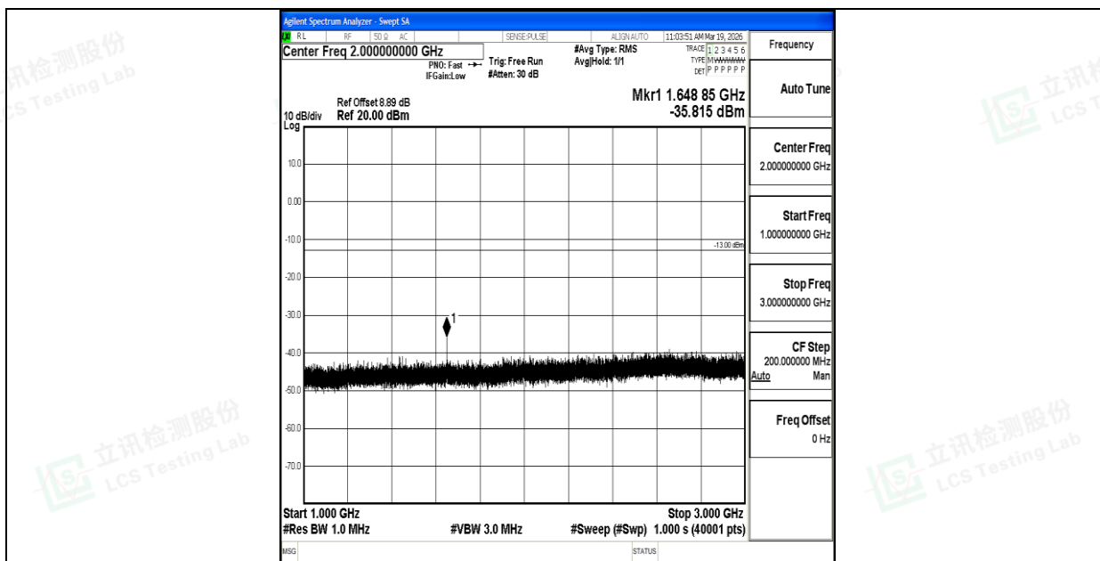
Band26_10MHz_16QAM_26840_1RB#0_1000~3000_1000~3000
