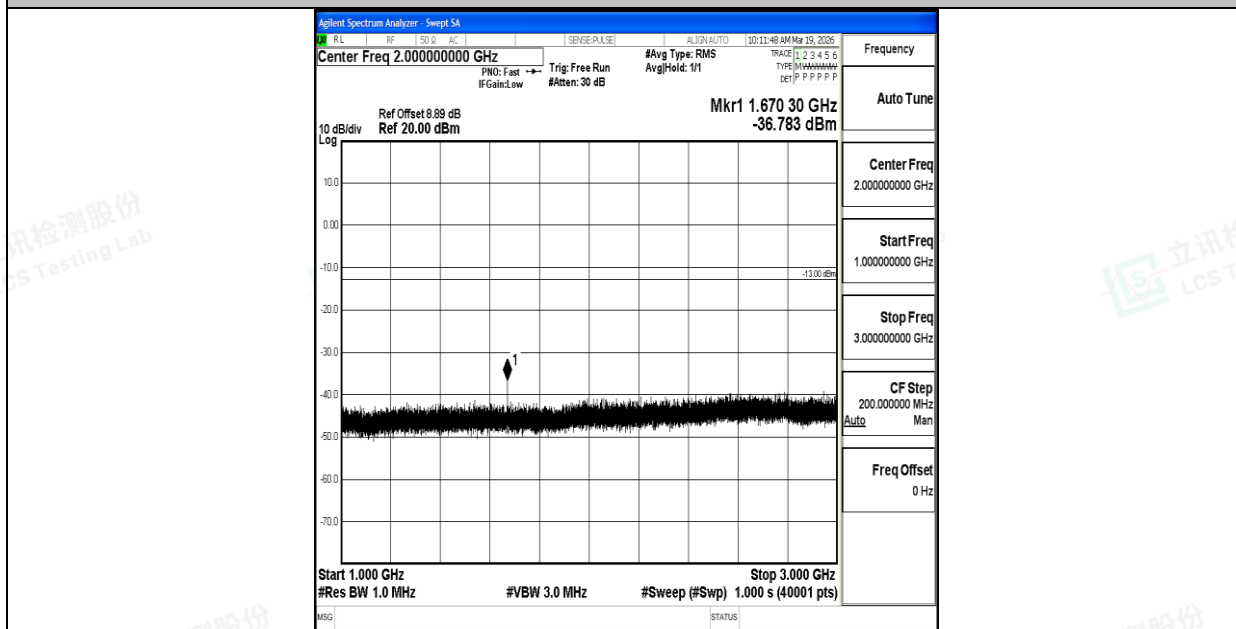
Band26_3MHz_QPSK_26915_1RB#0_1000~3000_1000~3000
