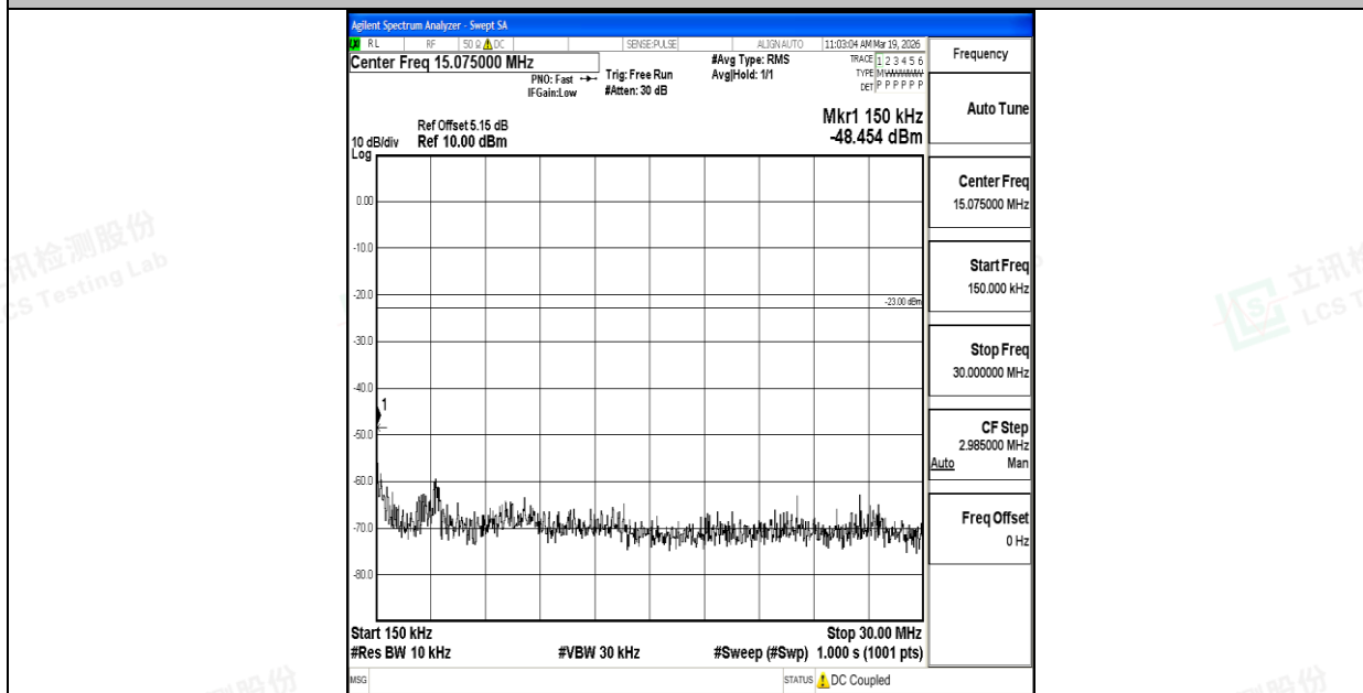
Band26_10MHz_QPSK_26840_1RB#0_0.15~30_0.15~30
