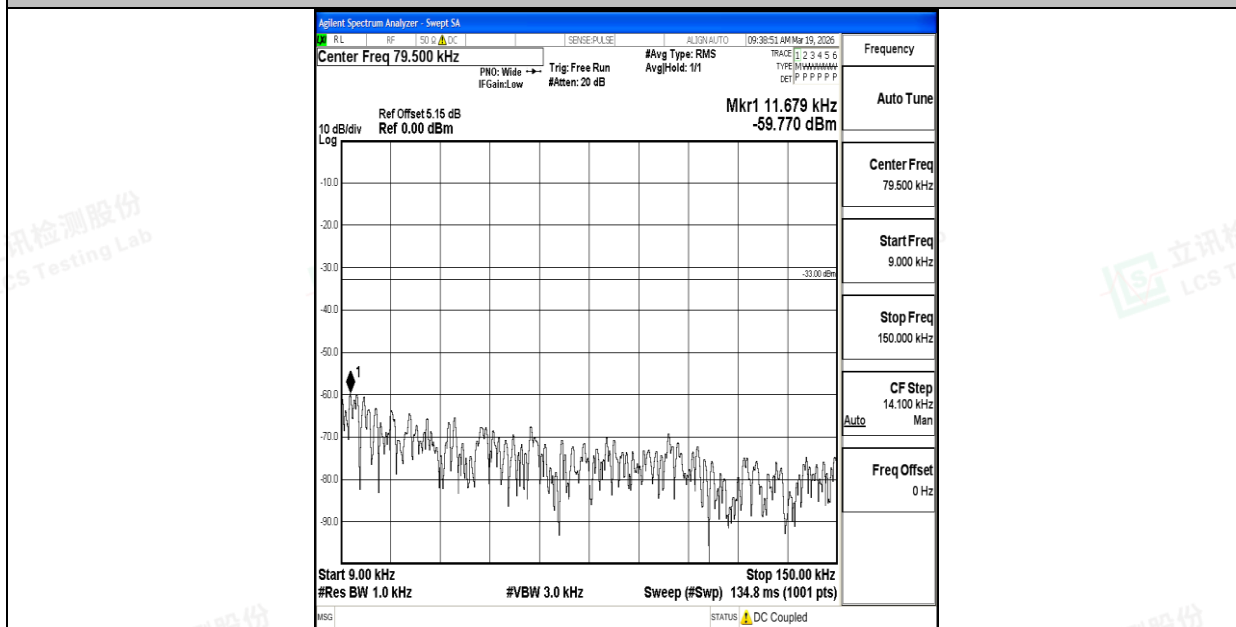
Band26_1.4MHz_16QAM_26915_1RB#0_0.009~0.15_0.009~0.15
