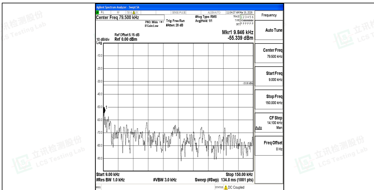
Band26_10MHz_QPSK_26915_1RB#0_0.009~0.15_0.009~0.15
