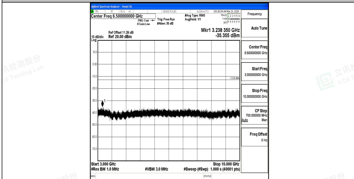
Band26_1.4MHz_16QAM_26797_1RB#0_3000~10000_3000~10000
