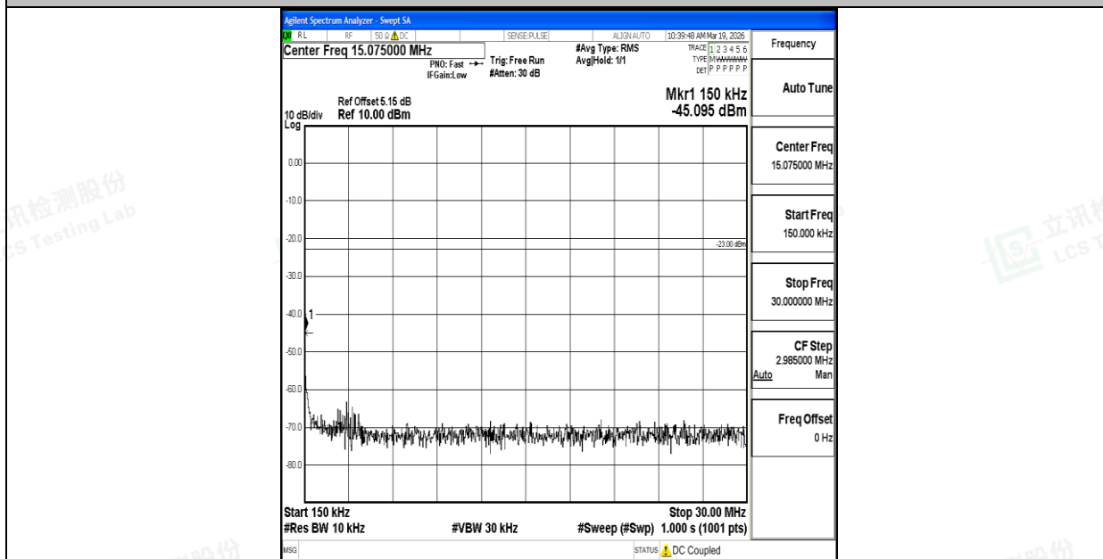
Band26_5MHz_QPSK_27015_1RB#0_0.15~30_0.15~30
