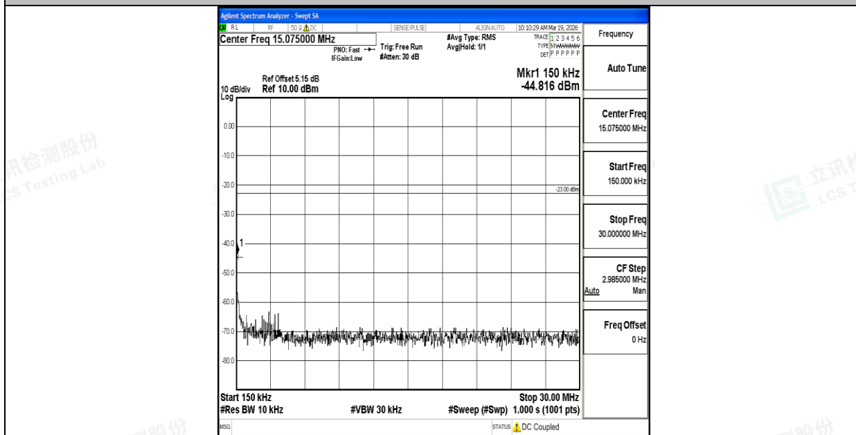
Band26_3MHz_QPSK_26805_1RB#0_0.15~30_0.15~30
