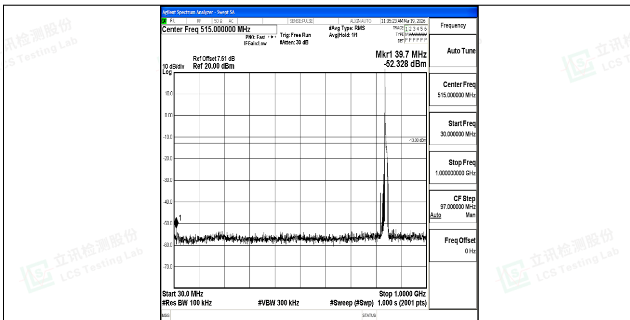
Band26_10MHz_QPSK_26990_1RB#0_30~1000_30~1000
