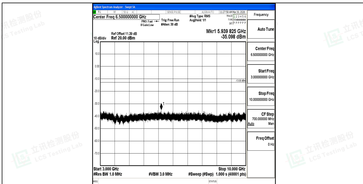
Band26_15MHz_QPSK_26915_1RB#0_3000~10000_3000~10000
