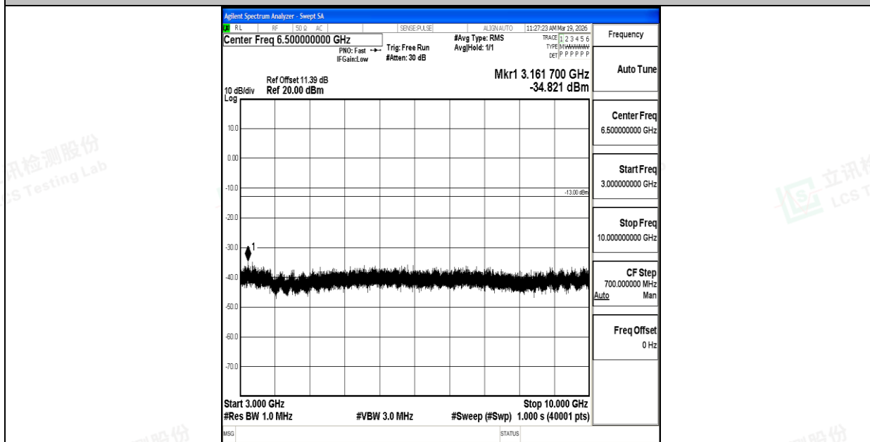
Band26_15MHz_16QAM_26865_1RB#0_3000~10000_3000~10000
