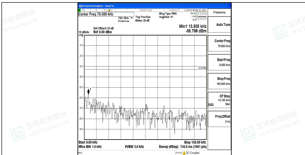
Band26_15MHz_QPSK_26965_1RB#0_0.009~0.15_0.009~0.15
