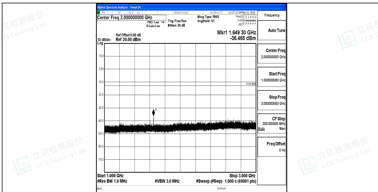
Band26_15MHz_16QAM_26865_1RB#0_1000~3000_1000~3000
