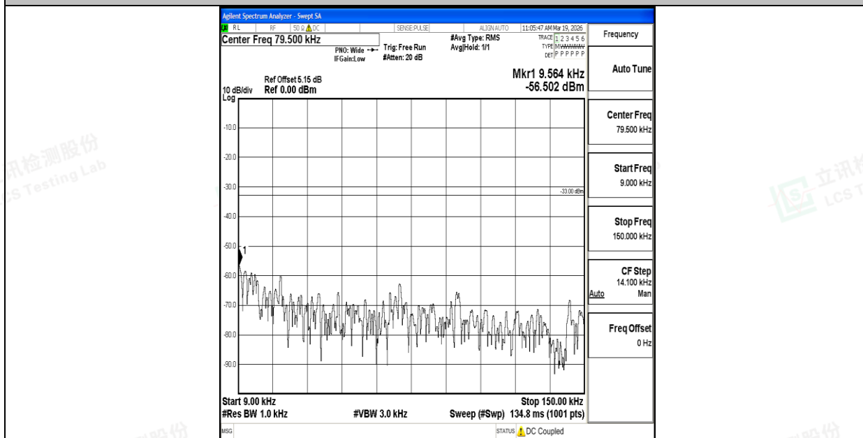
Band26_10MHz_16QAM_26990_1RB#0_0.009~0.15_0.009~0.15
