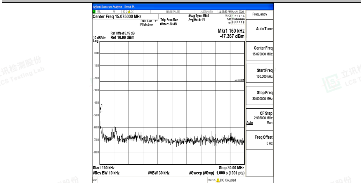
Band26_15MHz_QPSK_26965_1RB#0_0.15~30_0.15~30
