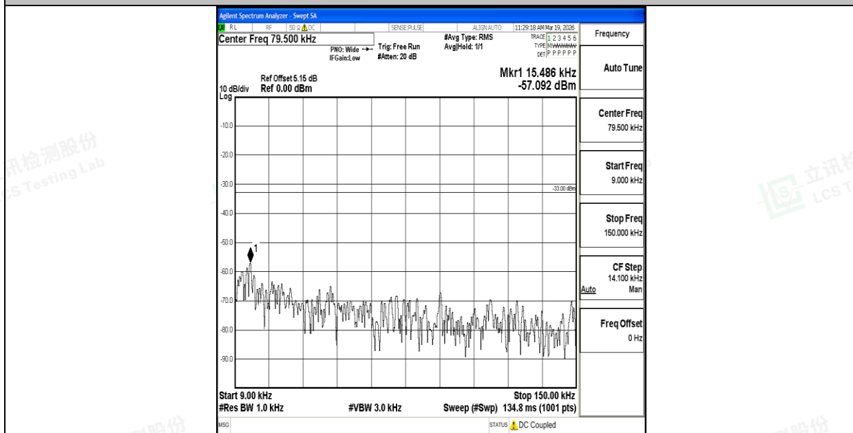
Band26_15MHz_16QAM_26965_1RB#0_0.009~0.15_0.009~0.15
