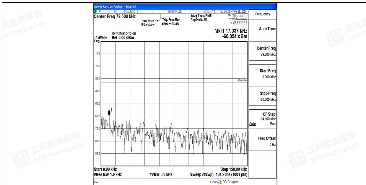
Band26_15MHz_QPSK_26865_1RB#0_0.009~0.15_0.009~0.15
