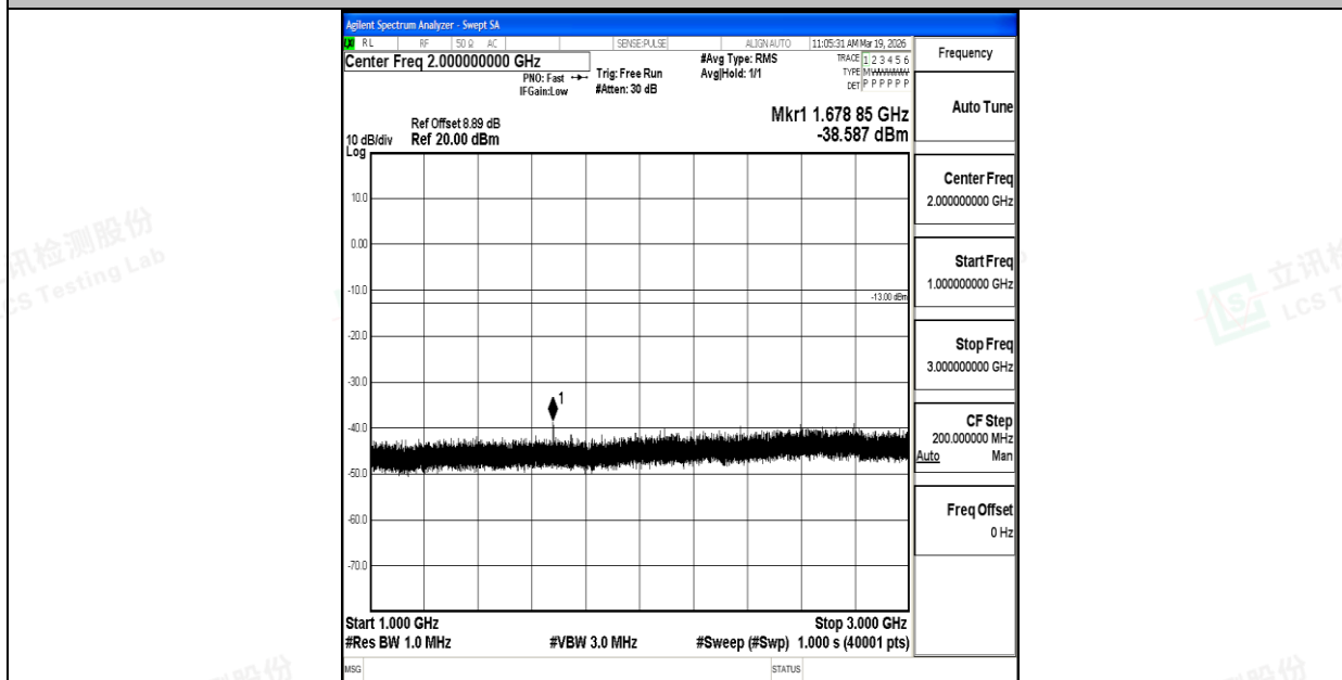
Band26_10MHz_QPSK_26990_1RB#0_1000~3000_1000~3000
