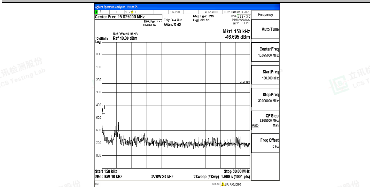
Band26_15MHz_QPSK_26865_1RB#0_0.15~30_0.15~30
