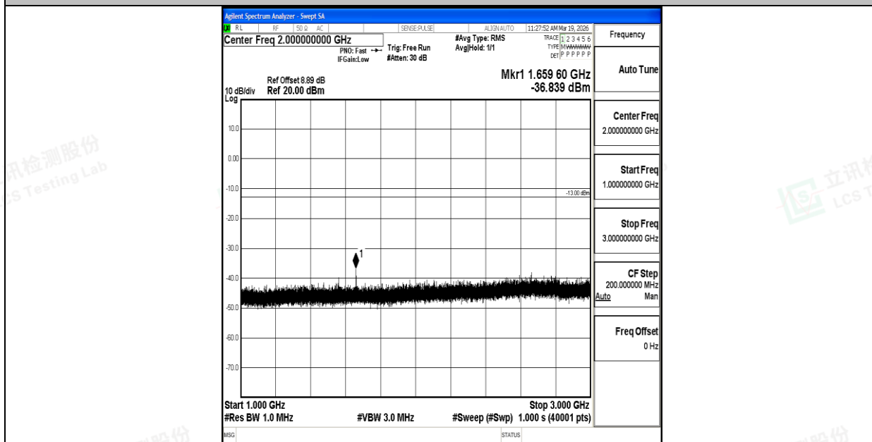
Band26_15MHz_QPSK_26915_1RB#0_1000~3000_1000~3000
