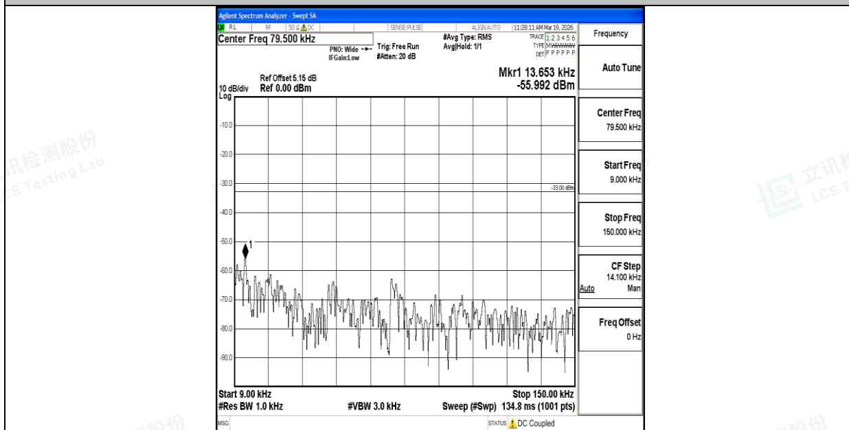
Band26_15MHz_16QAM_26915_1RB#0_0.009~0.15_0.009~0.15
