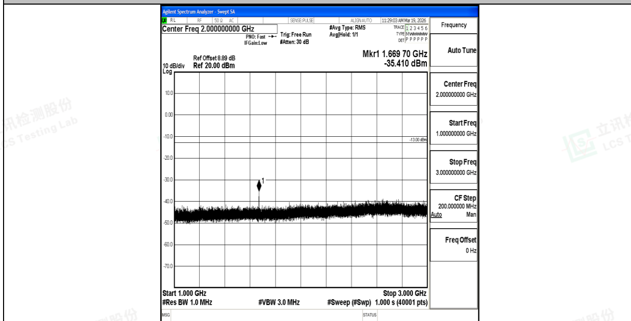
Band26_15MHz_QPSK_26965_1RB#0_1000~3000_1000~3000
