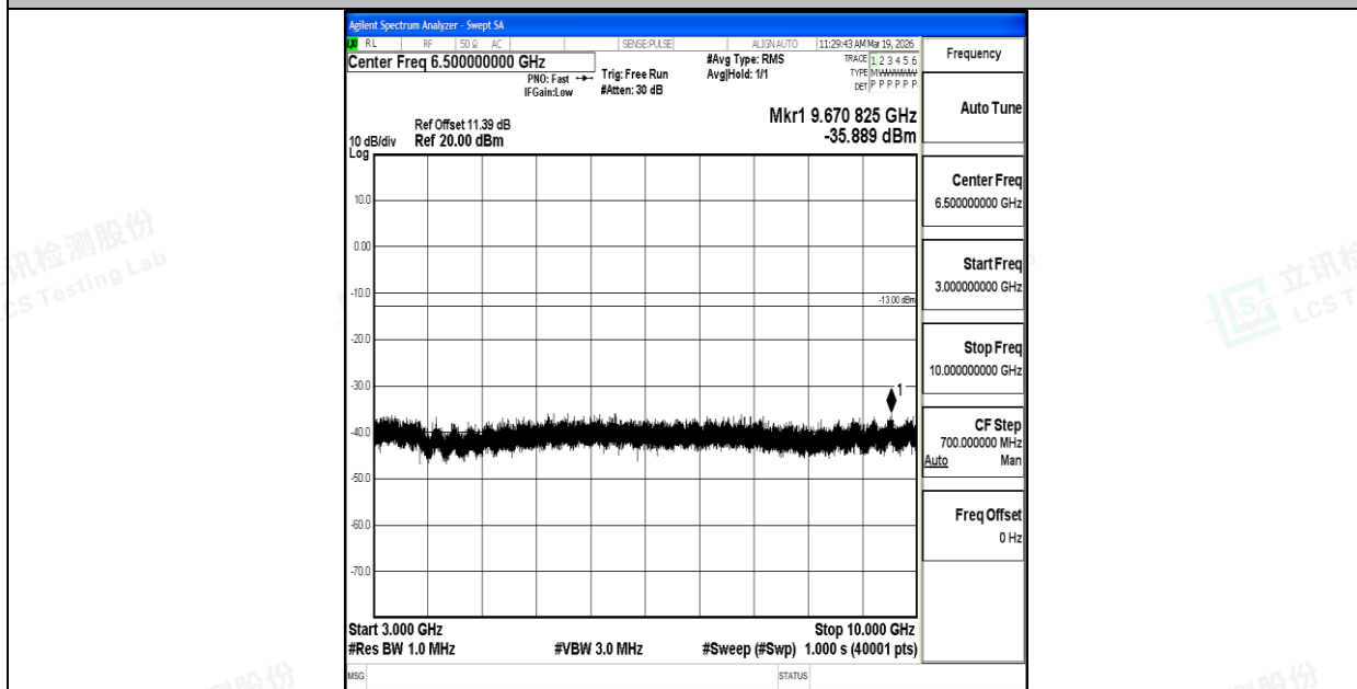
Band26_15MHz_16QAM_26965_1RB#0_3000~10000_3000~10000
