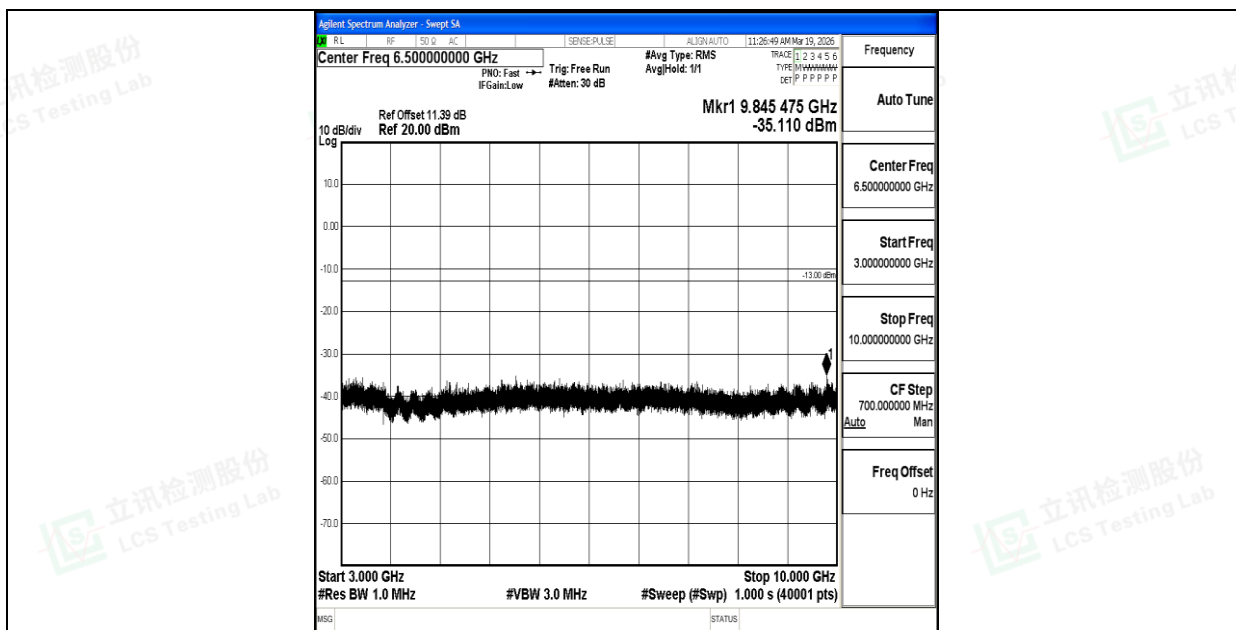
Band26_15MHz_QPSK_26865_1RB#0_3000~10000_3000~10000
