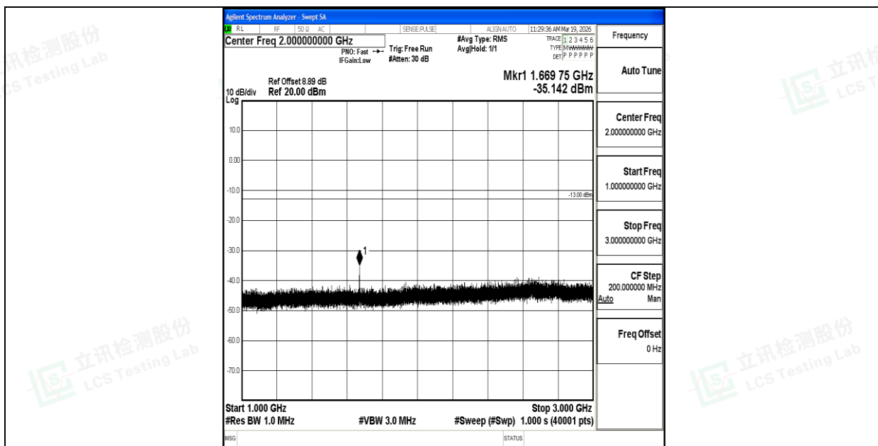
Band26_15MHz_16QAM_26965_1RB#0_1000~3000_1000~3000
