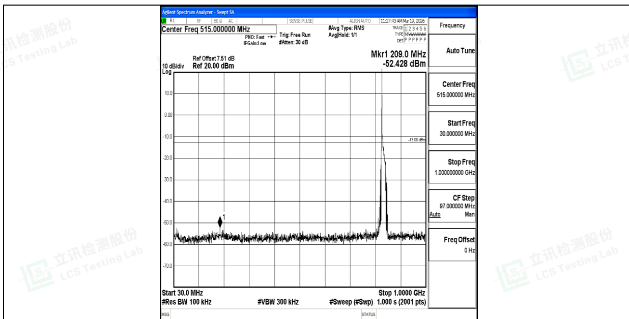
Band26_15MHz_QPSK_26915_1RB#0_30~1000_30~1000
