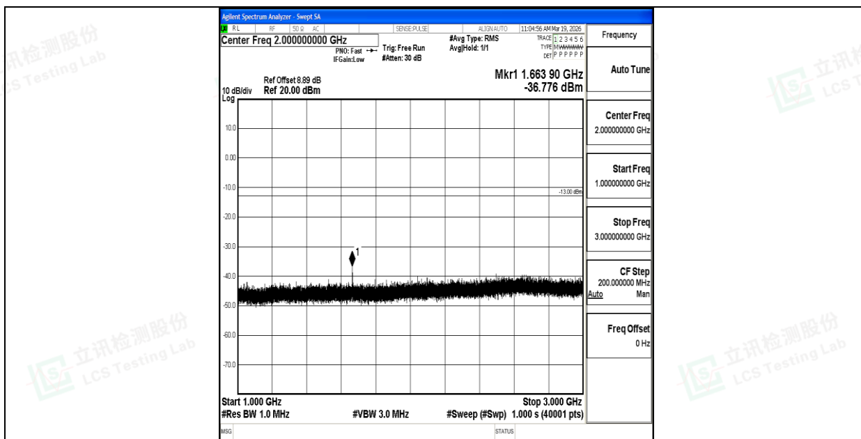
Band26_10MHz_16QAM_26915_1RB#0_1000~3000_1000~3000
