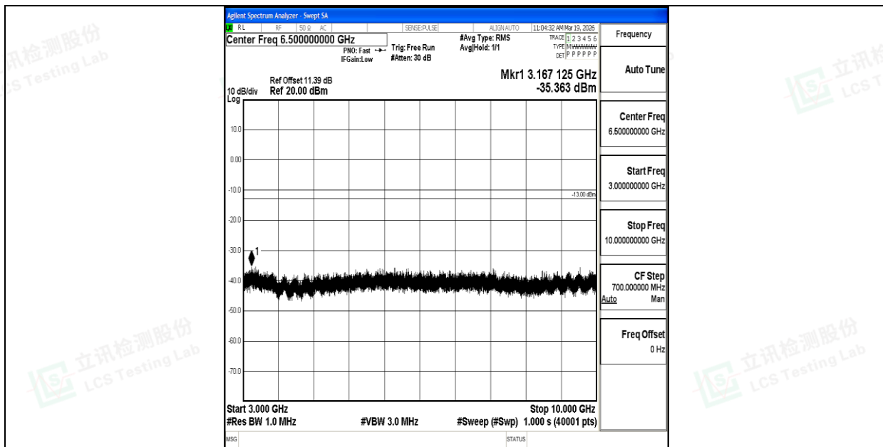
Band26_10MHz_QPSK_26915_1RB#0_3000~10000_3000~10000
