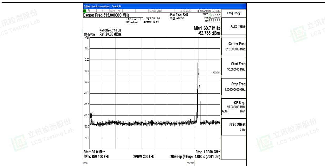
Band26_15MHz_QPSK_26965_1RB#0_30~1000_30~1000
