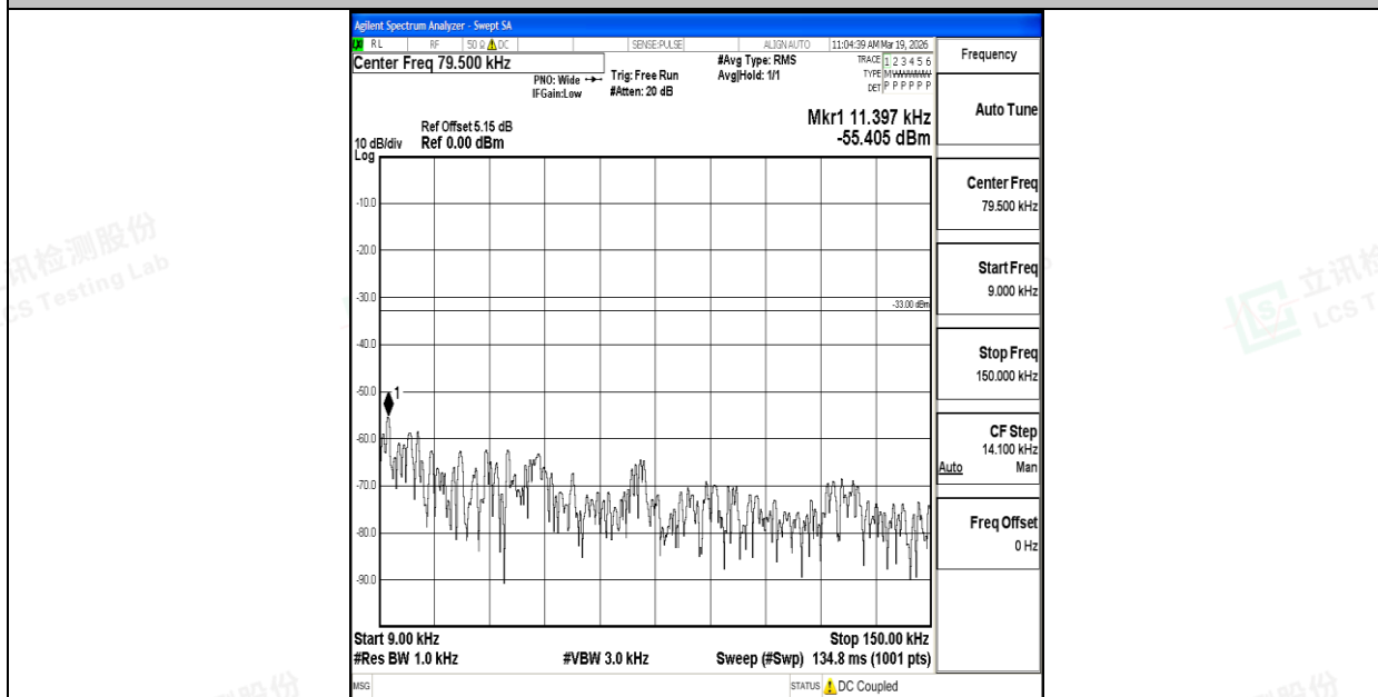
Band26_10MHz_16QAM_26915_1RB#0_0.009~0.15_0.009~0.15
