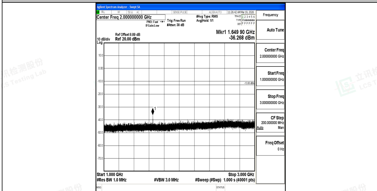
Band26_15MHz_QPSK_26865_1RB#0_1000~3000_1000~3000
