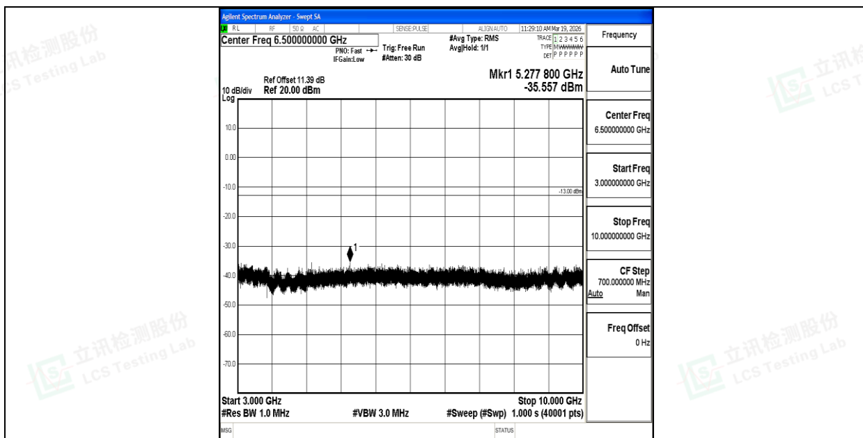
Band26_15MHz_QPSK_26965_1RB#0_3000~10000_3000~10000
