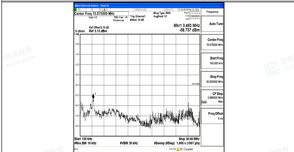
Band41_10MHz_QPSK_39700_1RB#0_0.15~30_0.15~30
