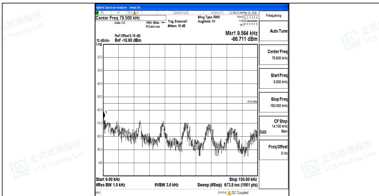
Band41_5MHz_QPSK_40620_1RB#0_0.009~0.15_0.009~0.15
