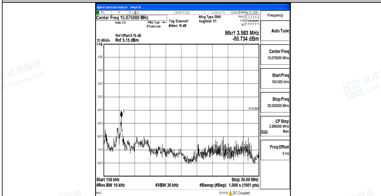
Band41_5MHz_QPSK_41565_1RB#0_0.15~30_0.15~30
