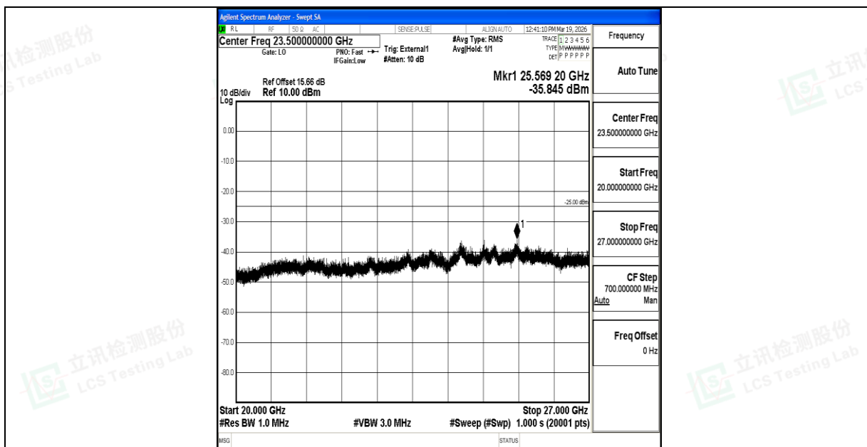
Band41_10MHz_QPSK_40620_1RB#0_20000~27000_20000~27000
