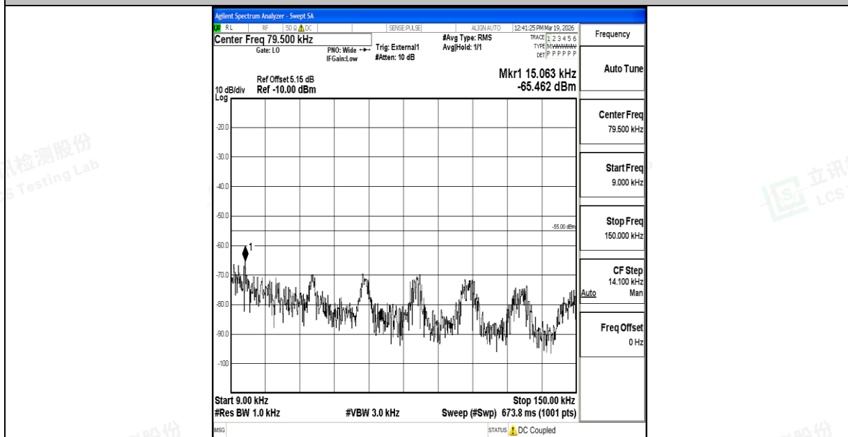
Band41_10MHz_16QAM_40620_1RB#0_0.009~0.15_0.009~0.15
