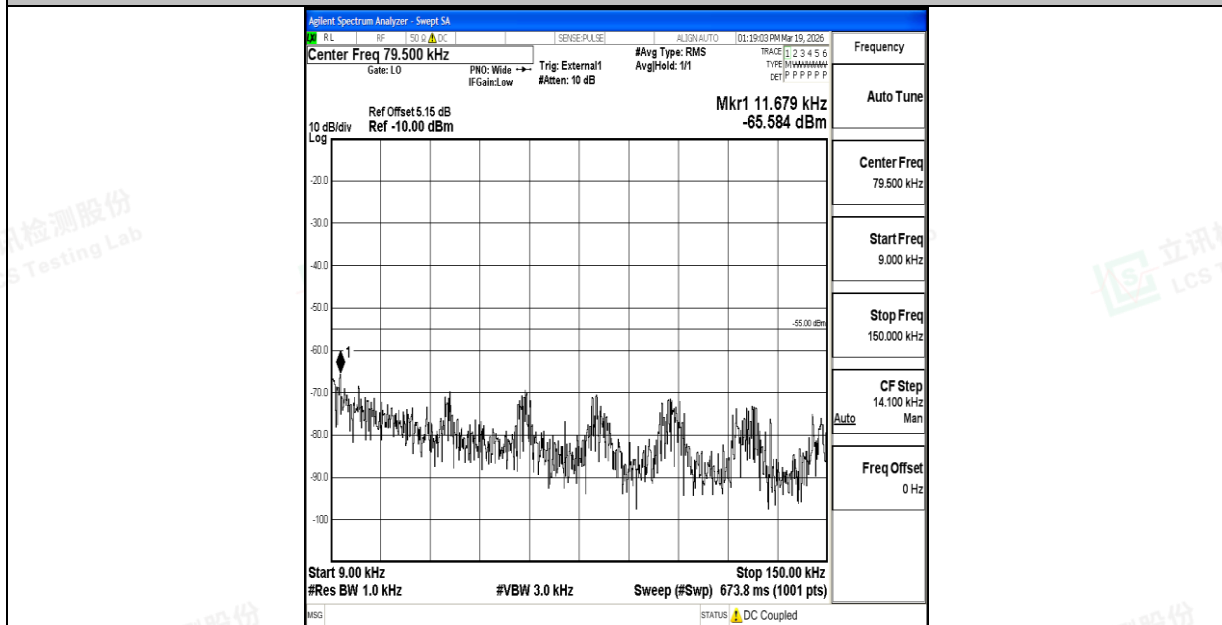
Band41_15MHz_16QAM_40620_1RB#0_0.009~0.15_0.009~0.15
