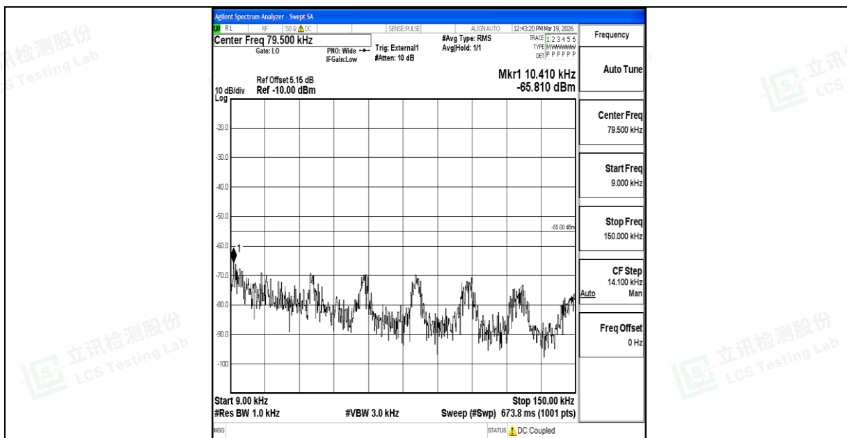
Band41_10MHz_QPSK_41540_1RB#0_0.009~0.15_0.009~0.15
