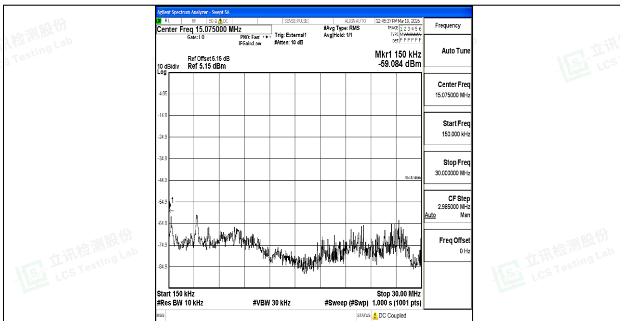
Band41_10MHz_16QAM_41540_1RB#0_0.15~30_0.15~30
