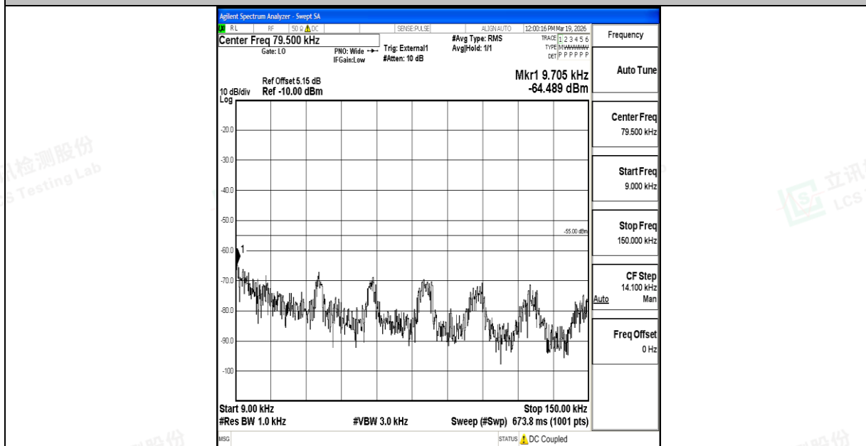
Band41_5MHz_16QAM_40620_1RB#0_0.009~0.15_0.009~0.15
