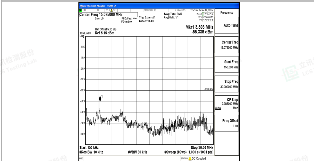
Band41_10MHz_QPSK_41540_1RB#0_0.15~30_0.15~30
