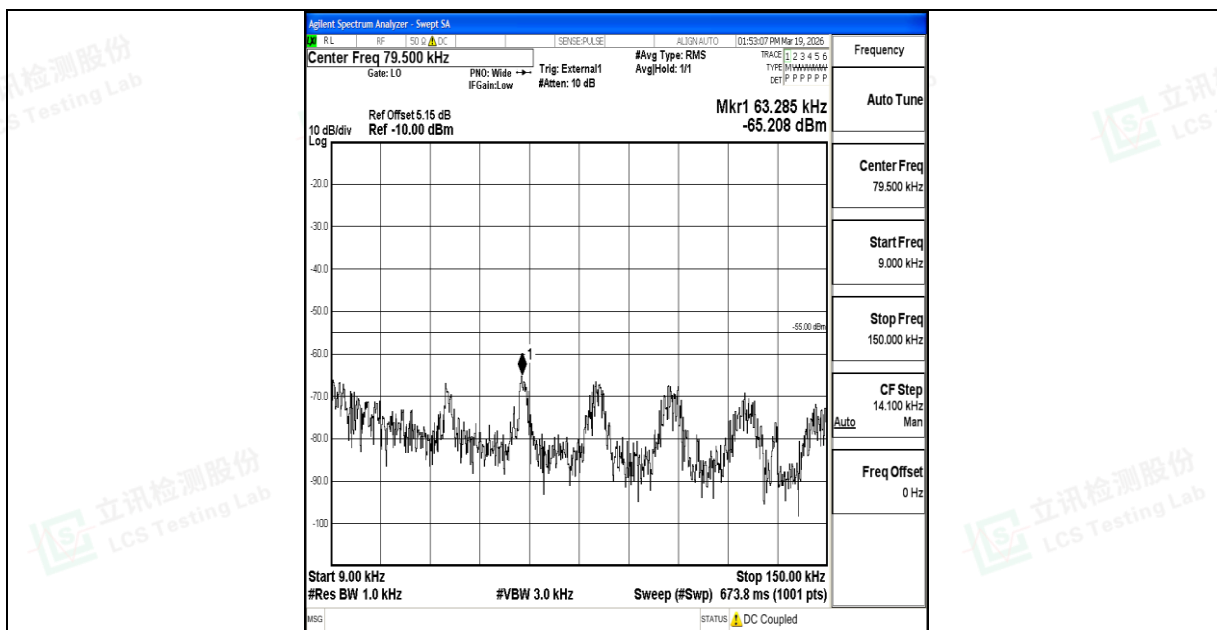
Band41_20MHz_QPSK_40620_1RB#0_0.009~0.15_0.009~0.15
