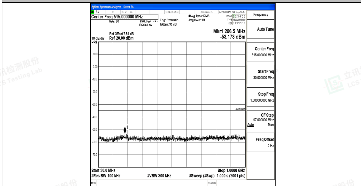
Band41_10MHz_16QAM_41540_1RB#0_30~1000_30~1000
