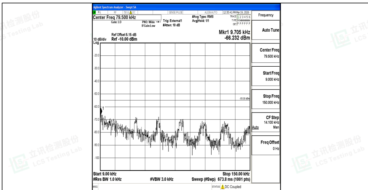
Band41_10MHz_QPSK_39700_1RB#0_0.009~0.15_0.009~0.15
