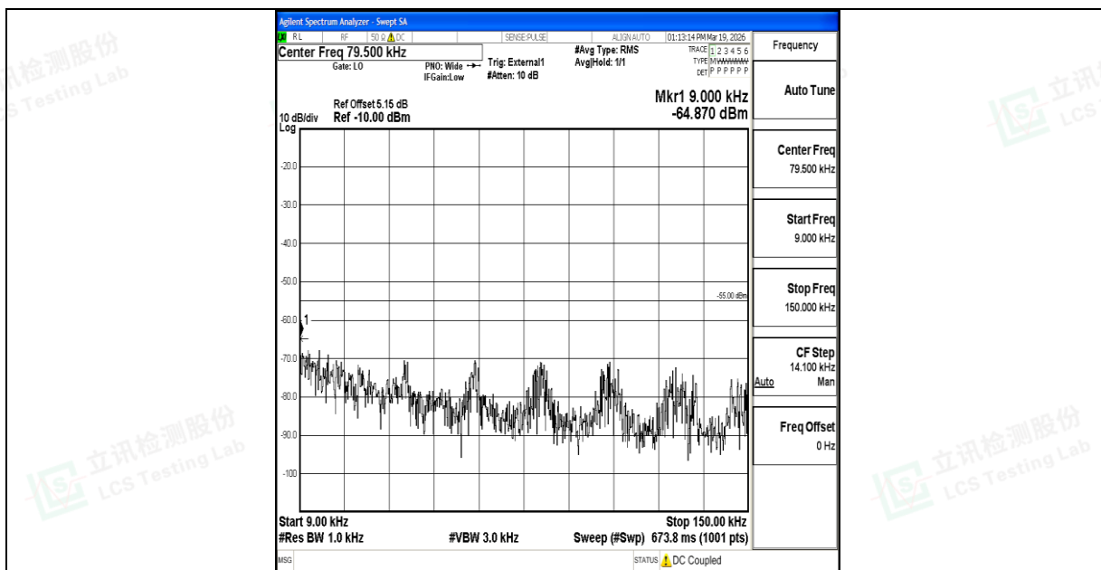
Band41_15MHz_QPSK_39725_1RB#0_0.009~0.15_0.009~0.15
