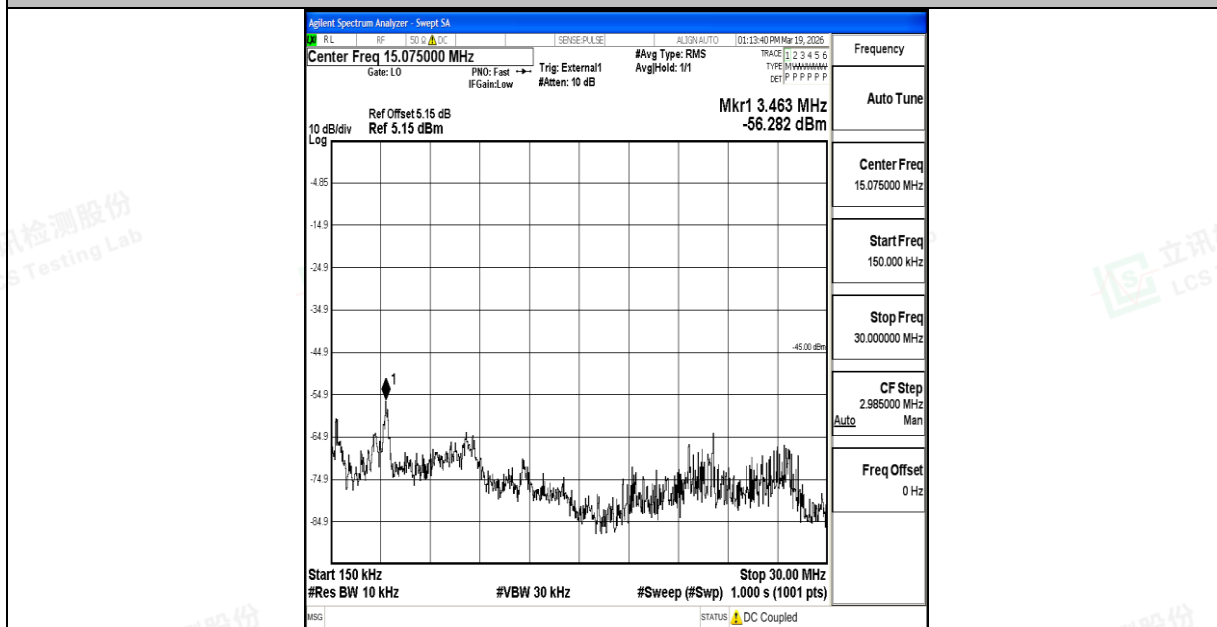
Band41_15MHz_QPSK_39725_1RB#0_0.15~30_0.15~30
