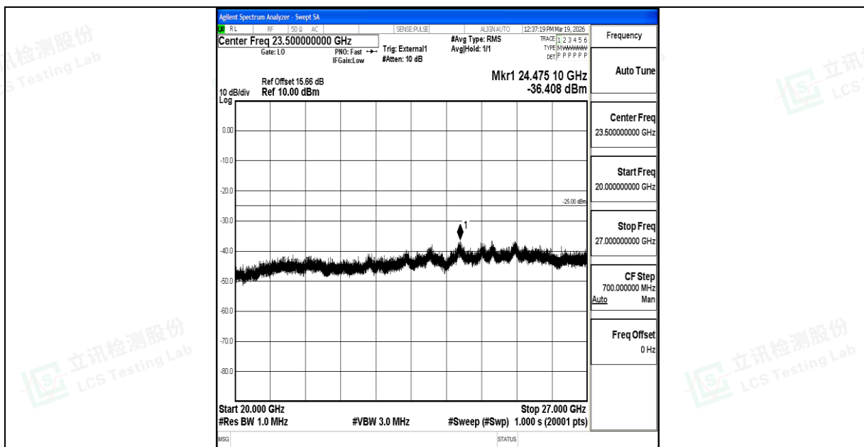
Band41_10MHz_QPSK_39700_1RB#0_20000~27000_20000~27000
