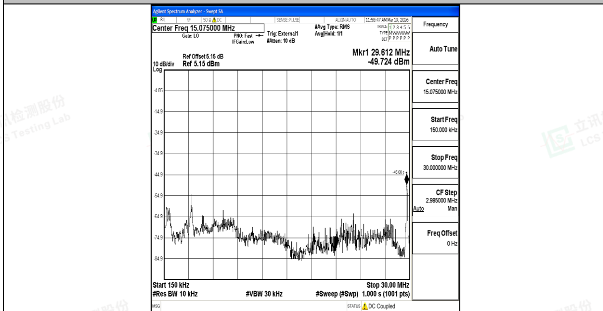
Band41_5MHz_QPSK_40620_1RB#0_0.15~30_0.15~30
