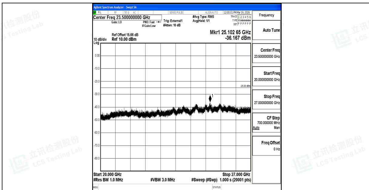
Band41_5MHz_QPSK_40620_1RB#0_20000~27000_20000~27000
