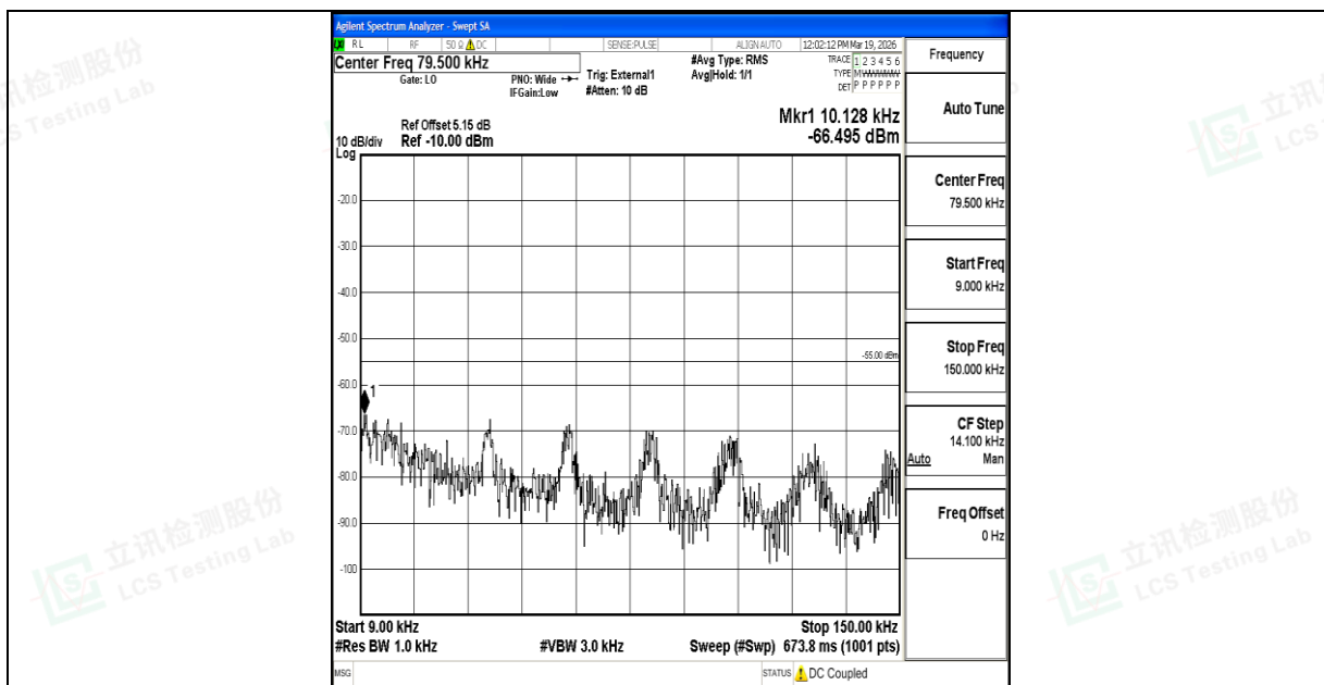
Band41_5MHz_QPSK_41565_1RB#0_0.009~0.15_0.009~0.15
