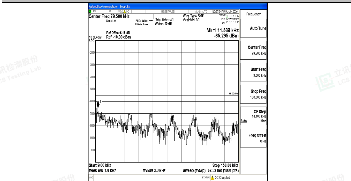
Band41_10MHz_16QAM_39700_1RB#0_0.009~0.15_0.009~0.15
