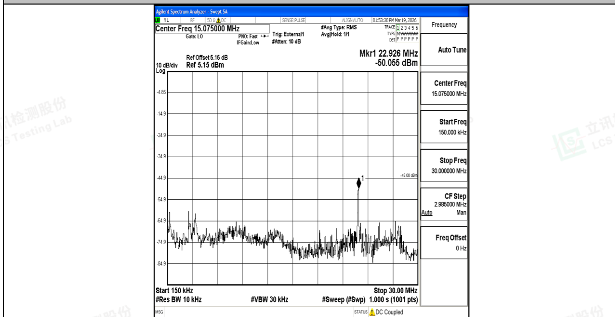
Band41_20MHz_QPSK_40620_1RB#0_0.15~30_0.15~30
