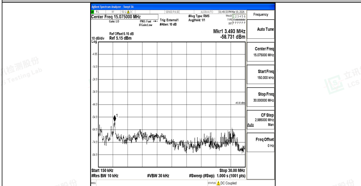
Band41_20MHz_QPSK_39750_1RB#0_0.15~30_0.15~30
