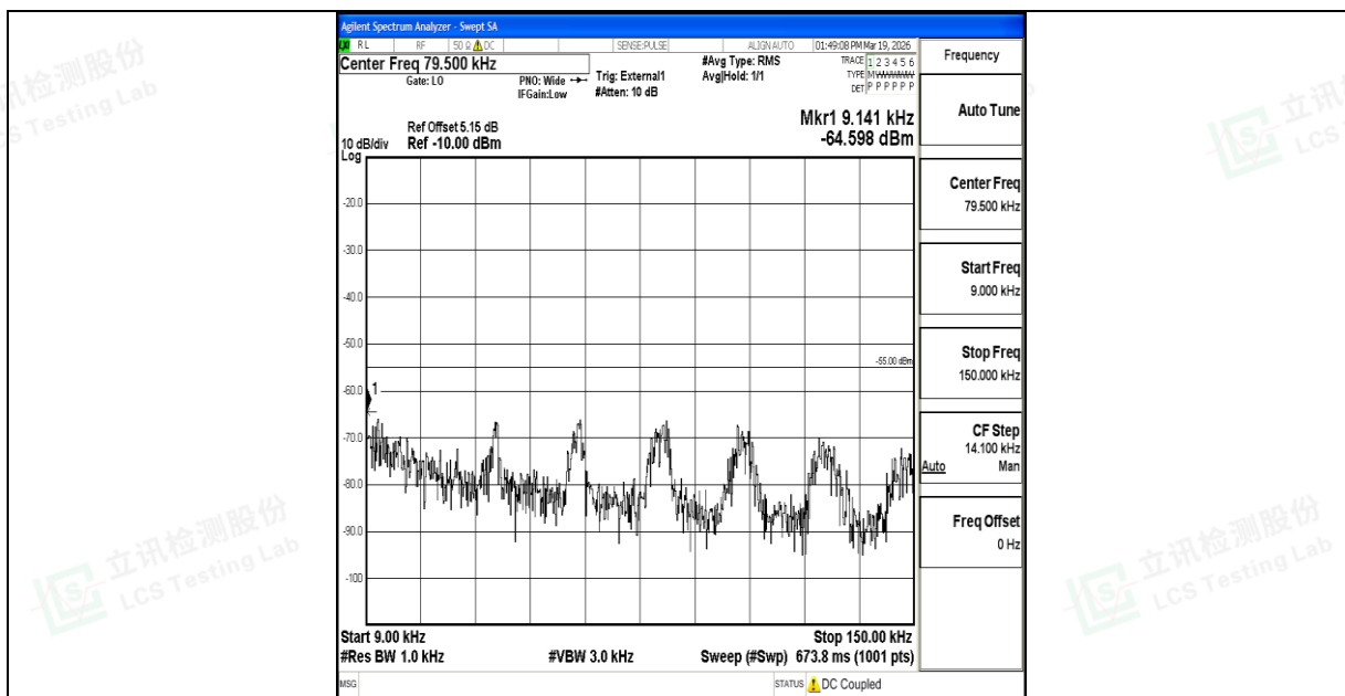
Band41_20MHz_QPSK_39750_1RB#0_0.009~0.15_0.009~0.15
