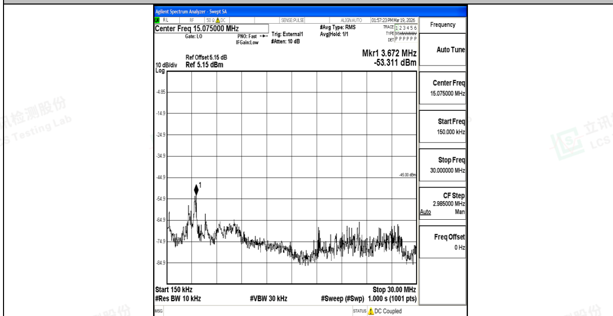
Band41_20MHz_QPSK_41490_1RB#0_0.15~30_0.15~30
