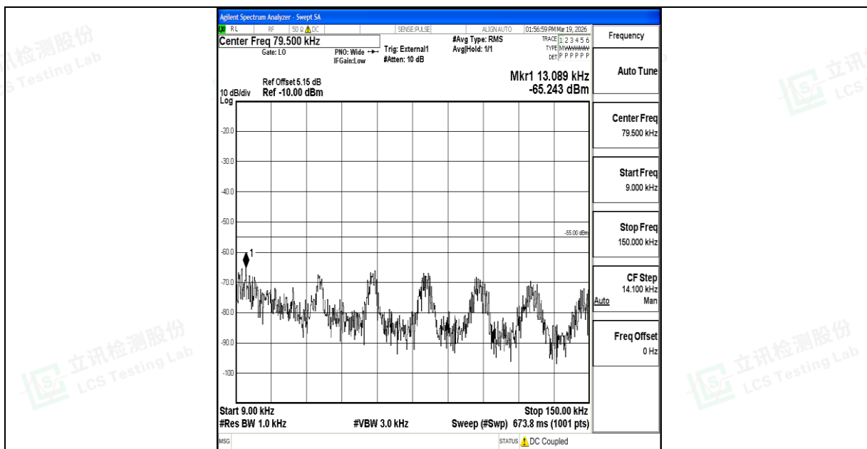
Band41_20MHz_QPSK_41490_1RB#0_0.009~0.15_0.009~0.15
