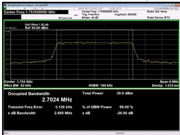
LTE Band 4 3MHz QPSK CH-High
