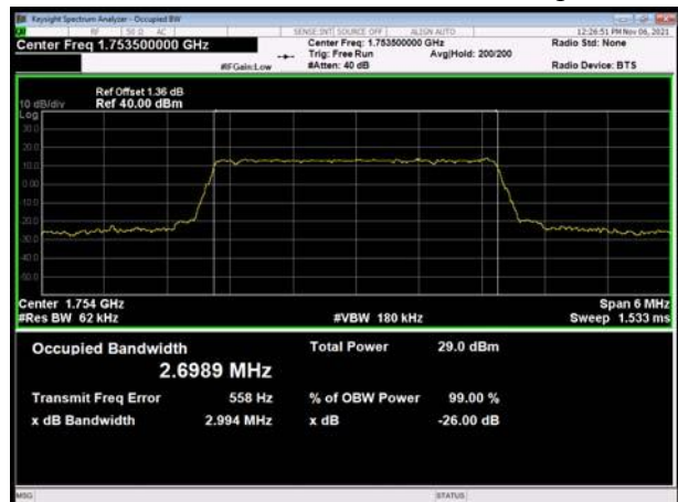
LTE Band 4 3MHz 16QAM CH-High
