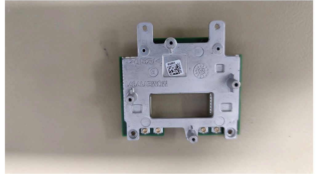
WIFI module Bottom : without shielding
