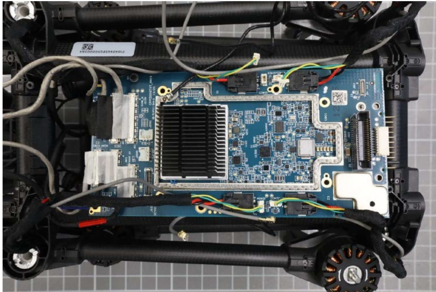
MOTHER BOARD – TOP VIEW – WITHOUT SHIELDING
