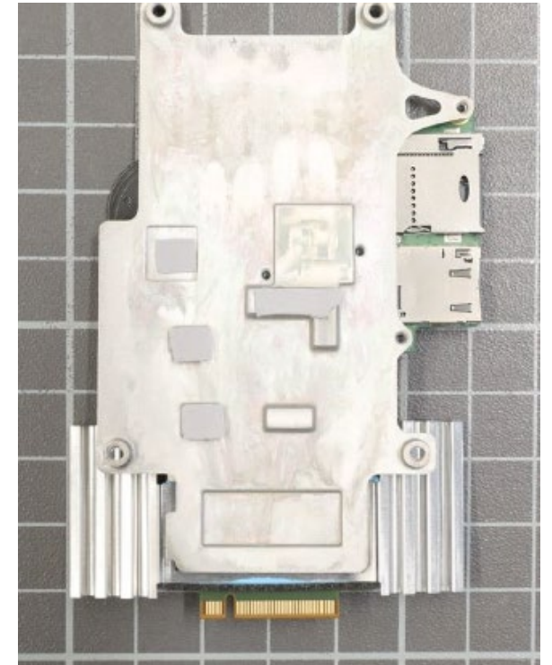
5G – MODULE – Bottom View
