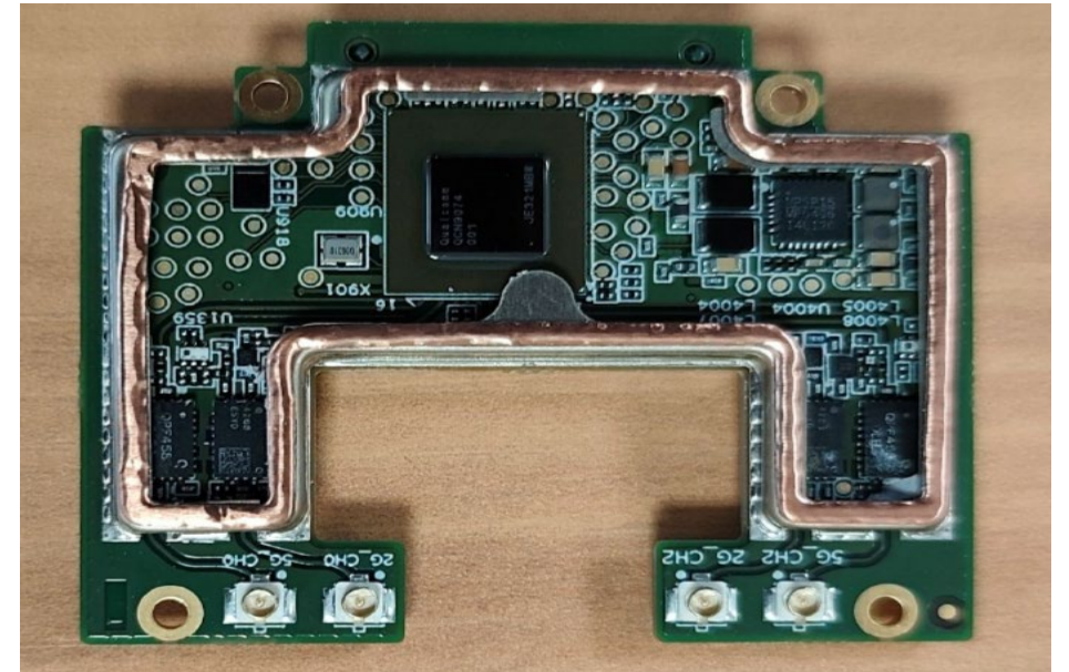
WIFI module Bottom : without shielding
