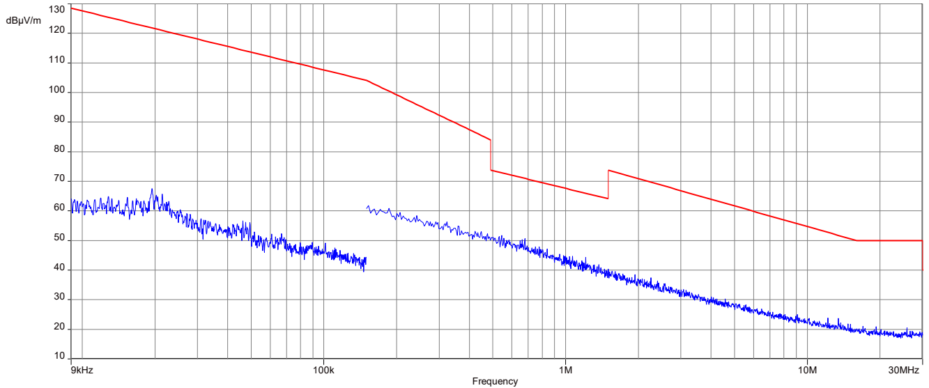
Plot 13: 9 kHz to 30 MHz, U-NII-1; lowest channel
