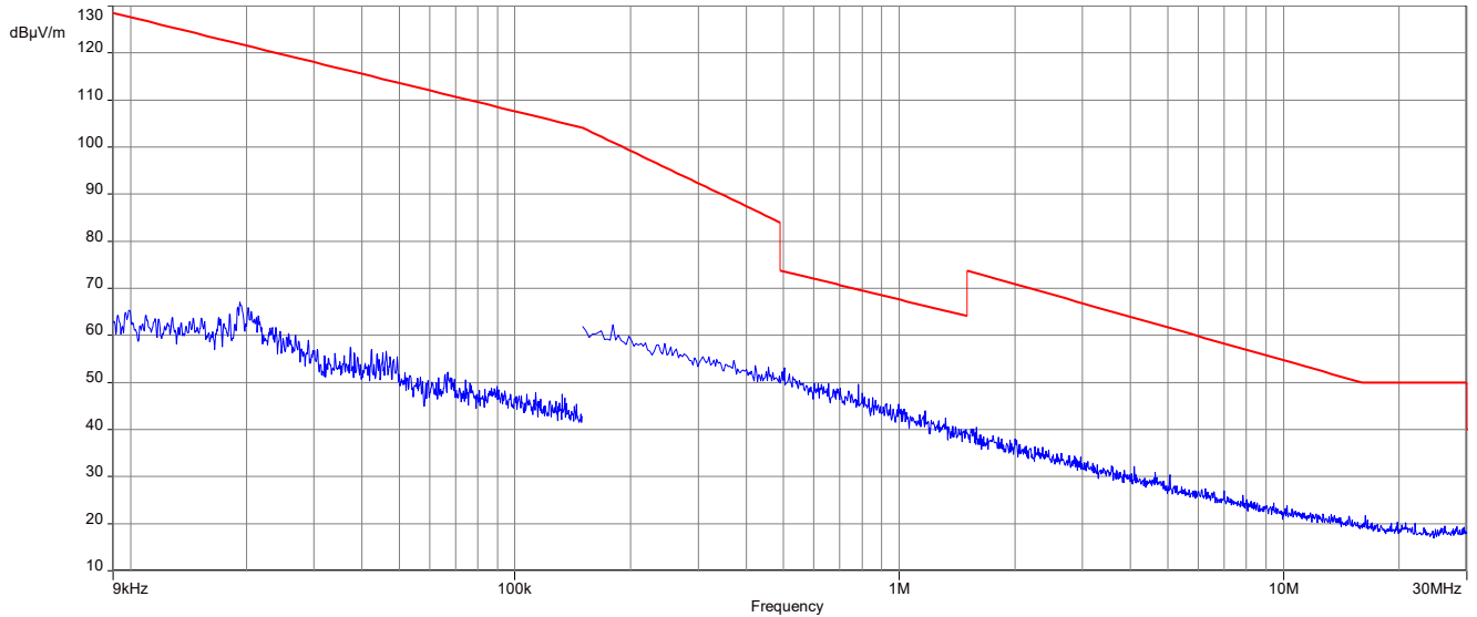
Plot 7: 9 kHz to 30 MHz, U-NII-1; lowest channel
