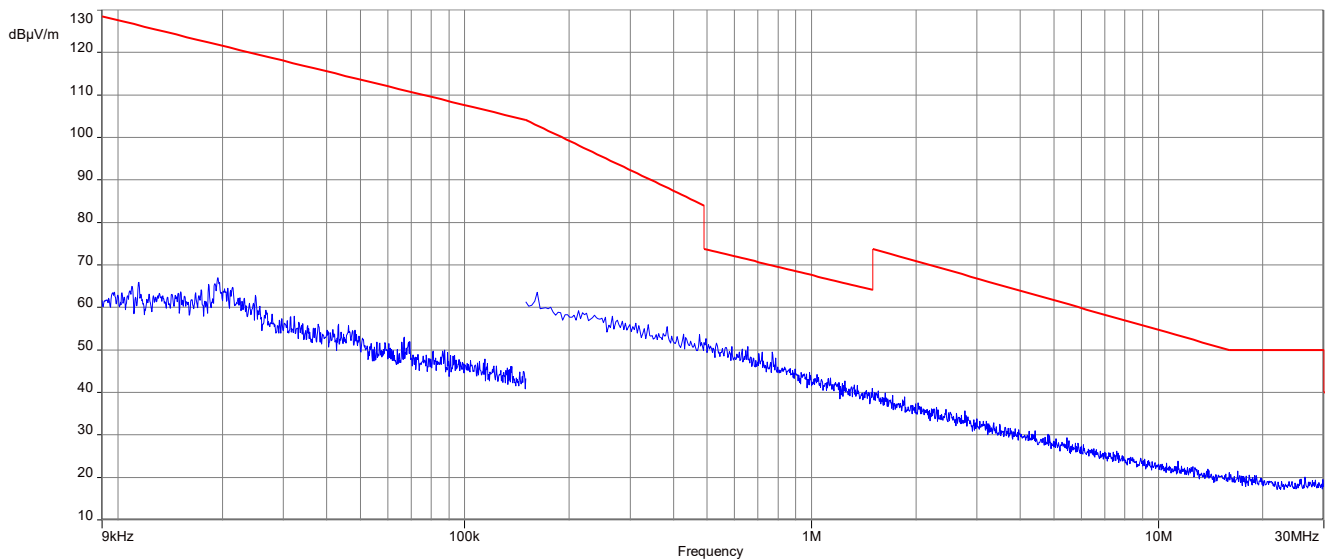
Plot 8: 9 kHz to 30 MHz, U-NII-1; middle channel
