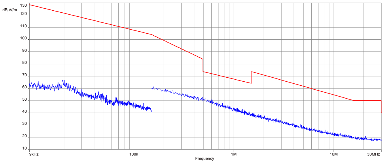
Plot 14: 9 kHz to 30 MHz, U-NII-1; middle channel
