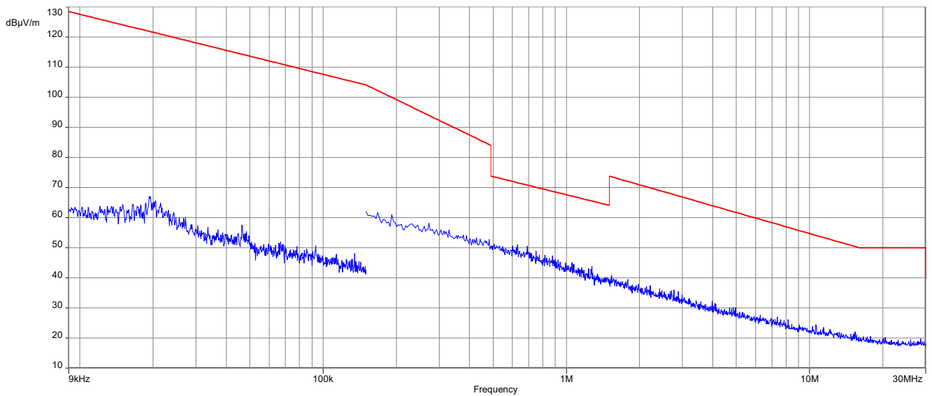
Plot 22: 9 kHz to 30 MHz, U-NII-3; lowest channel
