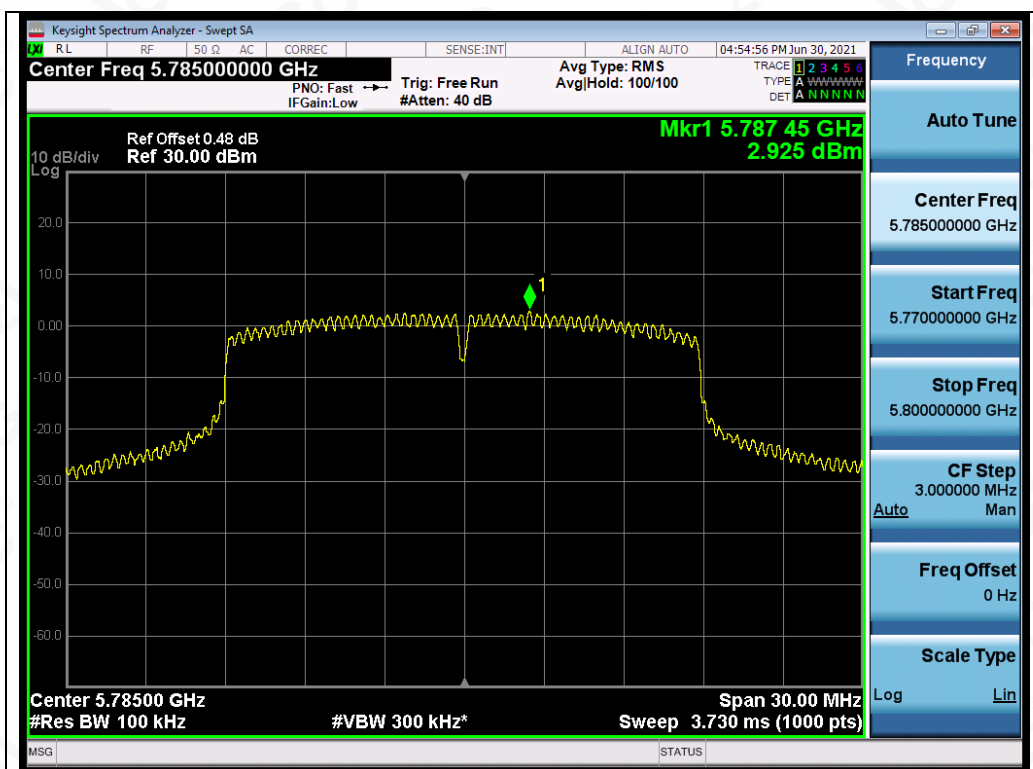
Test_Graph_802.11n20_ANT3_5785_MCS0_PSD
