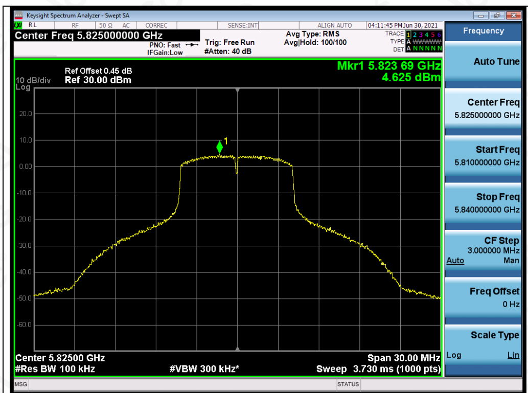
Test_Graph_OFDM_ANT4_5825_6Mbps_PSD
