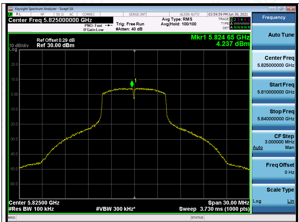
Test_Graph_OFDM_ANT3_5825_6Mbps_PSD
