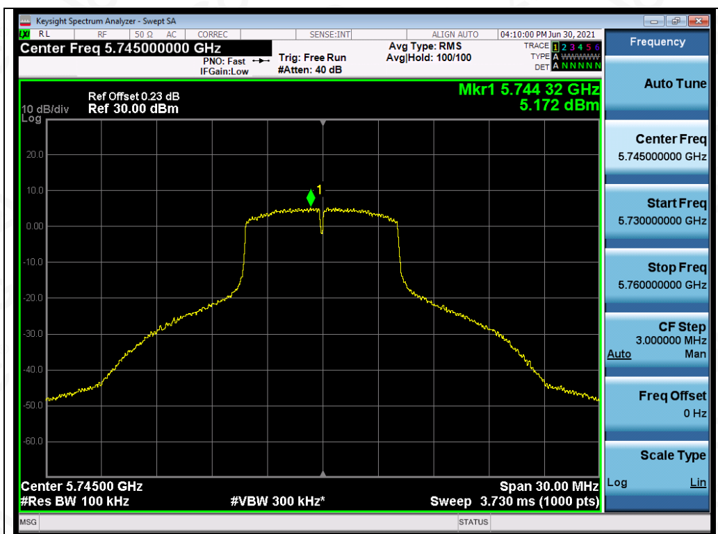
Test_Graph_OFDM_ANT4_5745_6Mbps_PSD
