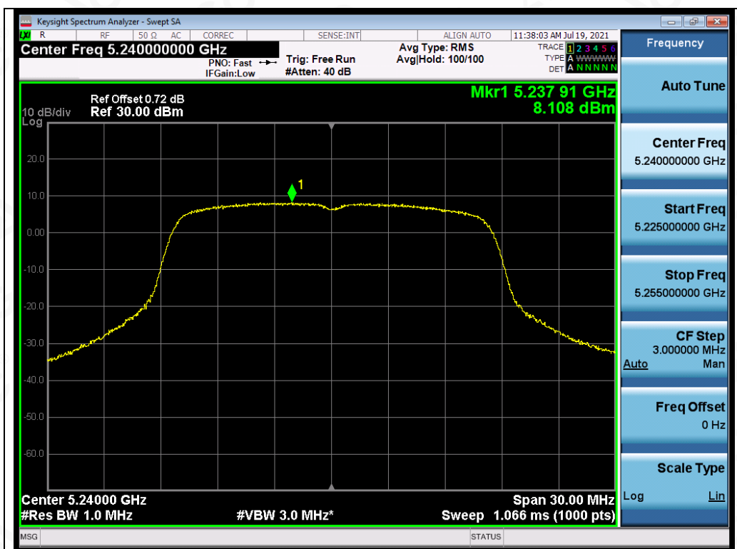
Test_Graph_802.11a_ANT3_5240_6Mbps_PSD
