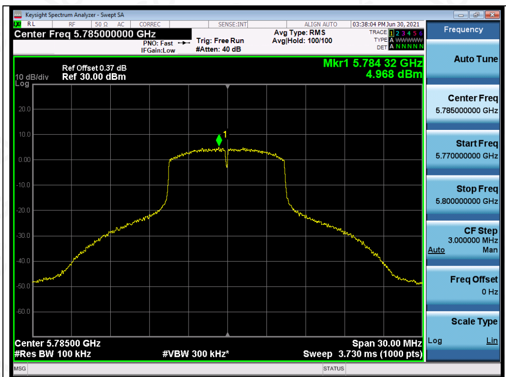
Test_Graph_OFDM_ANT1_5785_MCS0_PSD
