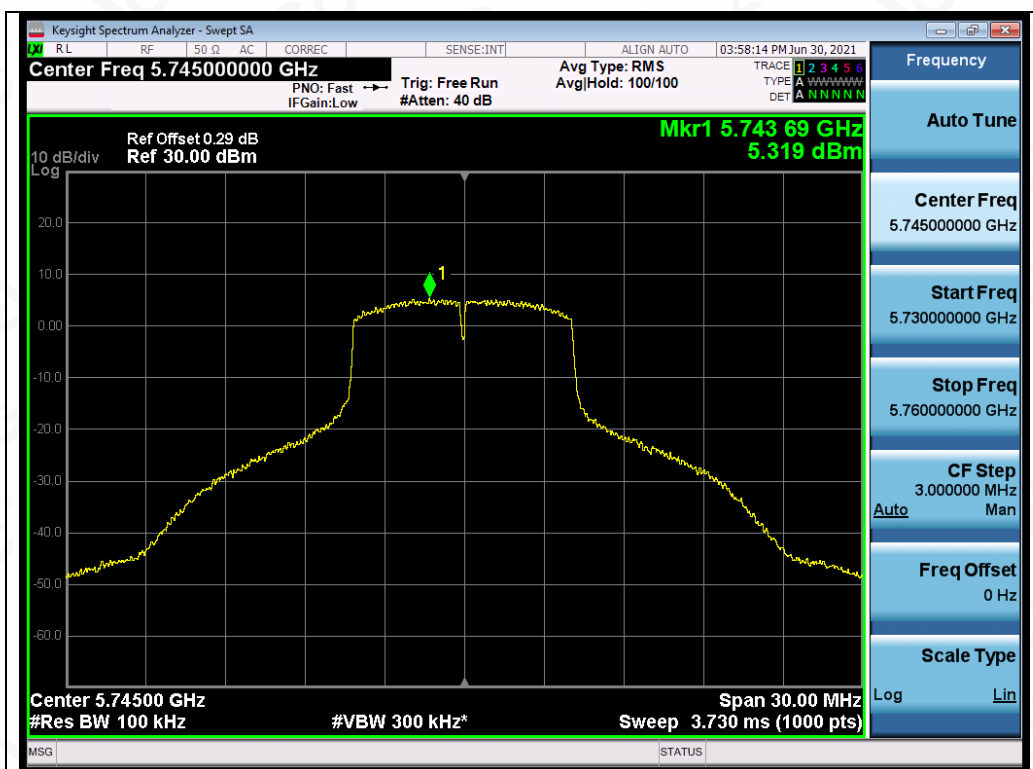
Test_Graph_OFDM_ANT3_5745_6Mbps_PSD
