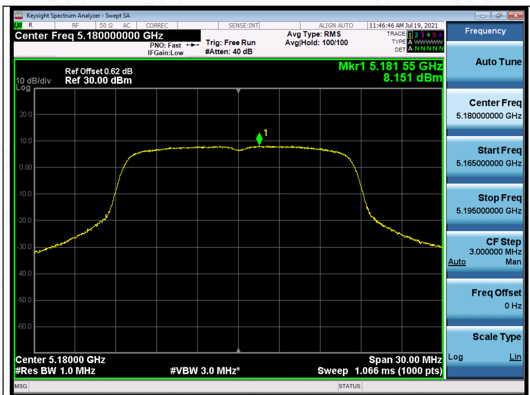
Test_Graph_802.11a_ANT4_5180_6Mbps_PSD
