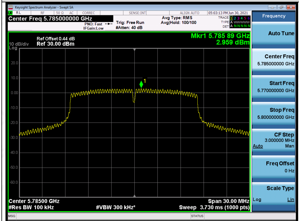
Test_Graph_802.11a_ANT4_5785_6Mbps_PSD
