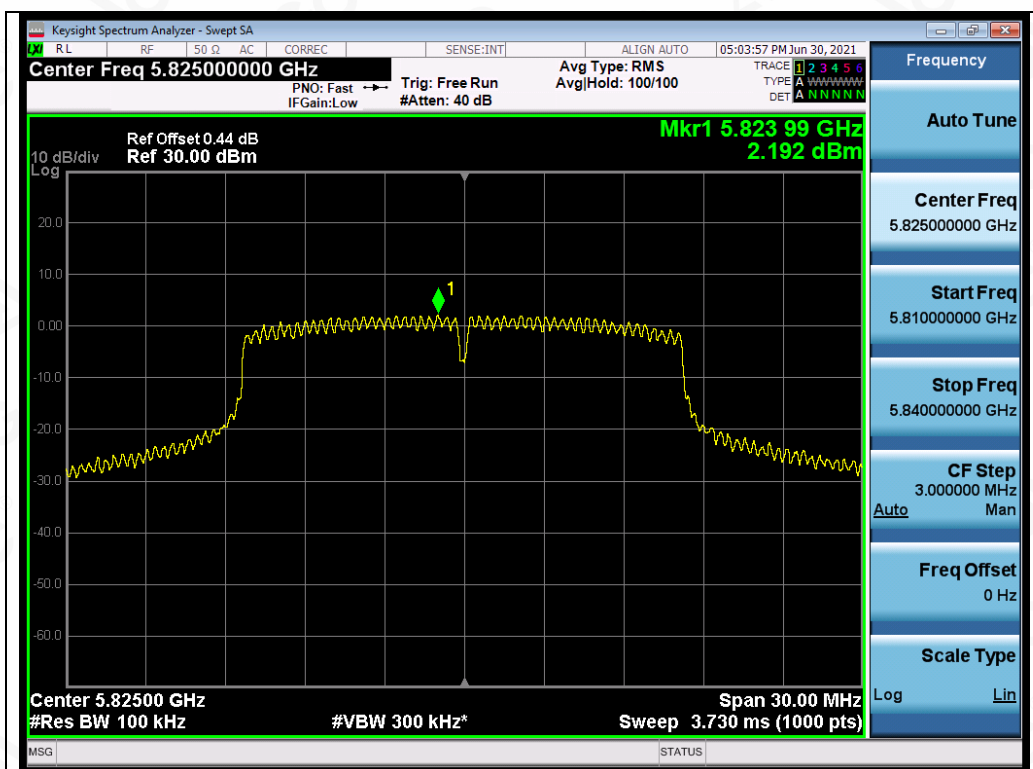
Test_Graph_802.11a_ANT4_5825_6Mbps_PSD
