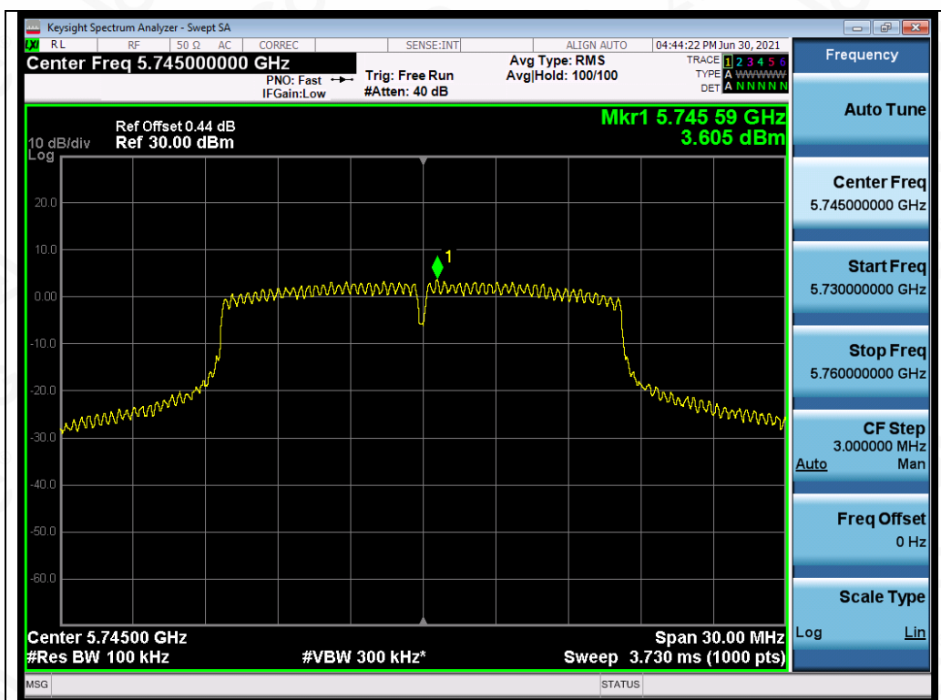
Test_Graph_802.11a_ANT3_5745_6Mbps_PSD
