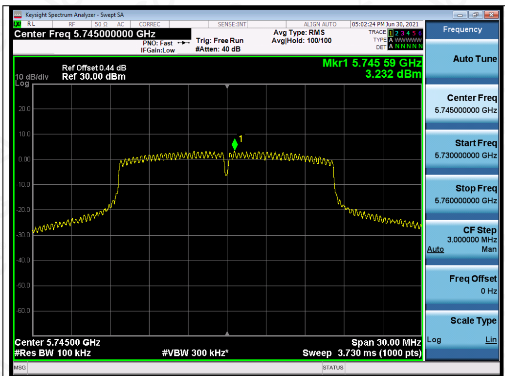
Test_Graph_802.11a_ANT4_5745_6Mbps_PSD
