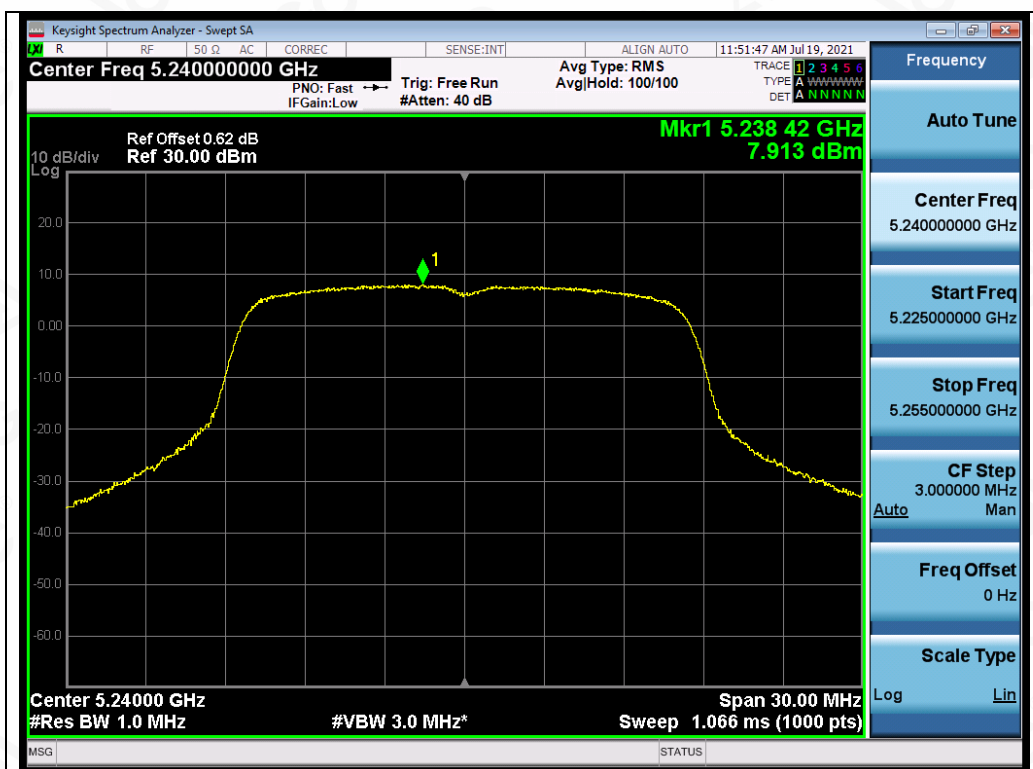
Test_Graph_802.11a_ANT4_5240_6Mbps_PSD
