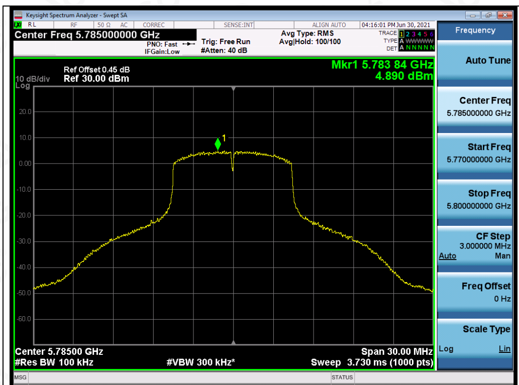
Test_Graph_OFDM_ANT4_5785_MCS0_PSD
