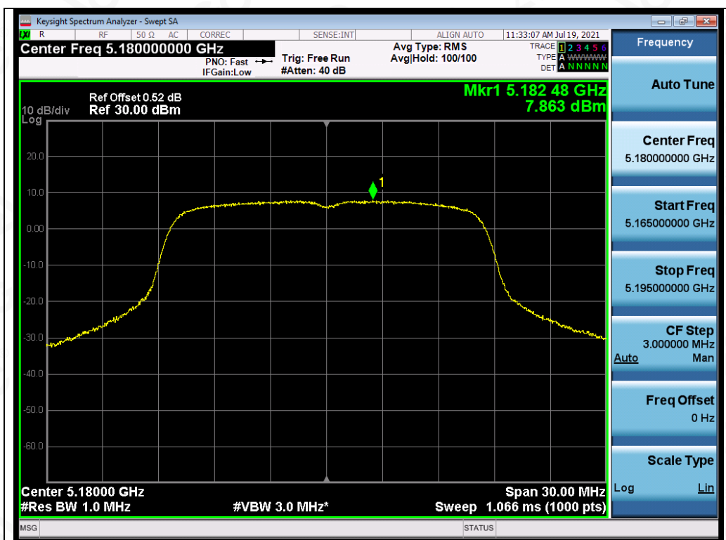
Test_Graph_802.11a_ANT3_5180_6Mbps_PSD
