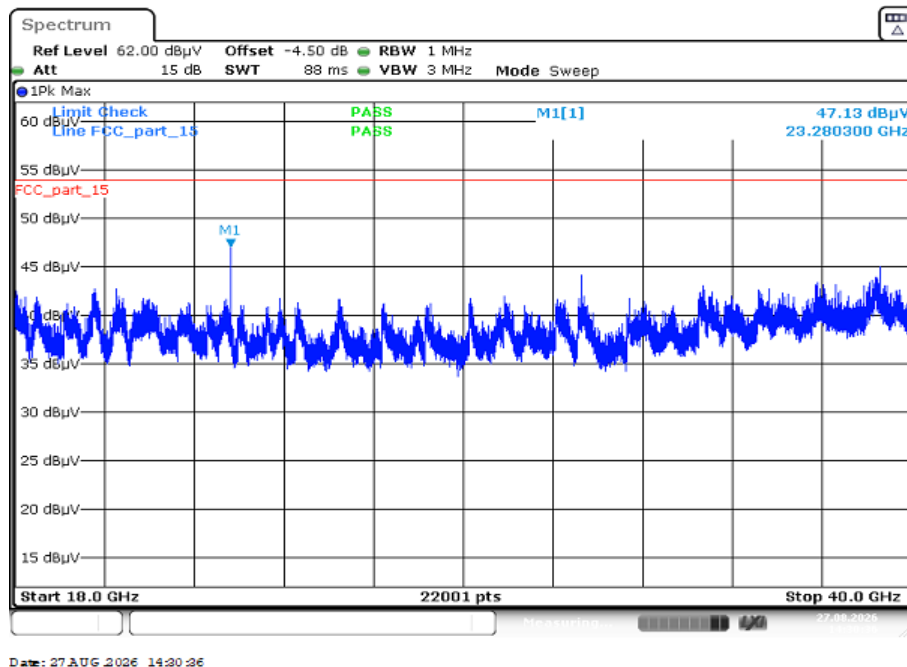
Plot 8: 18 GHz to 40 GHz; vertical & horizontal polarization; U-NII-3; all channels
