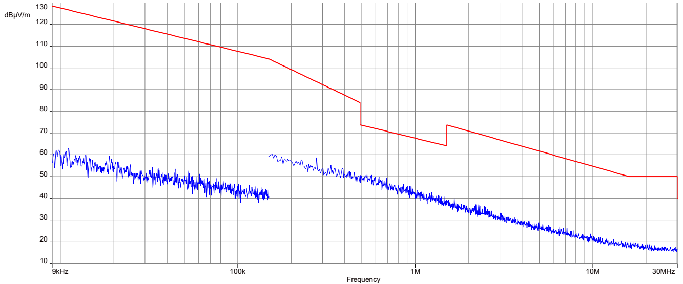
Plot 1: Antenna 1, 9 kHz to 30 MHz, U-NII-1; lowest channel
