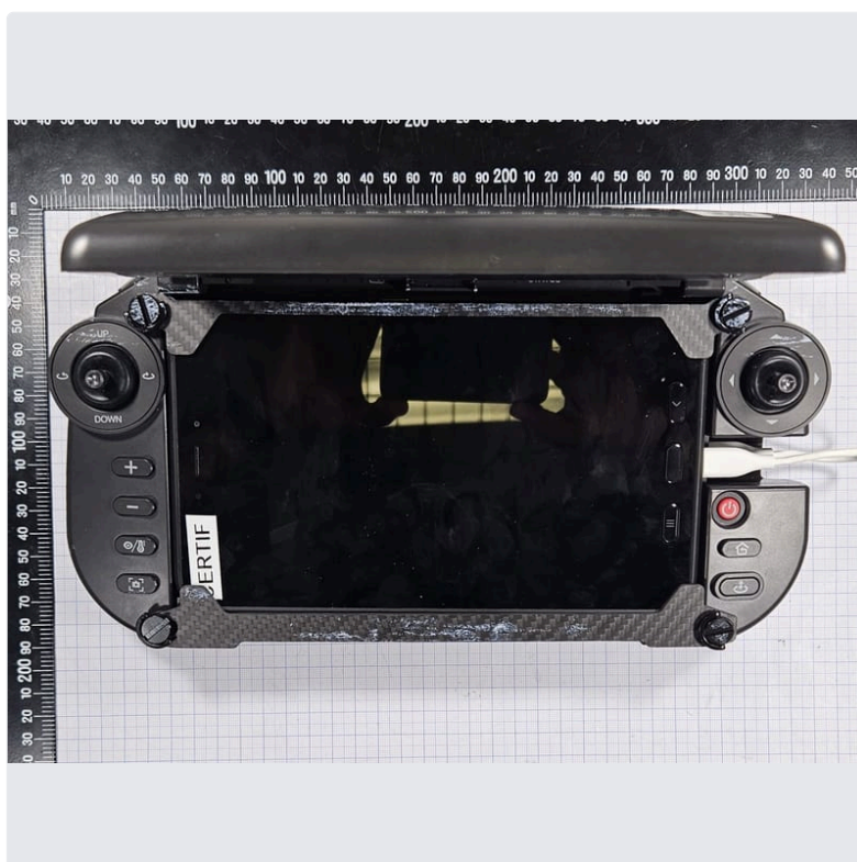
Photo 4 DUT - top view opened
