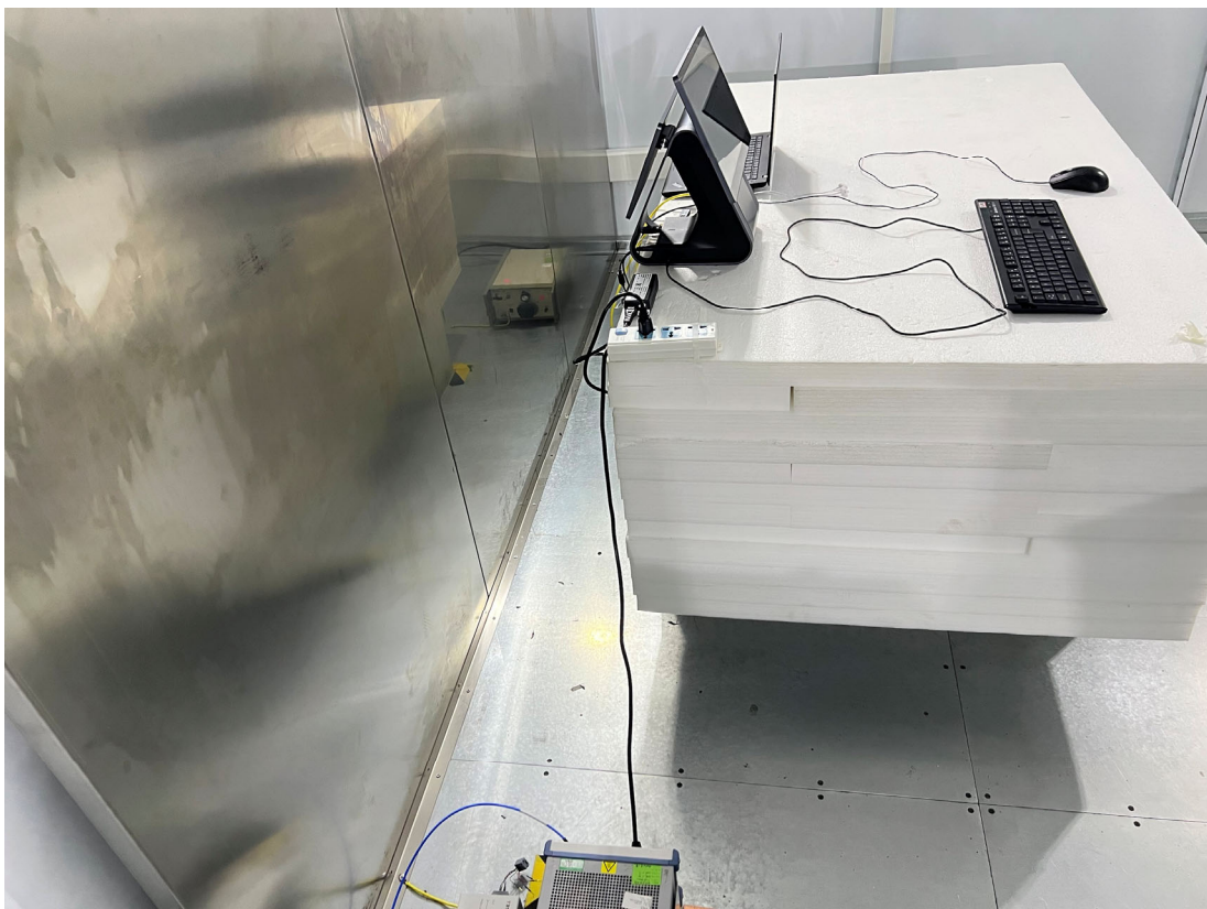
Conducted Emission - Side View(Adapter #1)
