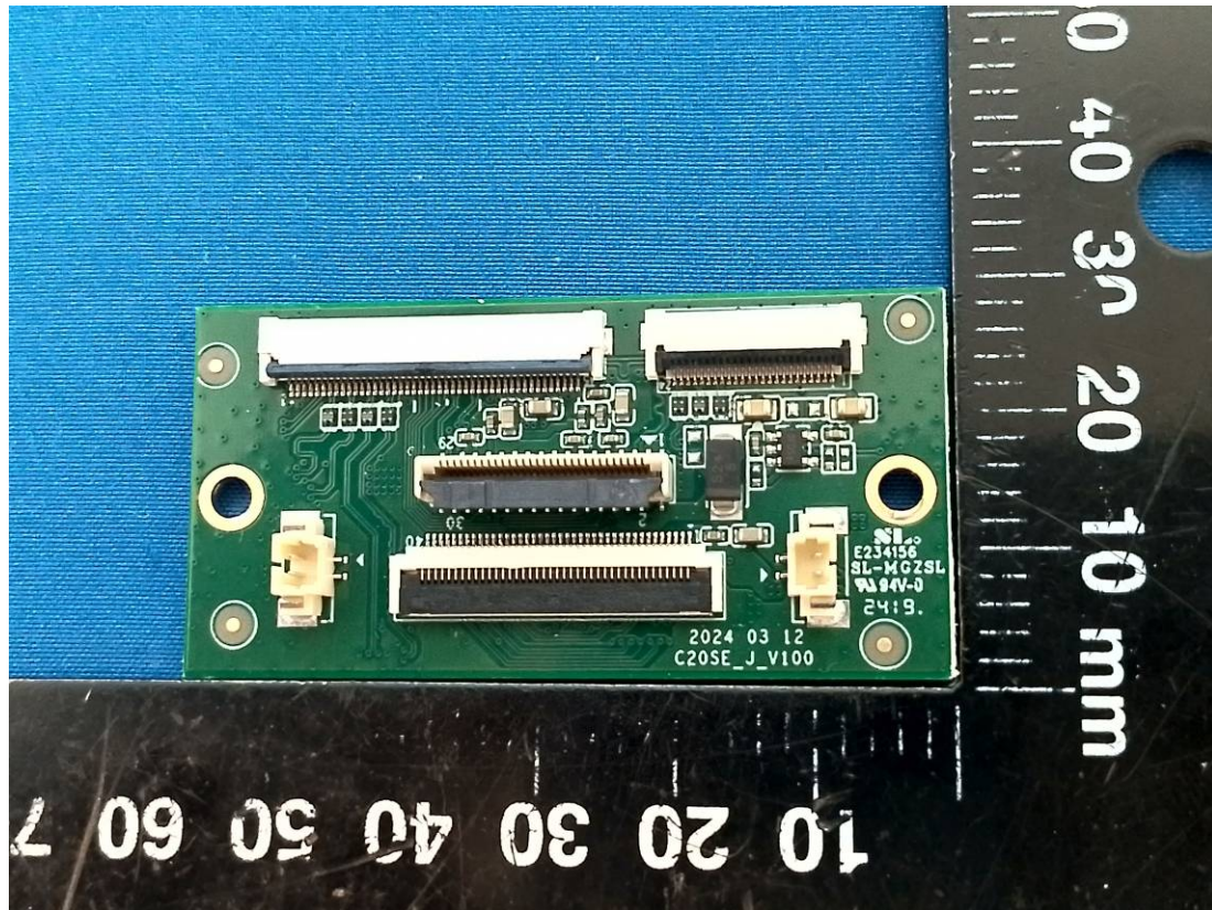
J Board
