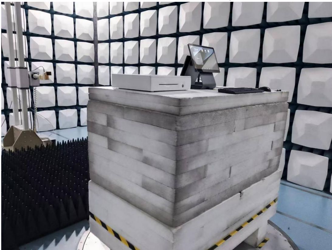
Radiated Emission 18-26.5GHz View Configuration 1#
