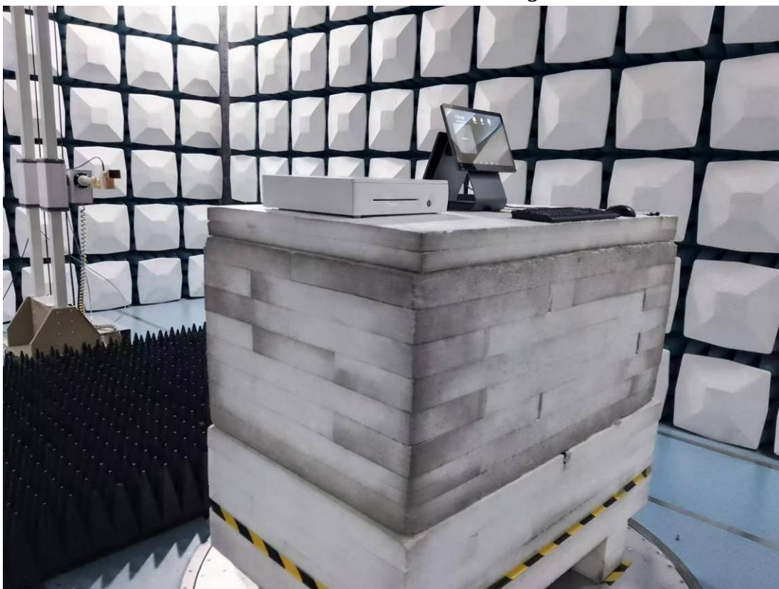
Radiated Emission 18-25GHz View Configuration 1#
