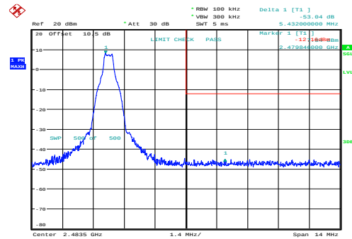
GFSK_High
