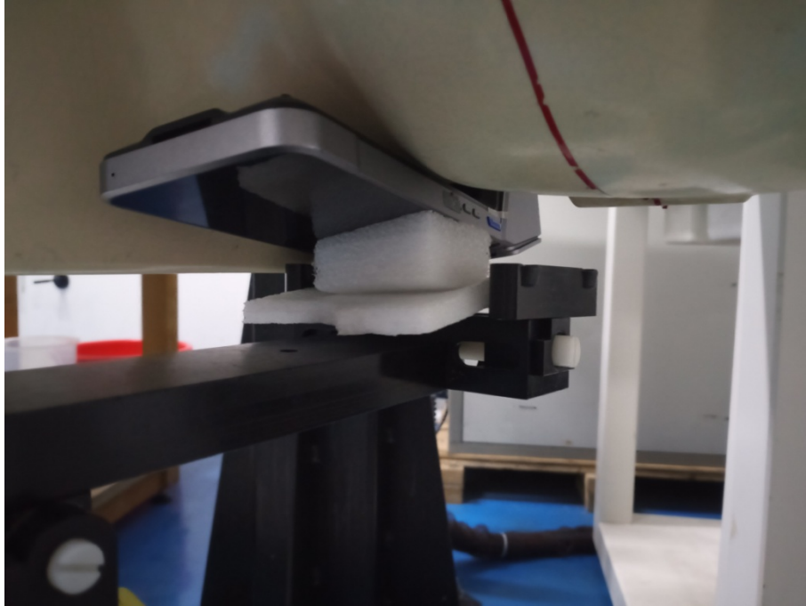
Body Back Setup Photo(WLAN 2.4G/5G/BT)
