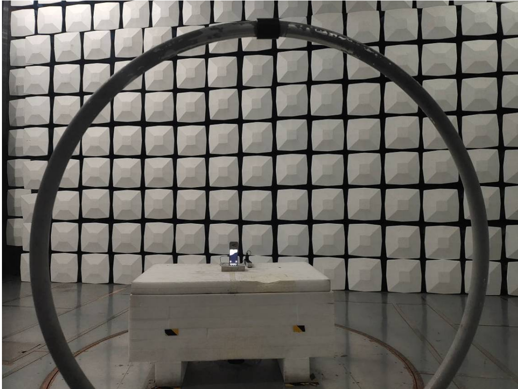
Radiated Emission 9k-30MHz Perpendicular View–Model: M20
