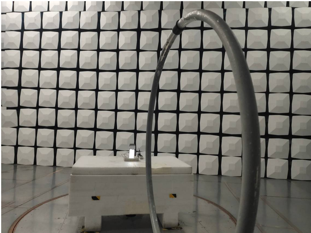
Radiated Emission 9k-30MHz Perpendicular View M1
