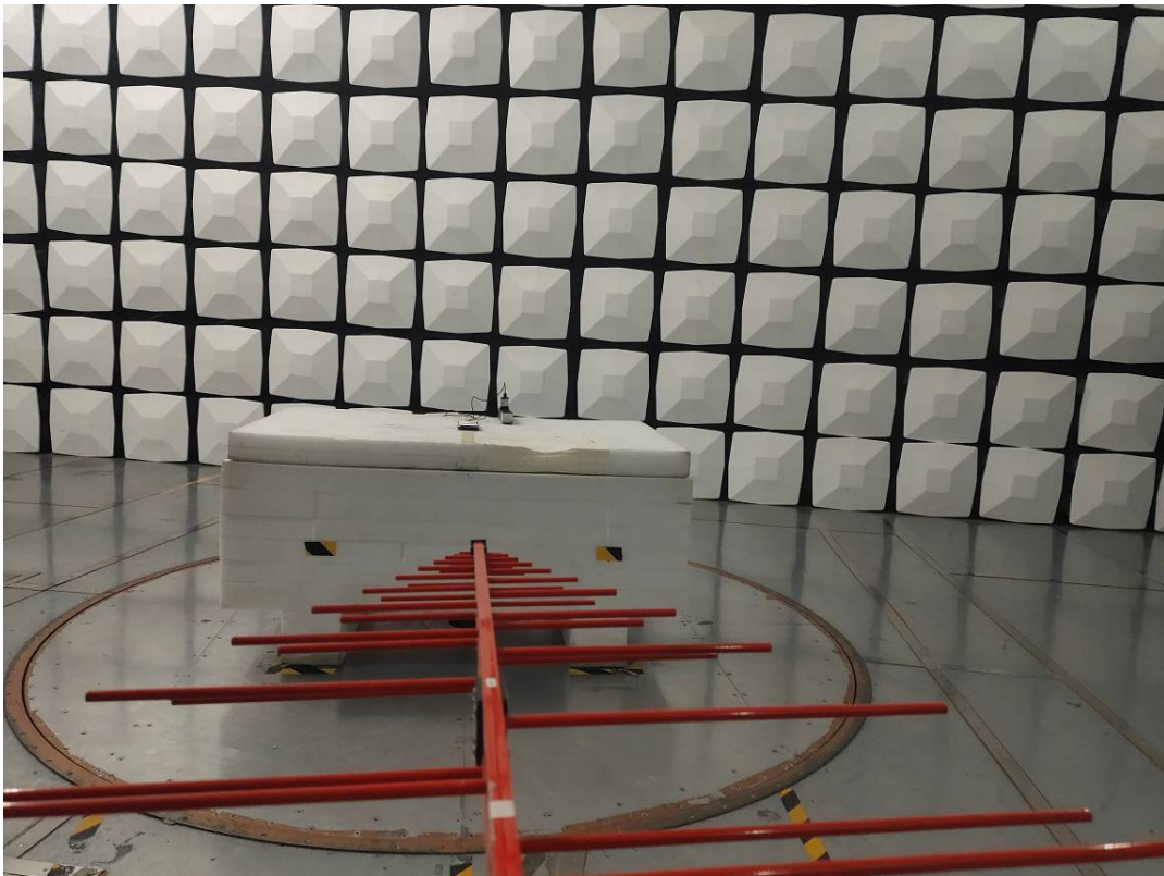
Radiated Emission 30M-1GHz front View M5
