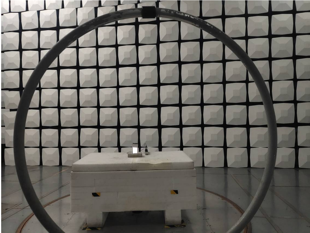
Radiated Emission 9k-30MHz Perpendicular View M5
