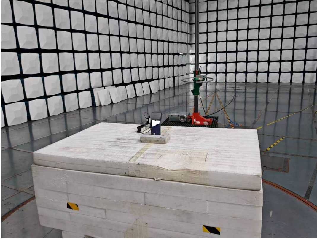
Radiated Emission 30M-1GHz front View M4
