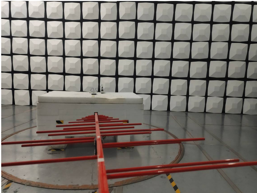
Radiated Emission 30M-1GHz front View M6
