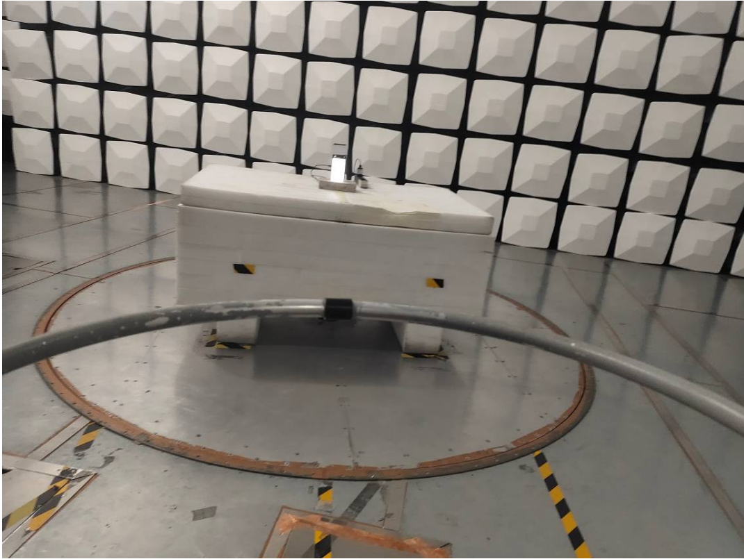
Radiated Emission 30M-1GHz front View M2
