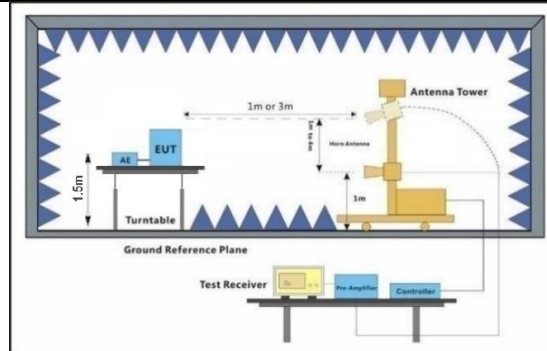
Figure 3. above 1GHz
