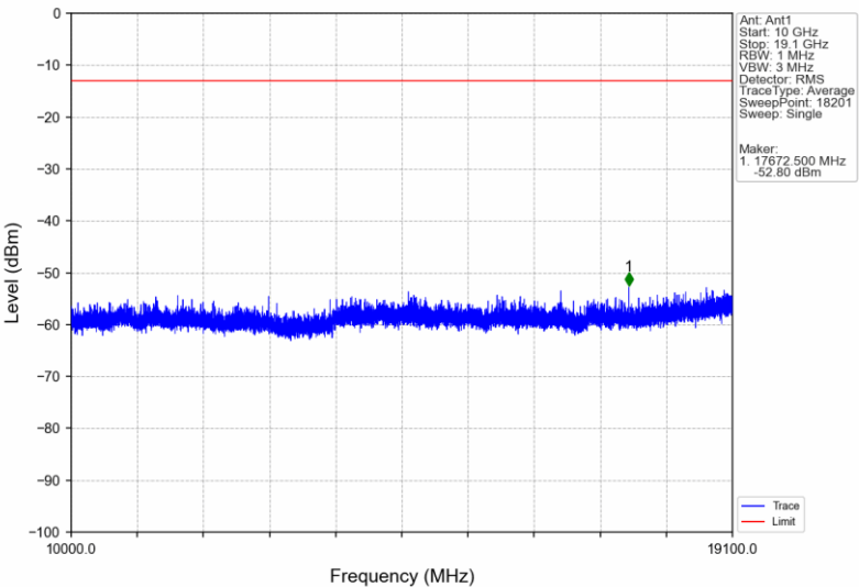
Band2_RMC_HCH_1907.6MHz_12.2kbps RMC_NTNV
