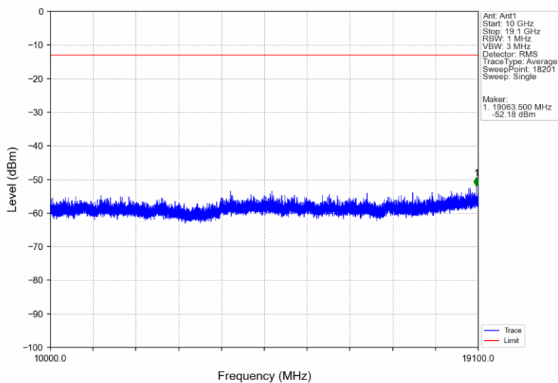
Band2_HSDPA_MCH_1880MHz_Subtest 1_NTNV
