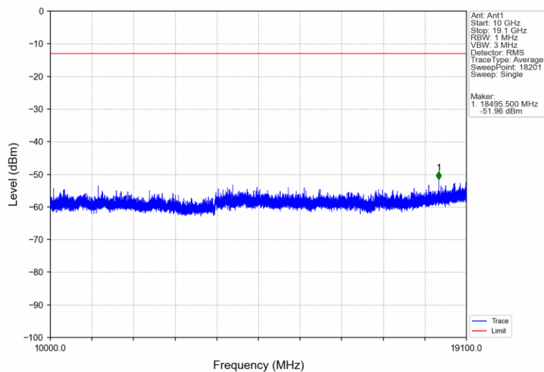
Band2_HSDPA_HCH_1907.6MHz_Subtest 1_NTNV
