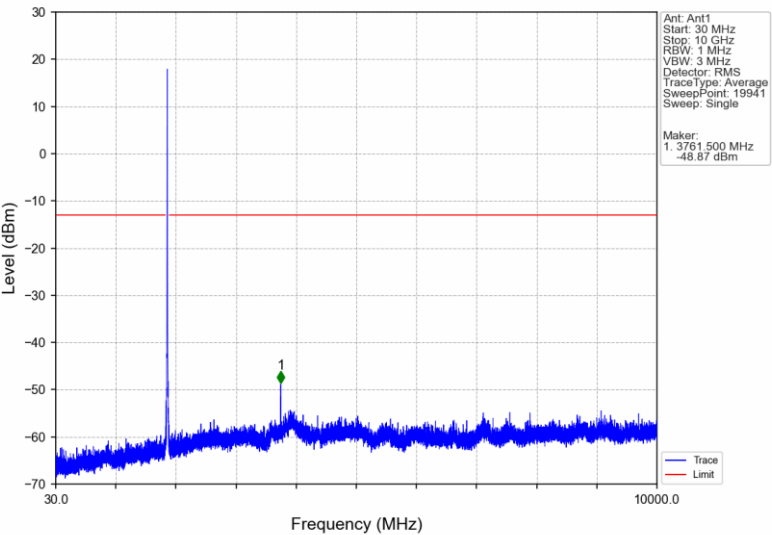
Band2_RMC_MCH_1880MHz_12.2kbps RMC_NTNV
