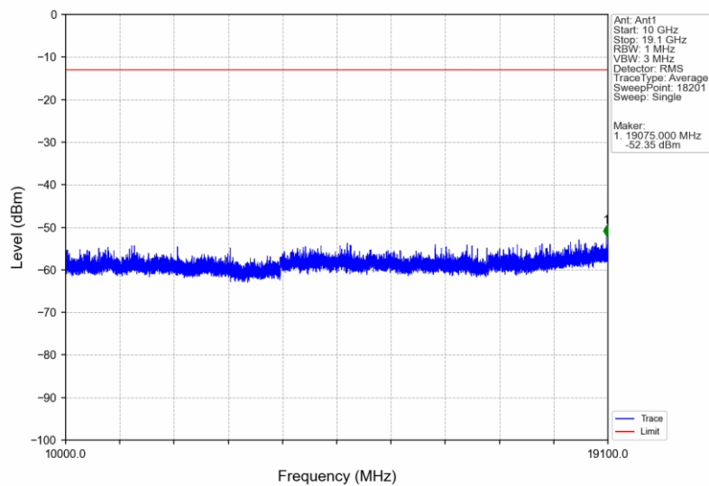
Band2_RMC_HCH_1907.6MHz_12.2kbps RMC_NTNV
