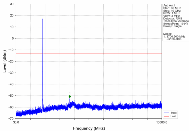
Band2_HSDPA_LCH_1852.4MHz_Subtest 1_NTNV
