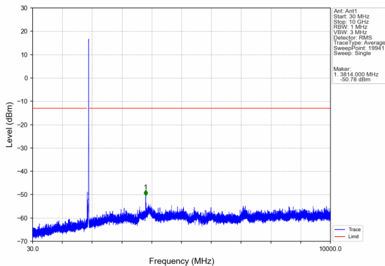
Band2_HSUPA_HCH_1907.6MHz_Subtest 1_NTNV
