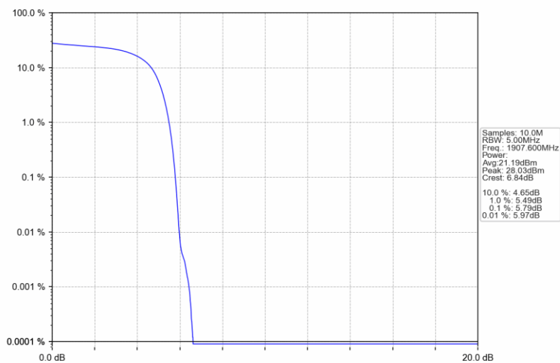
Band2_HSDPA_HCH_1907.6MHz_Subtest 1_NTNV
