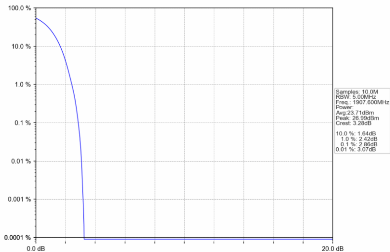
Band2_RMC_HCH_1907.6MHz_12.2kbps RMC_NTNV
