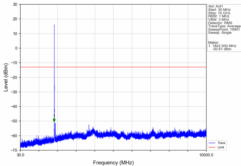
Band2_HSUPA_LCH_1852.4MHz_Subtest 1_NTNV
