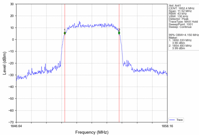
Band2_HSDPA_LCH_1852.4MHz_Subtest 1_NTNV
