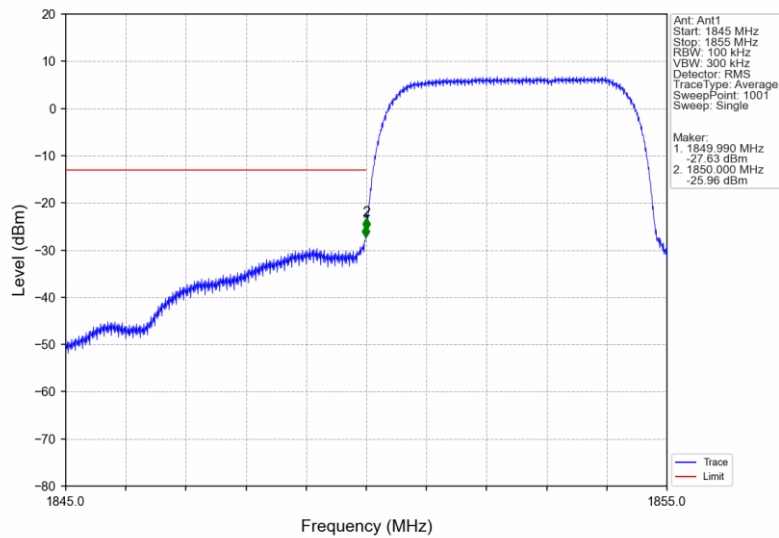
Band2_HSUPA_LCH_1852.4MHz_Subtest 1_NTNV
