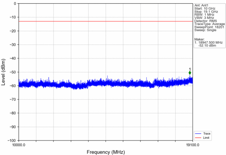
Band2_RMC_MCH_1880MHz_12.2kbps RMC_NTNV
