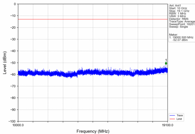
Band2_HSUPA_HCH_1907.6MHz_Subtest 1_NTNV
