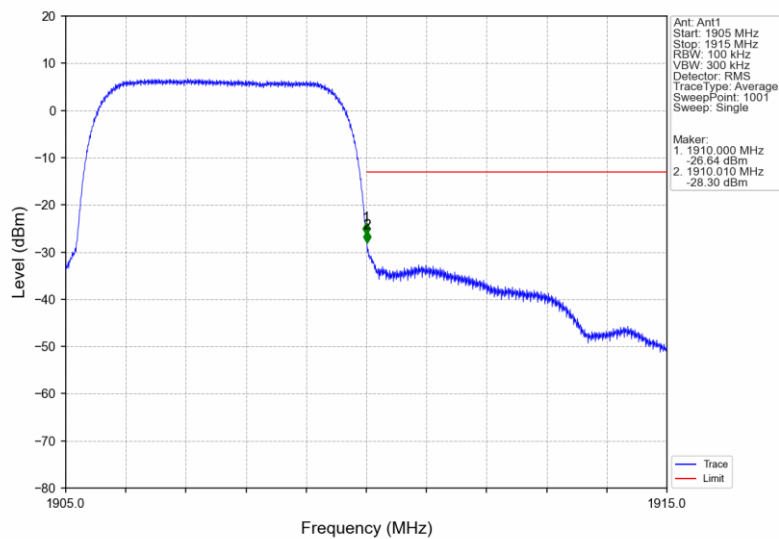
Band2_HSUPA_HCH_1907.6MHz_Subtest 1_NTNV
