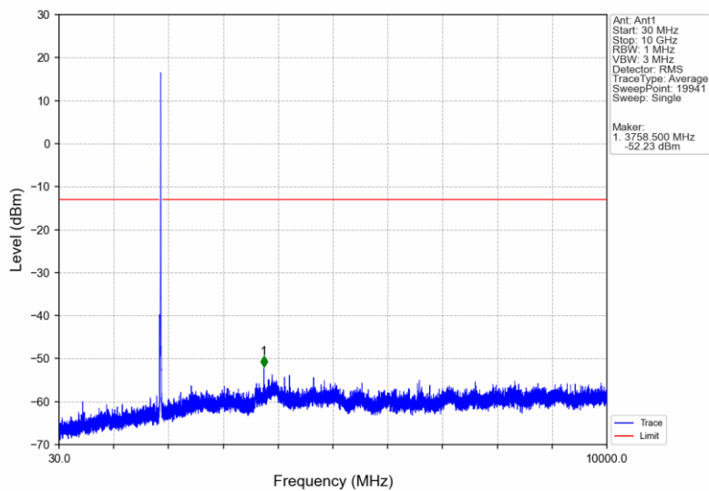
Band2_HSDPA_MCH_1880MHz_Subtest 1_NTNV
