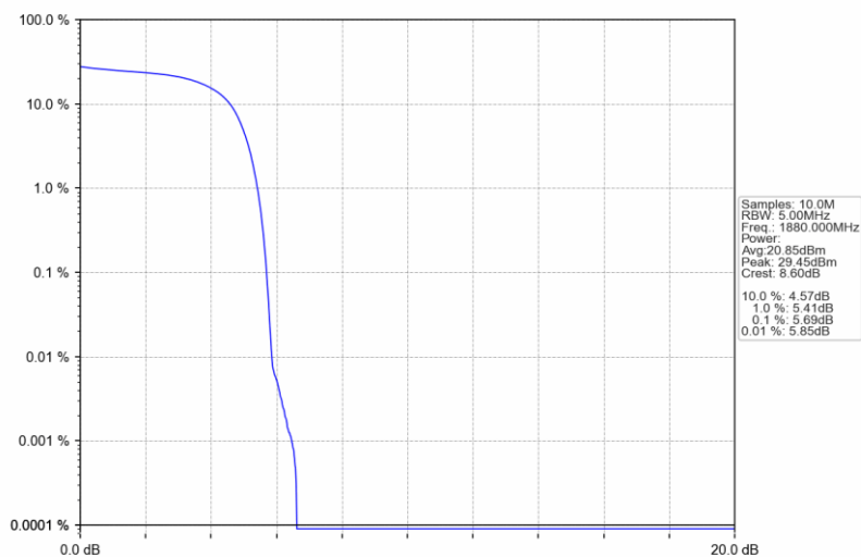
Band2_HSDPA_MCH_1880MHz_Subtest 1_NTNV
