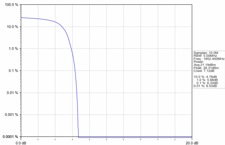
Band2_HSUPA_LCH_1852.4MHz_Subtest 1_NTNV
