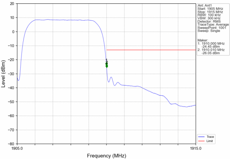
Band2_RMC_HCH_1907.6MHz_12.2kbps RMC_NTNV
