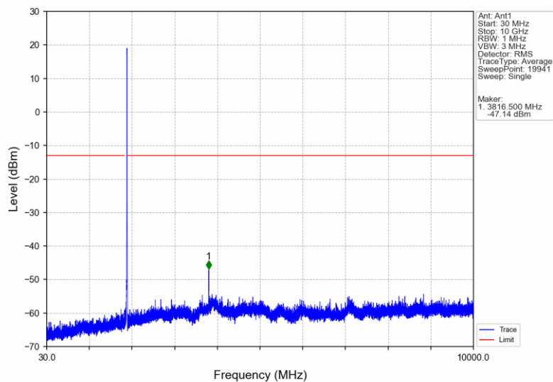
Band2_RMC_HCH_1907.6MHz_12.2kbps RMC_NTNV
