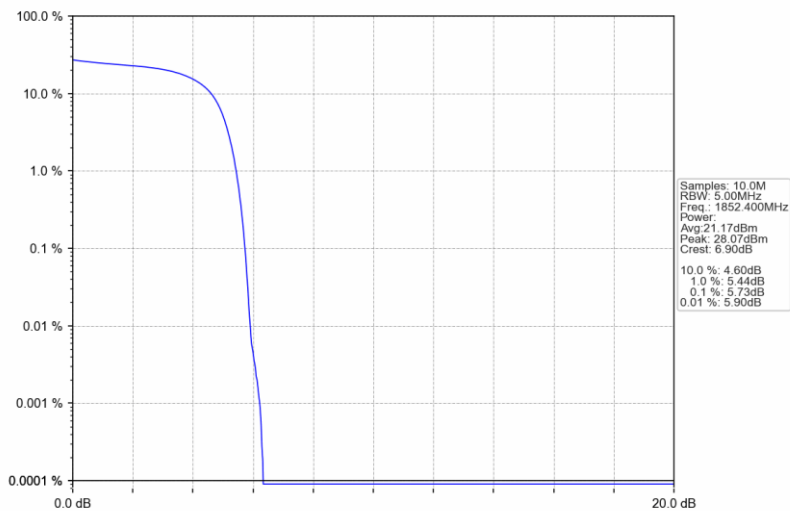
Band2_HSDPA_LCH_1852.4MHz_Subtest 1_NTNV
