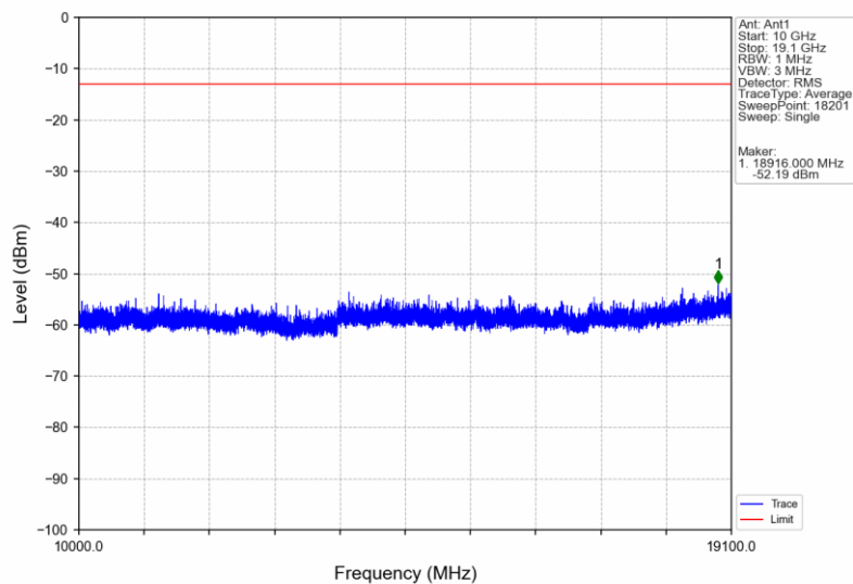
Band2_HSUPA_HCH_1907.6MHz_Subtest 1_NTNV
