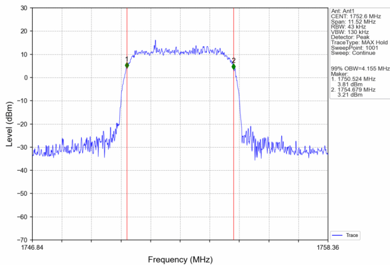
Band4_HSDPA_HCH_1752.6MHz_Subtest 1_NTNV
