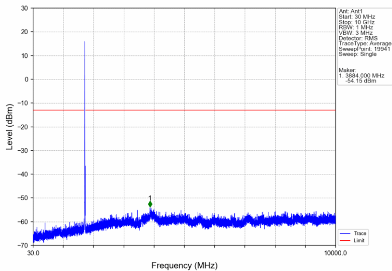
Band4_HSDPA_MCH_1732.6MHz_Subtest 1_NTNV
