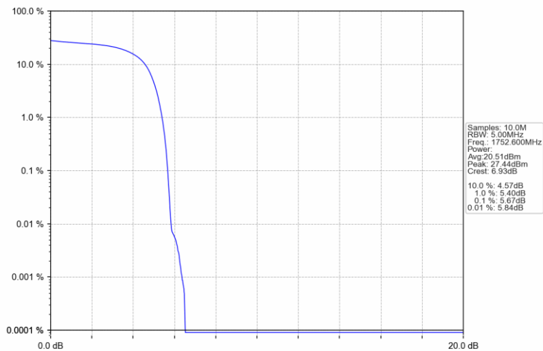
Band4_HSDPA_HCH_1752.6MHz_Subtest 1_NTNV
