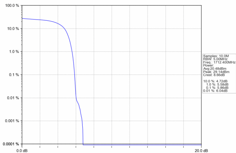
Band4_HSDPA_LCH_1712.4MHz_Subtest 1_NTNV
