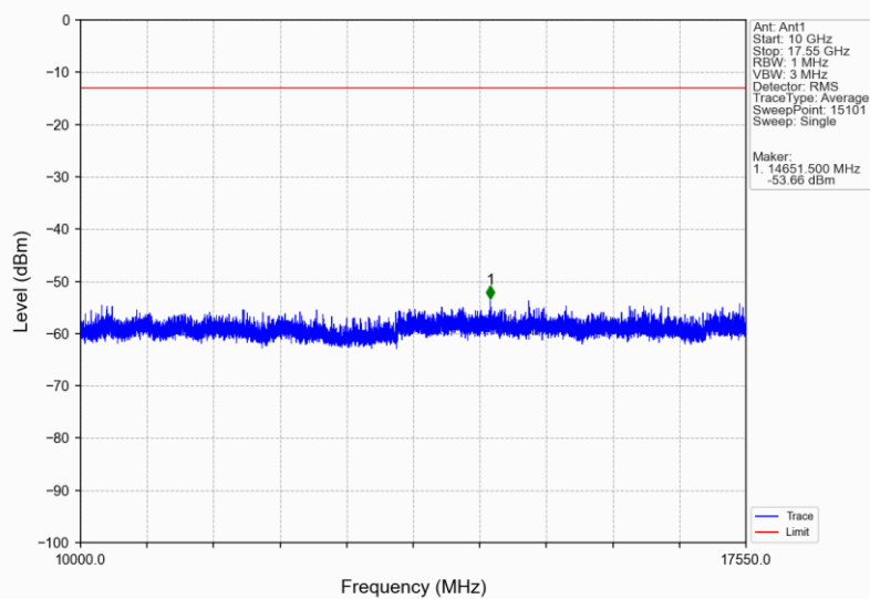
Band4_HSDPA_HCH_1752.6MHz_Subtest 1_NTNV
