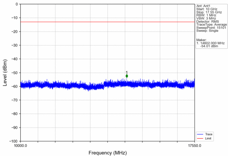
Band4_RMC_HCH_1752.6MHz_12.2kbps RMC_NTNV
