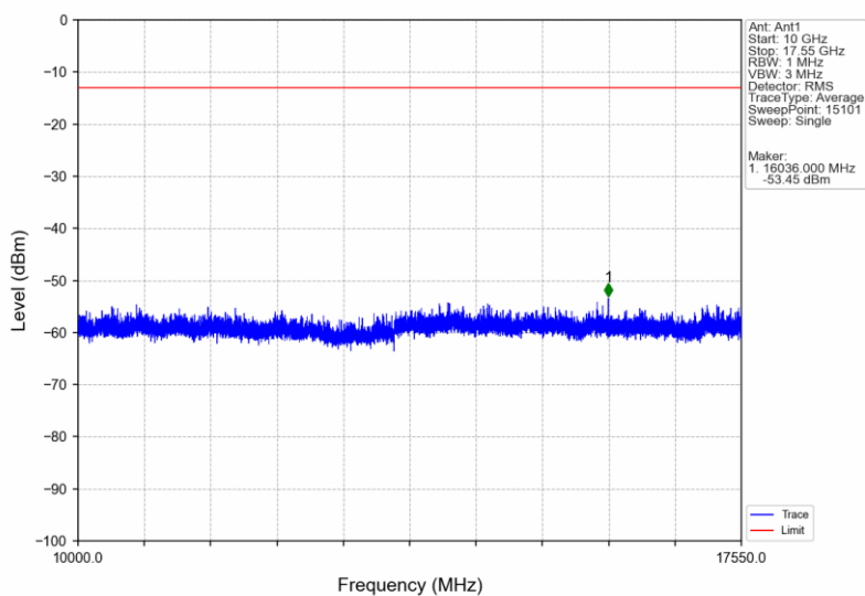
Band4_HSUPA_HCH_1752.6MHz_Subtest 1_NTNV
