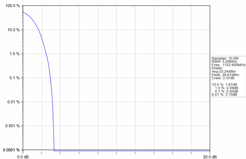
Band4_RMC_HCH_1752.6MHz_12.2kbps RMC_NTNV
