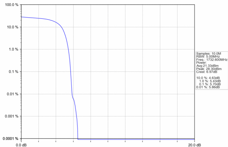
Band4_HSDPA_MCH_1732.6MHz_Subtest 1_NTNV
