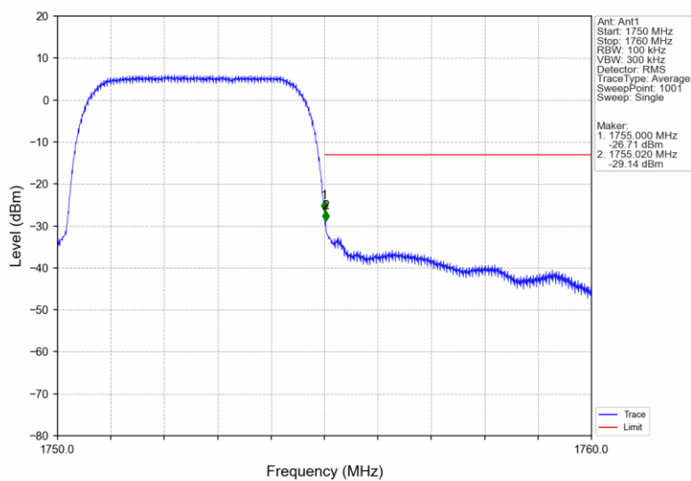
Band4_HSUPA_HCH_1752.6MHz_Subtest 1_NTNV
