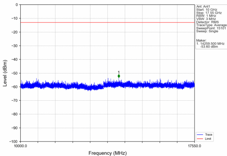
Band4_RMC_MCH_1732.6MHz_12.2kbps RMC_NTNV
