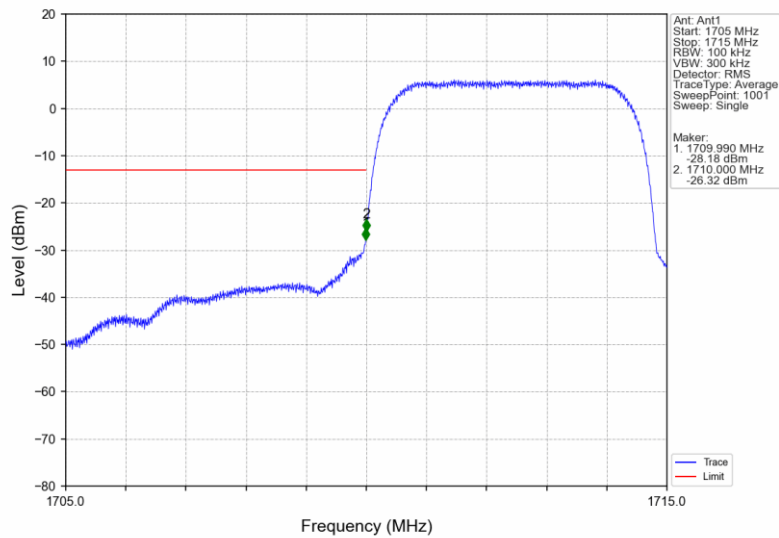
Band4_HSDPA_LCH_1712.4MHz_Subtest 1_NTNV
