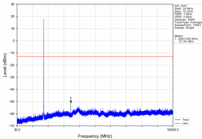
Band4_RMC_MCH_1732.6MHz_12.2kbps RMC_NTNV
