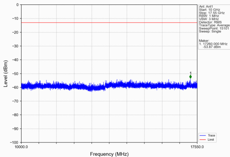
Band4_HSDPA_MCH_1732.6MHz_Subtest 1_NTNV
