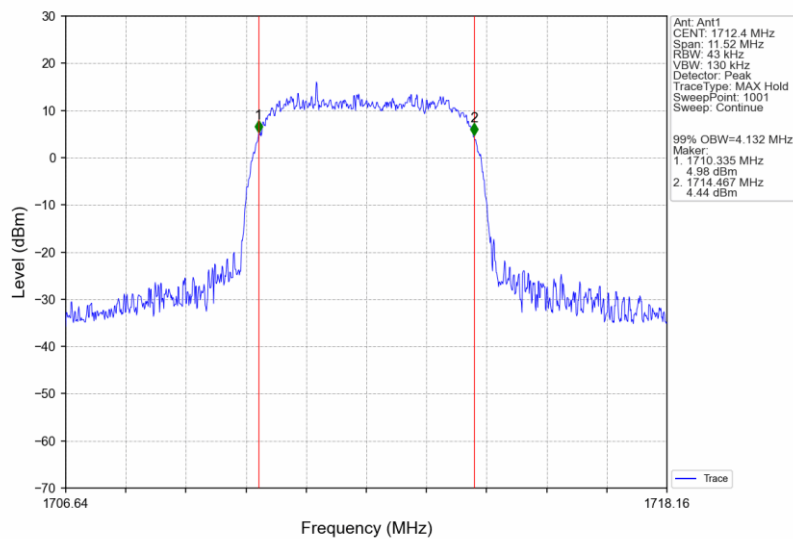
Band4_HSDPA_LCH_1712.4MHz_Subtest 1_NTNV
