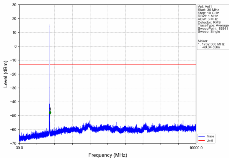
Band4_HSDPA_HCH_1752.6MHz_Subtest 1_NTNV
