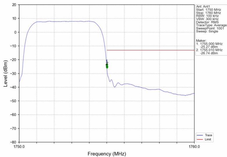
Band4_RMC_HCH_1752.6MHz_12.2kbps RMC_NTNV
