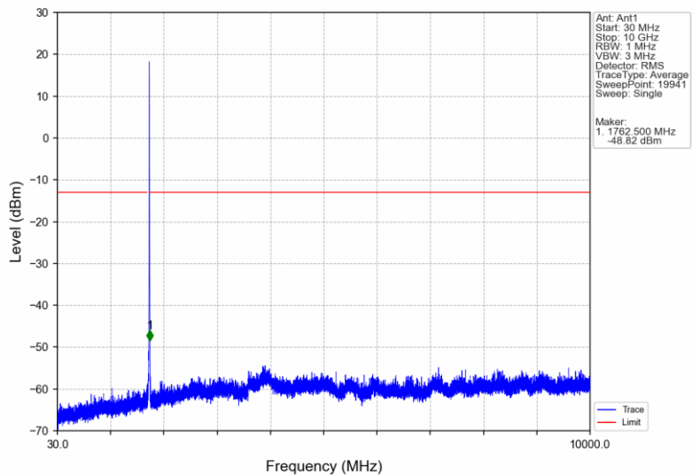
Band4_RMC_HCH_1752.6MHz_12.2kbps RMC_NTNV
