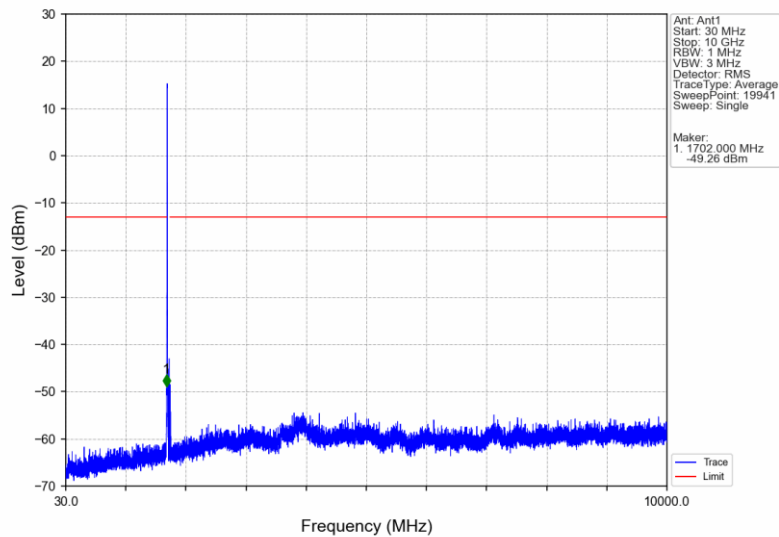
Band4_HSDPA_LCH_1712.4MHz_Subtest 1_NTNV
