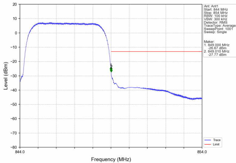
Band5_HSDPA_HCH_846.6MHz_Subtest 1_NTNV
