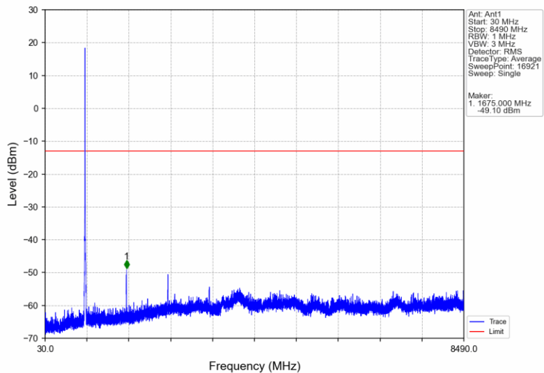
Band5_RMC_HCH_846.6MHz_12.2kbps RMC_NTNV
