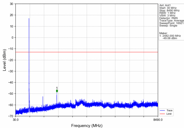
Band5_HSDPA_MCH_836.6MHz_Subtest 1_NTNV
