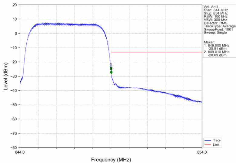
Band5_HSUPA_HCH_846.6MHz_Subtest 1_NTNV
