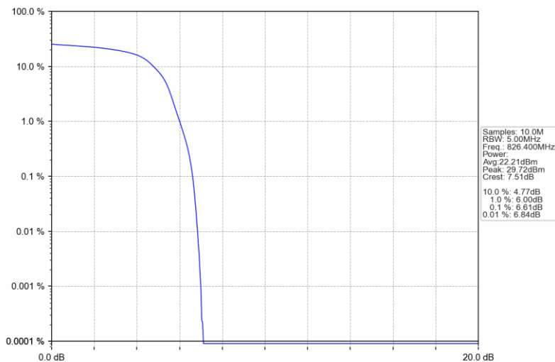
Band5_HSUPA_LCH_826.4MHz_Subtest 1_NTNV
