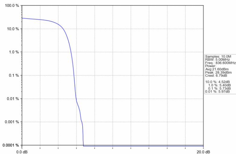
Band5_HSDPA_MCH_836.6MHz_Subtest 1_NTNV
