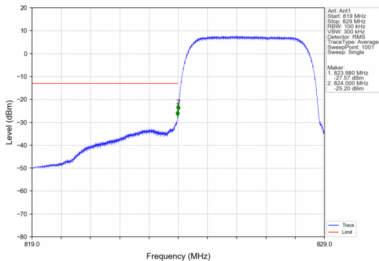
Band5_HSUPA_LCH_826.4MHz_Subtest 1_NTNV
