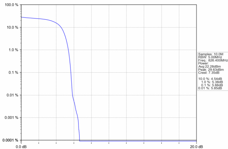
Band5_HSDPA_LCH_826.4MHz_Subtest 1 NTN
