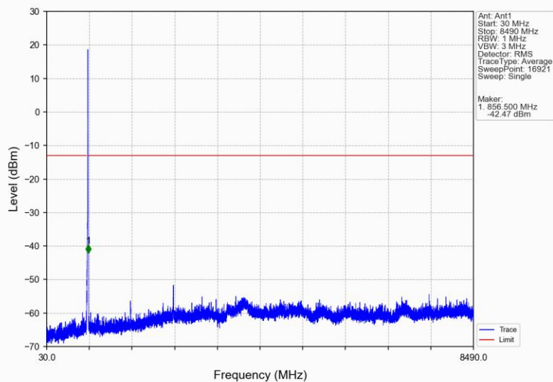
Band5_HSDPA_LCH_826.4MHz_Subtest 1 NTN
