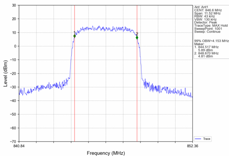
Band5_HSUPA_HCH_846.6MHz_Subtest 1_NTNV
