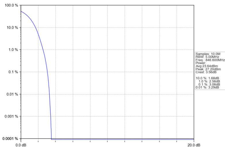
Band5_RMC_HCH_846.6MHz_12.2kbps RMC_NTNV
