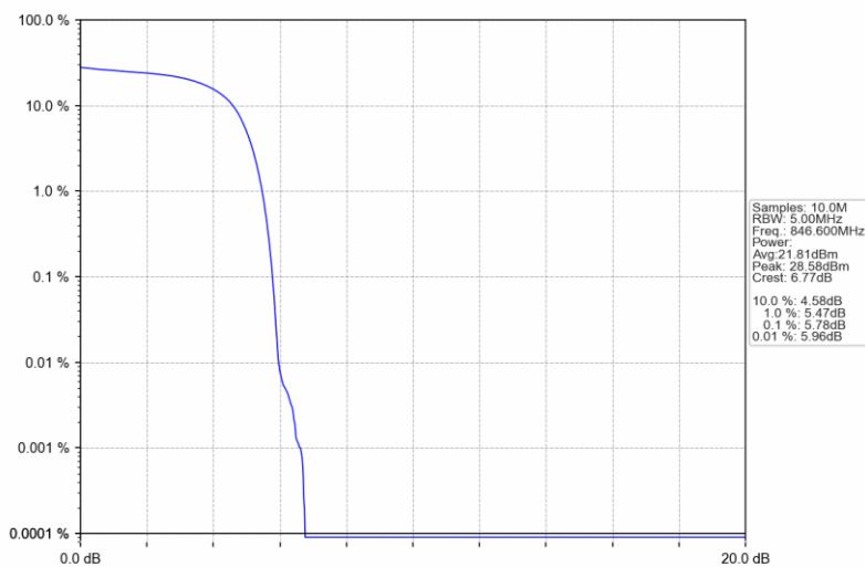
Band5_HSDPA_HCH_846.6MHz_Subtest 1_NTNV
