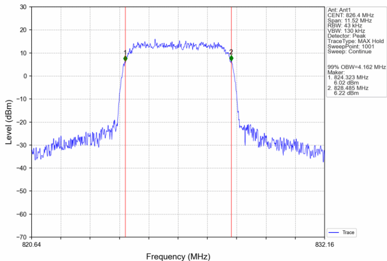
Band5_HSDPA_LCH_826.4MHz_Subtest 1 NTN
