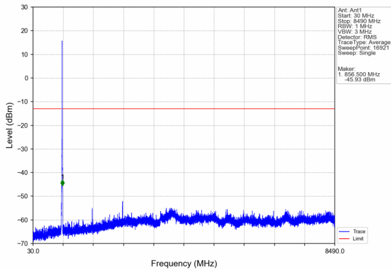
Band5_HSDPA_HCH_846.6MHz_Subtest 1_NTNV
