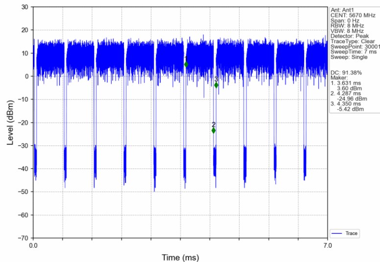
802.11ac(VHT40)_HCH_5670MHz_Ant1_NTNV
