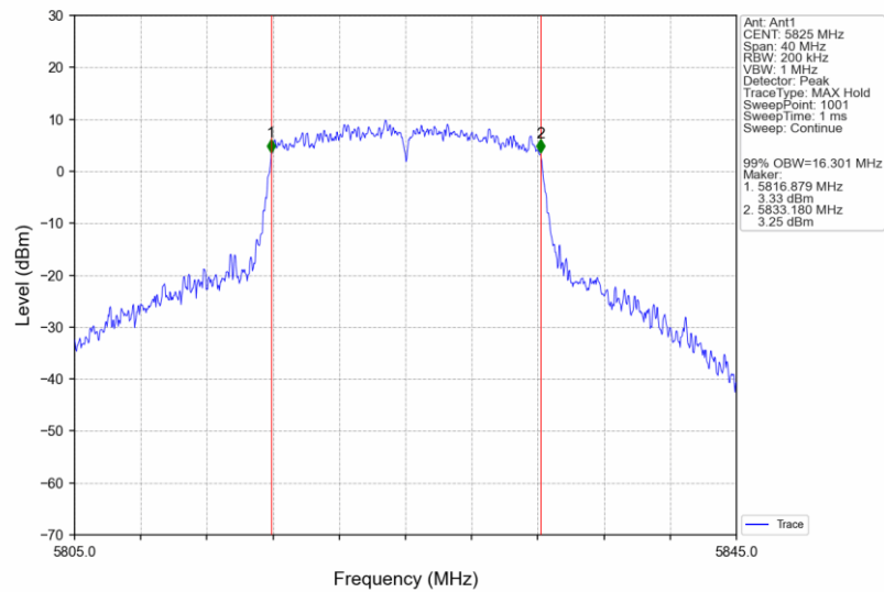
802.11a_HCH_5825MHz_Ant1_NTNV
