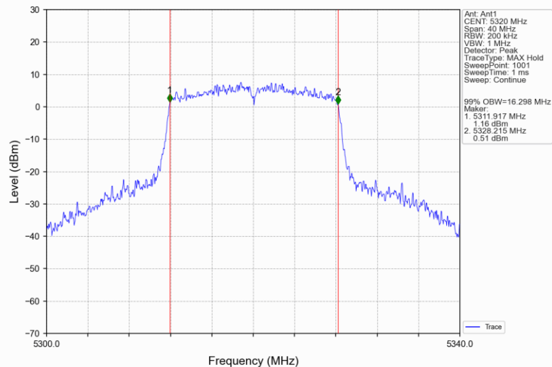
802.11a_HCH_5320MHz_Ant1_NTNV
