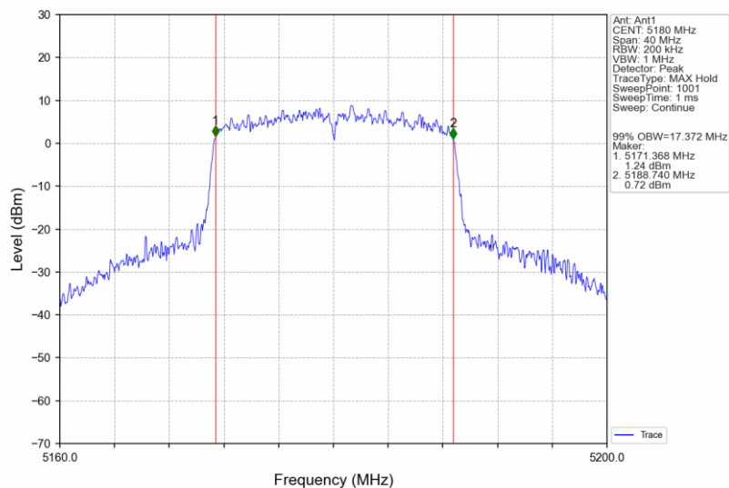
802.11ac(VHT20)_LCH_5180MHz_Ant1_NTNV
