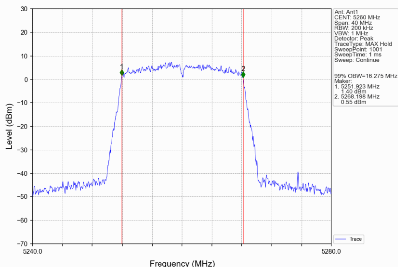
802.11a_LCH_5260MHz_Ant1_NTNV
