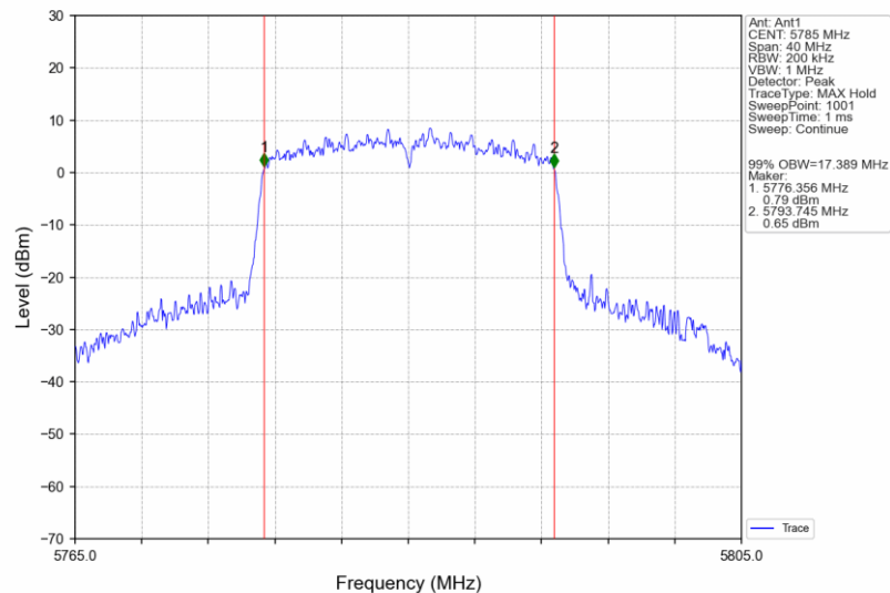
802.11ac(VHT20)_MCH_5785MHz_Ant1_NTNV
