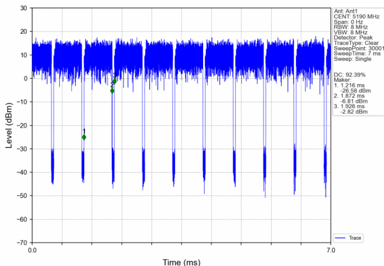
802.11ac(VHT40)_LCH_5190MHz_Ant1_NTNV
