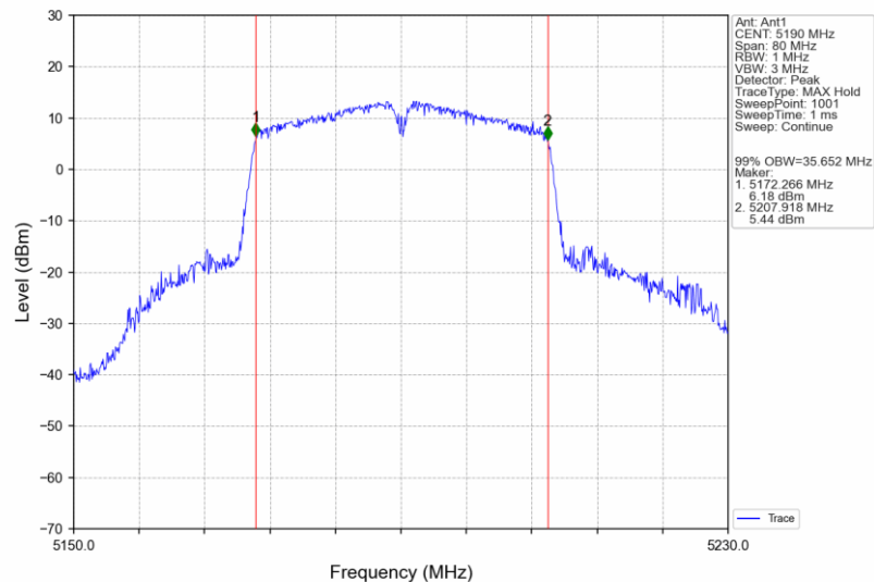
802.11ac(VHT40)_LCH_5190MHz_Ant1_NTNV
